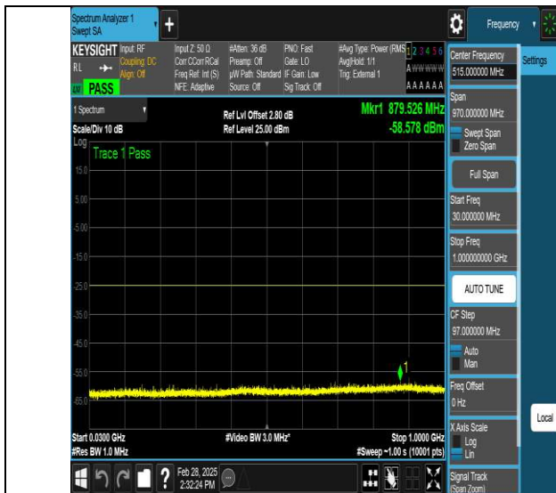
NTNV-N41-PC3-30-10-L-DFT-QPSK-Edge_1RB_Left-Ant1-PASS
