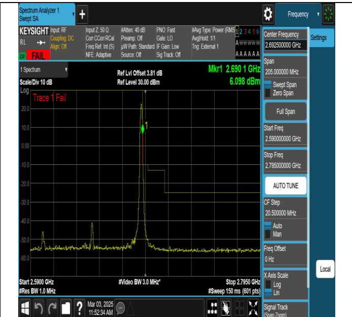
NTNV-N41-PC3-30-90-H-DFT-QPSK-Edge_1RB_Right-Ant1- FAIL
