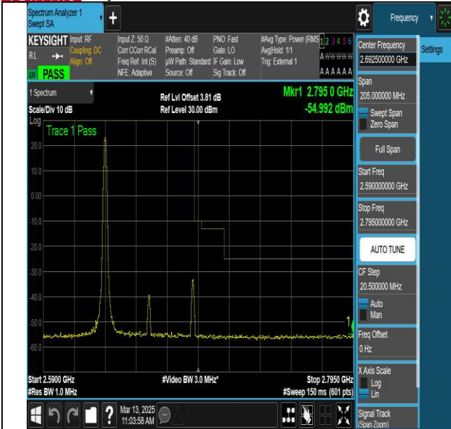
NTNV-N41-PC3-30-60-H-DFT-QPSK-Edge_1RB_Left-Ant1- PASS
