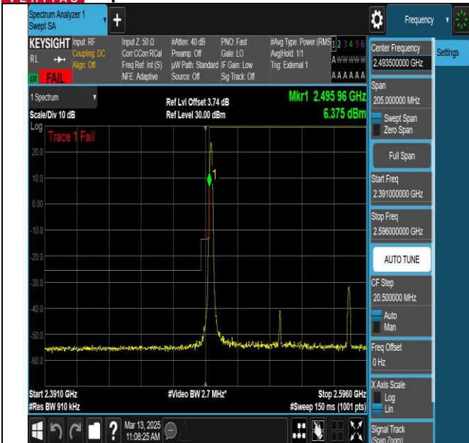
NTNV-N41-PC3-30-90-L-DFT-QPSK-Edge_1RB_Left-Ant1- FAIL
