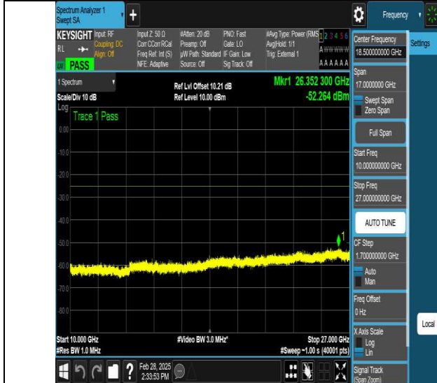
NTNV-N41-PC3-30-10-L-DFT-QPSK-Edge_1RB_Left-Ant1-PASS
