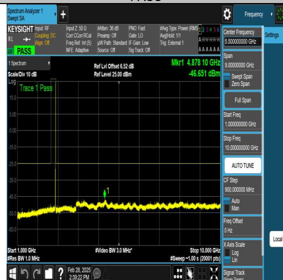
NTNV-N41-PC3-30-10-H-DFT-QPSK-Edge_1RB_Left-Ant1-PASS
