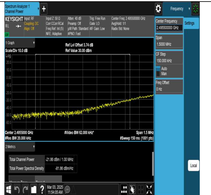
NTNV-N41-PC3-30-100-L-DFT-QPSK-Edge_1RB_Left-Ant1- PASS
