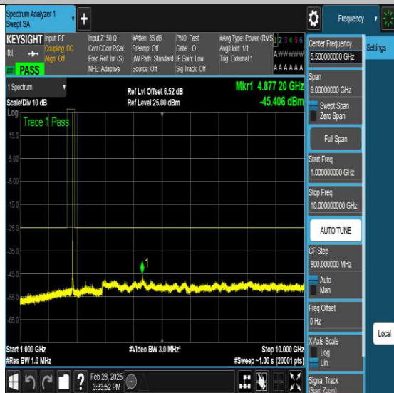
NTNV-N41-PC3-30-30-H-DFT-QPSK-Edge_1RB_Left-Ant1-PASS
