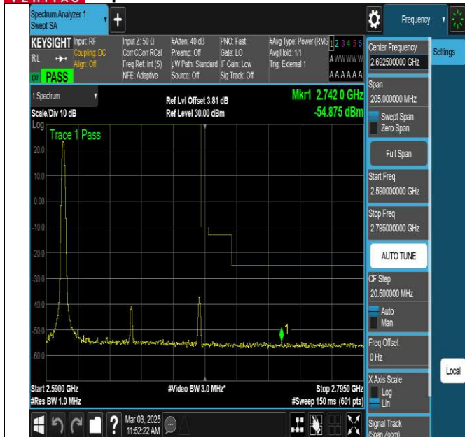
NTNV-N41-PC3-30-90-H-DFT-QPSK-Edge_1RB_Left-Ant1- PASS
