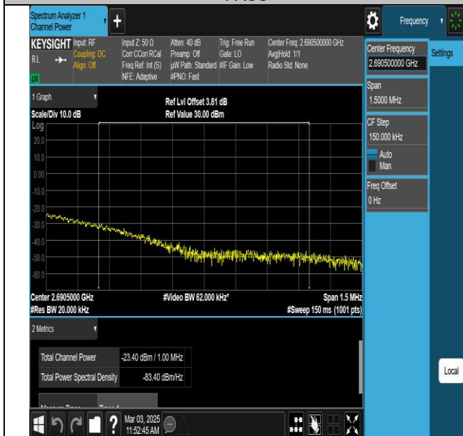
NTNV-N41-PC3-30-90-H-DFT-QPSK-Edge_1RB_Right-Ant1- PASS
