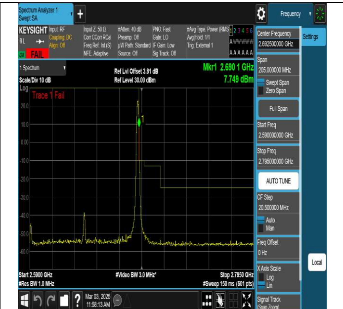
NTNV-N41-PC3-30-100-H-DFT-QPSK-Edge_1RB_Right-Ant1- FAIL
