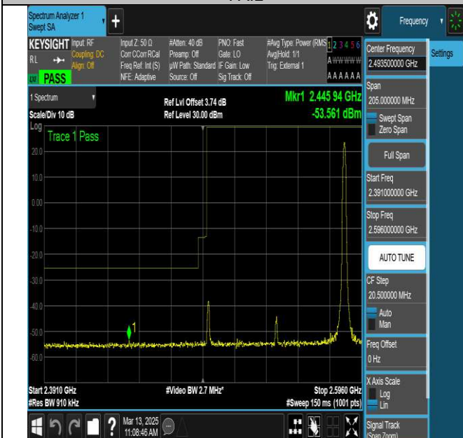
NTNV-N41-PC3-30-90-L-DFT-QPSK-Edge_1RB_Right-Ant1- PASS
