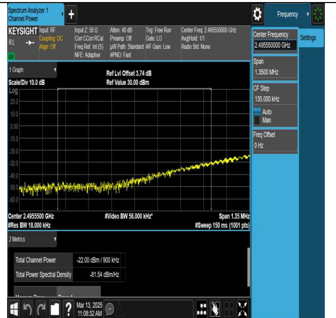
NTNV-N41-PC3-30-90-L-DFT-QPSK-Edge_1RB_Left-Ant1- PASS
