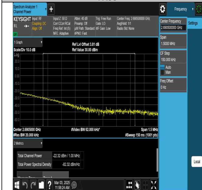
NTNV-N41-PC3-30-100-H-DFT-QPSK-Edge_1RB_Right-Ant1- PASS
