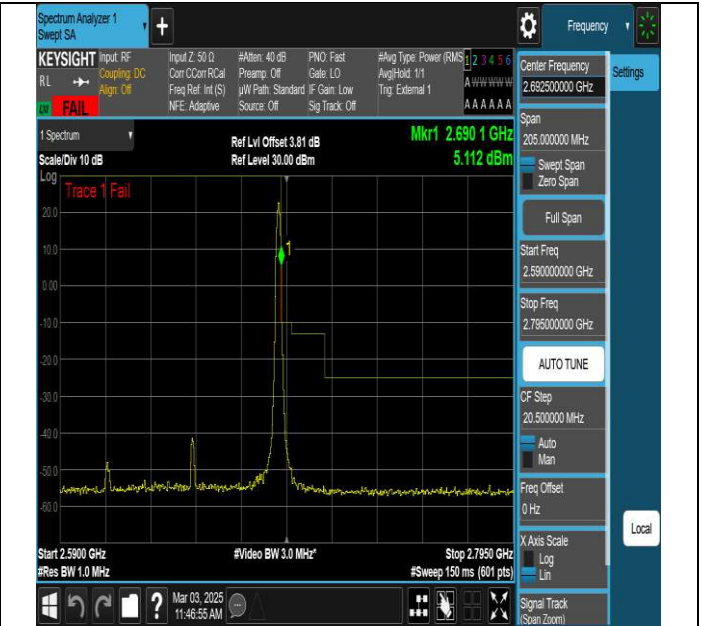
NTNV-N41-PC3-30-80-H-DFT-QPSK-Edge_1RB_Right-Ant1- FAIL
