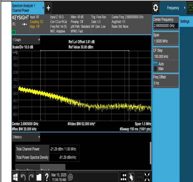
NTNV-N41-PC3-30-60-H-DFT-QPSK-Edge_1RB_Right-Ant1- PASS
