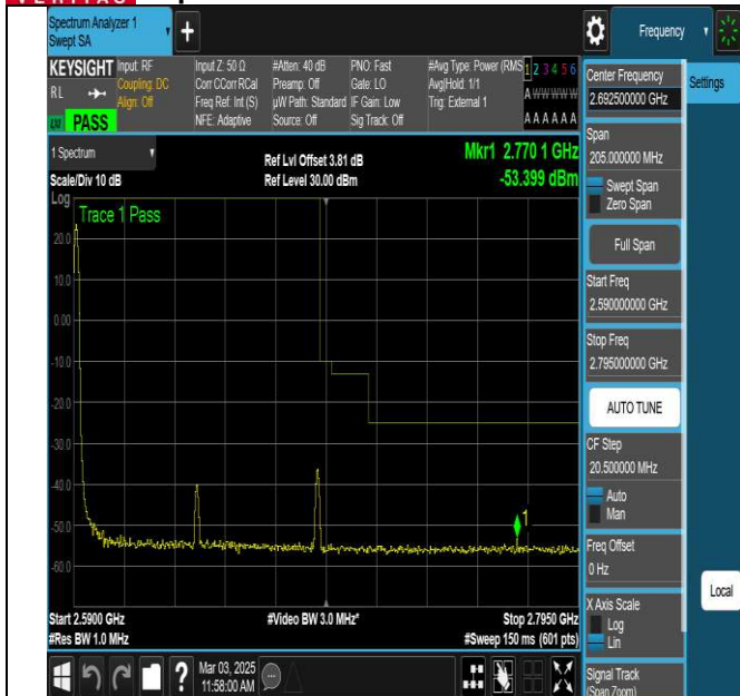
NTNV-N41-PC3-30-100-H-DFT-QPSK-Edge_1RB_Left-Ant1- PASS
