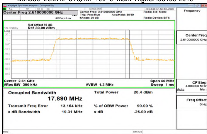
Band38_20MHz_64QAM_100_0_Main_HighCH38150-2610
