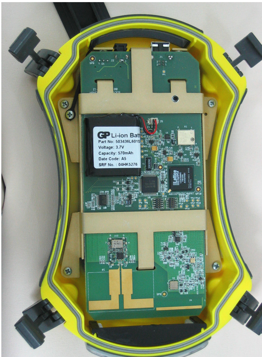
Photograph No.1 FP200HH handheld reader Internal view
