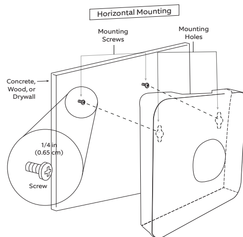
Fig. 1: Horizontal Mounting
