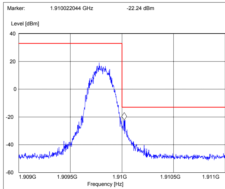
Picture 6 Upper bandedge, EGPRS 1900 channel 810, flip closed
