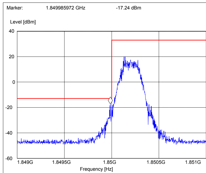
Picture 9 Lower bandedge, EGPRS 1900 channel 512, flip open
