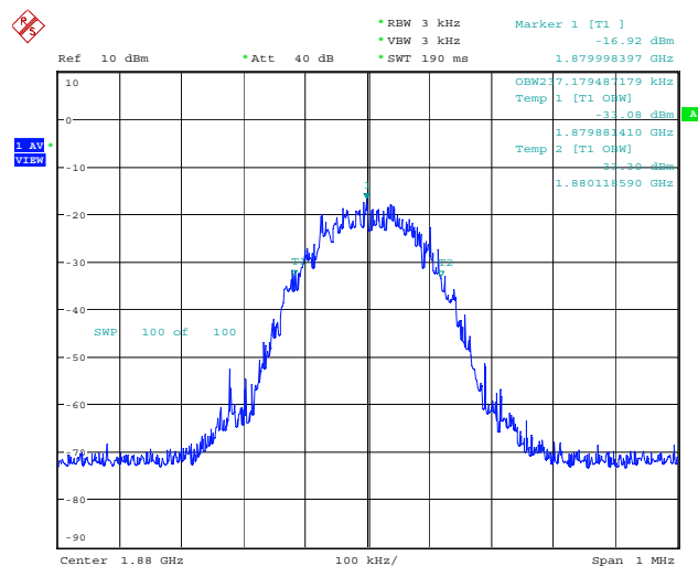
Picture 1 99% occupied bandwidth, GSM channel 661
