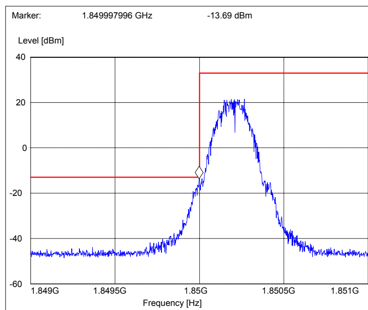
Picture 7 Lower bandedge, GSM 1900 channel 512, flip open
