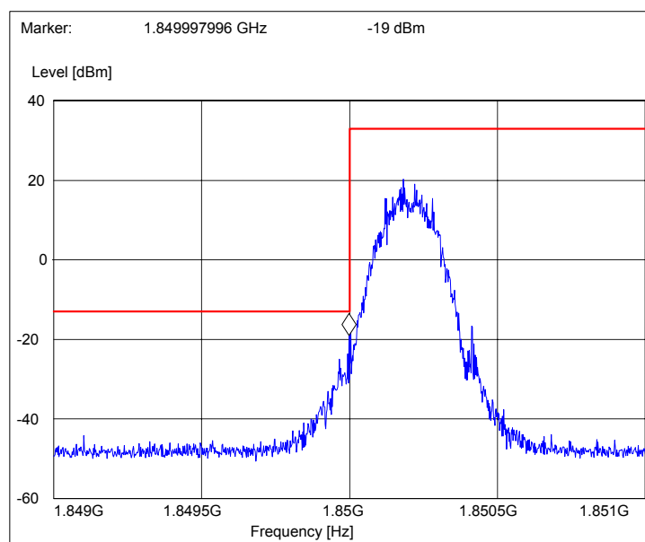
Picture 5 Lower bandedge, EGPRS 1900 channel 512, flip closed
