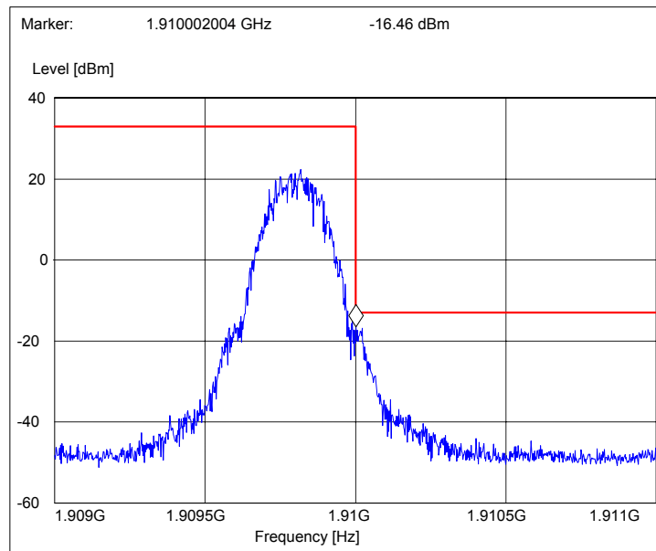
Picture 4 Upper bandedge, GSM 1900 channel 810, flip closed
