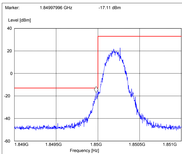
Picture 3 Lower bandedge, GSM 1900 channel 512, flip closed
