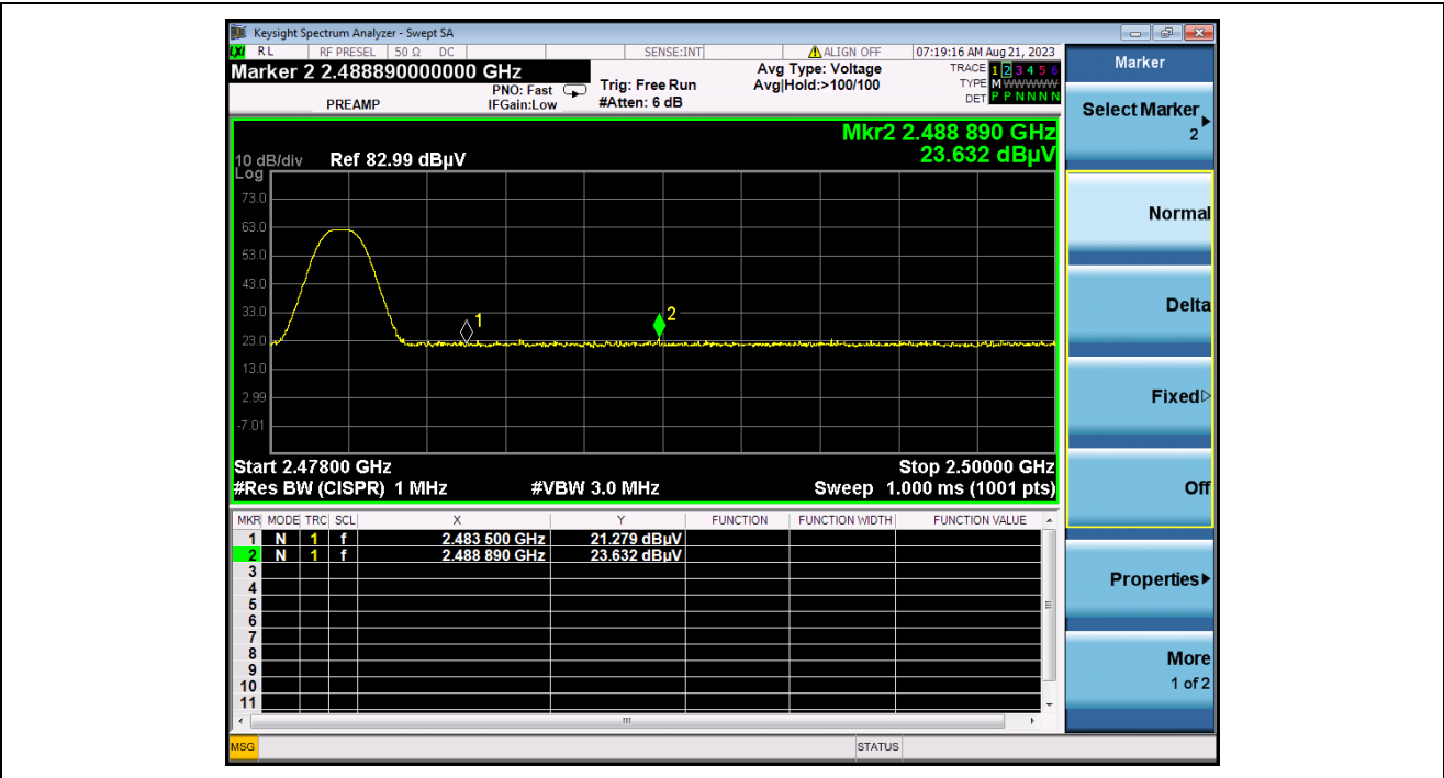
(PEAK, Channel 78, GFSK)
