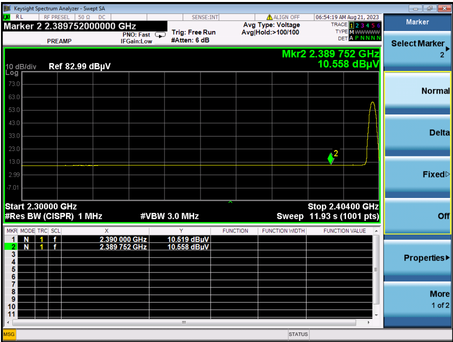
(AVERAGE, Channel 0, 8-DPSK)
