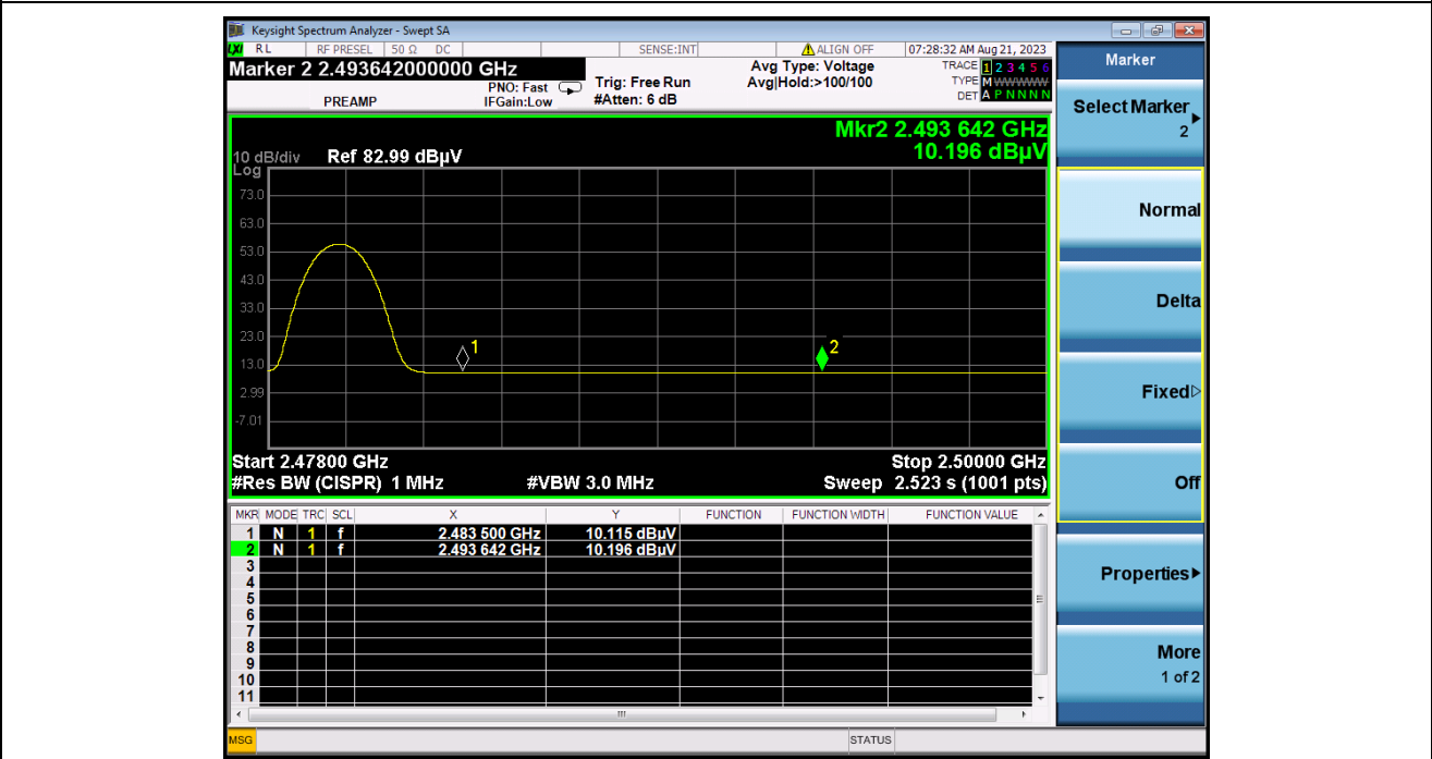
(AVERAGE, Channel 78, 8-DPSK)
