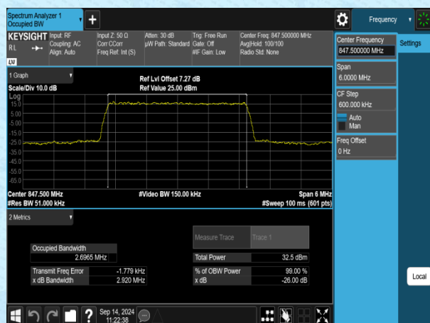
Band5-3MHz-QPSK-20635-15RB#0-PASS
