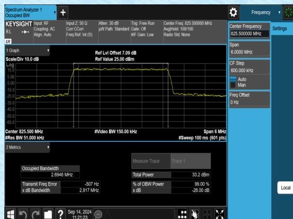
Band5-3MHz-QPSK-20415-15RB#0-PASS
