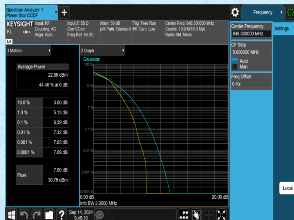
Band5-1.4MHz-16QAM-20643-6RB#0-PASS
