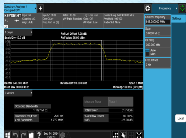
Band5-1.4MHz-16QAM-20643-6RB#0-PASS
