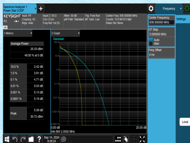
Band5-1.4MHz-QPSK-20525-1RB#0-PASS
