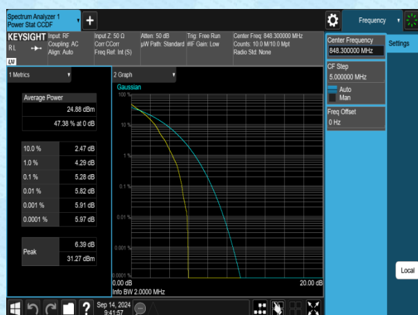
Band5-1.4MHz-QPSK-20643-1RB#0-PASS
