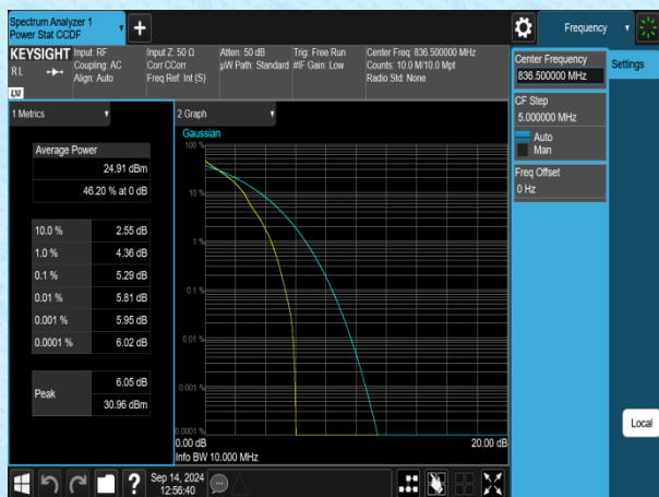
Band5-10MHz-QPSK-20525-1RB#0-PASS
