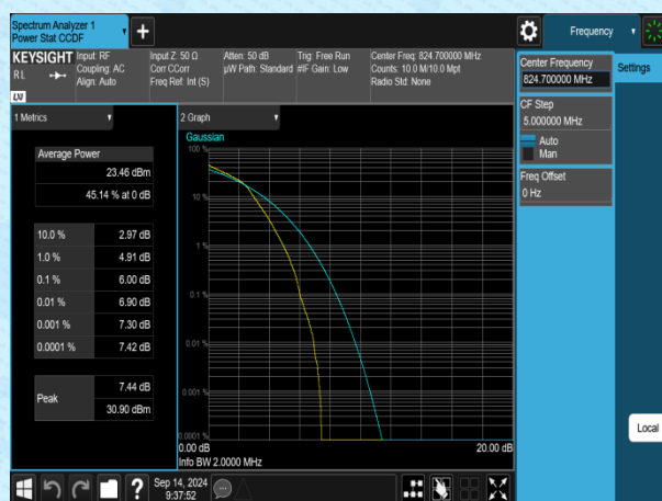
Band5-1.4MHz-16QAM-20407-6RB#0-PASS
