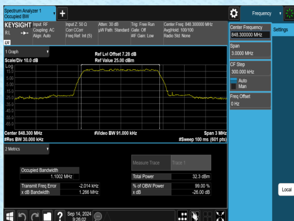
Band5-1.4MHz-QPSK-20643-6RB#0-PASS
