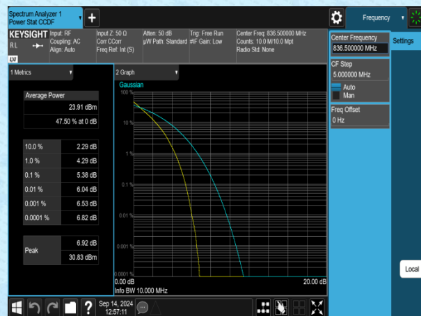
Band5-10MHz-QPSK-20525-50RB#0-PASS
