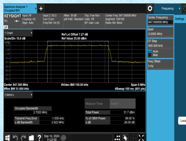
Band5-3MHz-16QAM-20635-15RB#0-PASS
