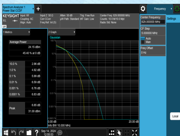
Band5-10MHz-16QAM-20450-1RB#0-PASS
