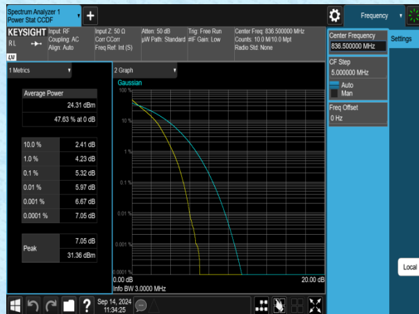
Band5-3MHz-QPSK-20525-15RB#0-PASS
