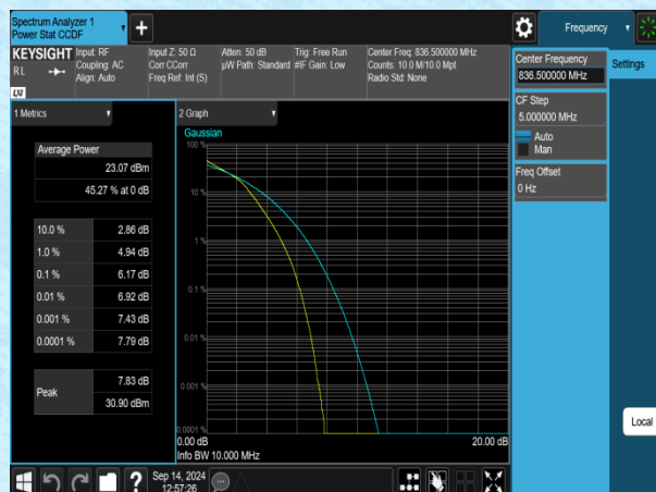
Band5-10MHz-16QAM-20525-50RB#0-PASS
