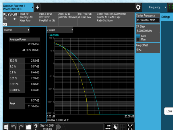
Band5-3MHz-16QAM-20635-15RB#0-PASS
