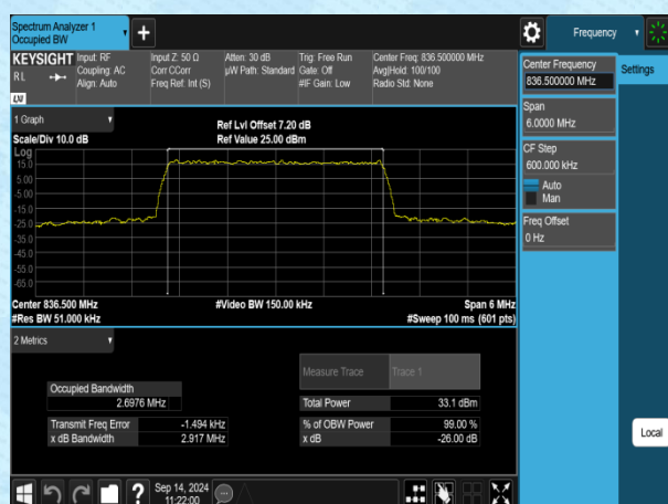
Band5-3MHz-QPSK-20525-15RB#0-PASS
