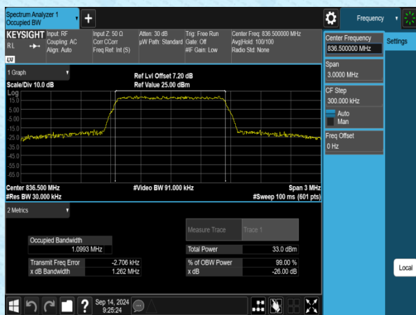
Band5-1.4MHz-QPSK-20525-6RB#0-PASS
