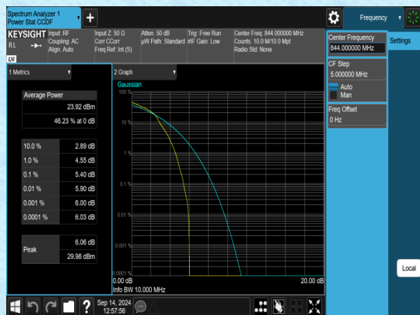
Band5-10MHz-16QAM-20600-1RB#0-PASS
