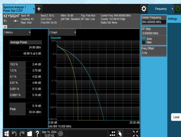
Band5-10MHz-QPSK-20600-1RB#0-PASS
