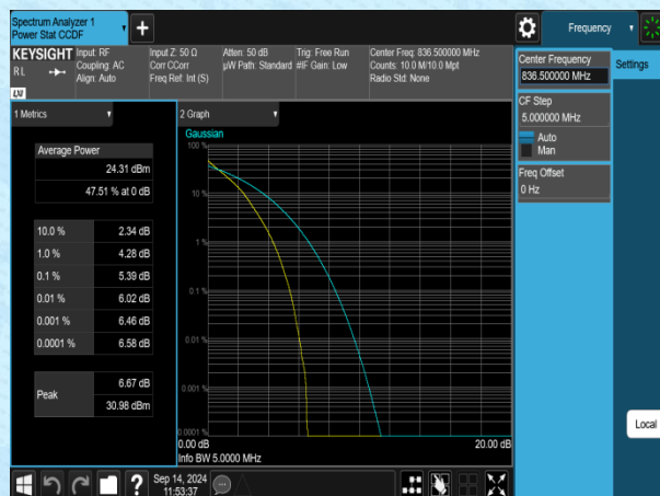
Band5-5MHz-QPSK-20525-25RB#0-PASS
