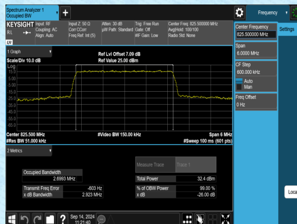
Band5-3MHz-16QAM-20415-15RB#0-PASS
