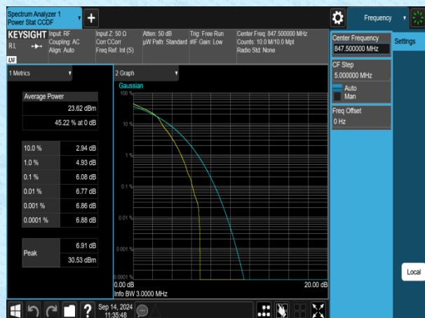
Band5-3MHz-16QAM-20635-1RB#0-PASS
