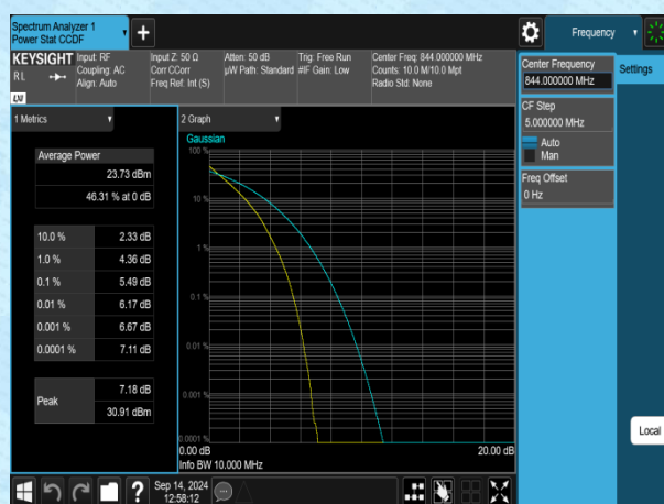
Band5-10MHz-QPSK-20600-50RB#0-PASS
