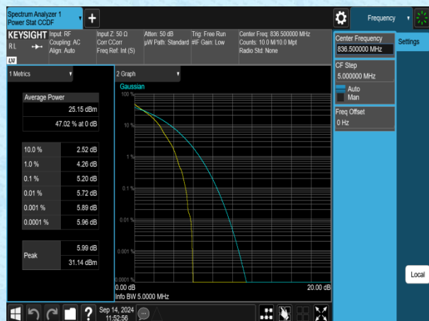
Band5-5MHz-QPSK-20525-1RB#0-PASS
