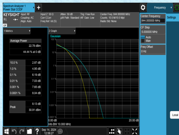
Band5-10MHz-16QAM-20600-50RB#0-PASS
