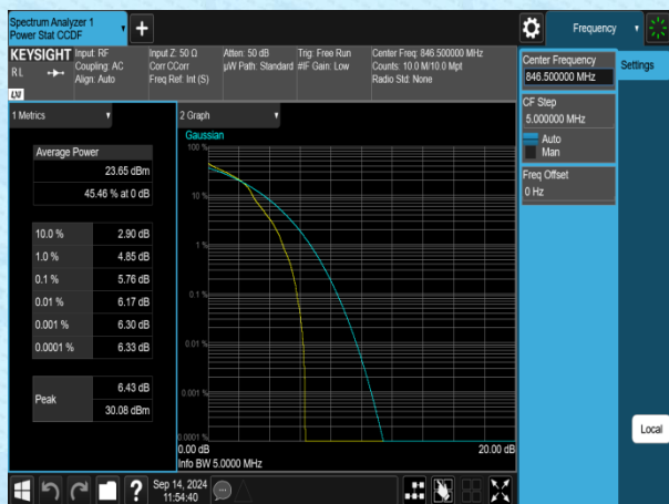
Band5-5MHz-16QAM-20625-1RB#0-PASS
