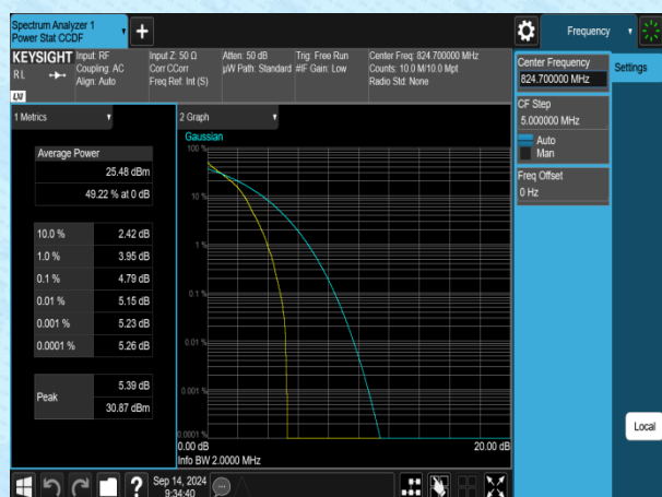
Band5-1.4MHz-QPSK-20407-1RB#0-PASS
