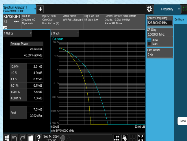
Band5-5MHz-16QAM-20425-25RB#0-PASS
