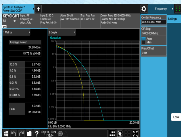
Band5-3MHz-16QAM-20415-1RB#0-PASS
