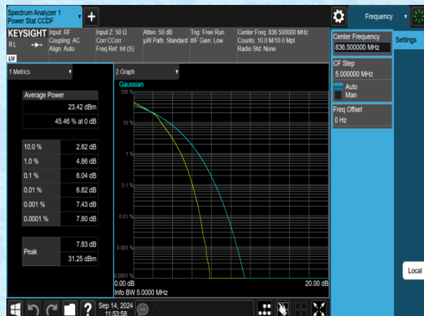
Band5-5MHz-16QAM-20525-25RB#0-PASS
