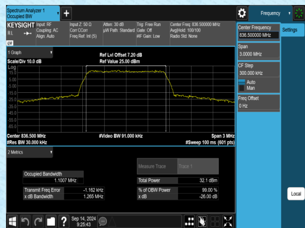
Band5-1.4MHz-16QAM-20525-6RB#0-PASS
