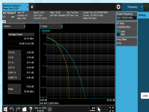
Band5-1.4MHz-16QAM-20407-1RB#0-PASS
