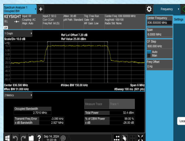
Band5-3MHz-16QAM-20525-15RB#0-PASS
