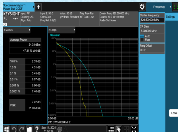
Band5-5MHz-QPSK-20425-25RB#0-PASS
