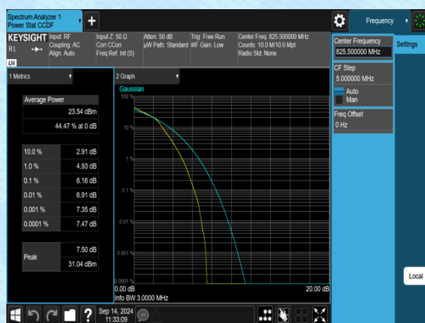
Band5-3MHz-16QAM-20415-15RB#0-PASS
