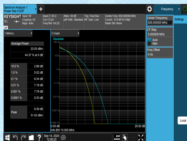
Band5-10MHz-16QAM-20450-50RB#0-PASS
