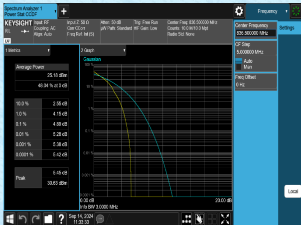
Band5-3MHz-QPSK-20525-1RB#0-PASS
