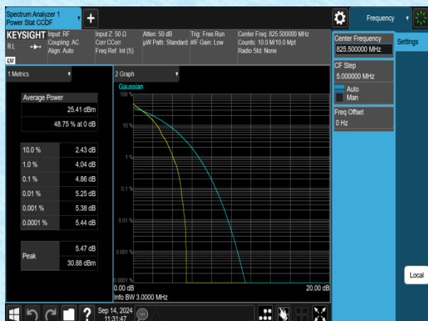
Band5-3MHz-QPSK-20415-1RB#0-PASS
