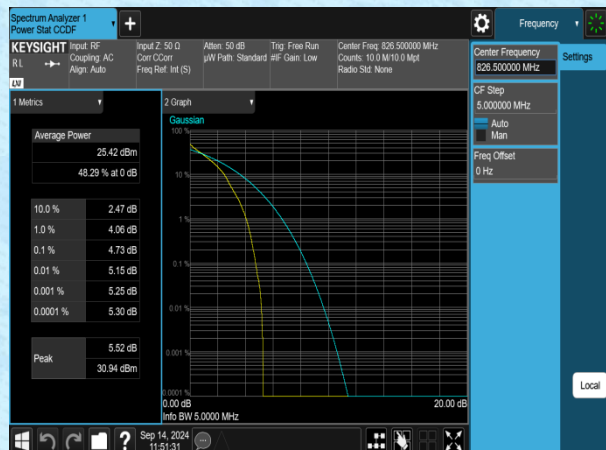
Band5-5MHz-QPSK-20425-1RB#0-PASS
