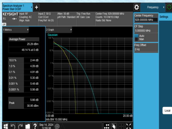
Band5-10MHz-QPSK-20450-1RB#0-PASS
