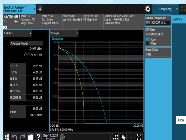
Band5-3MHz-QPSK-20635-1RB#0-PASS
