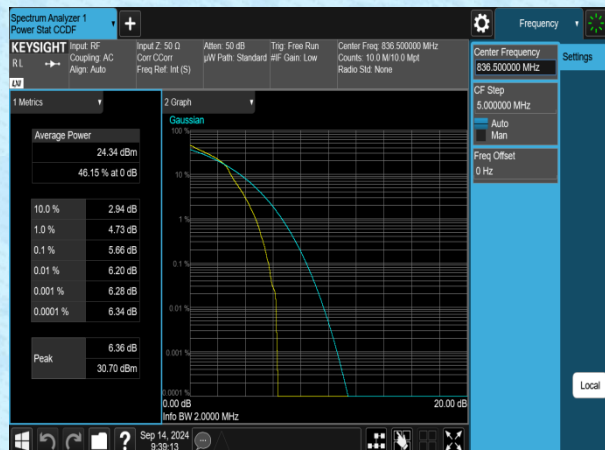
Band5-1.4MHz-16QAM-20525-1RB#0-PASS
