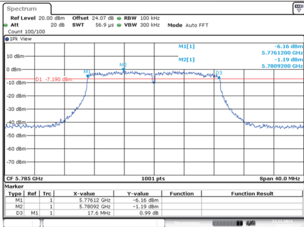
11AC20MIMO-Ant1-5785-PASS
