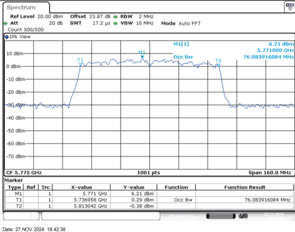
11AC80MIMO-Ant2-5775
