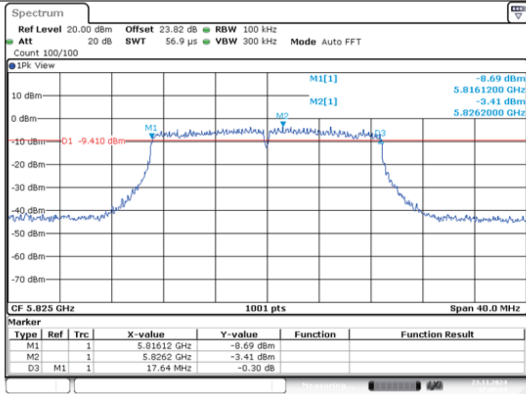
11AC20MIMO-Ant1-5825-PASS
