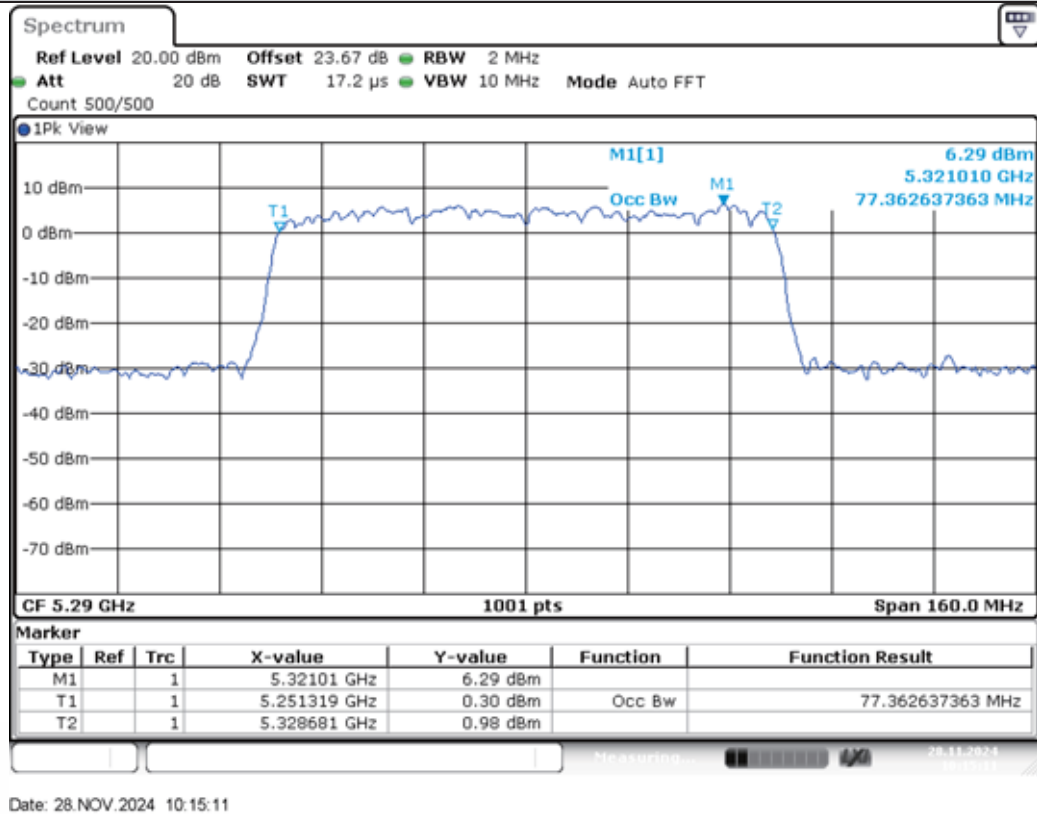
11AX80MIMO-Ant2-5290
