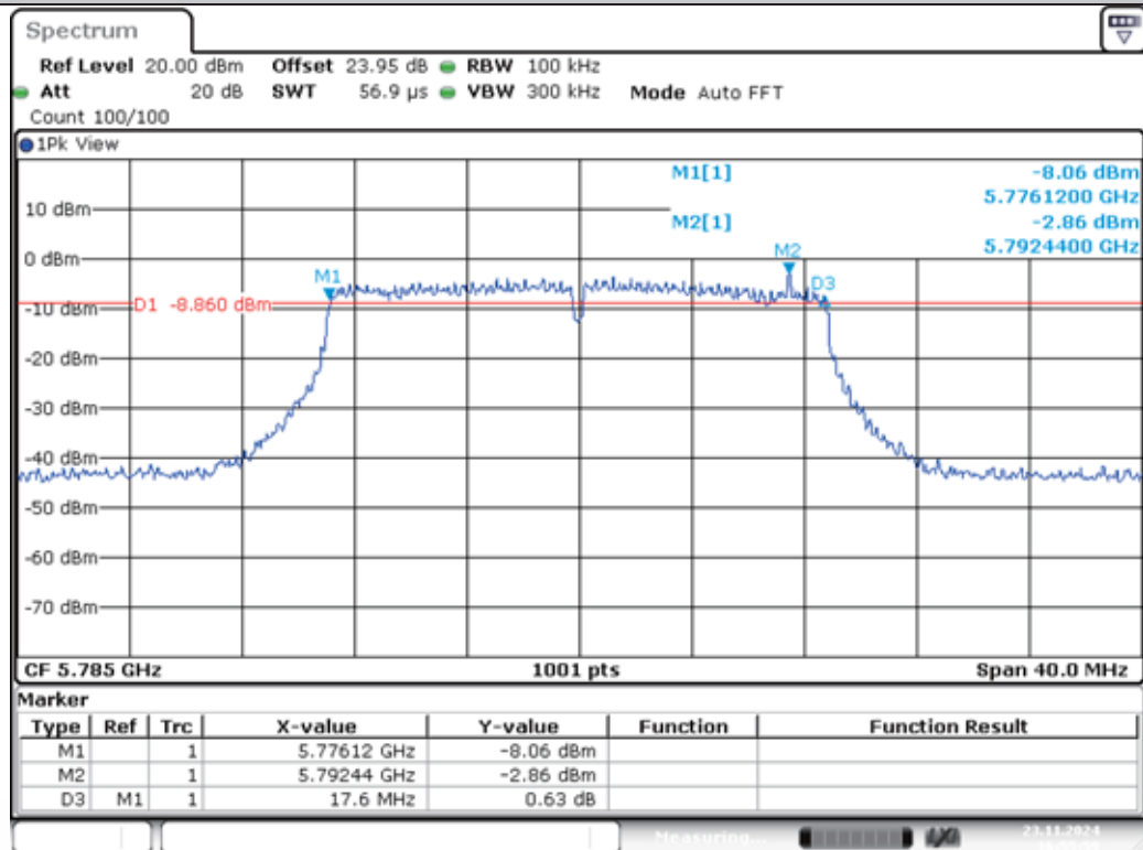
11AC20MIMO-Ant1-5785-PASS
