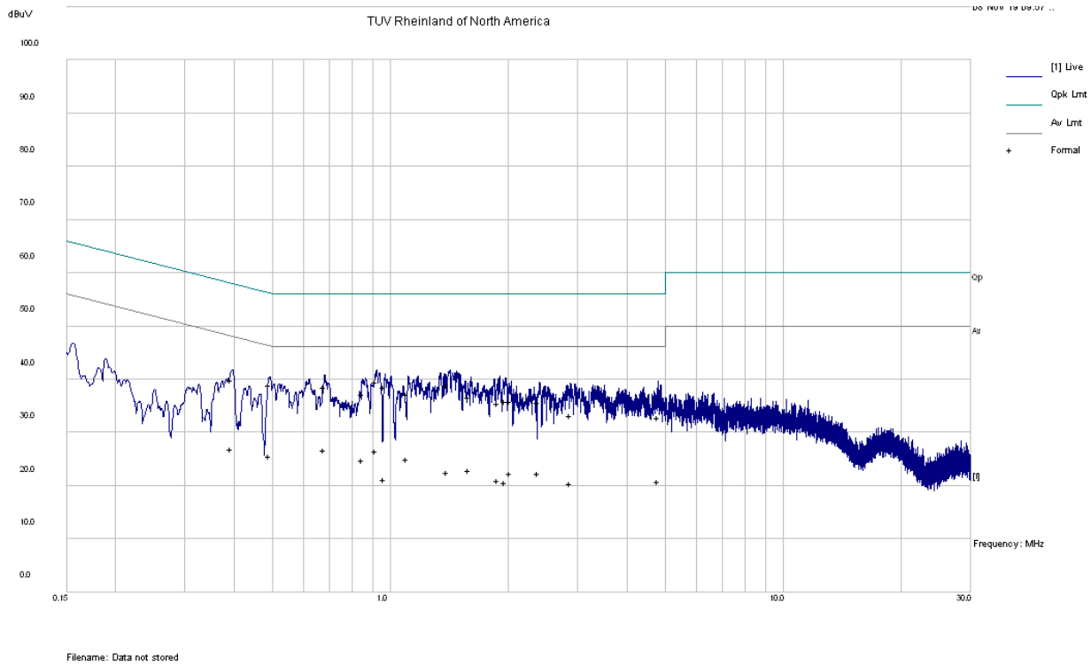
Conducted Emissions .150-30 MHz. 110VAC line
