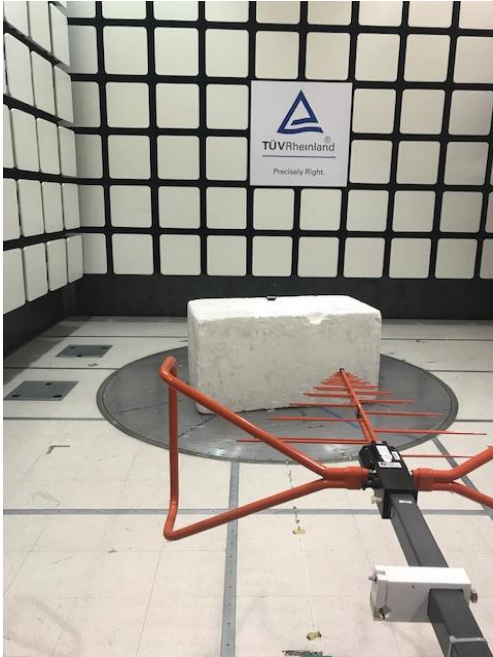
Figure 1 - Radiated Emissions Setup 30 - 1000 MHz - Front
