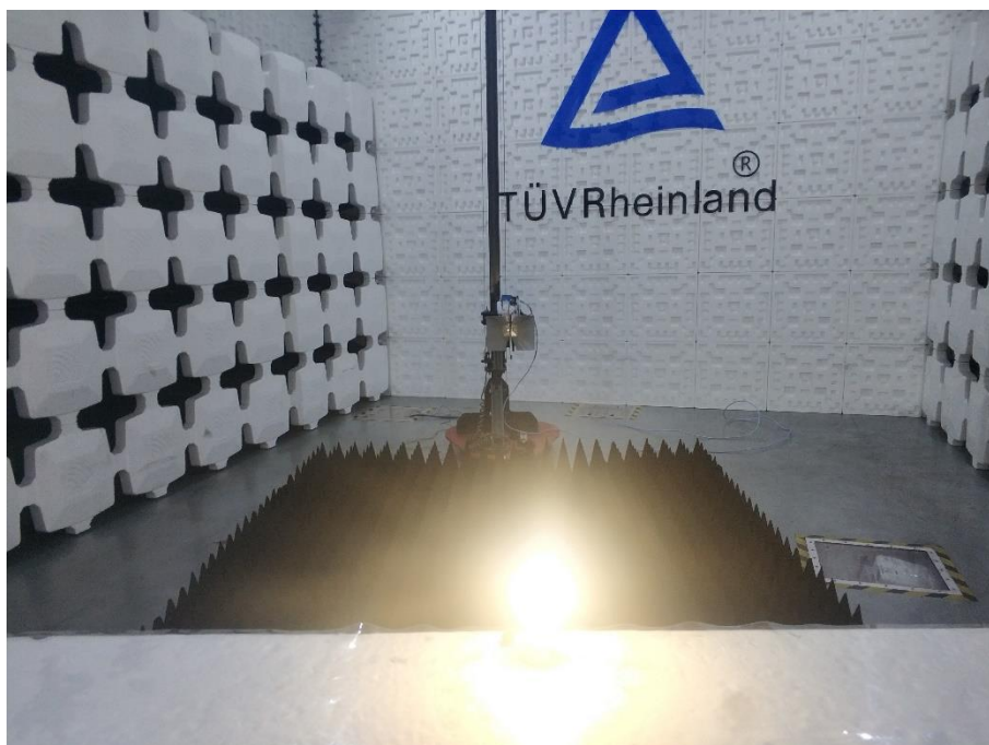
Photograph 4: Set-up for Radiated Emission, Above 1GHz
