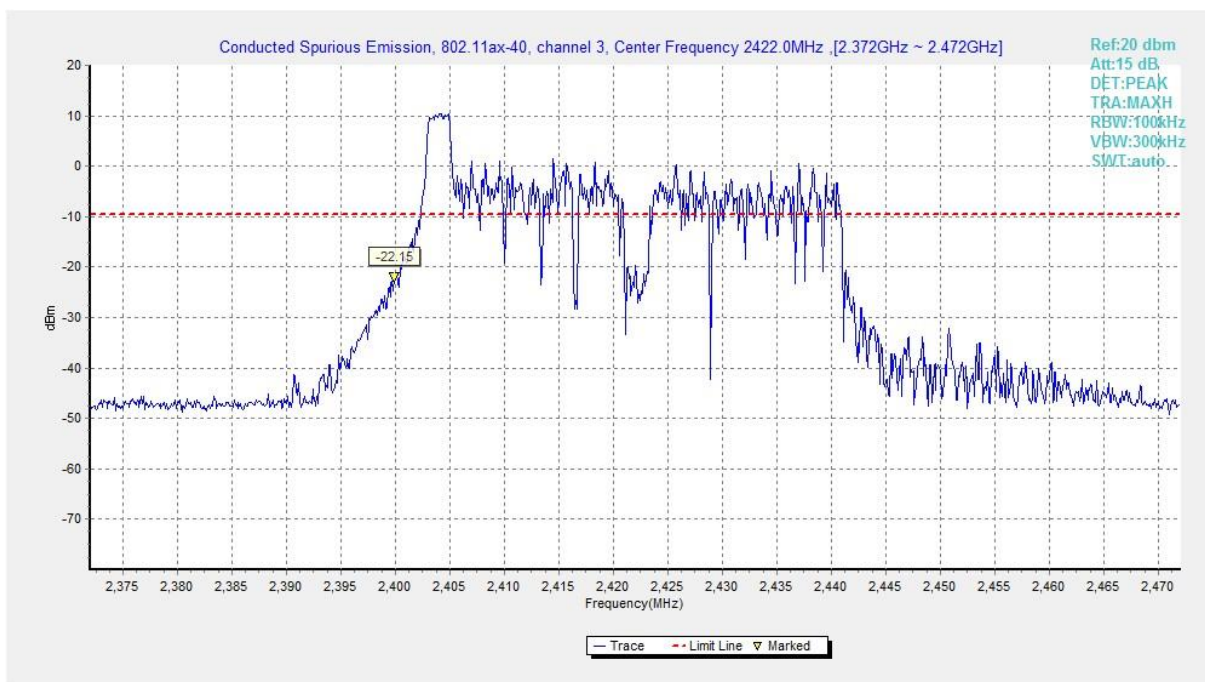
Fig.A.6.1.217 Transmitter Spurious Emission - Conducted (802.11ax-HE40, Ch3, Center Frequency)
