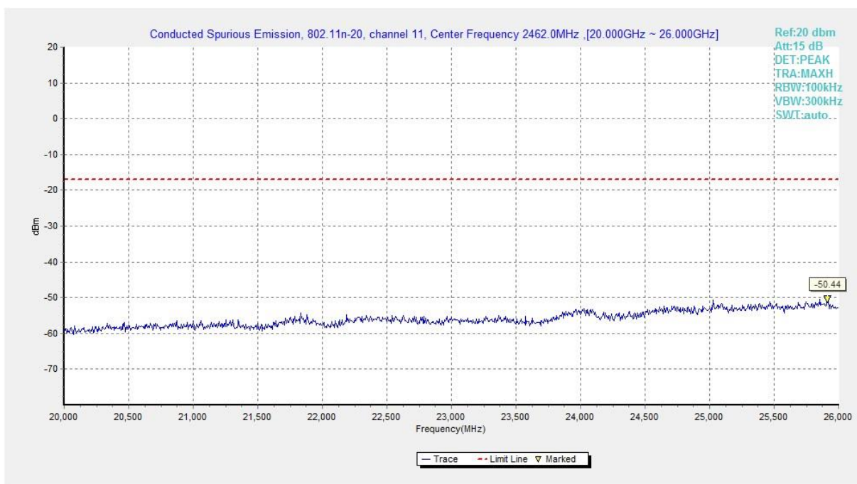
Fig.A.6.1.264 Transmitter Spurious Emission - Conducted (802.11n-HT20, Ch11, 20 GHz-26 GHz)
