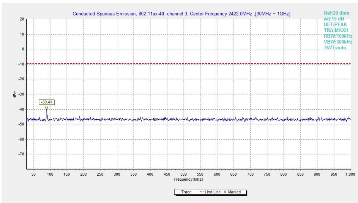
Fig.A.6.1.218 Transmitter Spurious Emission - Conducted (802.11ax-HE40, Ch3, 30 MHz-1 GHz)
