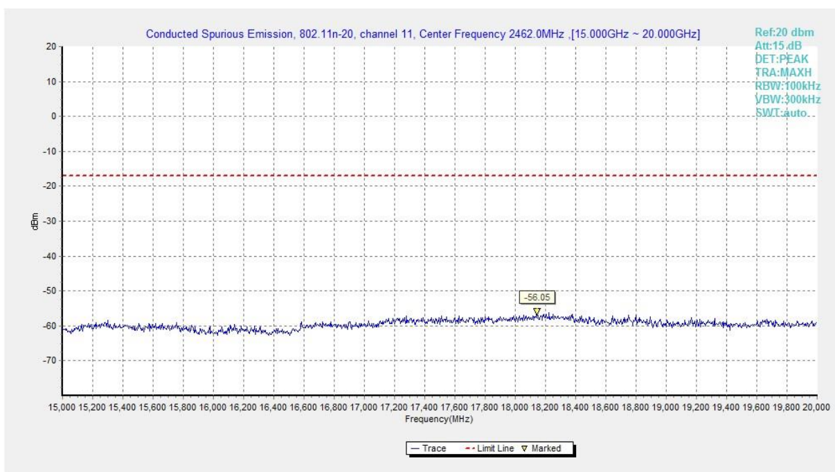
Fig.A.6.1.263 Transmitter Spurious Emission - Conducted (802.11n-HT20, Ch11, 15 GHz-20 GHz)
