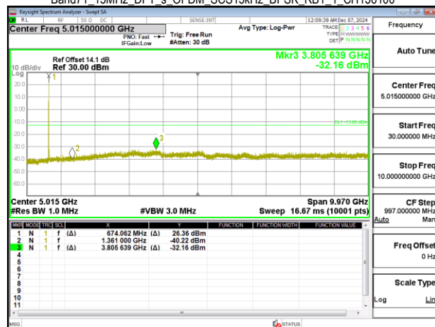
Band71 15MHz DFT s OFDM_SCS15kHz BPSK RB1 1 CH138100
