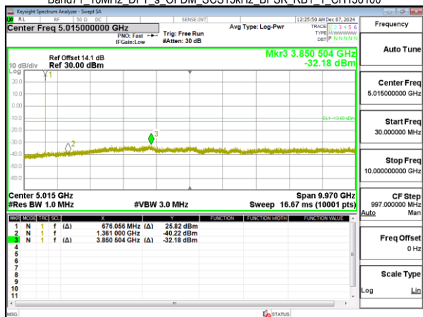
Band71 10MHz DFT s OFDM_SCS15kHz BPSK RB1 1 CH13600
