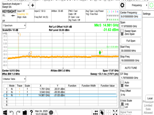
Band66_20MHz_DFT_s_OFDM_SCS15kHz_BPSK_RB1_1_CH354000_below 18G
