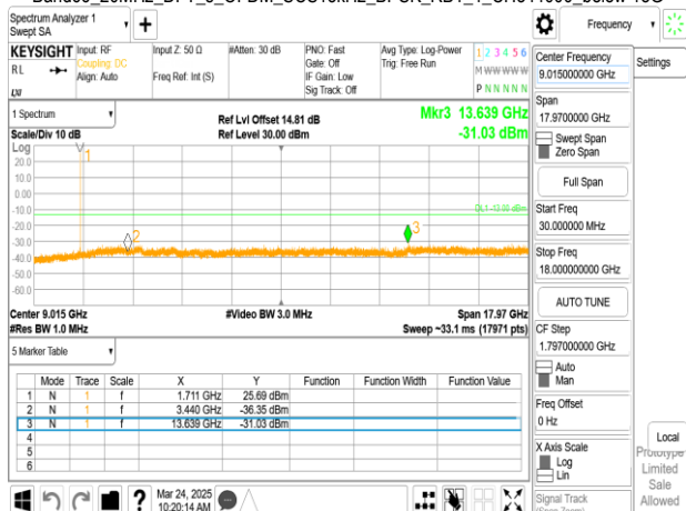
Band66_20MHz_DFT_s_OFDM_SCS15kHz_BPSK_RB1_1_CH349000_below 18G
