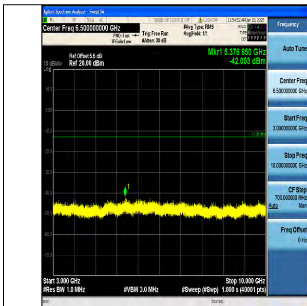
Band13_5MHz_QPSK_23255_1RB#0_3000~10000_3000~10000
