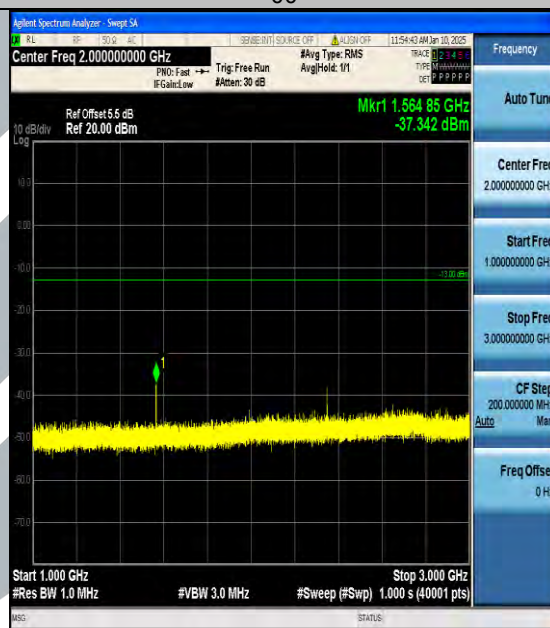
Band13_5MHz_QPSK_23255_1RB#0_1000~3000_1000~3000
