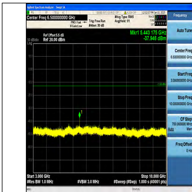
Band13_10MHz_QPSK_23230_1RB#0_3000~10000_3000~10000
