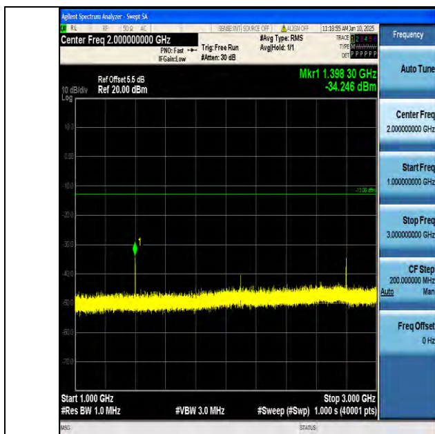
Band12_3MHz_16QAM_23025_1RB#0_1000~3000_1000~3000
