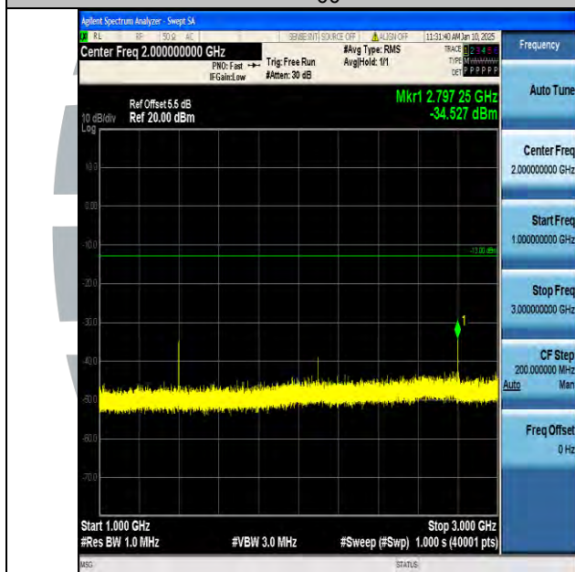
Band12_5MHz_16QAM_23035_1RB#0_1000~3000_1000~3000
