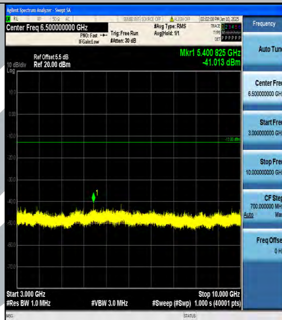
Band17_5MHz_16QAM_23755_1RB#0_3000~10000_3000~10000
