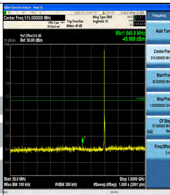
Band12_3MHz_QPSK_23095_1RB#0_30~1000_30~1000
