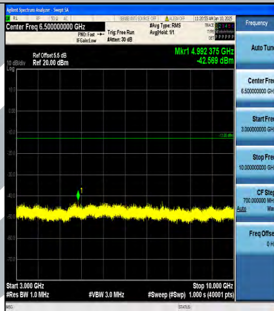
Band12_3MHz_16QAM_23165_1RB#0_3000~10000_3000~10000
