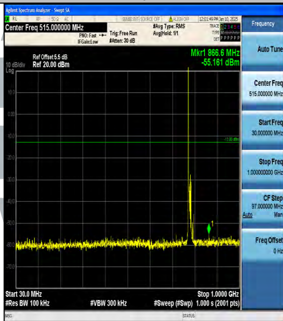
Band13_10MHz_QPSK_23230_1RB#0_30~1000_30~1000
