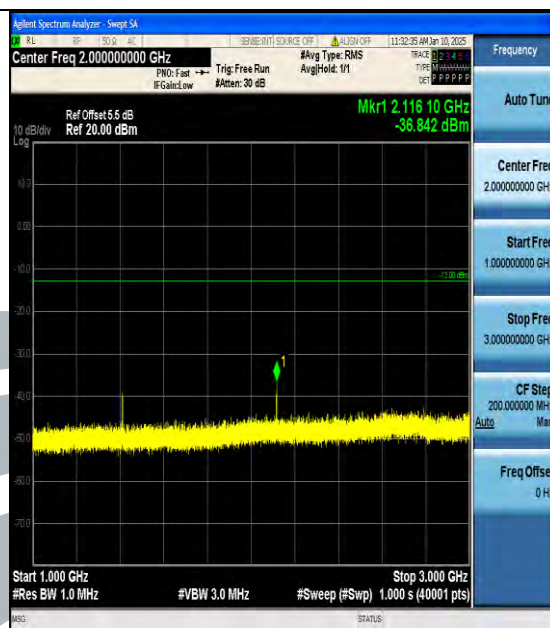
Band12_5MHz_16QAM_23095_1RB#0_1000~3000_1000~3000
