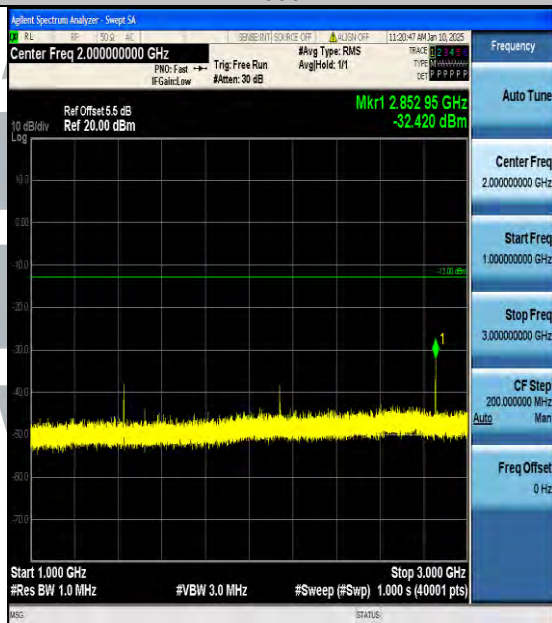
Band12_3MHz_16QAM_23165_1RB#0_1000~3000_1000~3000
