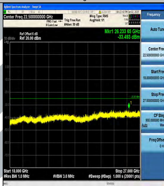
Band7_20MHz_16QAM_21100_1RB#0_18000~27000_18000~27000
