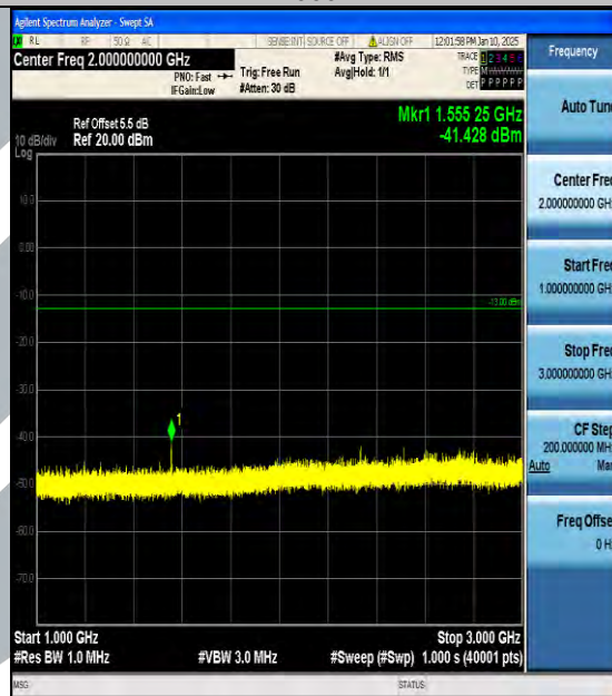
Band13_10MHz_QPSK_23230_1RB#0_1000~3000_1000~3000
