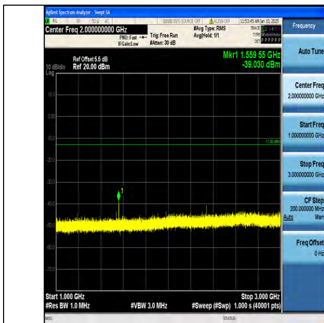
Band13_5MHz_QPSK_23230_1RB#0_1000~3000_1000~3000
