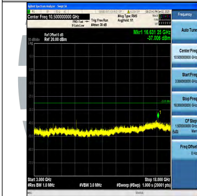
Band7_20MHz_16QAM_21350_1RB#0_3000~18000_3000~18000
