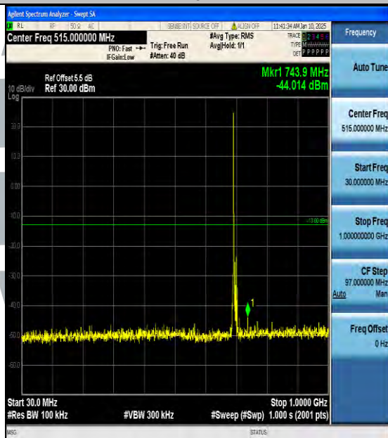
Band12_10MHz_QPSK_23060_1RB#0_30~1000_30~1000
