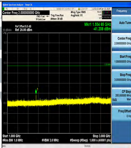
Band13_5MHz_16QAM_23205_1RB#0_1000~3000_1000~3000
