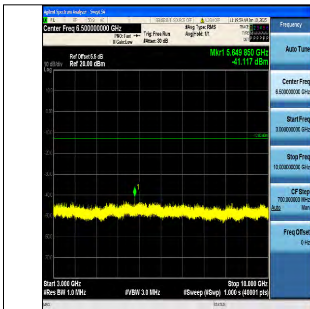
Band12_3MHz_16QAM_23095_1RB#0_3000~10000_3000~10000
