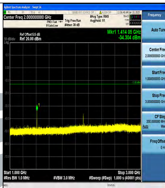
Band12_1.4MHz_16QAM_23095_1RB#0_1000~3000_1000~3000
