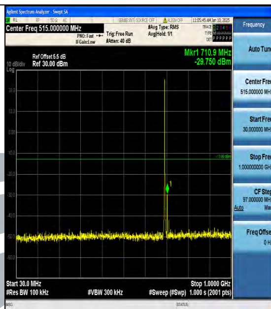
Band12_1.4MHz_16QAM_23017_1RB#0_30~1000_30~1000
