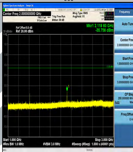
Band12_3MHz_16QAM_23095_1RB#0_1000~3000_1000~3000
