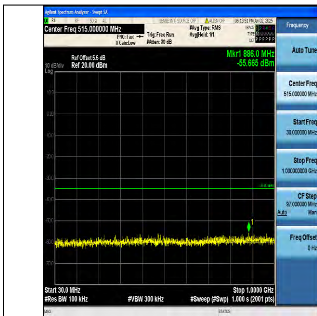
Band7_15MHz_16QAM_21375_1RB#0_30~1000_30~1000
