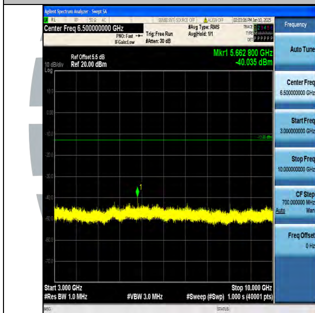
Band17_5MHz_16QAM_23790_1RB#0_3000~10000_3000~10000
