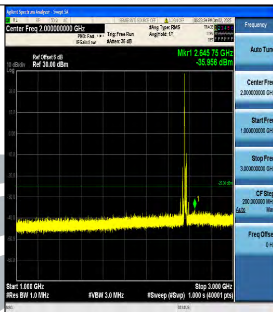
Band7_20MHz_16QAM_21350_1RB#0_1000~3000_1000~3000
