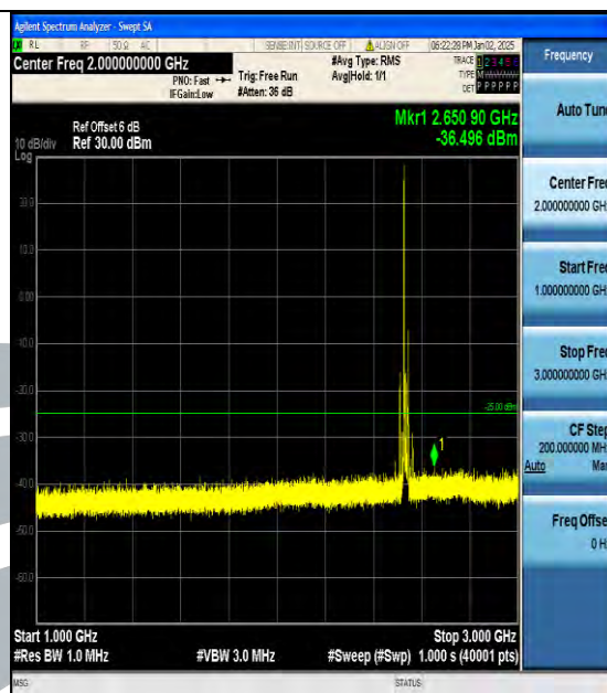
Band7_20MHz_16QAM_21100_1RB#0_1000~3000_1000~3000
