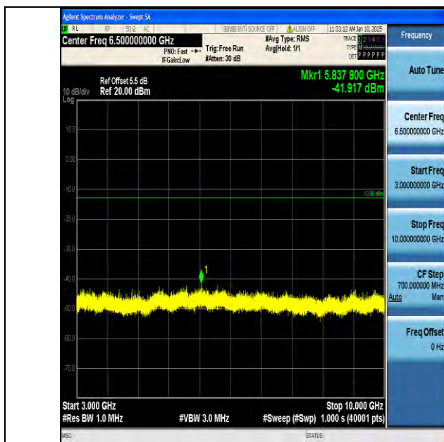
Band12_5MHz_QPSK_23155_1RB#0_3000~10000_3000~10000
