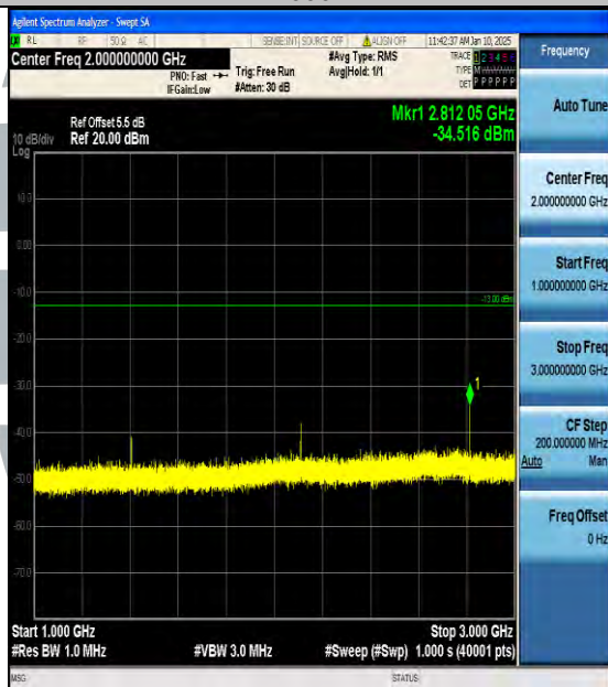
Band12_10MHz_QPSK_23095_1RB#0_1000~3000_1000~3000
