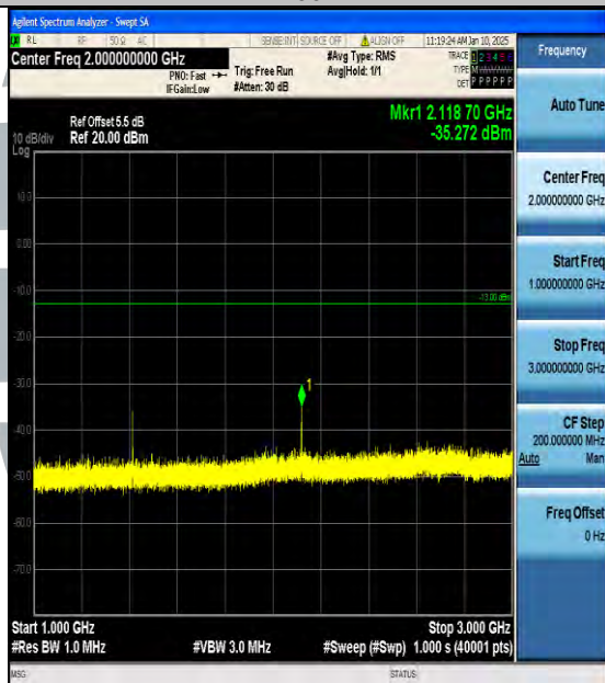
Band12_3MHz_QPSK_23095_1RB#0_1000~3000_1000~3000
