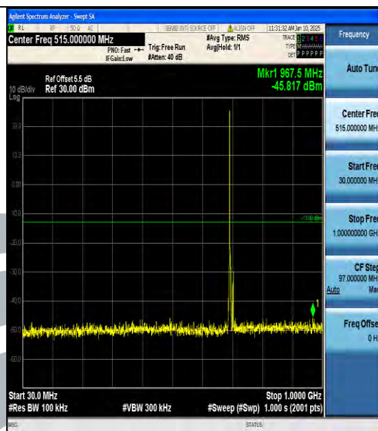
Band12_5MHz_16QAM_23035_1RB#0_30~1000_30~1000
