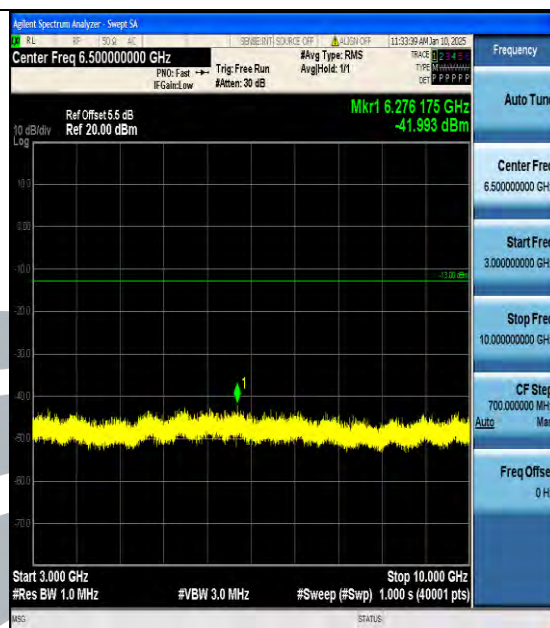
Band12_5MHz_16QAM_23155_1RB#0_3000~10000_3000~10000
