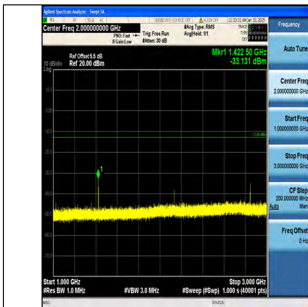
Band12_5MHz_16QAM_23155_1RB#0_1000~3000_1000~3000
