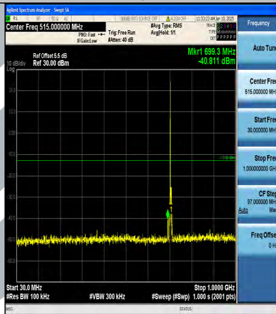
Band12_5MHz_16QAM_23155_1RB#0_30~1000_30~1000
