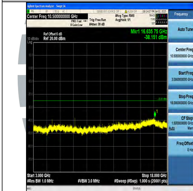
Band7_15MHz_16QAM_21375_1RB#0_3000~18000_3000~18000
