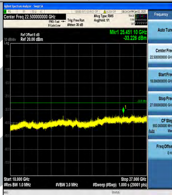
Band7_15MHz_16QAM_21375_1RB#0_18000~27000_18000~27000
