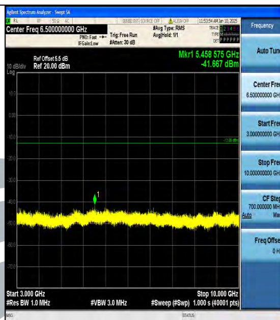
Band13_5MHz_QPSK_23230_1RB#0_3000~10000_3000~10000
