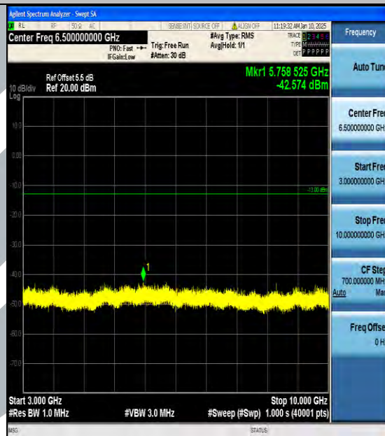
Band12_3MHz_QPSK_23095_1RB#0_3000~10000_3000~10000
