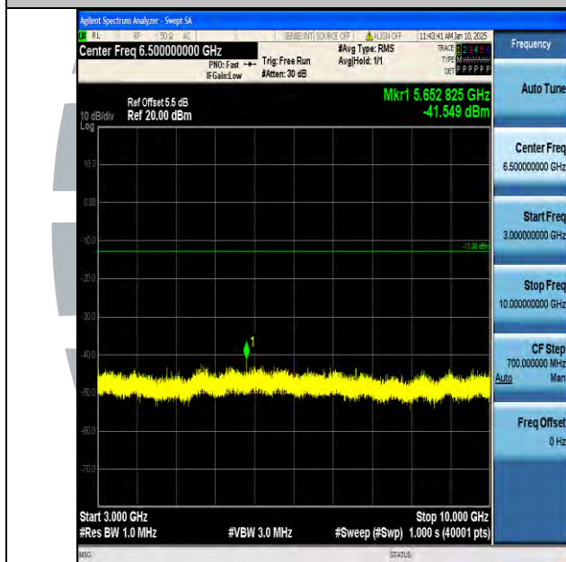
Band12_10MHz_QPSK_23130_1RB#0_3000~10000_3000~10000
