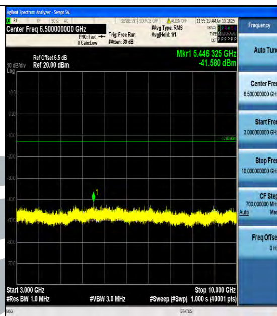
Band13_5MHz_16QAM_23255_1RB#0_3000~10000_3000~10000
