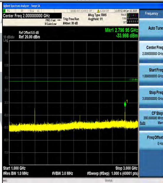
Band12_1.4MHz_16QAM_23017_1RB#0_1000~3000_1000~3000
