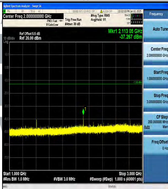
Band17_5MHz_16QAM_23755_1RB#0_1000~3000_1000~3000
