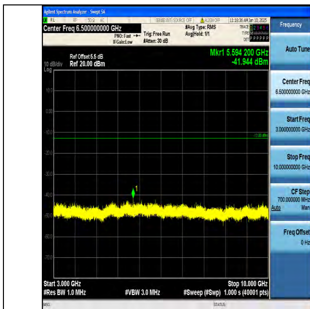
Band12_3MHz_QPSK_23025_1RB#0_3000~10000_3000~10000
