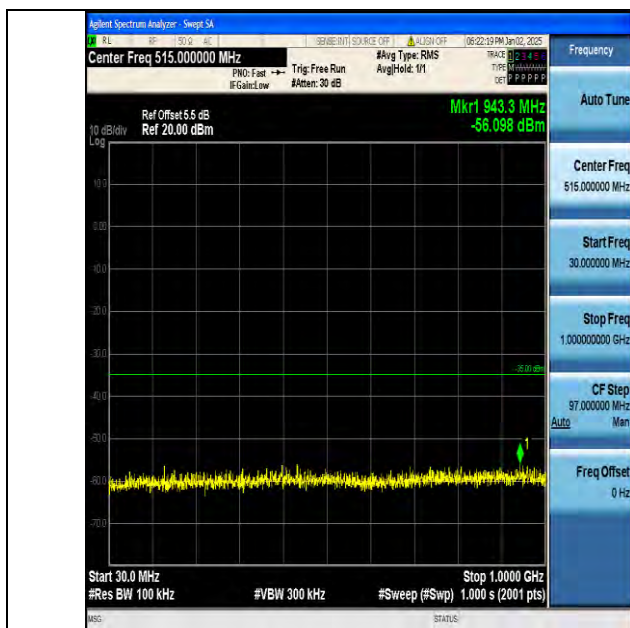
Band7_20MHz_16QAM_21100_1RB#0_30~1000_30~1000
