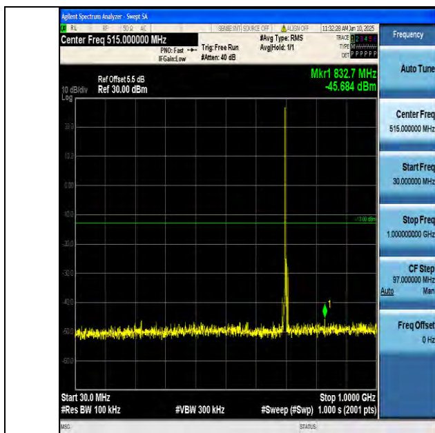
Band12_5MHz_16QAM_23095_1RB#0_30~1000_30~1000
