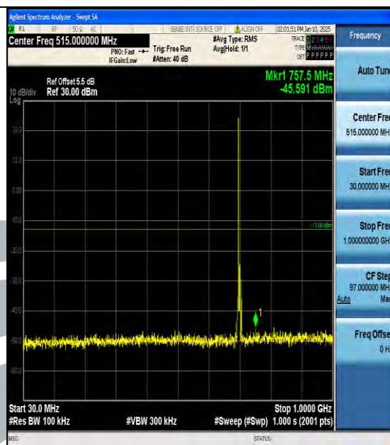
Band17_5MHz_16QAM_23755_1RB#0_30~1000_30~1000
