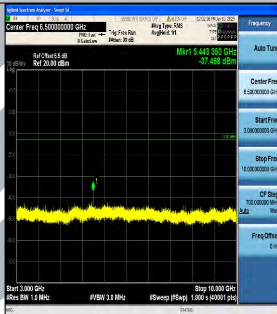
Band13_10MHz_16QAM_23230_1RB#0_3000~10000_3000~10000
