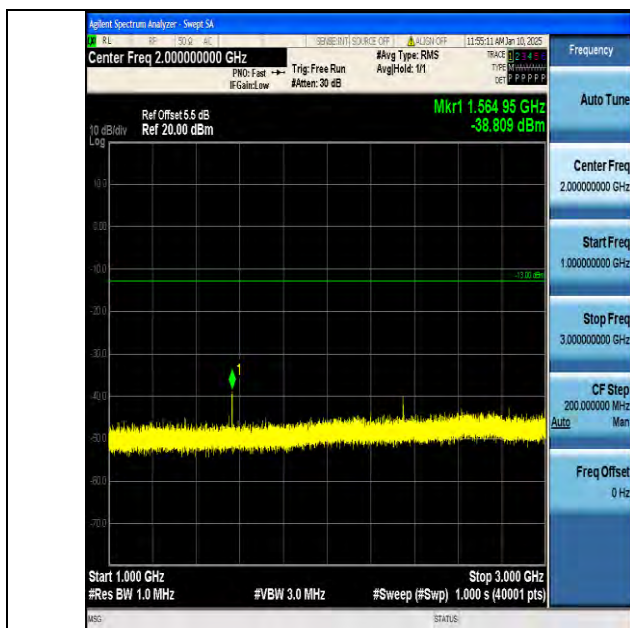
Band13_5MHz_16QAM_23255_1RB#0_1000~3000_1000~3000
