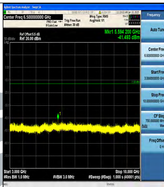
Band12_3MHz_16QAM_23025_1RB#0_3000~10000_3000~10000
