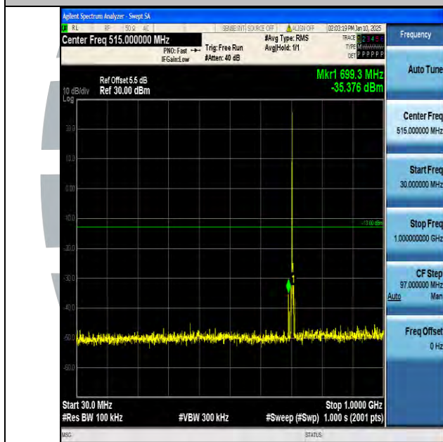
Band17_5MHz_QPSK_23825_1RB#0_30~1000_30~1000
