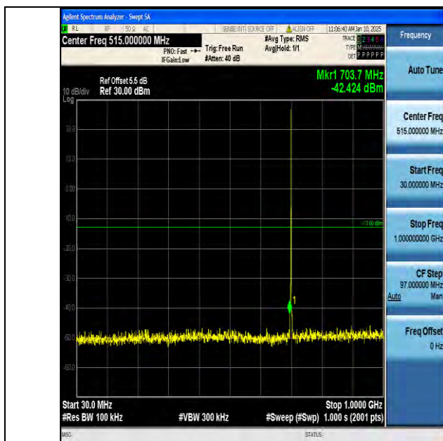
Band12_1.4MHz_16QAM_23095_1RB#0_30~1000_30~1000
