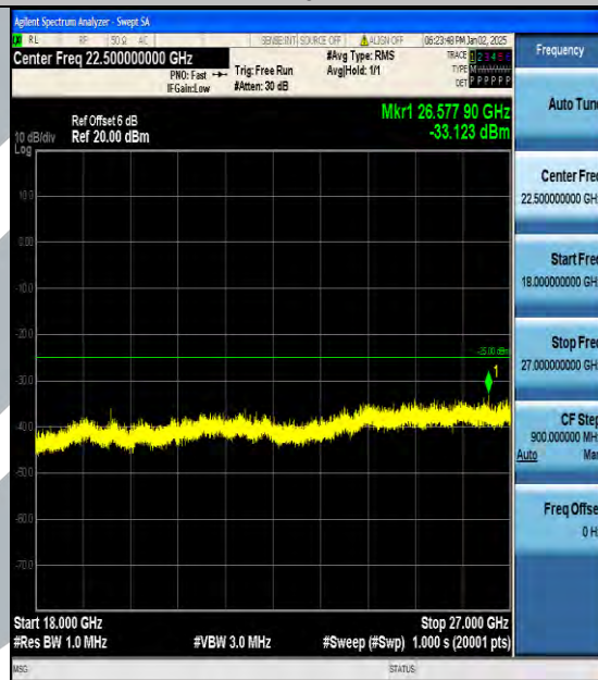
Band7_20MHz_16QAM_21350_1RB#0_18000~27000_18000~27000
