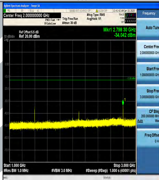
Band12_10MHz_QPSK_23060_1RB#0_1000~3000_1000~3000
