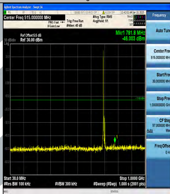
Band12_10MHz_16QAM_23060_1RB#0_30~1000_30~1000
