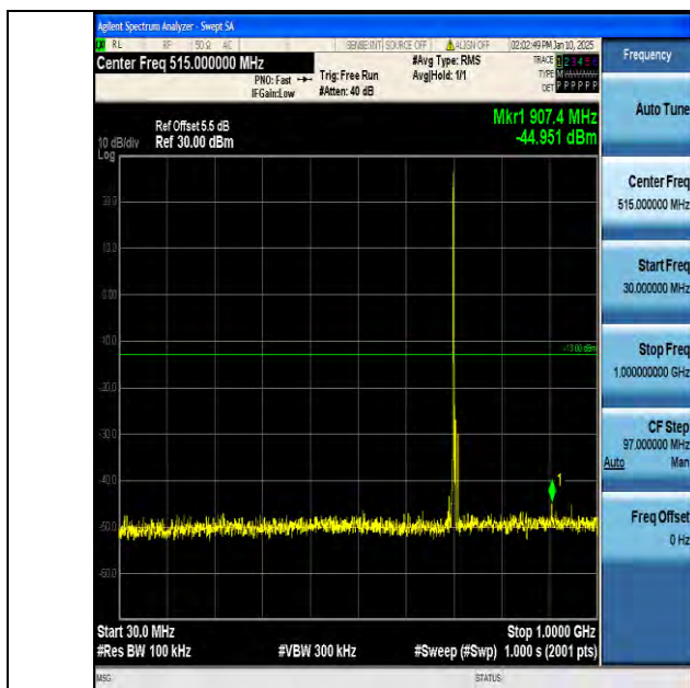
Band17_5MHz_16QAM_23790_1RB#0_30~1000_30~1000
