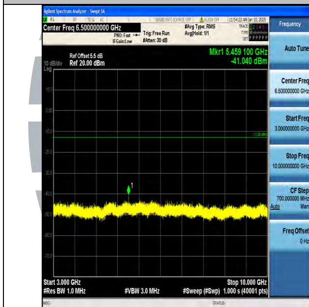
Band13_5MHz_16QAM_23230_1RB#0_3000~10000_3000~10000
