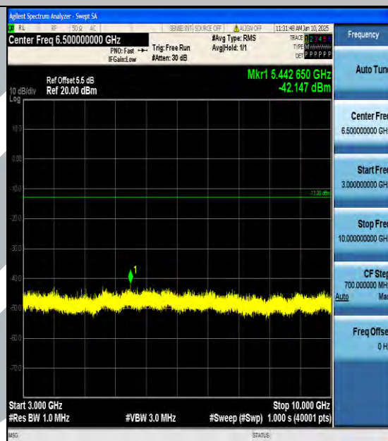
Band12_5MHz_16QAM_23035_1RB#0_3000~10000_3000~10000
