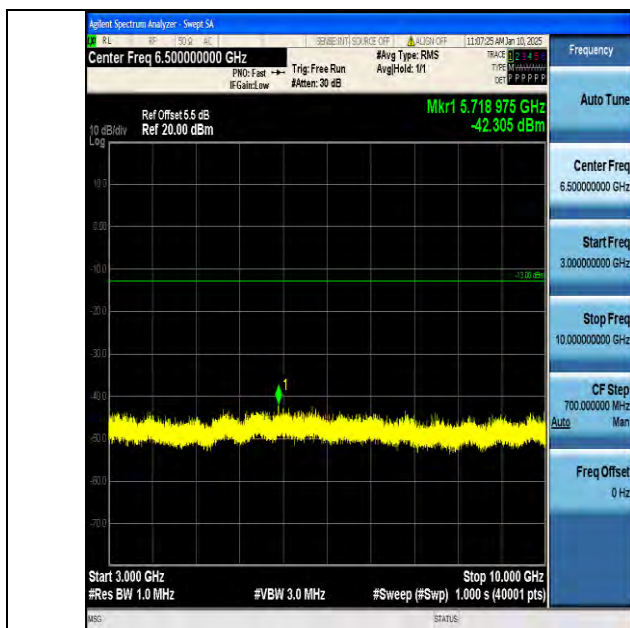
Band12_1.4MHz_QPSK_23173_1RB#0_3000~10000_3000~10000
