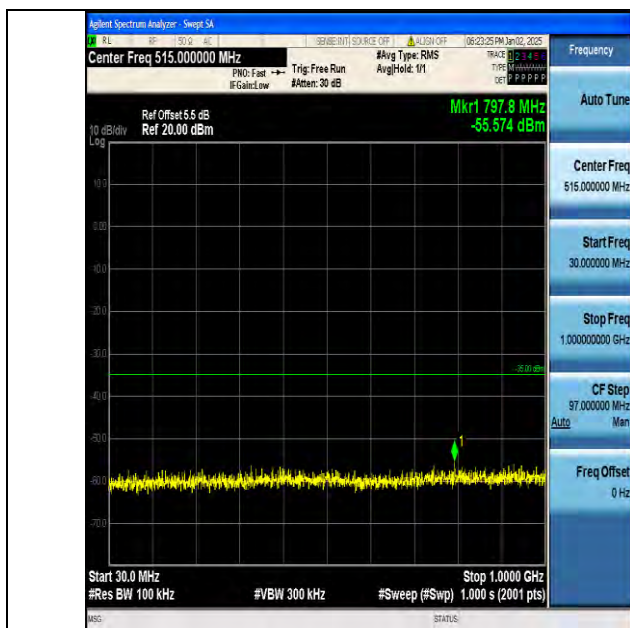
Band7_20MHz_16QAM_21350_1RB#0_30~1000_30~1000
