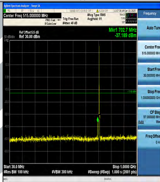
Band12_1.4MHz_16QAM_23173_1RB#0_30~1000_30~1000
