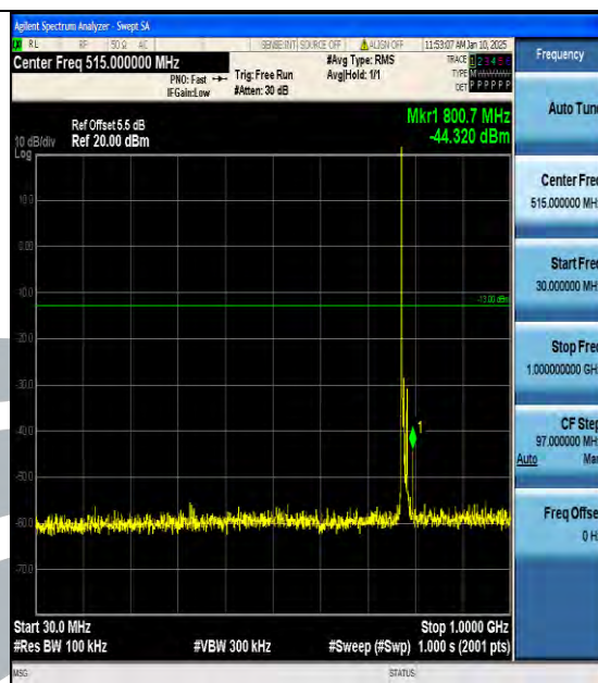
Band13_5MHz_16QAM_23205_1RB#0_30~1000_30~1000
