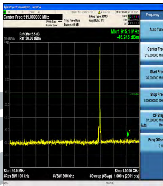
Band12_10MHz_QPSK_23095_1RB#0_30~1000_30~1000
