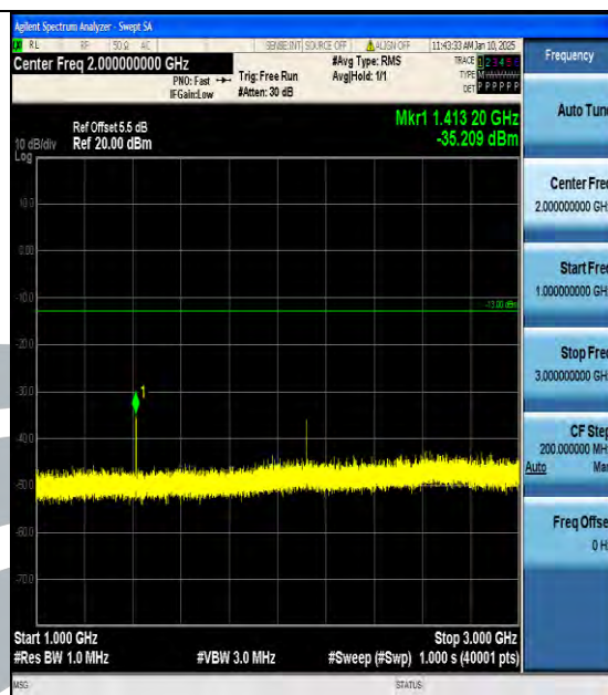
Band12_10MHz_QPSK_23130_1RB#0_1000~3000_1000~3000
