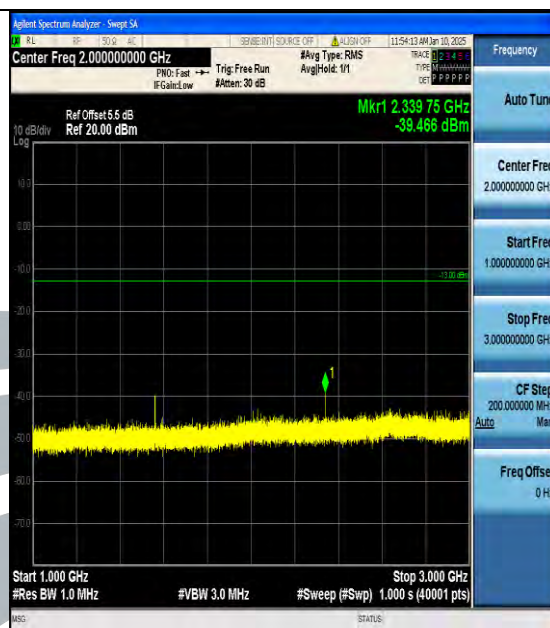
Band13_5MHz_16QAM_23230_1RB#0_1000~3000_1000~3000
