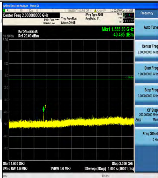
Band13_10MHz_16QAM_23230_1RB#0_1000~3000_1000~3000
