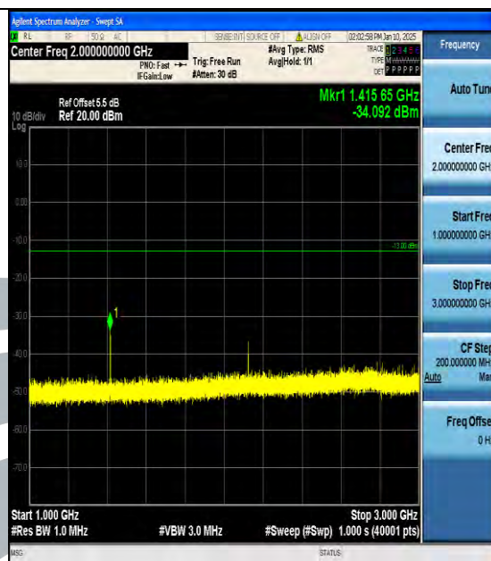
Band17_5MHz_16QAM_23790_1RB#0_1000~3000_1000~3000
