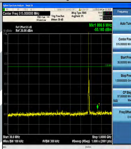
Band13_5MHz_16QAM_23255_1RB#0_30~1000_30~1000
