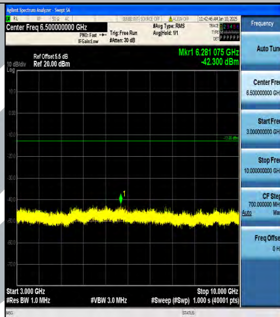
Band12_10MHz_QPSK_23095_1RB#0_3000~10000_3000~10000
