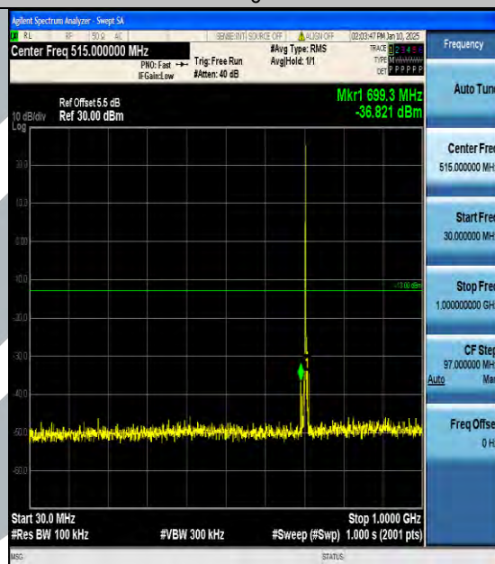
Band17_5MHz_16QAM_23825_1RB#0_30~1000_30~1000
