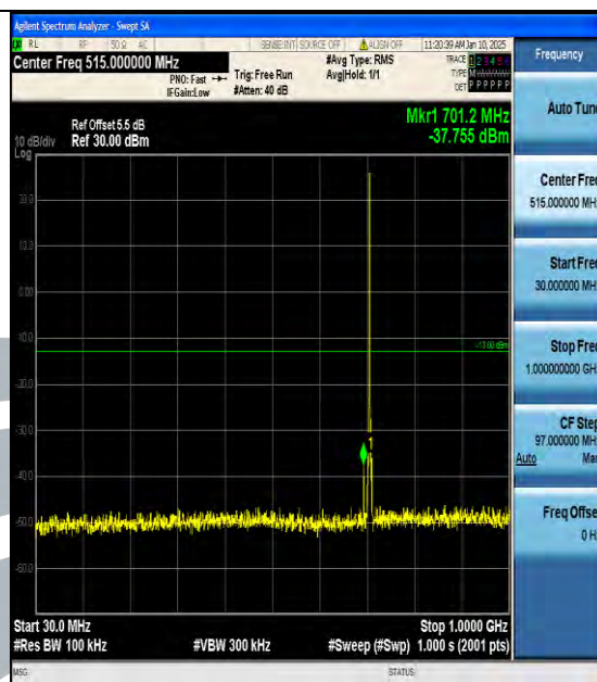
Band12_3MHz_16QAM_23165_1RB#0_30~1000_30~1000
