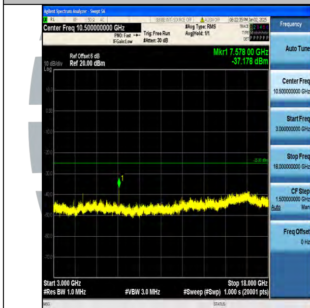
Band7_20MHz_16QAM_21100_1RB#0_3000~18000_3000~18000
