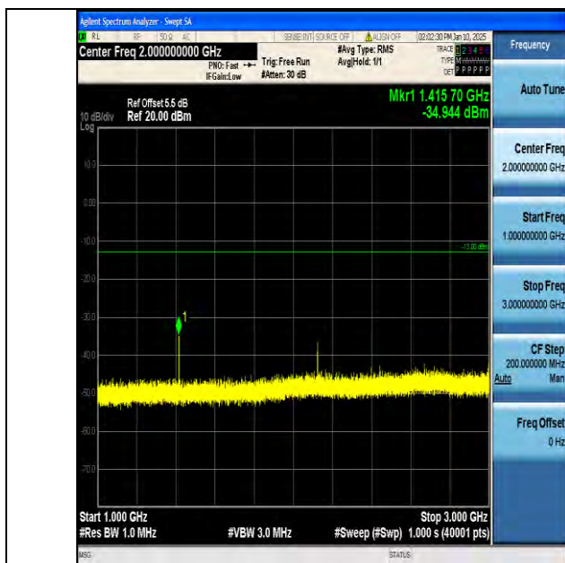
Band17_5MHz_QPSK_23790_1RB#0_1000~3000_1000~3000
