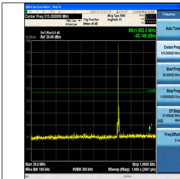
Band12_10MHz_QPSK_23130_1RB#0_30~1000_30~1000
