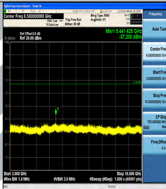
Band13_5MHz_16QAM_23205_1RB#0_3000~10000_3000~10000
