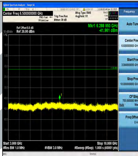
Band12_1.4MHz_16QAM_23017_1RB#0_3000~10000_3000~10000
