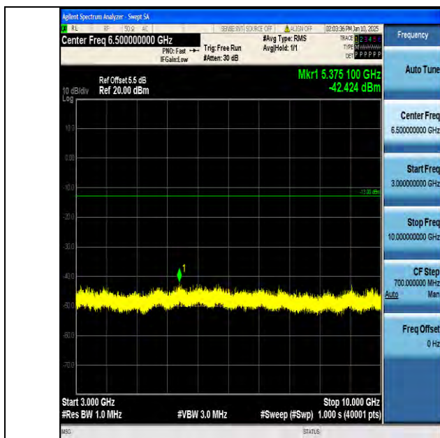
Band17_5MHz_QPSK_23825_1RB#0_3000~10000_3000~10000
