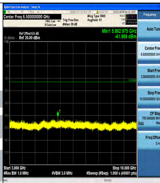
Band17_5MHz_QPSK_23790_1RB#0_3000~10000_3000~10000
