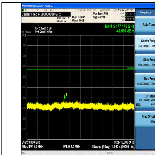
Band12_10MHz_QPSK_23060_1RB#0_3000~10000_3000~10000
