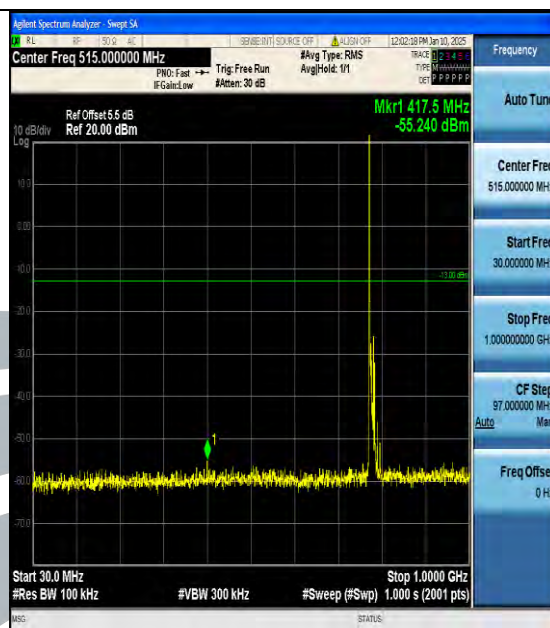
Band13_10MHz_16QAM_23230_1RB#0_30~1000_30~1000
