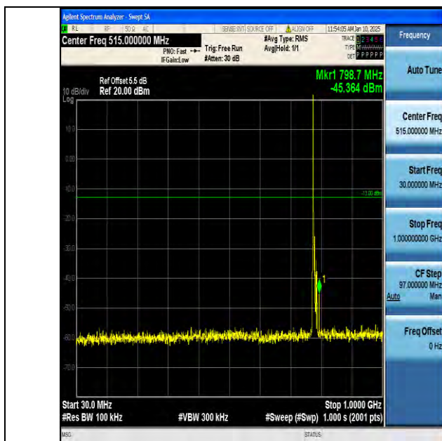
Band13_5MHz_16QAM_23230_1RB#0_30~1000_30~1000
