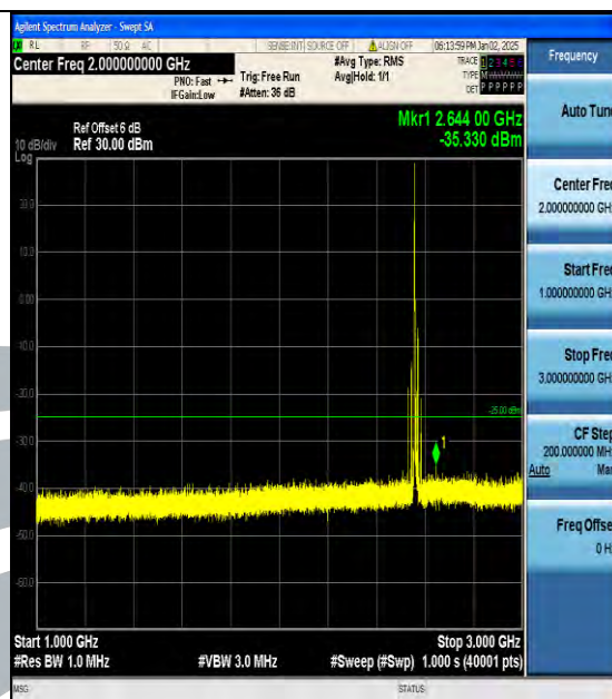
Band7_15MHz_16QAM_21375_1RB#0_1000~3000_1000~3000
