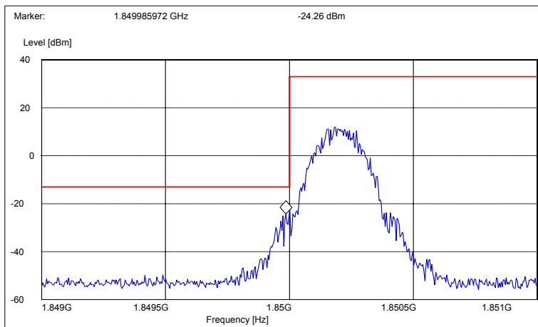
Picture 3 Lower bandedge, channel 512
