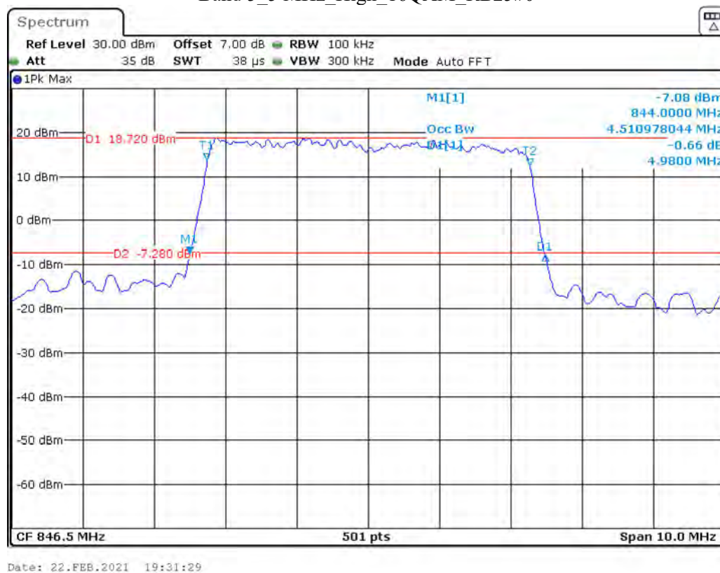
Band 5 5 MHz High 16QAM RB25#0
