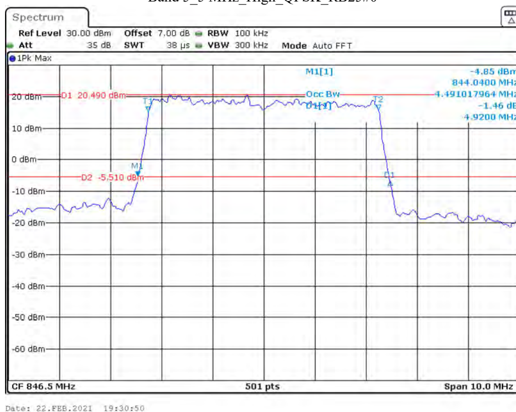
Band 5 5 MHz High QPSK RB25#0
