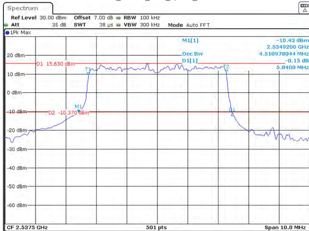
Band 41_5 MHz_Low_QPSK_RB25#0
