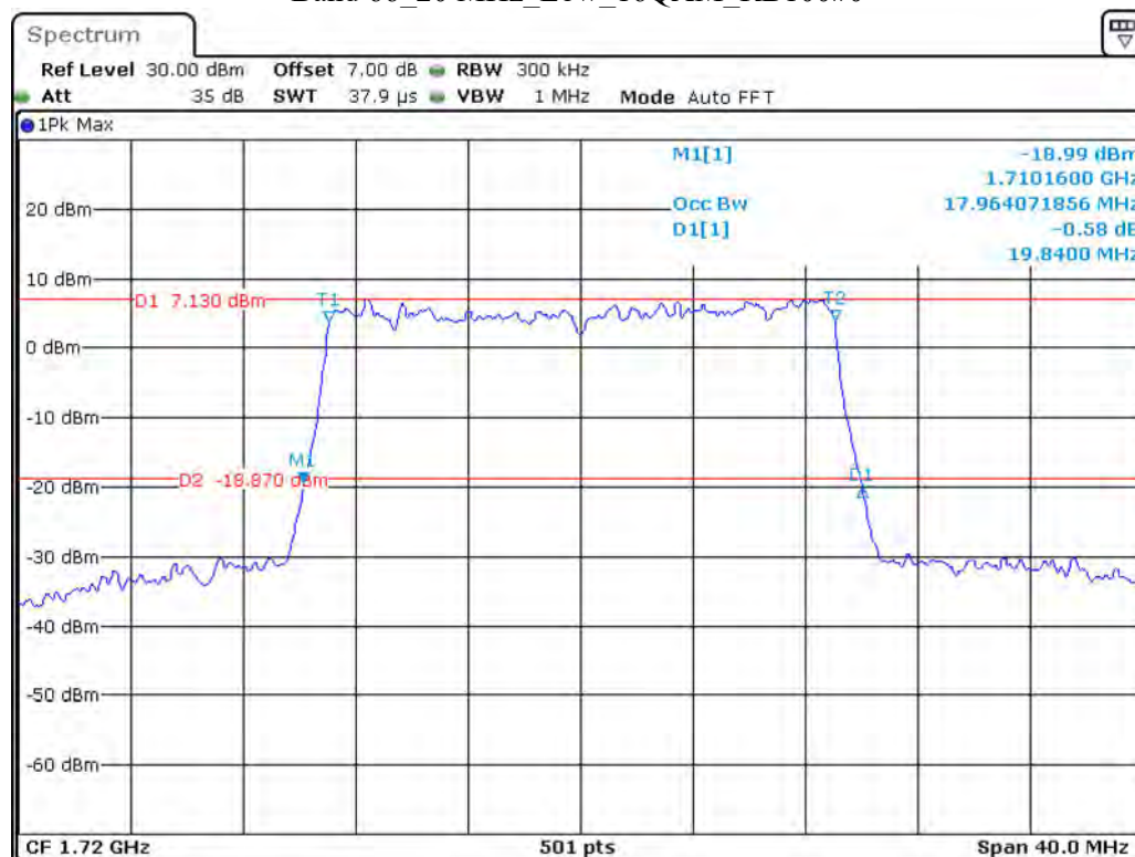
Band 66 20 MHz Low 16QAM RB100#0
