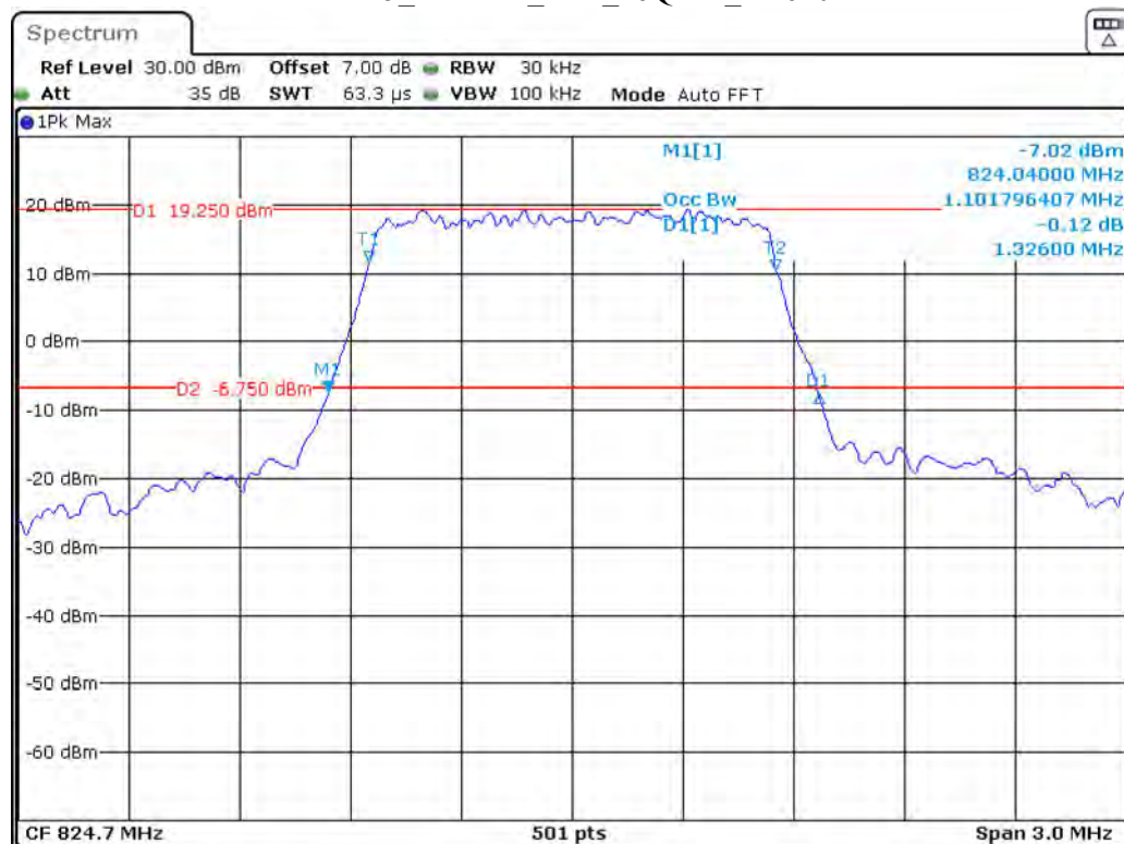
Band 5_1.4 MHz_Low_16QAM_RB6#0
