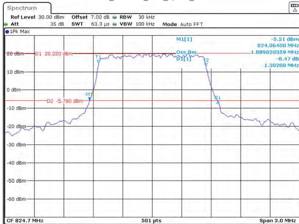
Band 5_1.4 MHz_Low_QPSK_RB6#0
