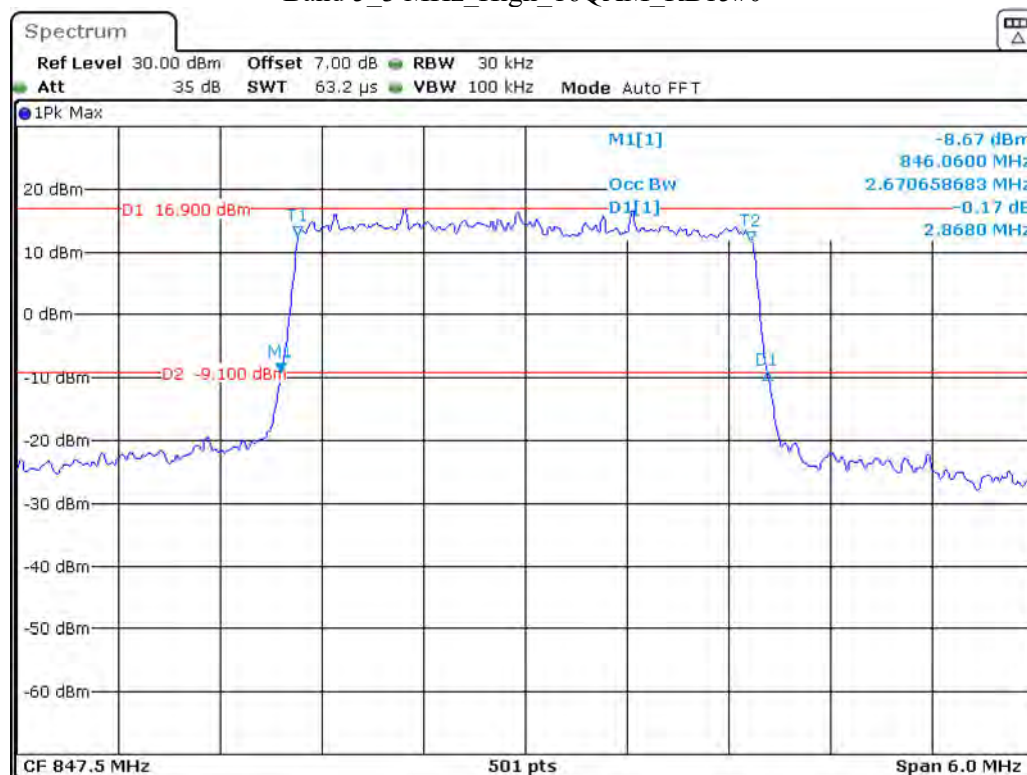
Band 5 3 MHz High 16QAM RB15#0
