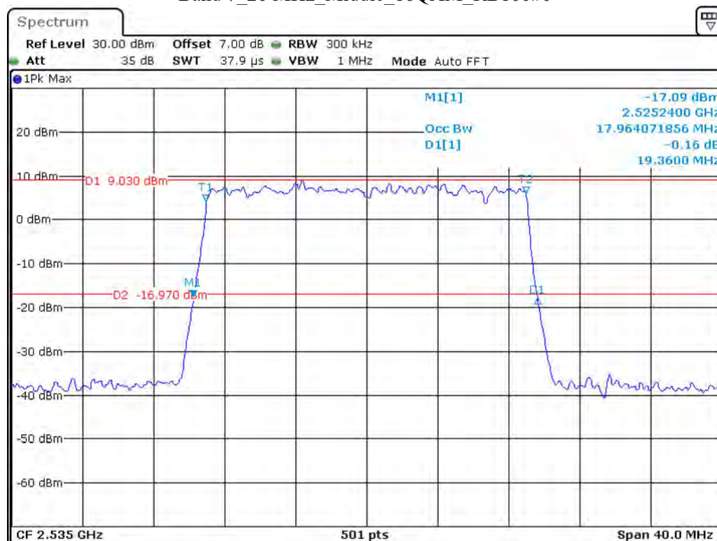
Band 7 20 MHz Middle 16QAM RB100#0
