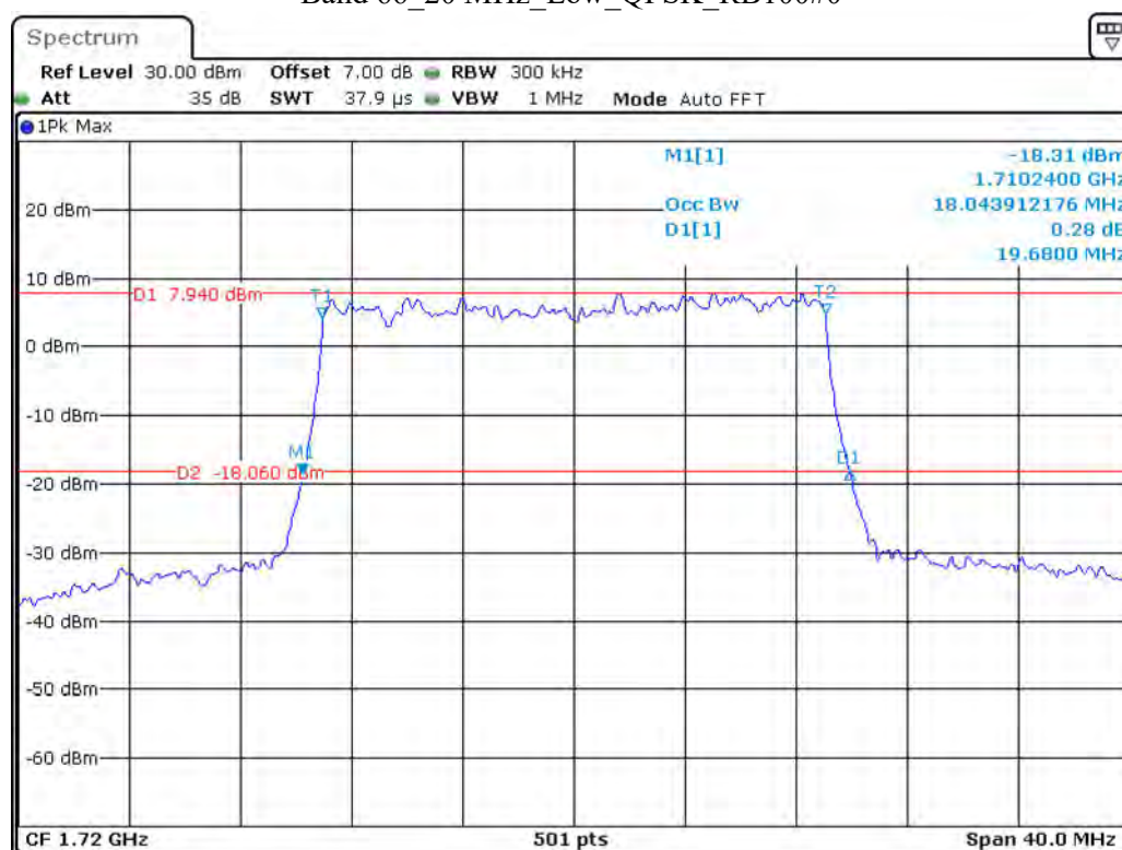
Band 66 20 MHz Low QPSK RB100#0
