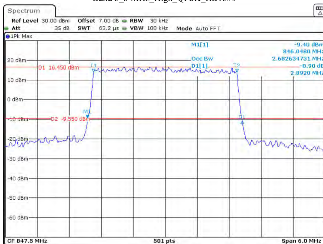
Band 5 3 MHz High QPSK RB15#0
