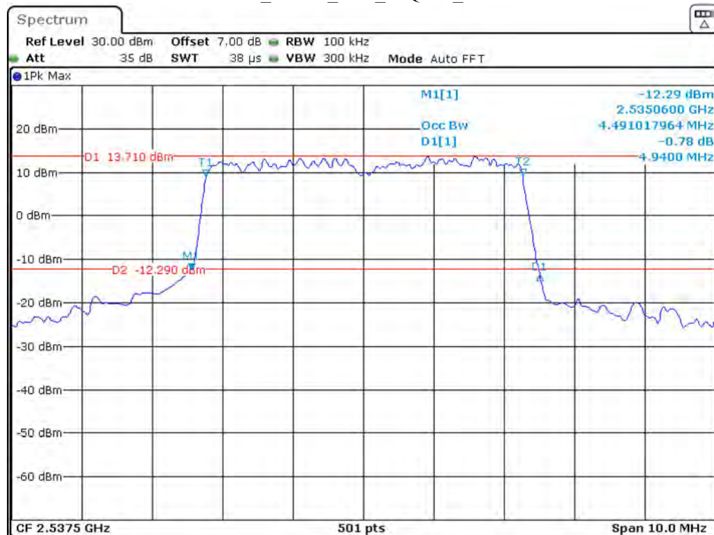
Band 41_5 MHz_Low_16QAM_RB25#0
