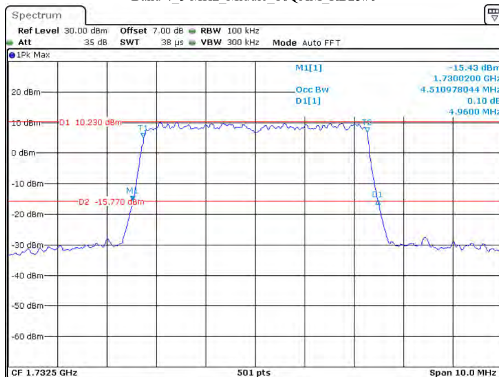
Band 4 5 MHz Middle 16QAM RB25#0
