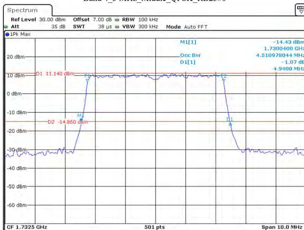
Band 4 5 MHz Middle QPSK RB25#0
