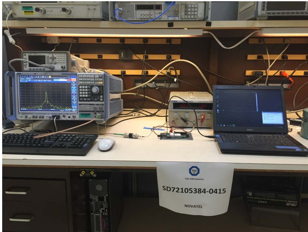
Conducted Testing
