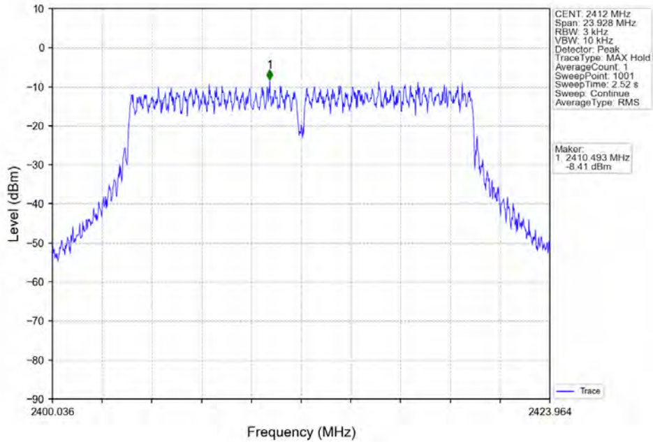
802.11g LCH 2412MHz MIMO NTN
