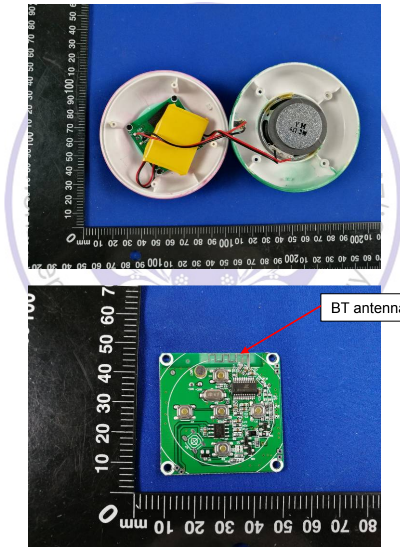
Internal Photos of EUT
