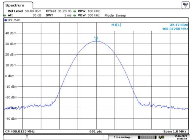
Low Channel, 4FSK, 400.0125 MHz
