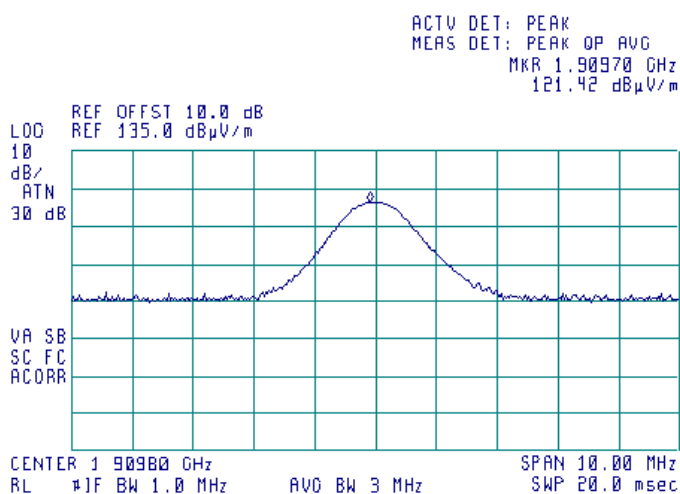
Plot 8.1.12 Transmitter carrier field strength at high frequency in horizontal antenna polarization, EUT horizontal position
