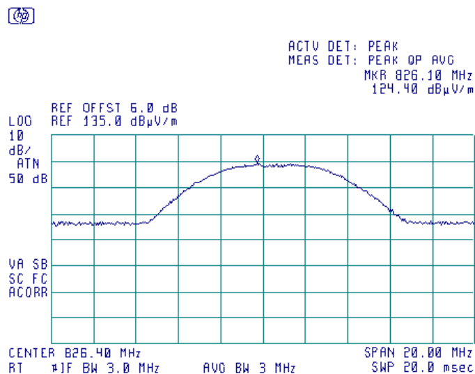
Plot 7.1.16 Transmitter carrier field strength at low frequency in horizontal antenna polarization, EUT horizontal position
