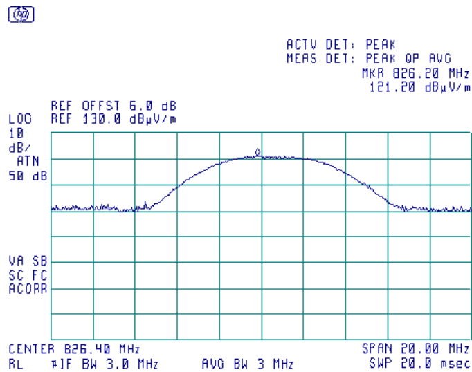
Plot 7.1.15 Transmitter carrier field strength at low frequency in vertical antenna polarization, EUT horizontal position
