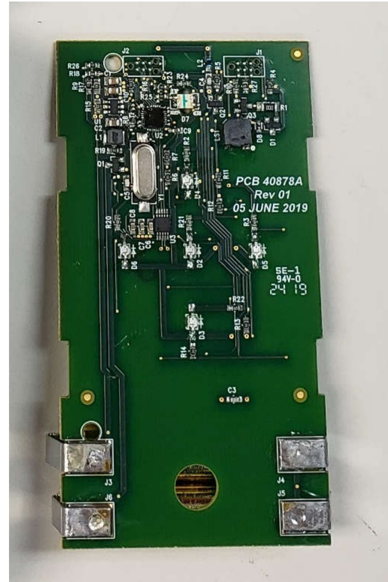
PCB Bottom View
