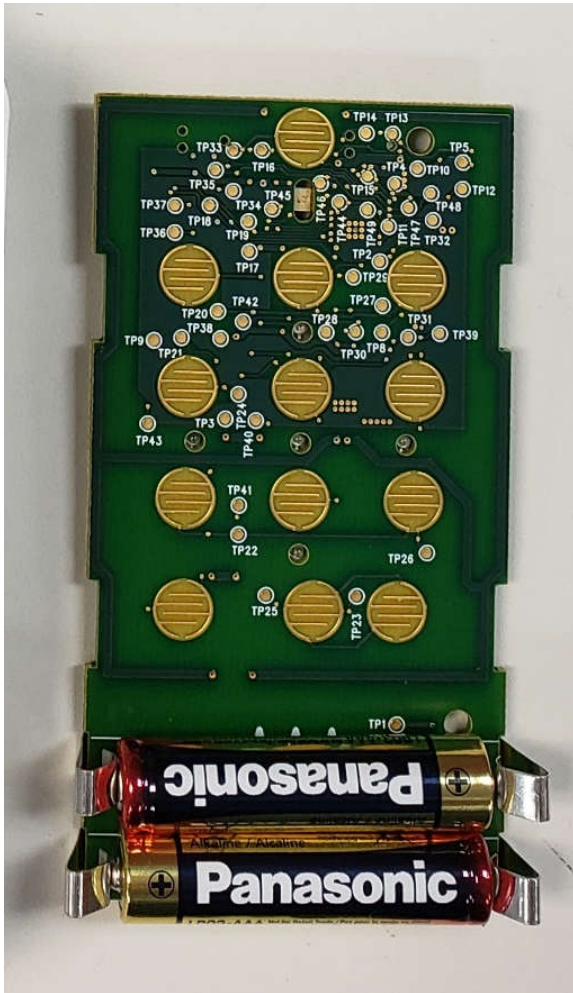
Internal View
