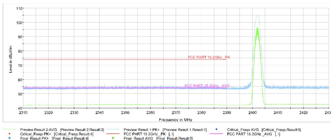
Fig.13. Frequency Band Edges: GFSK, Channel 0, 2.31 GHz – 2.45GHz
