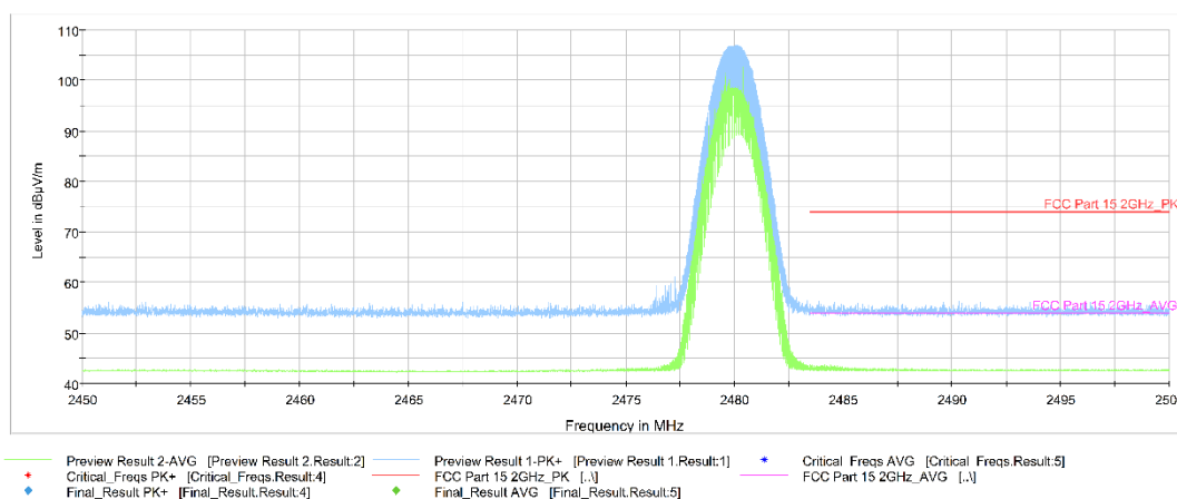
Fig.14. Frequency Band Edges: GFSK, Channel 78, ch11, 2.45 GHz - 2.50GHz
