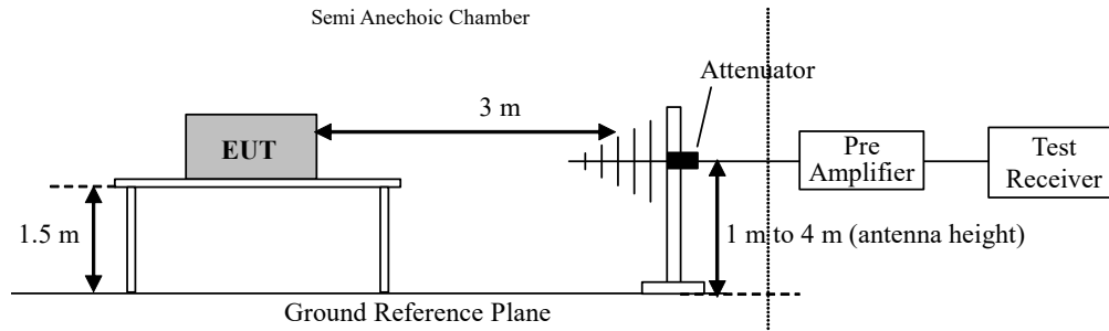
Figure 1: Test Setup
