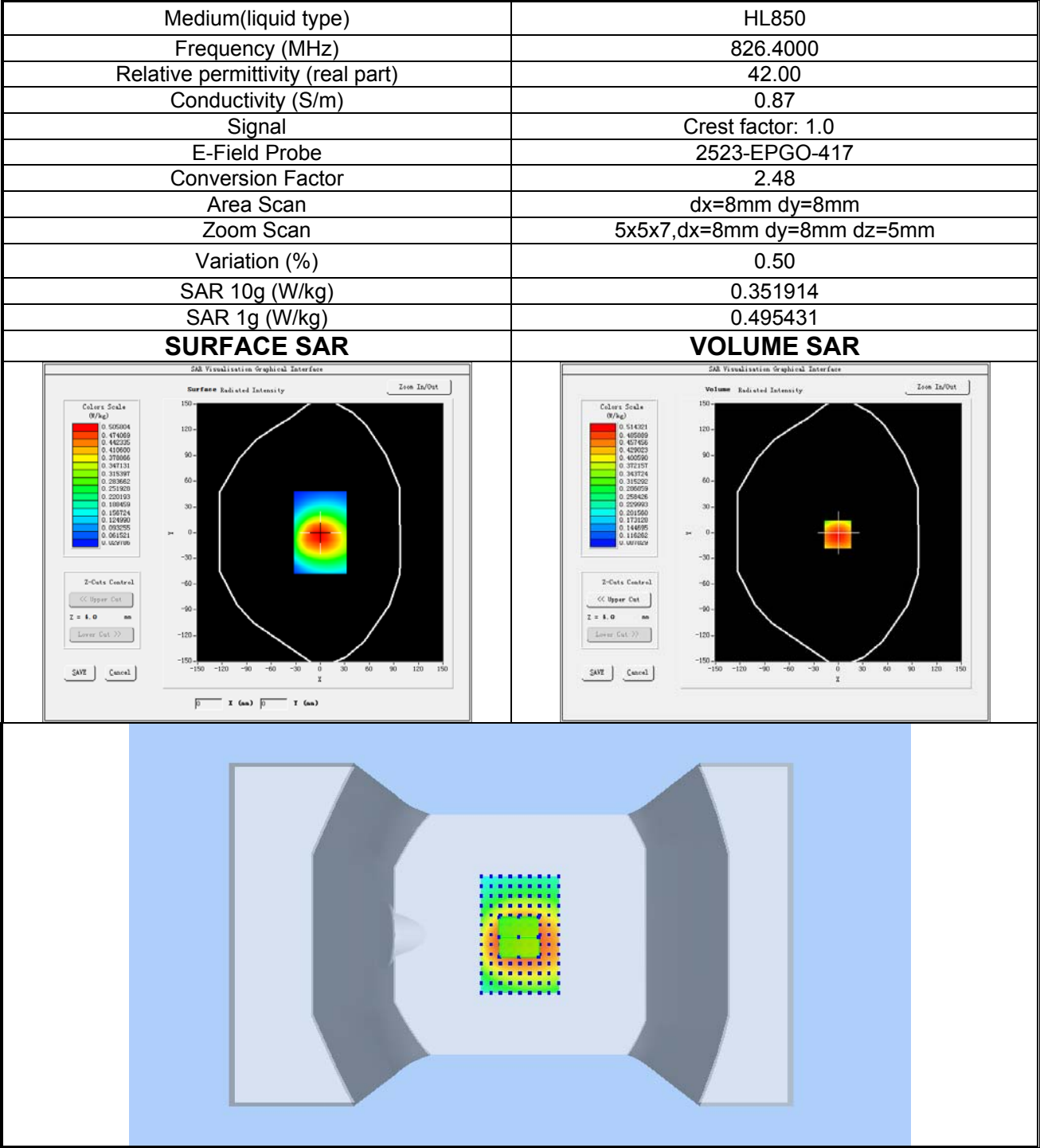
Plot 4: WCDMA BAND V, Low channel (Body-worn, Front Side) Product Description: LTE MiFi Router Test Date: 2024-02-28
