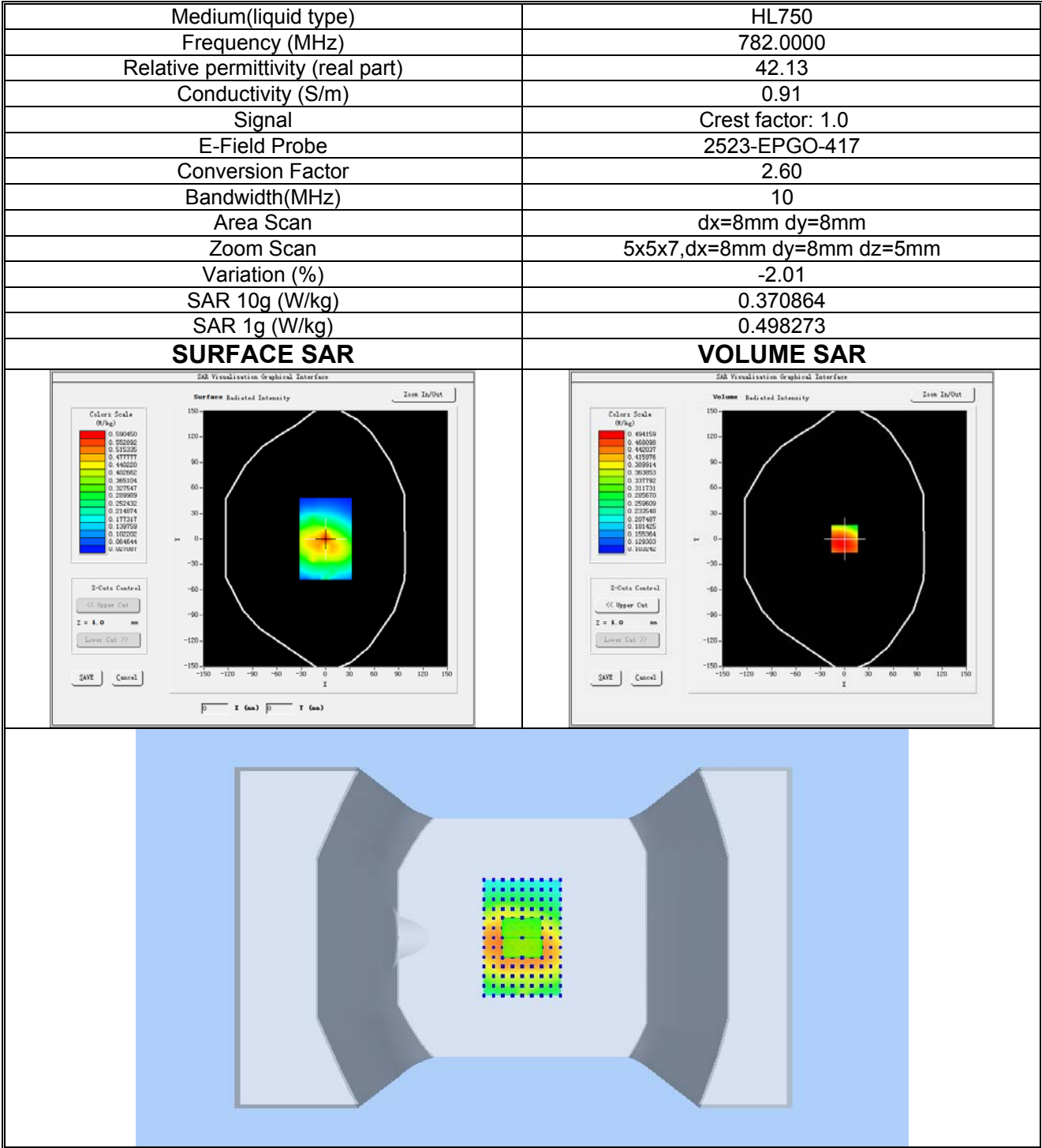
Plot 9: LTE BAND 13, Low channel (Body-worn, Front Side) Product Description: LTE MiFi Router Test Date: 2024-02-27
