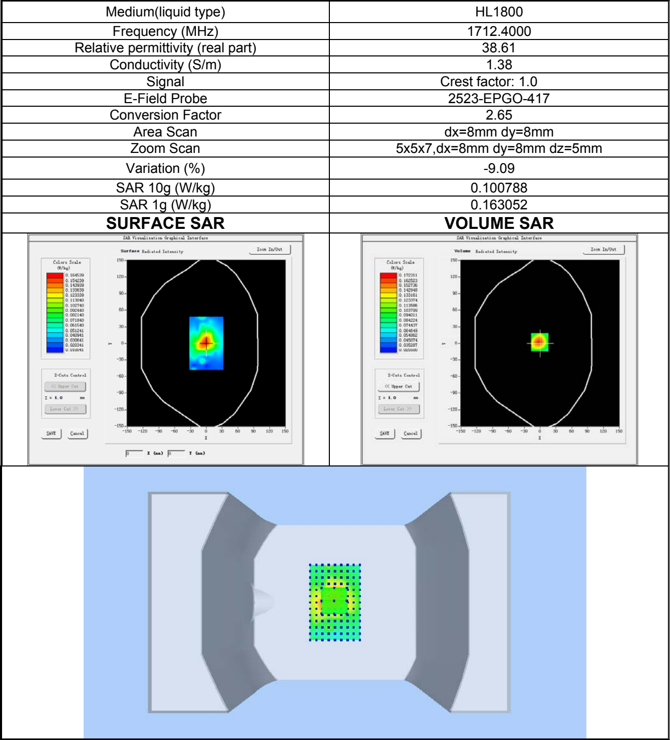
Plot 3: WCDMA BAND IV, Low channel (Body-worn, Top Edge) Product Description: LTE MiFi Router Test Date: 2024-02-26
