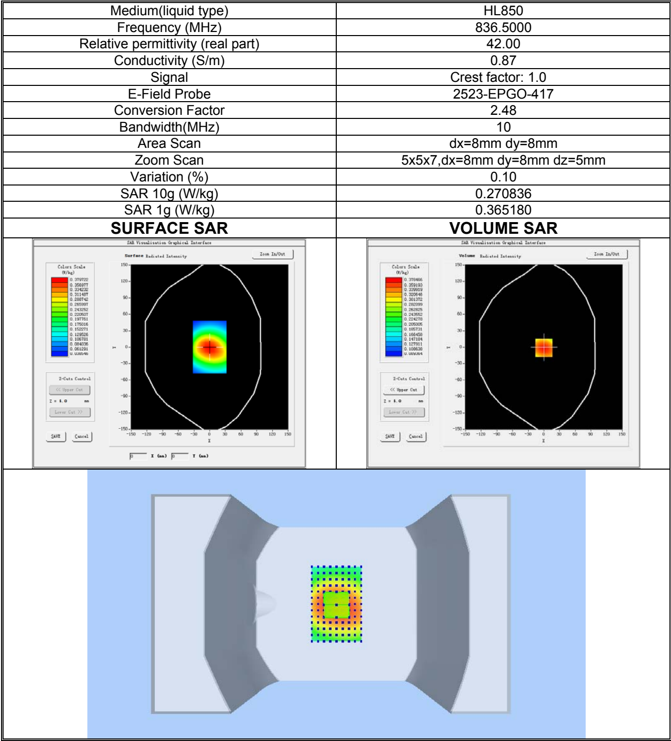
Plot 7: LTE BAND 5, Middle channel (Body-worn, Front Side) Product Description: LTE MiFi Router Test Date: 2024-02-28
