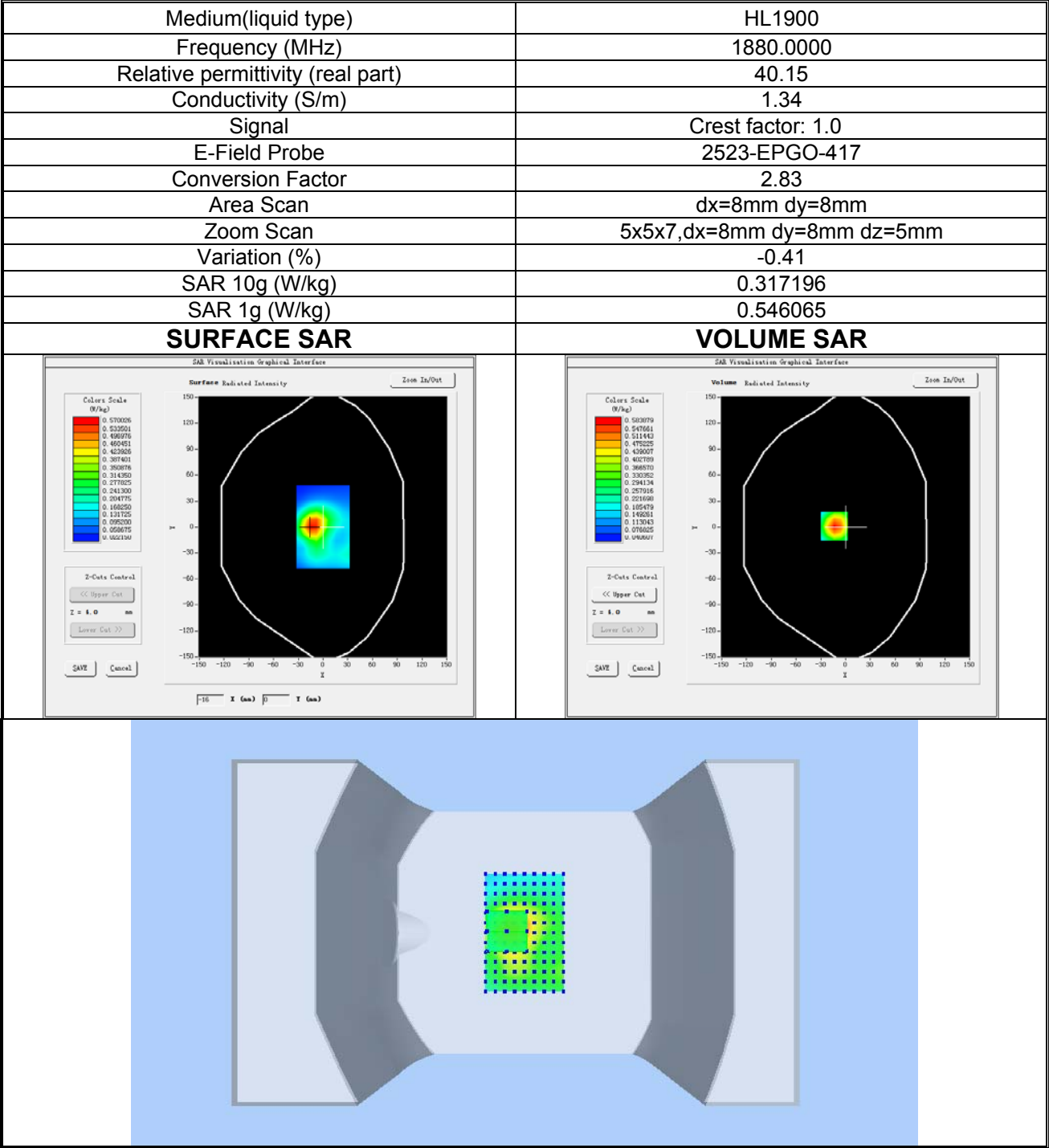
Plot 2: WCDMA BAND II, Middle channel (Body-worn, Front Side) Product Description: LTE MiFi Router Test Date: 2024-02-27
