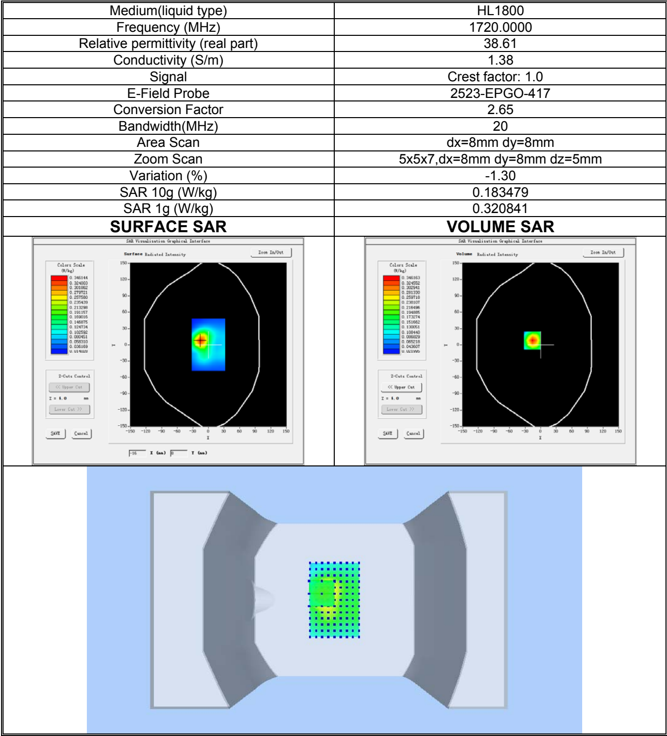
Plot 10: LTE BAND 66, Low channel (Body-worn, Front Side) Product Description: LTE MiFi Router Test Date: 2024-02-26
