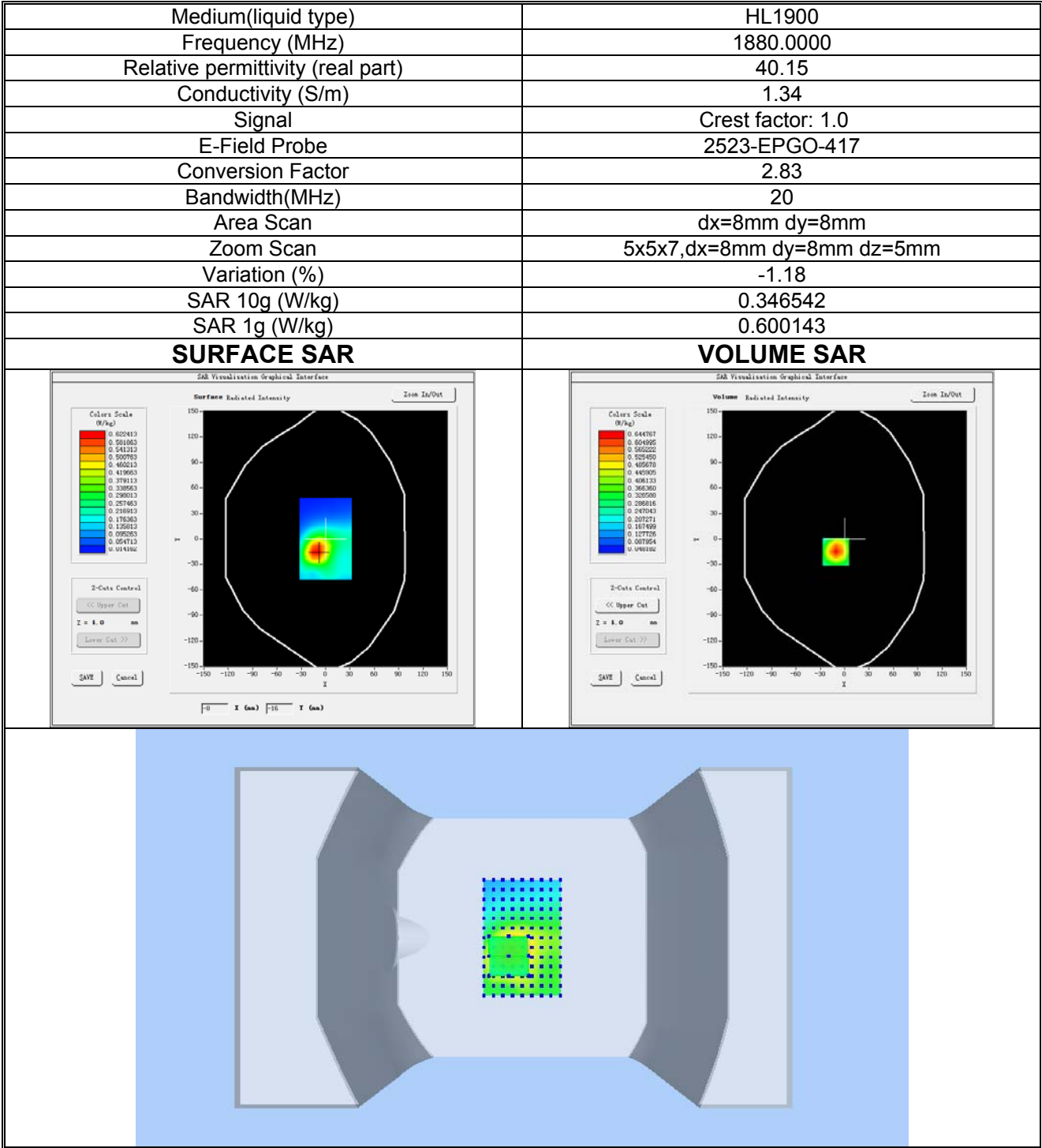
Plot 5: LTE BAND 2, Middle channel (Body-worn, Front Side) Product Description:LTE MiFi Router Test Date: 2024-02-27
