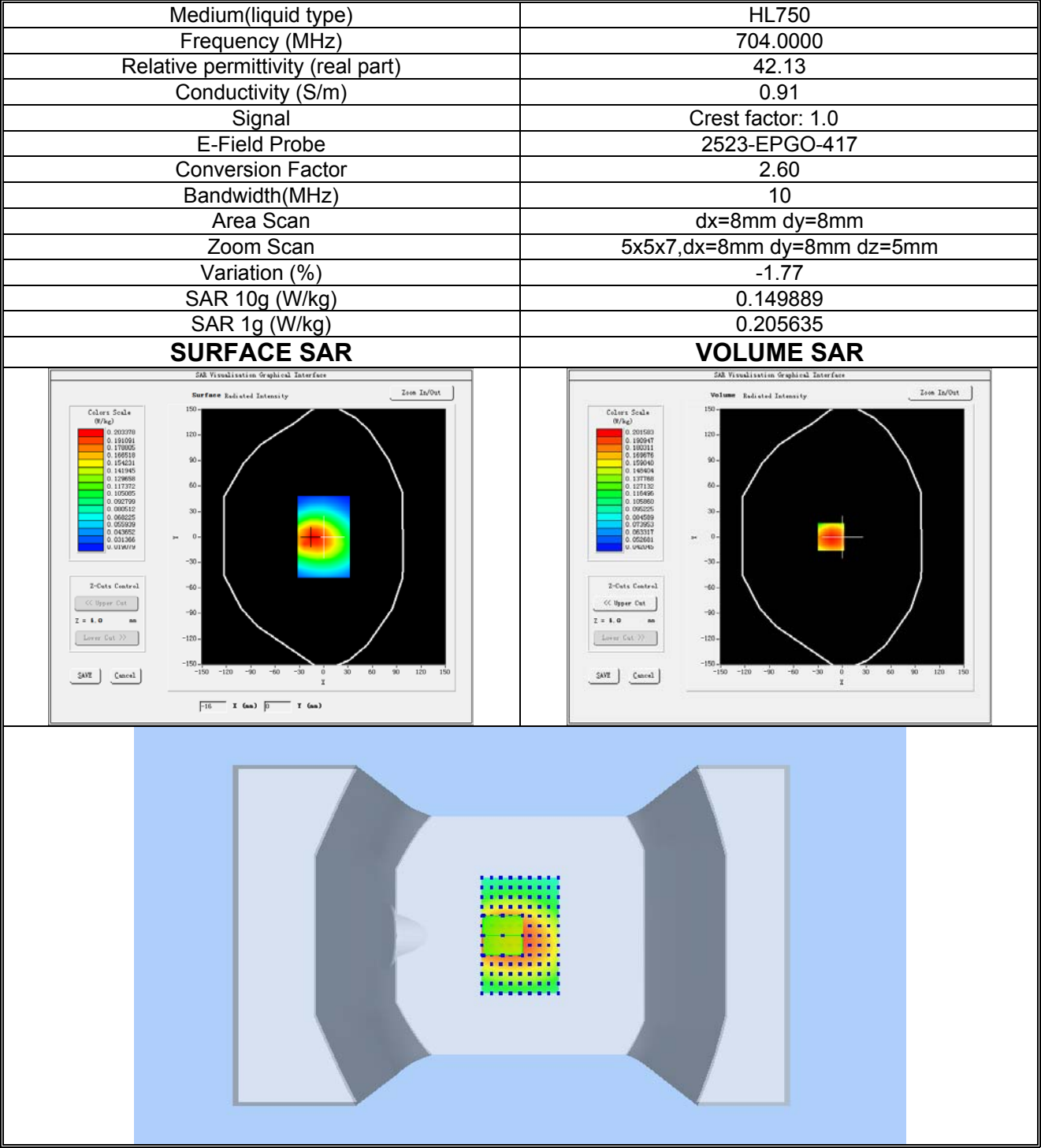
Plot 8: LTE BAND 12, Low channel (Body-worn, Front Side) Product Description: LTE MiFi Router Test Date: 2024-02-27
