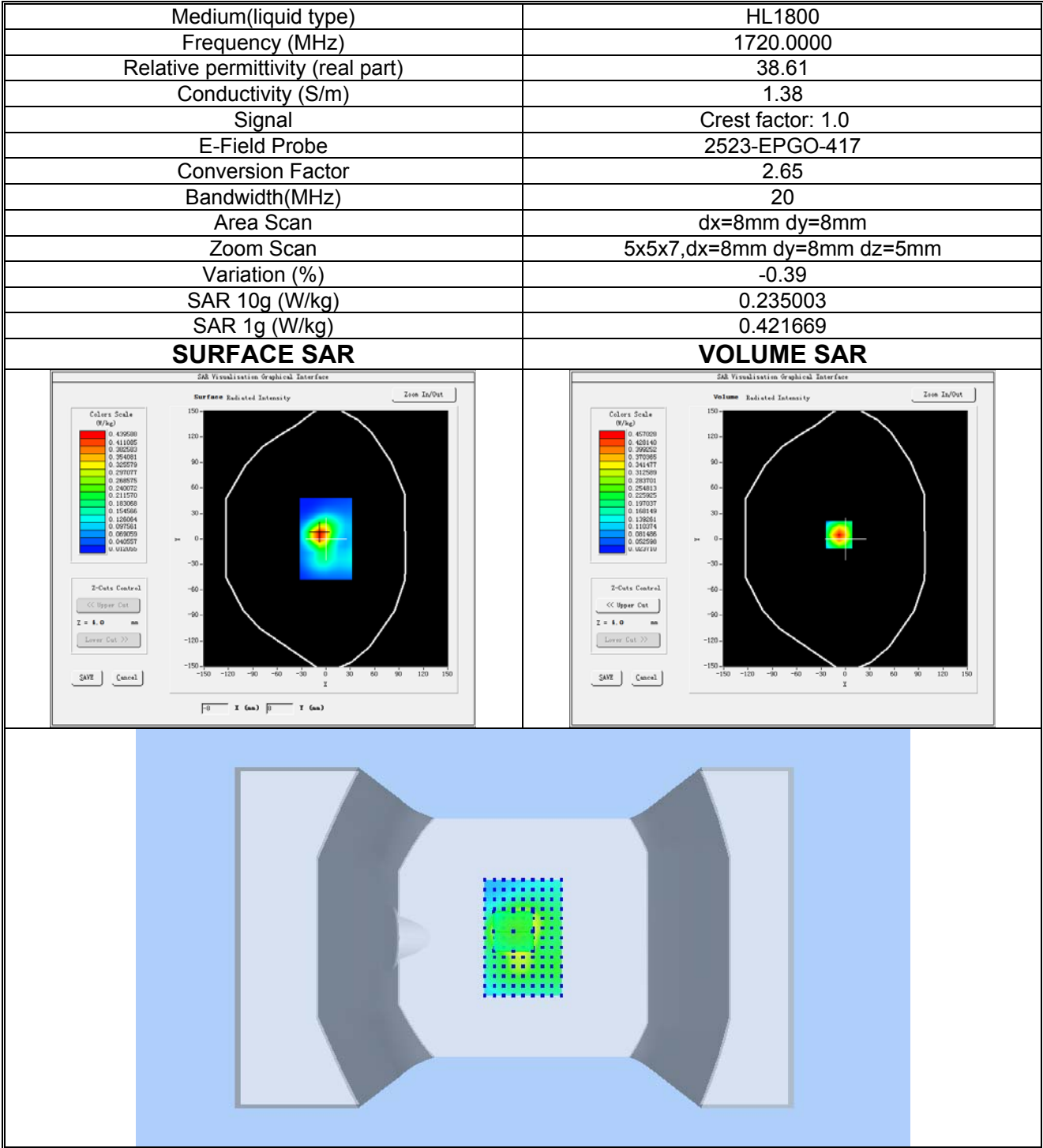
Plot 6: LTE BAND 4, Low channel (Body-worn, Front Side) Product Description: LTE MiFi Router Test Date: 2024-02-26
