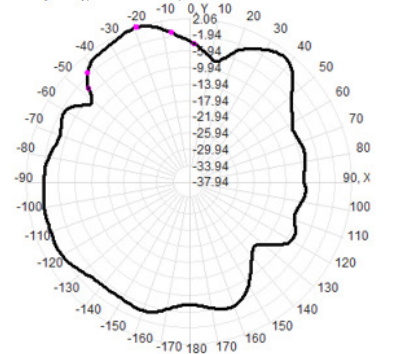
Total(H-XY), Max= 2.03dBi, CirD=17.52
