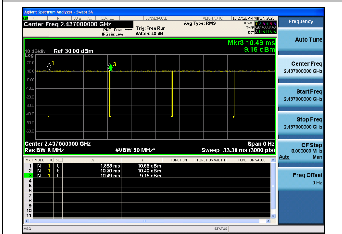
NTNV-11B-Ant1-2437
