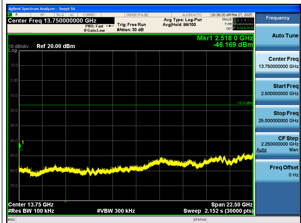
Test_Graph_802.11b_ANT2_2462_1Mbps_Higher Band Emissions
