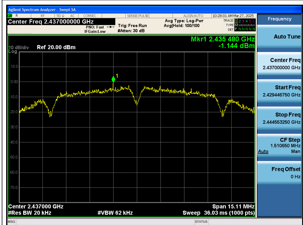
Test_Graph_802.11b_ANT2_2437_1Mbps_PSD
