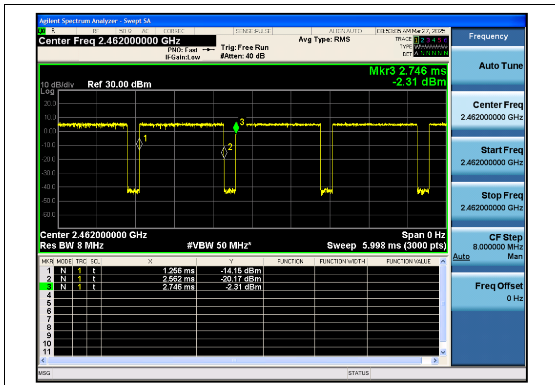
NTNV-11N20SISO-Ant1-2462
