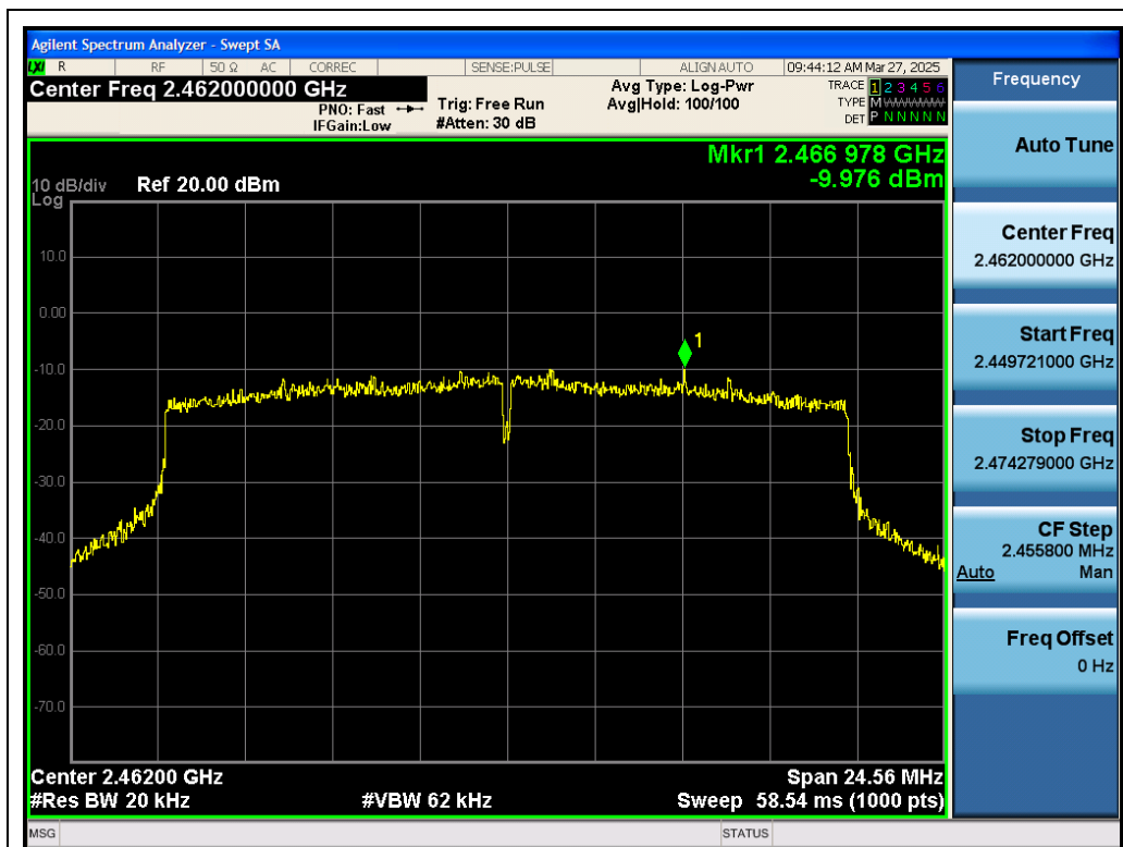
Test_Graph_802.11ax20_ANT2_2462_MCS0_PSD
