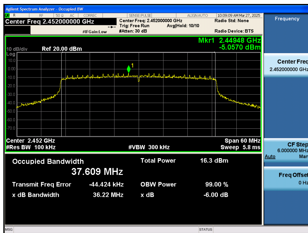
Test_Graph_802.11ax40_ANT2_2452_MCS0_DTSBW
