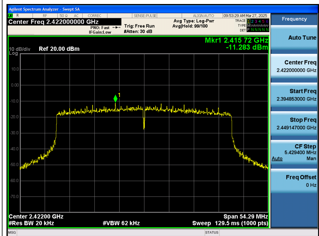
Test_Graph_802.11ax40_ANT2_2422_MCS0_PSD
