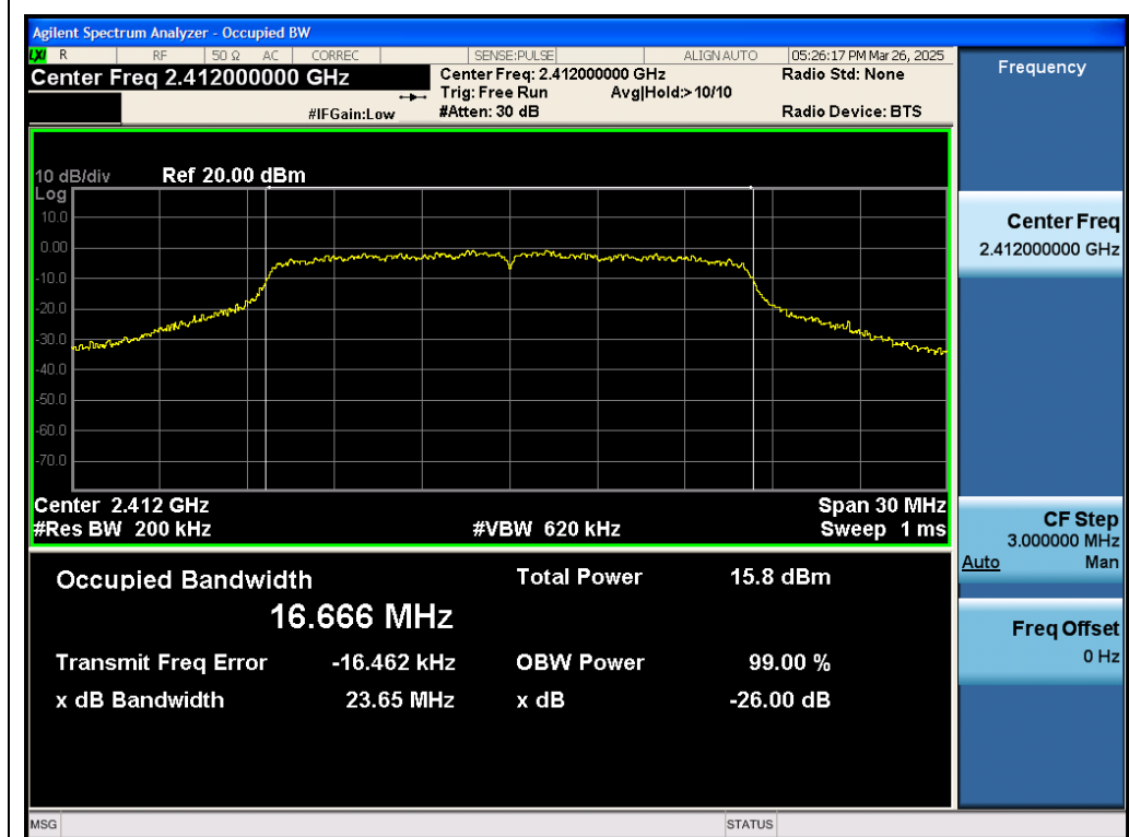
Test_Graph_802.11g_ANT2_2412_6Mbps_OBW
