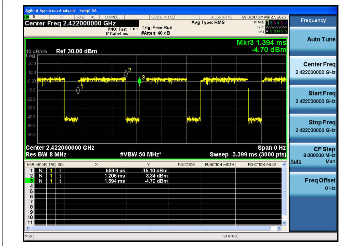
NTNV-11N40SISO-Ant1-2422
