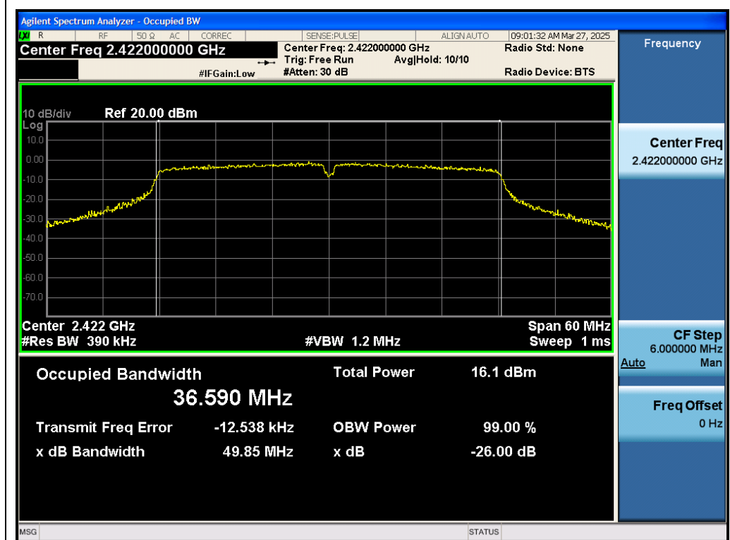
Test_Graph_802.11n40_ANT2_2422_MCS0_OBW
