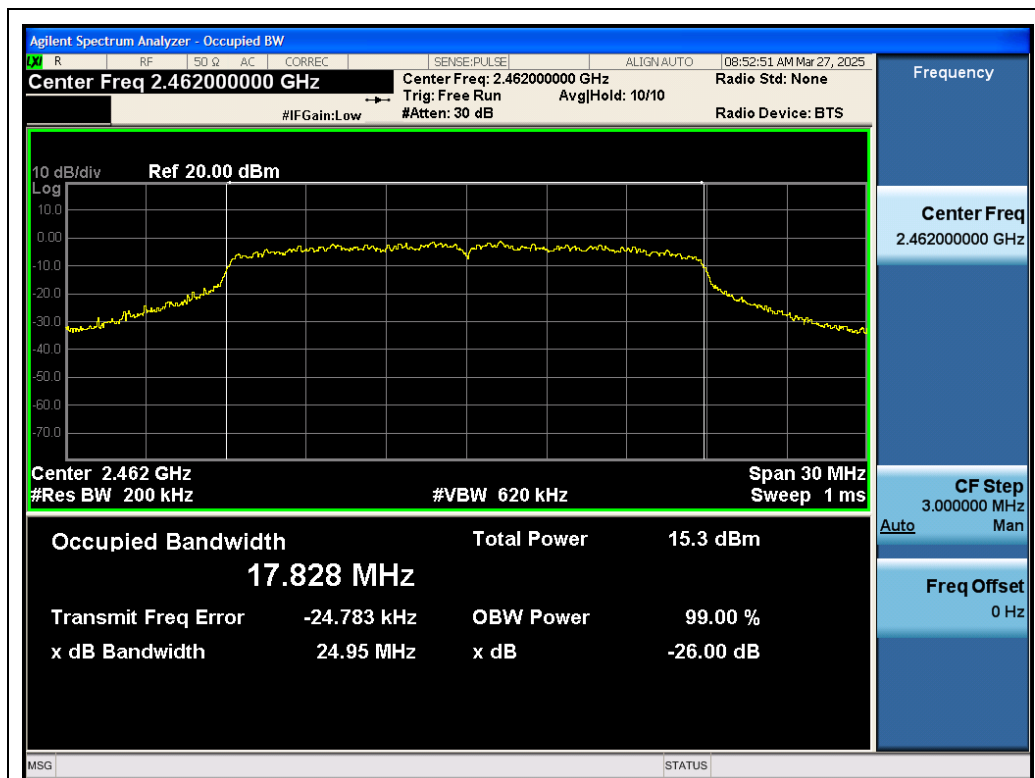
Test_Graph_802.11n20_ANT2_2462_MCS0_OBW
