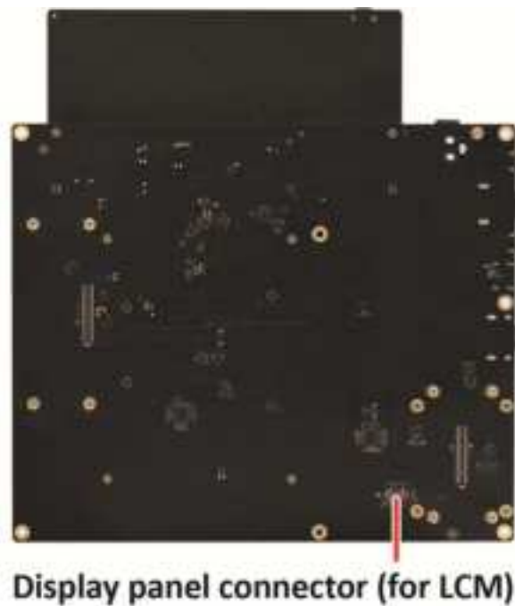
Figure 3-11. Locate Display Panel Connector
