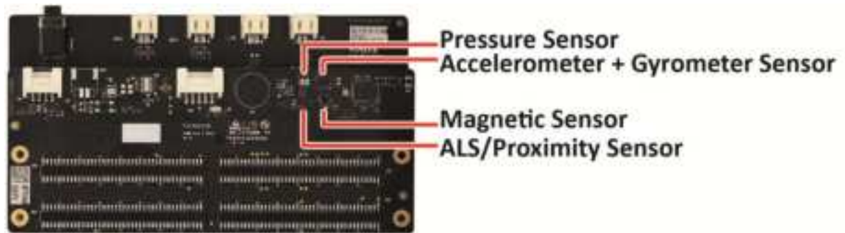
Figure 3-16. Locate Sensors
