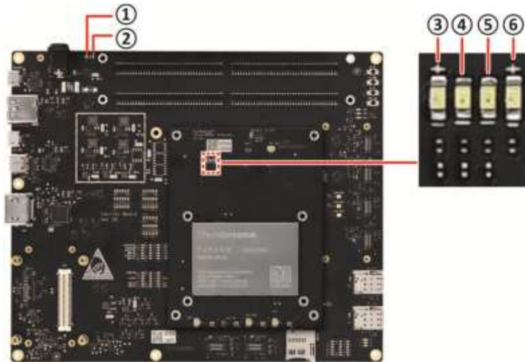
Figure 3-15. Locate LEDs
