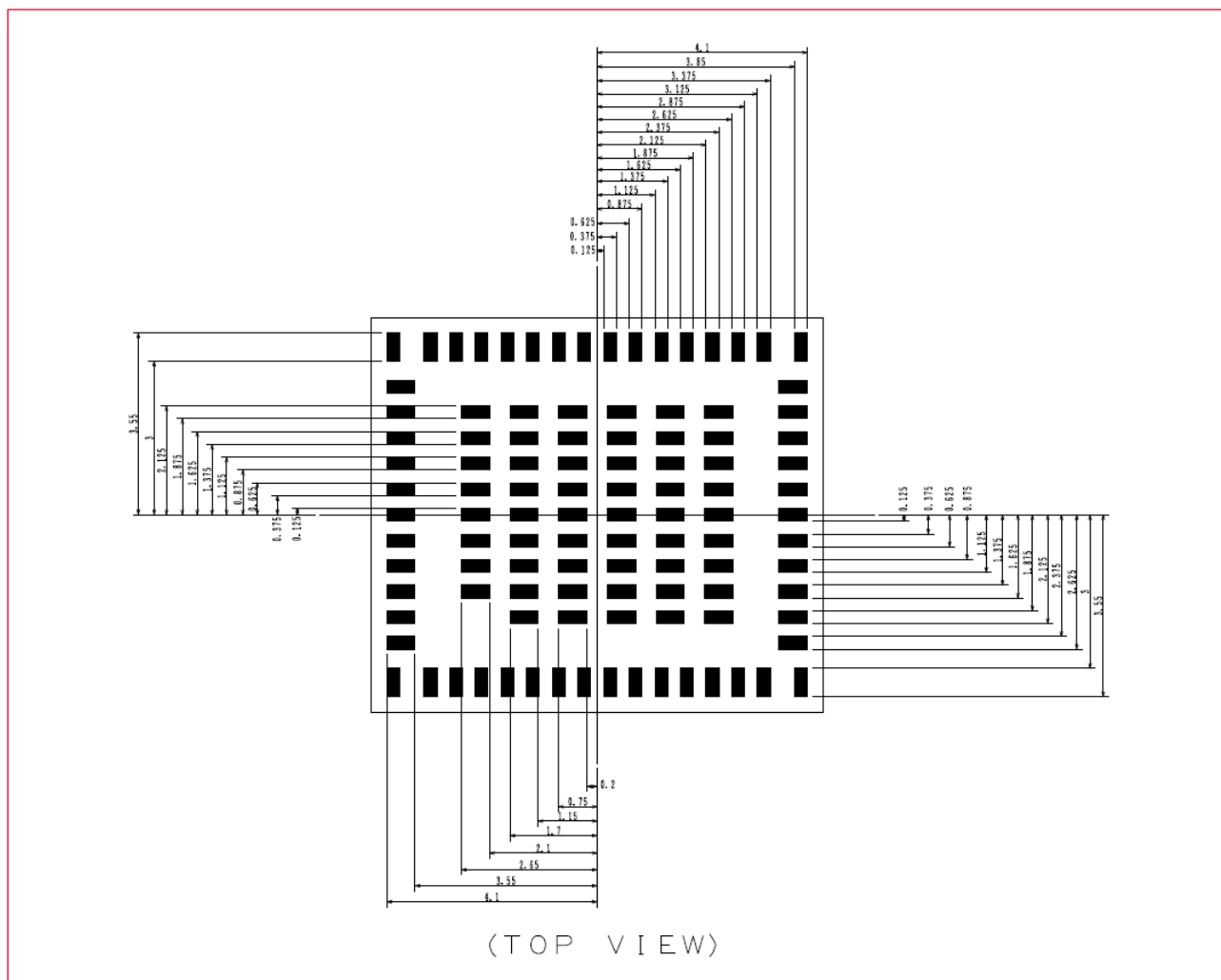
Figure 22: Land Pattern (in mm)
