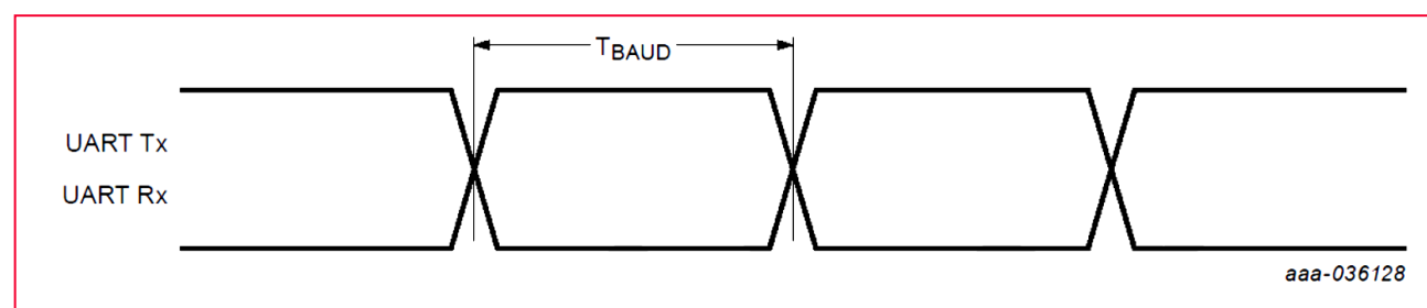
Figure 16: UART Timing Default Mode Signals
