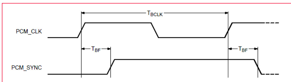
Figure 18: PCM_SYNC Signals (Master Mode)
