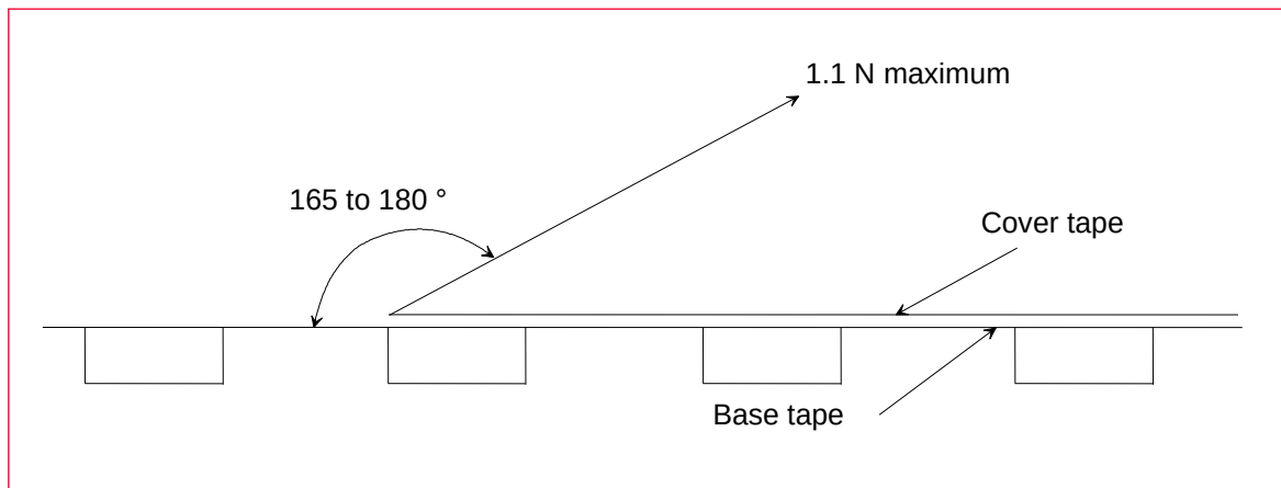
Figure 27: Peeling Force
