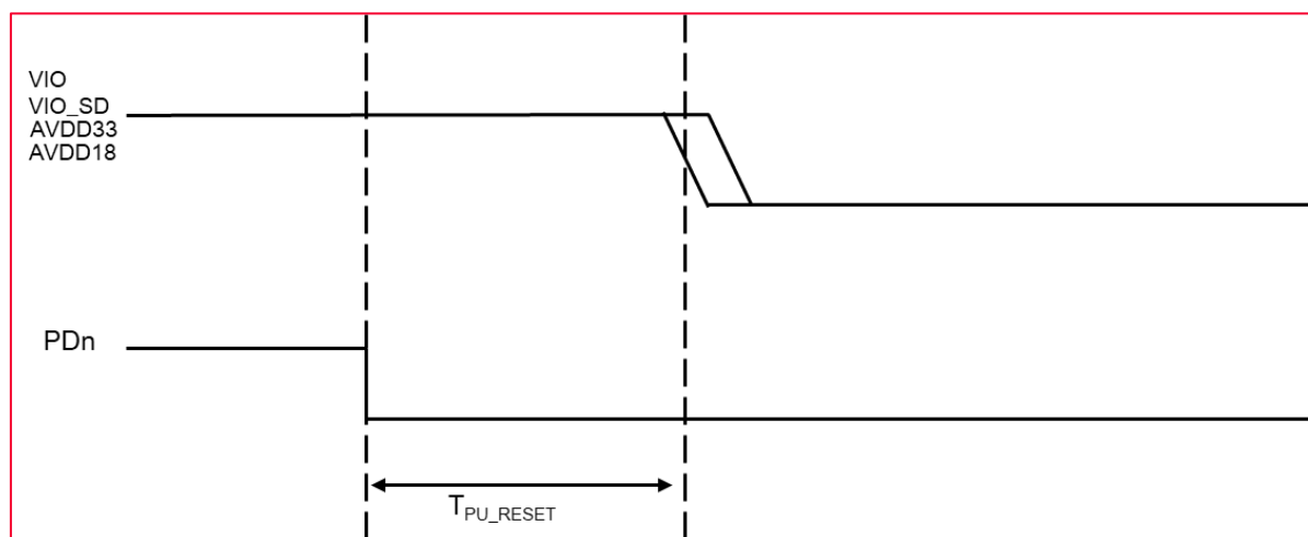
Figure 8: Power-Off Sequence
