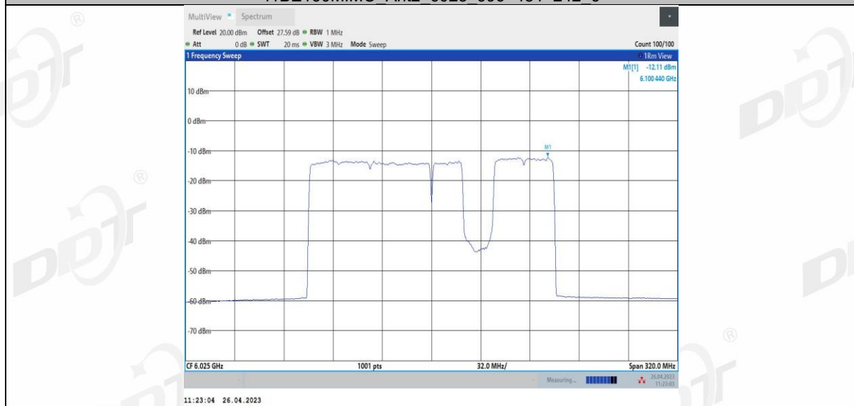
11BE160MIMO Ant2 6025_996+484+242_7
