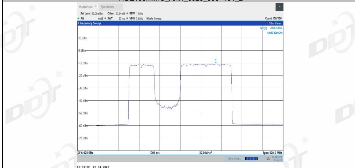
11BE160MIMO Ant4_6025_996+484_3
