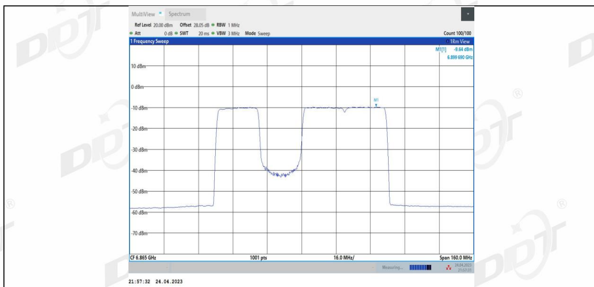
11BE80MIMO Ant3 6865 484+242_3
