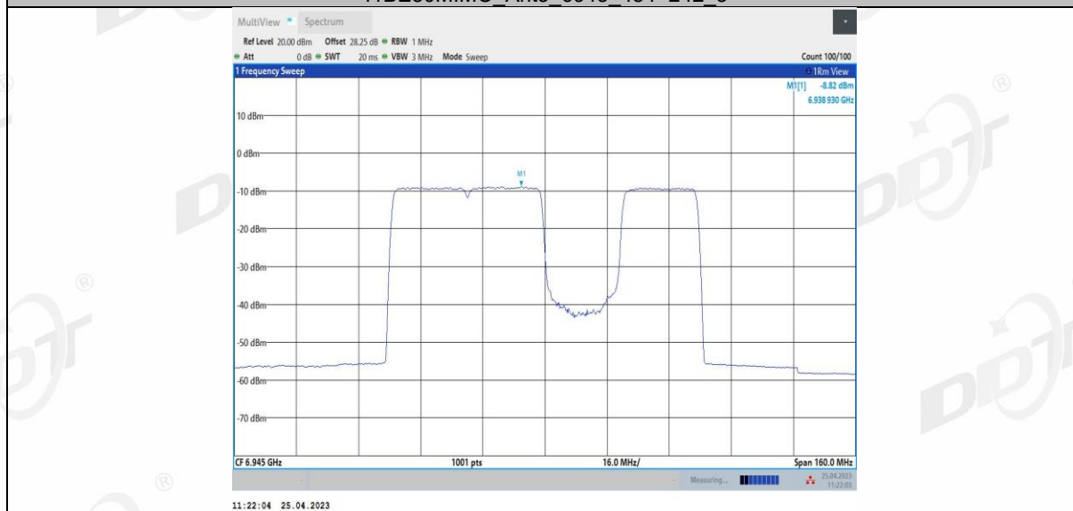
11BE80MIMO Ant3 6945 484+242 4
