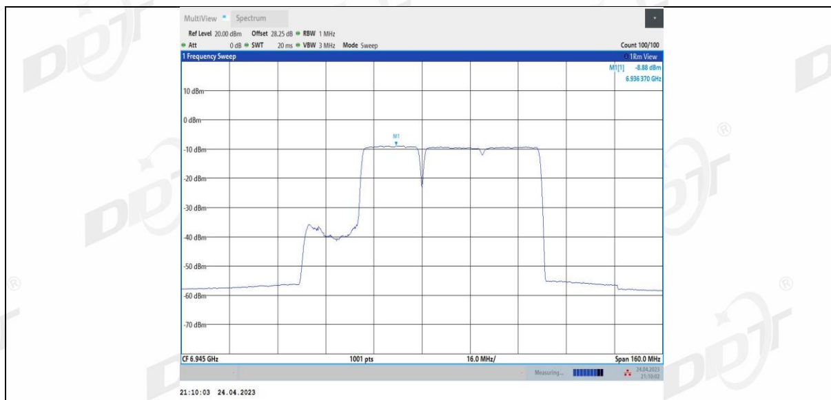
11BE80MIMO Ant3 6945 484+242 2
