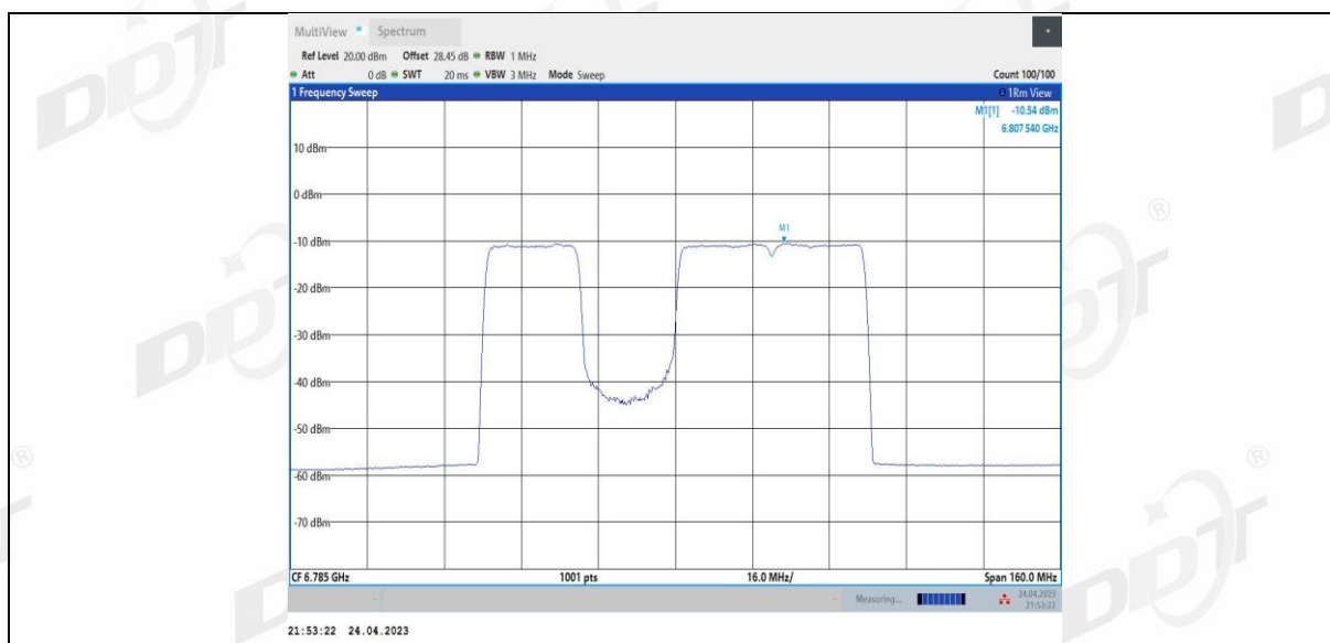
11BE80MIMO Ant4 6785 484+242_3
