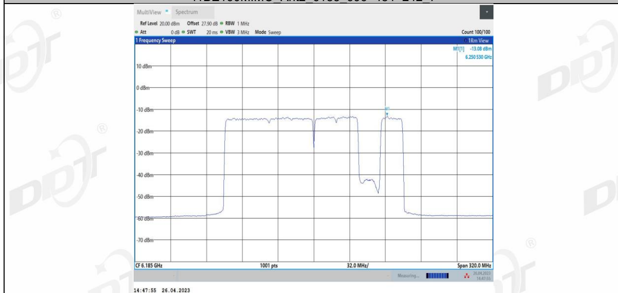
11BE160MIMO Ant2 6185 996+484+242 8
