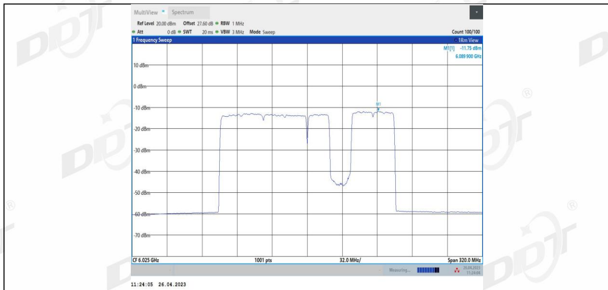
11BE160MIMO Ant3 6025_996+484+242_7
