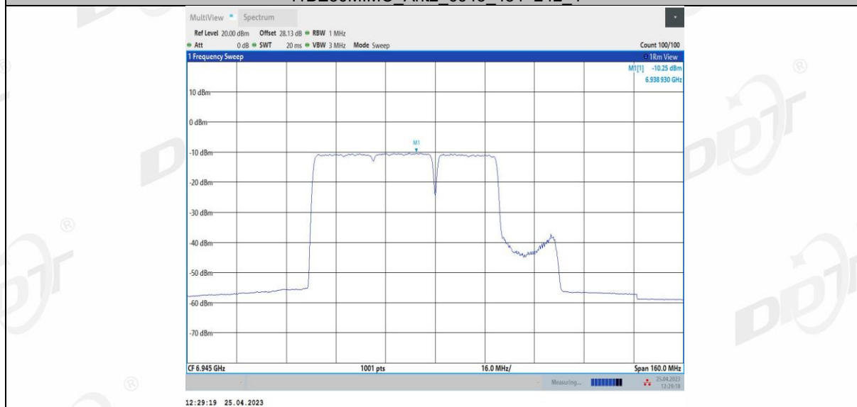
11BE80MIMO Ant3 6945 484+242_1
