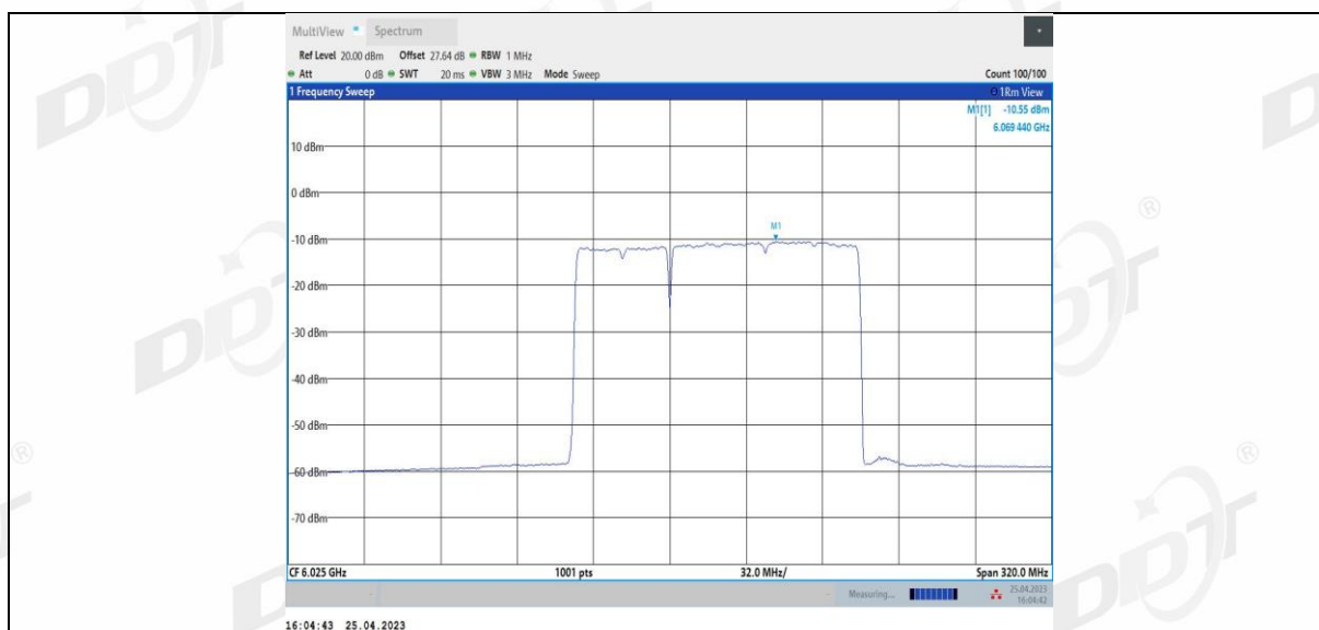
11BE160MIMO Ant4_6025_996+484_2
