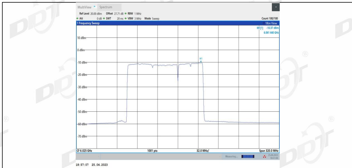
11BE160MIMO Ant1_6025_996+484+242_5
