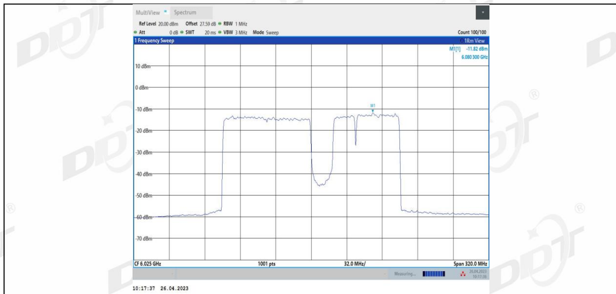
11BE160MIMO Ant2 6025_996+484+242_6
