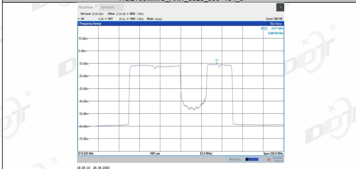
11BE160MIMO Ant4_6025_996+484_4
