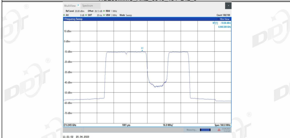
11BE80MIMO Ant2 6945 484+242_4
