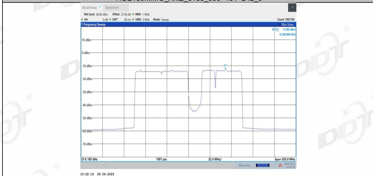
11BE160MIMO Ant2 6185 996+484+242 6
