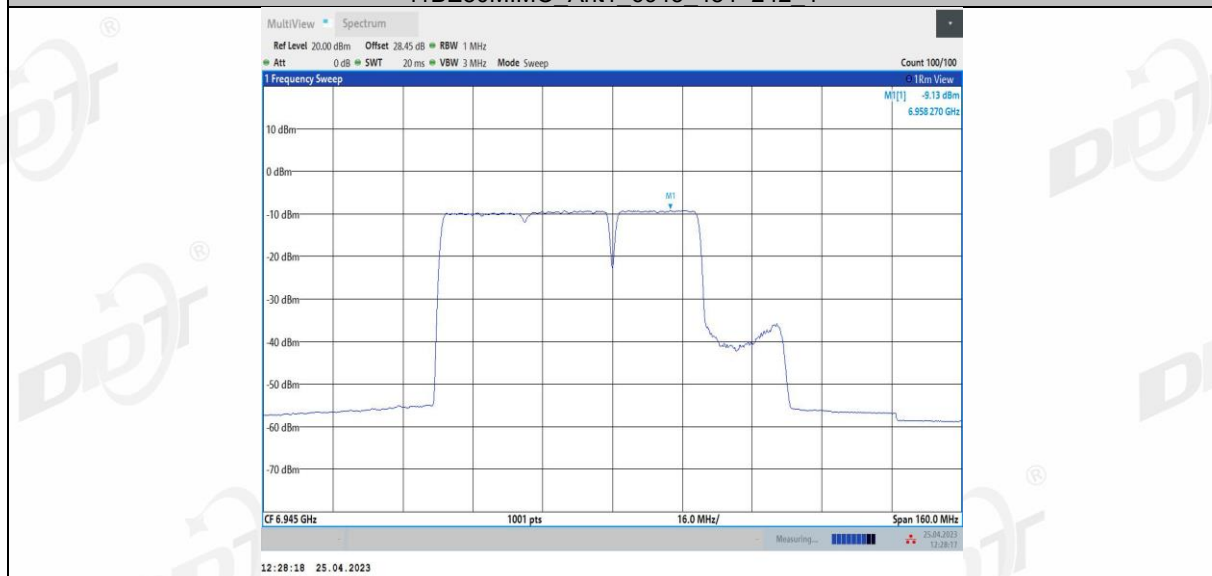
11BE80MIMO Ant2 6945 484+242 1
