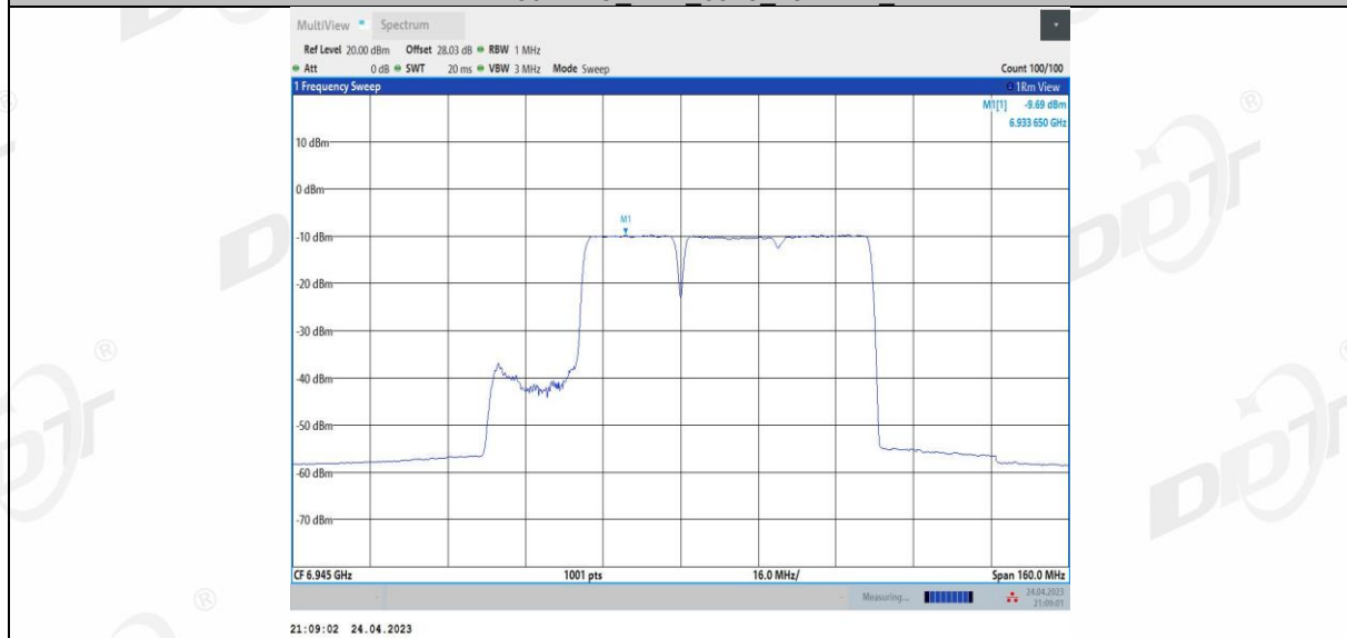
11BE80MIMO Ant2 6945 484+242 2
