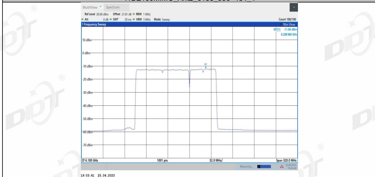
11BE160MIMO Ant2 6185 996+484+242 5
