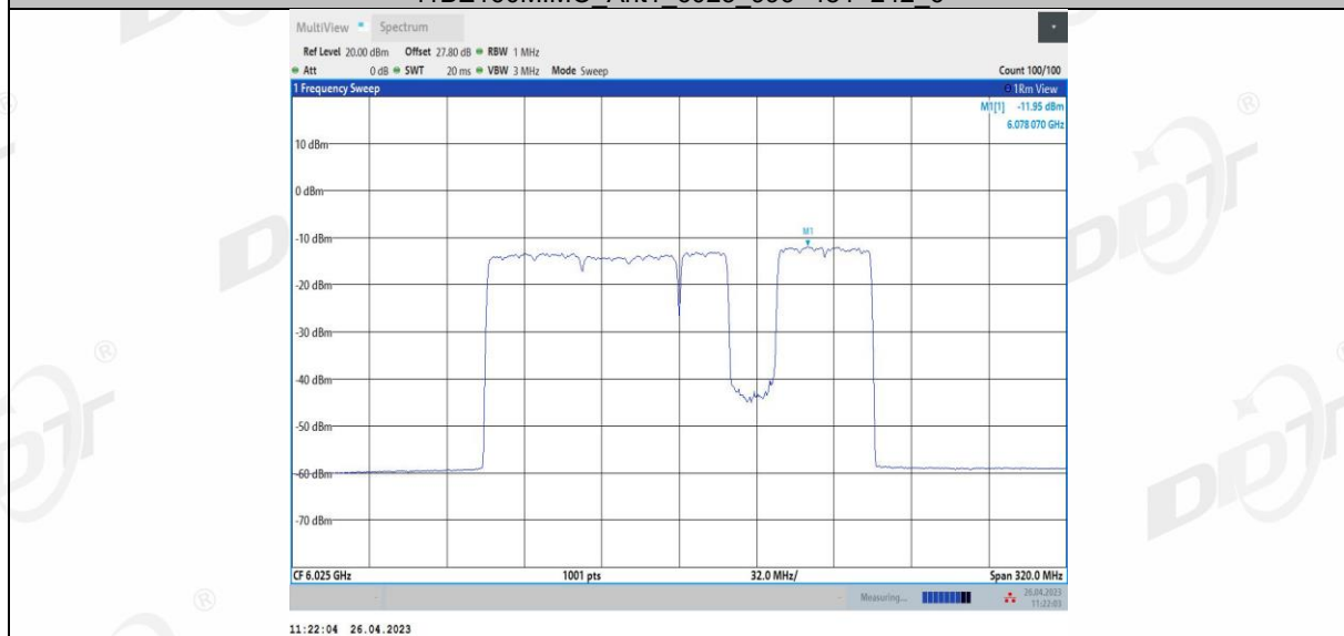
11BE160MIMO Ant1_6025_996+484+242_7
