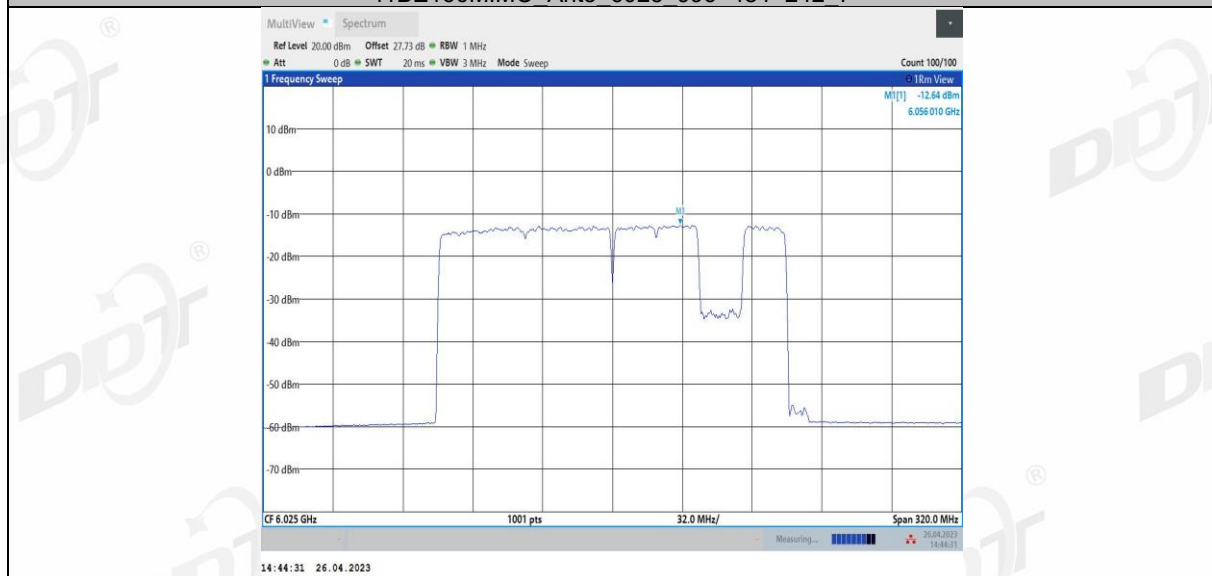
11BE160MIMO Ant3 6025_996+484+242_8
