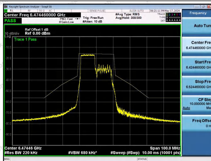
NTNV-11AX20SISO-Ant1-6475-106Tone-RU53-PASS
