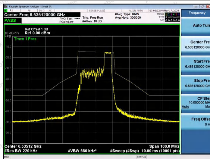
NTNV-11AX20SISO-Ant1-6535-52Tone-RU40-PASS
