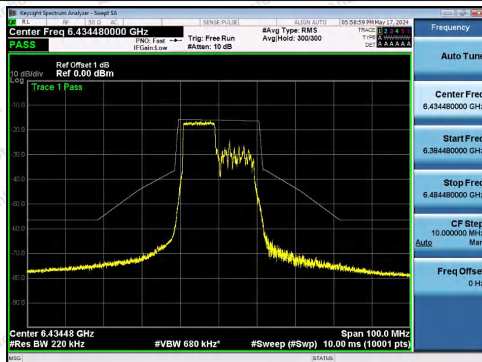
NTNV-11AX20SISO-Ant1-6435-106Tone-RU53-PASS
