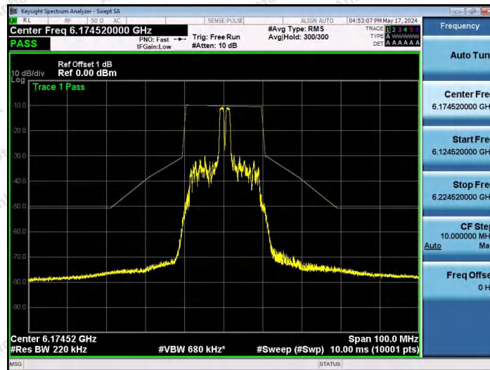
NTNV-11AX20SISO-Ant1-6175-26Tone-RU4-PASS
