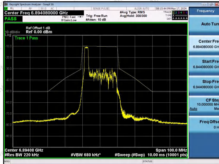
NTNV-11AX20SISO-Ant1-6895-26Tone-RU0-PASS
