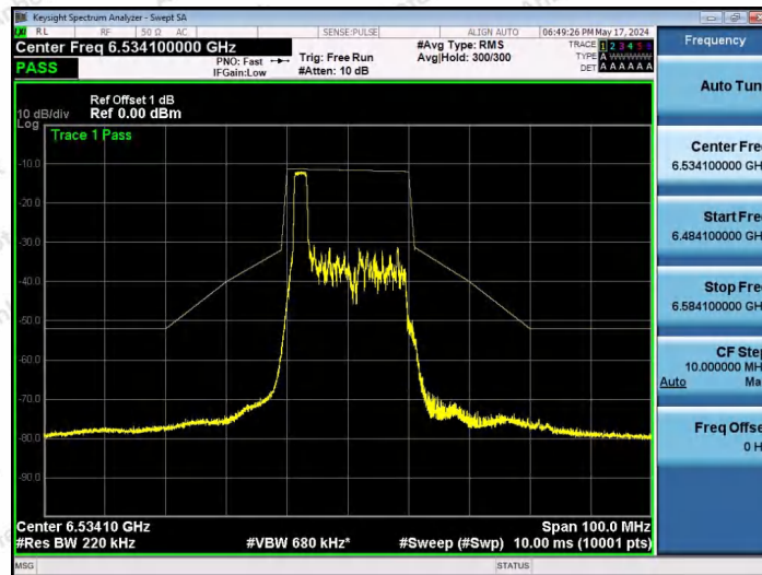
NTNV-11AX20SISO-Ant1-6535-26Tone-RU0-PASS
