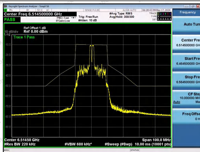
NTNV-11AX20SISO-Ant1-6515-26Tone-RU4-PASS
