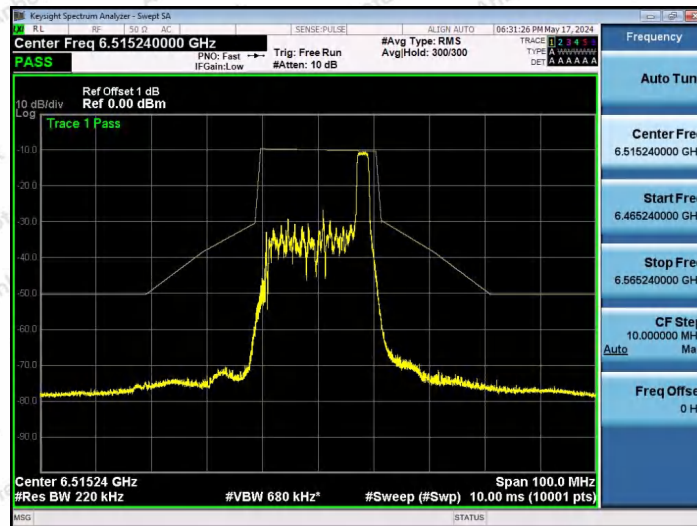
NTNV-11AX20SISO-Ant1-6515-26Tone-RU8-PASS
