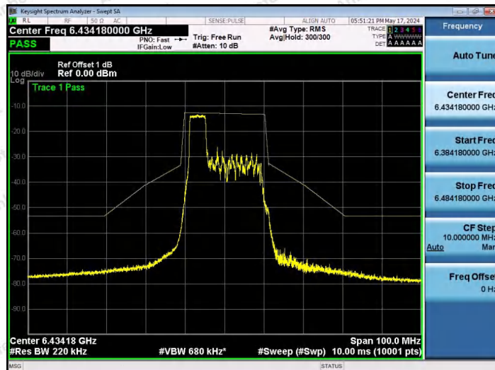
NTNV-11AX20SISO-Ant1-6435-52Tone-RU37-PASS
