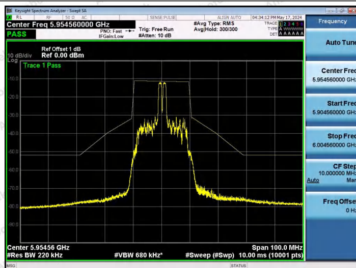
NTNV-11AX20SISO-Ant1-5955-26Tone-RU4-PASS
