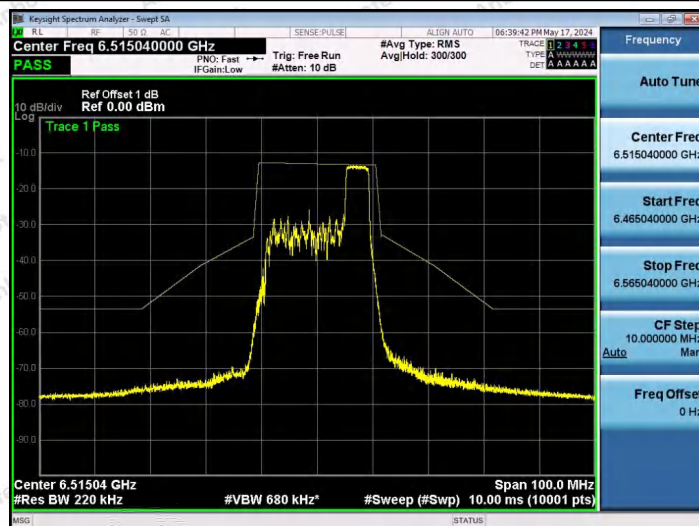
NTNV-11AX20SISO-Ant1-6515-52Tone-RU40-PASS
