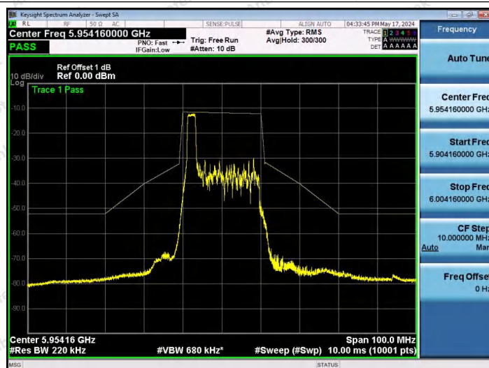
NTNV-11AX20SISO-Ant1-5955-26Tone-RU0-PASS
