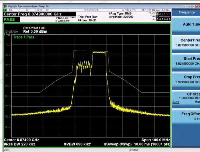
NTNV-11AX20SISO-Ant1-6875-106Tone-RU54-PASS
