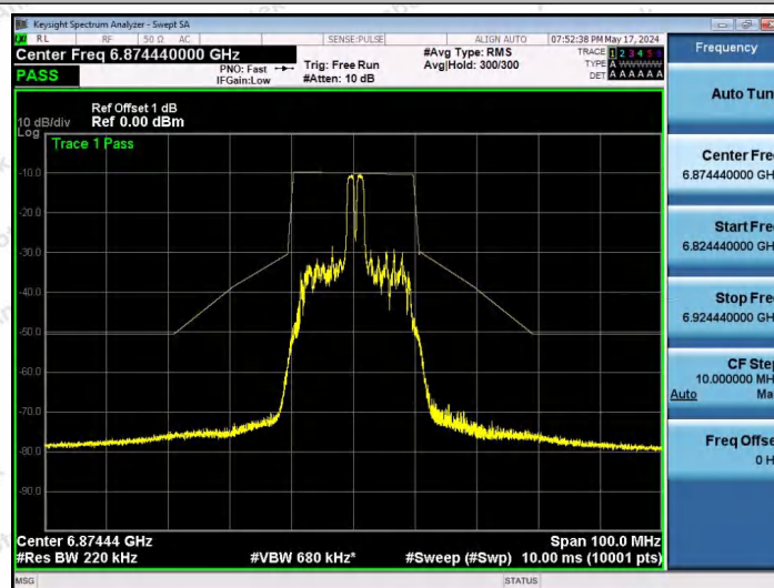
NTNV-11AX20SISO-Ant1-6875-26Tone-RU4-PASS
