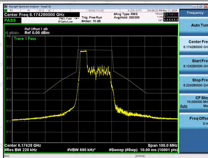
NTNV-11AX20SISO-Ant1-6175-52Tone-RU37-PASS
