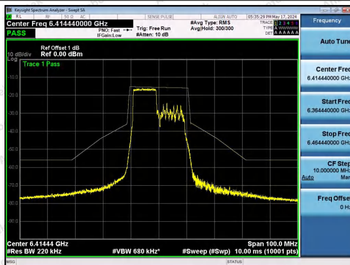
NTNV-11AX20SISO-Ant1-6415-106Tone-RU53-PASS
