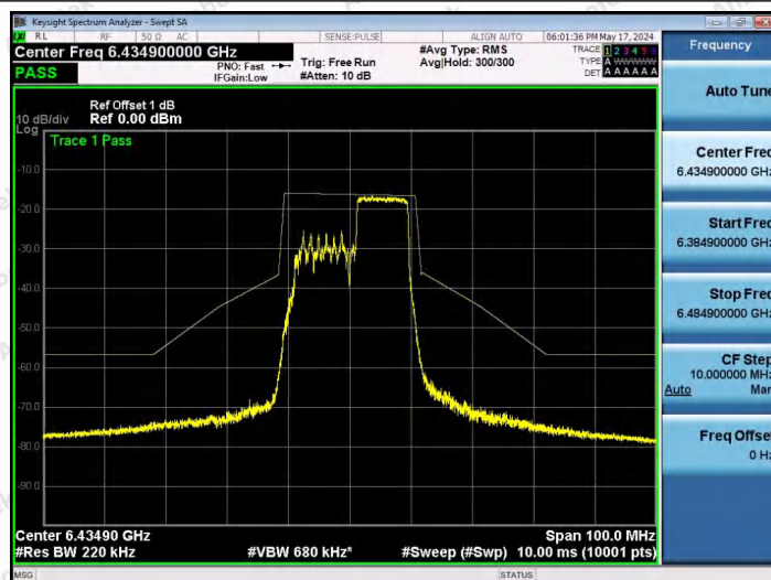
NTNV-11AX20SISO-Ant1-6435-106Tone-RU54-PASS
