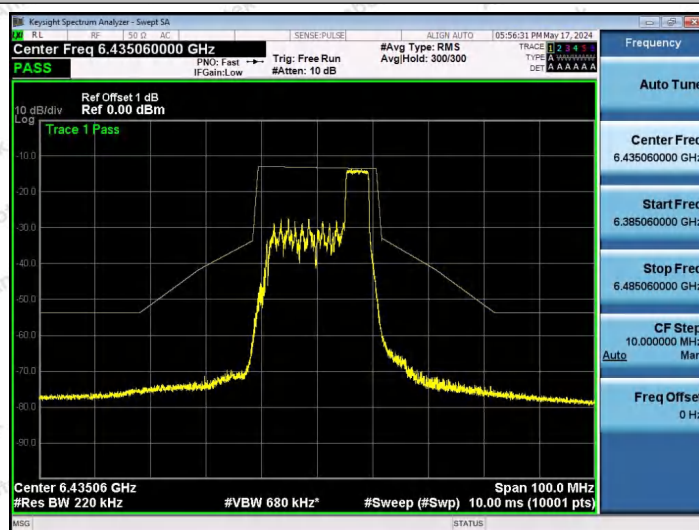
NTNV-11AX20SISO-Ant1-6435-52Tone-RU40-PASS
