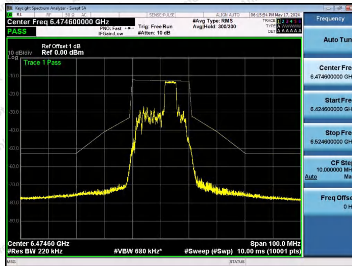
NTNV-11AX20SISO-Ant1-6475-52Tone-RU39-PASS
