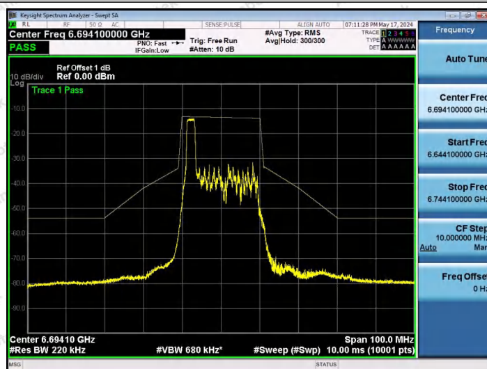
NTNV-11AX20SISO-Ant1-6695-26Tone-RU0-PASS
