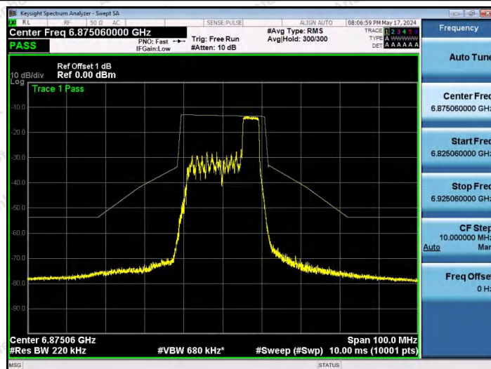
NTNV-11AX20SISO-Ant1-6875-52Tone-RU40-PASS
