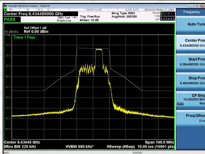
NTNV-11AX20SISO-Ant1-6435-52Tone-RU39-PASS
