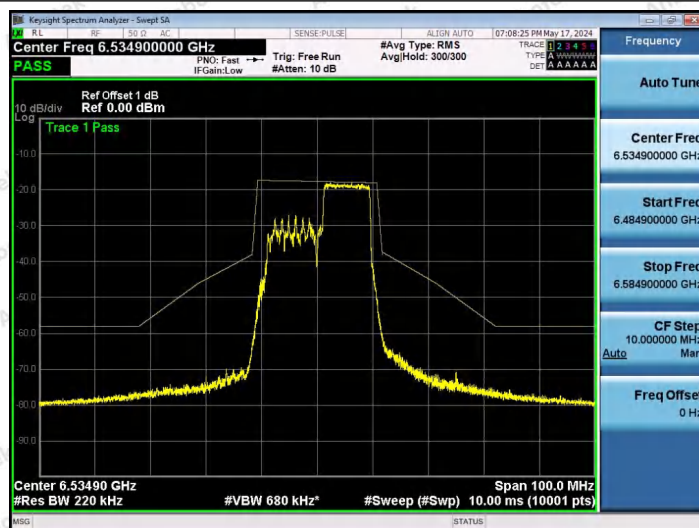
NTNV-11AX20SISO-Ant1-6535-106Tone-RU54-PASS
