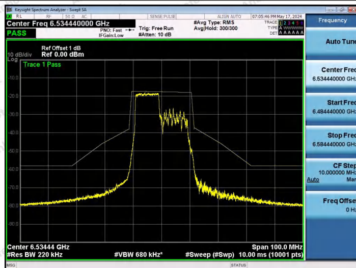
NTNV-11AX20SISO-Ant1-6535-106Tone-RU53-PASS
