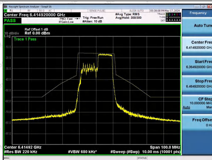
NTNV-11AX20SISO-Ant1-6415-106Tone-RU54-PASS
