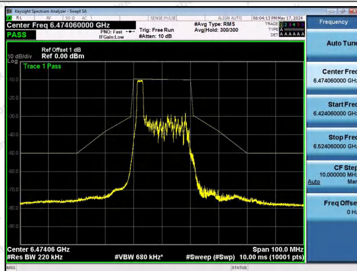
NTNV-11AX20SISO-Ant1-6475-26Tone-RU0-PASS
