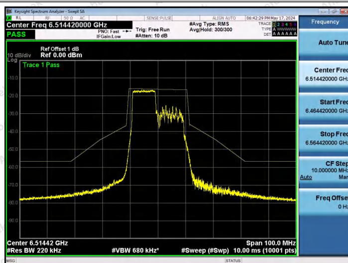
NTNV-11AX20SISO-Ant1-6515-106Tone-RU53-PASS
