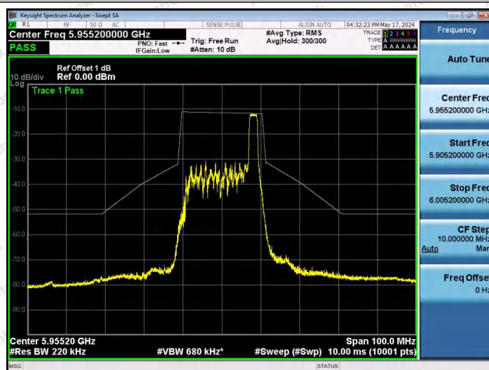
NTNV-11AX20SISO-Ant1-5955-26Tone-RU8-PASS
