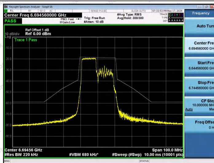
NTNV-11AX20SISO-Ant1-6695-106Tone-RU53-PASS
