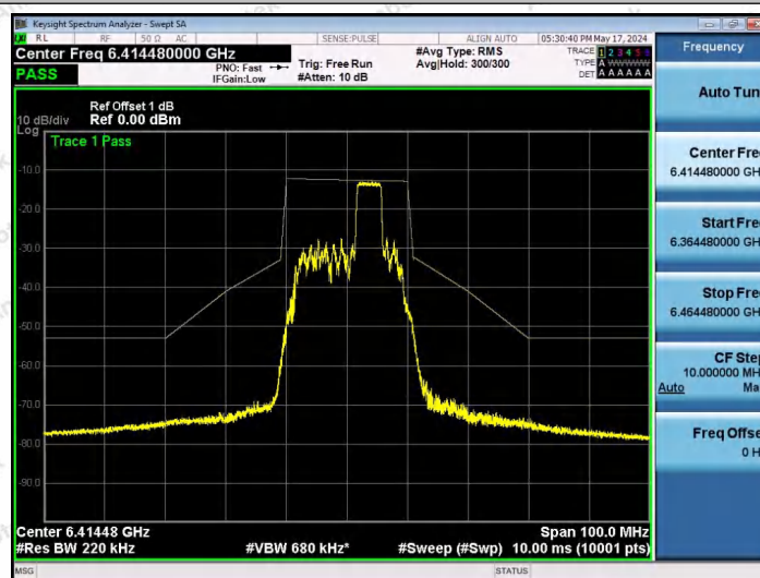
NTNV-11AX20SISO-Ant1-6415-52Tone-RU39-PASS
