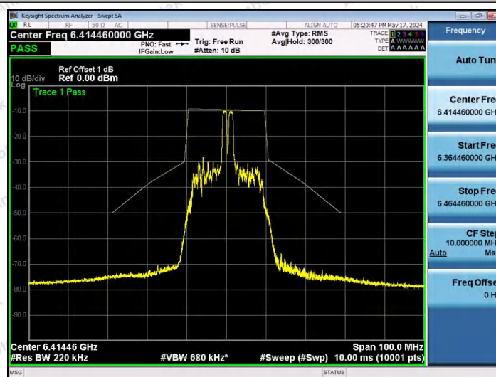
NTNV-11AX20SISO-Ant1-6415-26Tone-RU4-PASS
