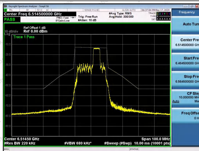
NTNV-11AX20SISO-Ant1-6515-52Tone-RU39-PASS
