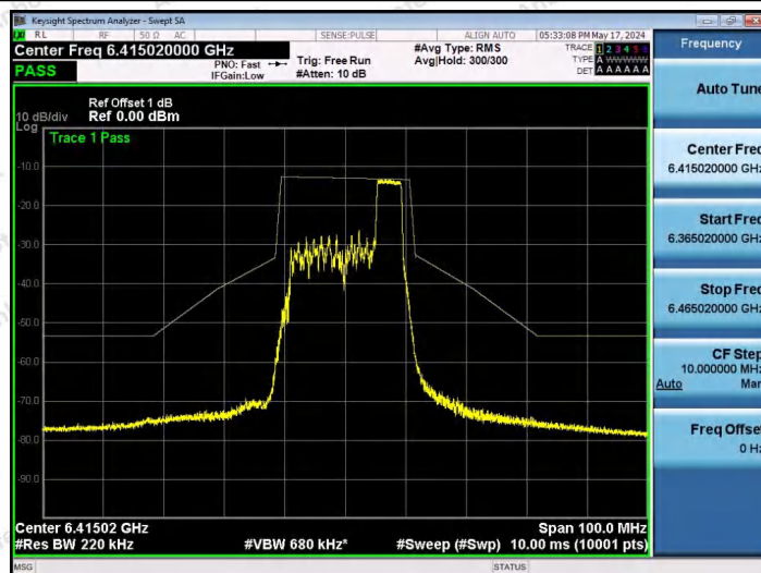
NTNV-11AX20SISO-Ant1-6415-52Tone-RU40-PASS
