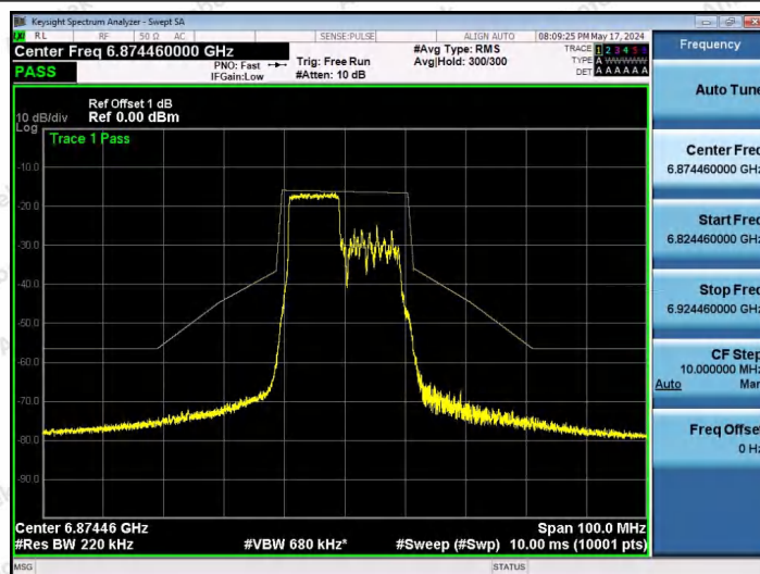
NTNV-11AX20SISO-Ant1-6875-106Tone-RU53-PASS
