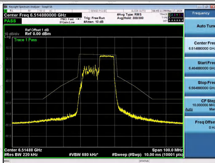
NTNV-11AX20SISO-Ant1-6515-106Tone-RU54-PASS
