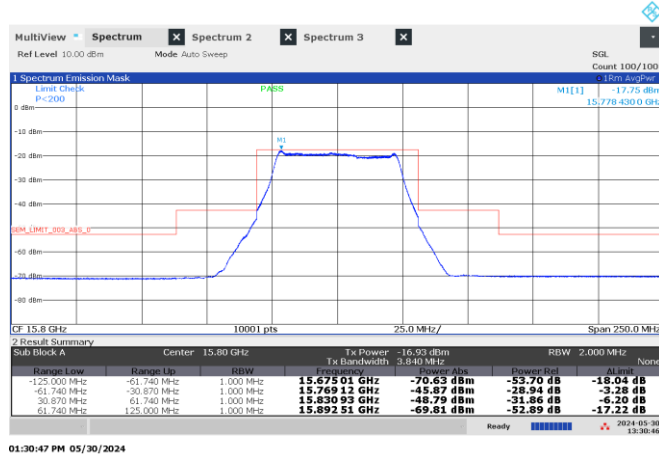
Figure 8.4-47: Emission mask, Low channel: 15.80 GHz, shortest pulse. (50 MHz BW)
