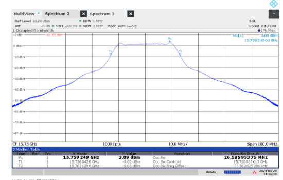
Figure 8.1-13: 99% OBW Low channel: 15.75 GHz, shortest pulse (25 MHz BW)
