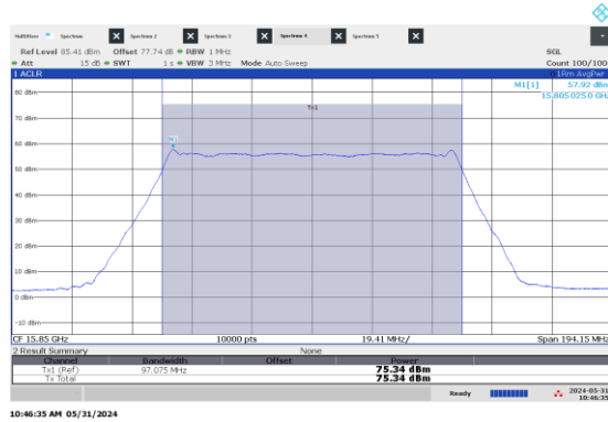
Figure 8.3-19: EIRP Power, Low channel: 15.85 GHz, shortest pulse (100 MHz BW)
