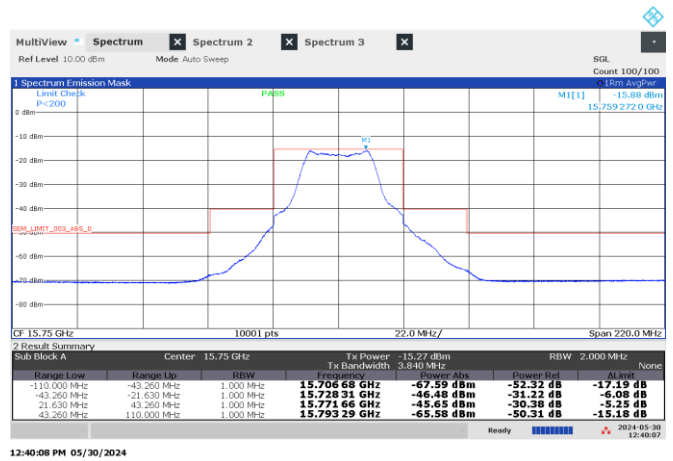
Figure 8.4-38: Emission mask, Low channel: 15.75 GHz, shortest pulse. (25 MHz BW)
