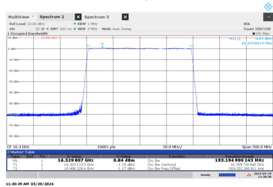
Figure 8.1-24: 99% OBW High channel: 16.40 GHz, shortest pulse (200 MHz BW)
