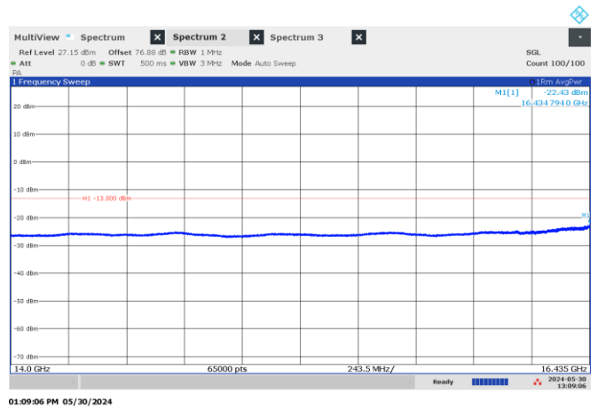
Figure 8.4-44: Emission mask, beyond \pm 250\% of BW (low frequency range), High channel: 16.55 GHz, shortest pulse. (25 MHz BW)
