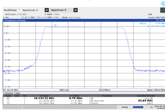
Figure 8.2-5: 26 dB OBW Middle channel: 16.15 GHz, longest pulse (50 MHz BW)
