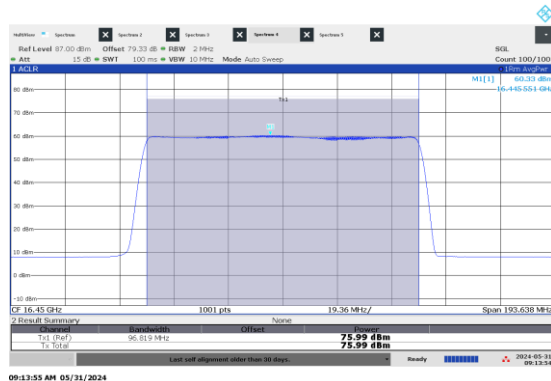
Figure 8.3-9: EIRP Power, High channel: 16.45 GHz, longest pulse (100 MHz BW)
