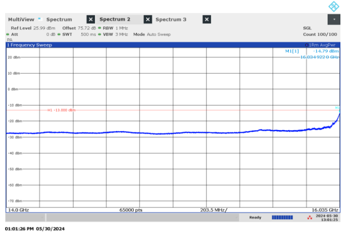
Figure 8.4-40: Emission mask, beyond \pm 250\% of BW (low frequency range), Middle channel: 16.15 GHz, shortest pulse. (25 MHz BW)
