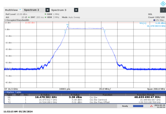
Figure 8.1-18: 99% OBW High channel: 16.50 GHz, shortest pulse (50 MHz BW)
