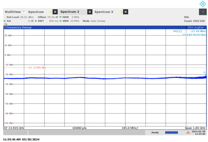
Figure 8.4-34: Emission mask, beyond \pm 250\% of BW (low frequency range), High channel: 16.40 GHz, longest pulse. (200 MHz BW)
