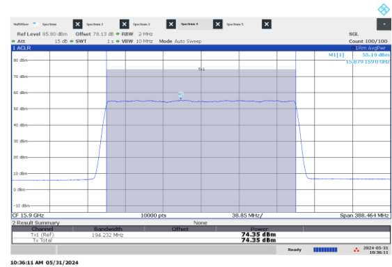
Figure 8.3-22: EIRP Power, Low channel: 15.90 GHz, shortest pulse (200 MHz BW)
