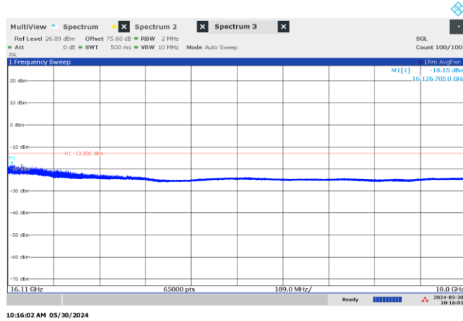
Figure 8.4-21: Emission mask, beyond \pm 250\% of BW (high frequency range), Low channel: 15.85 GHz, longest pulse. (100 MHz BW)
