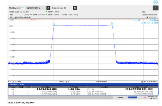
Figure 8.1-22: 99% OBW Low channel: 15.90 GHz, shortest pulse (200 MHz BW)
