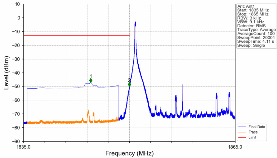
Band25_15MHz_16QAM_LCH_1857.5MHz_RB_1_0_NTNV
