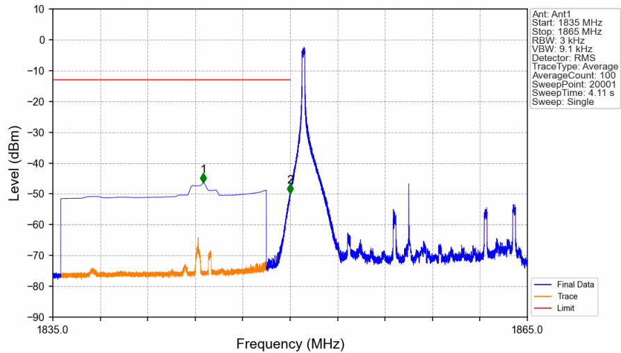
Band25_15MHz_QPSK_LCH_1857.5MHz_RB_1_0_NTNV
