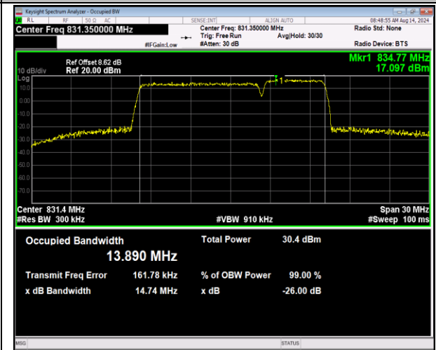
5-5-10MHz-5MHz-QPSK-QPSK-20450-20522-50RB#0-2 5RB#0-PASS
