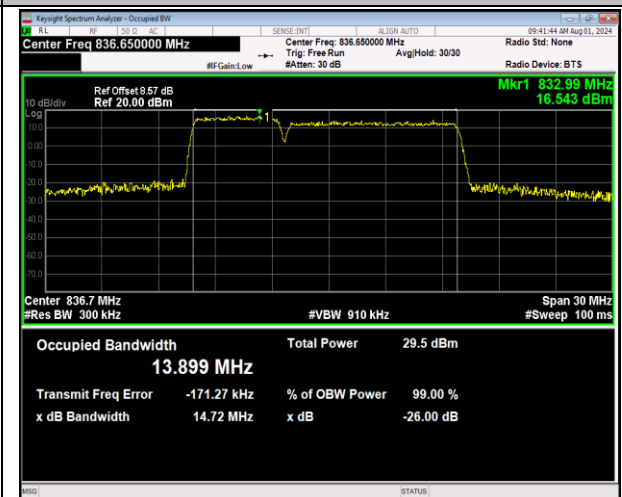
5-5-5MHz-10MHz-64QAM-64QAM-20478-20550-25RB# 0-50RB#0-PASS
