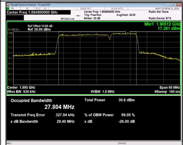
2-2-20MHz-10MHz-64QAM-64QAM-19001-19145-100RB#0-50RB#0-PASS
