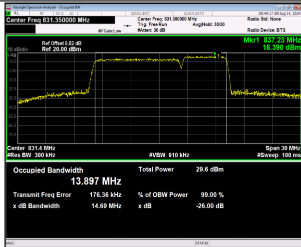
5-5-10MHz-5MHz-16QAM-16QAM-20450-20522-50RB#0- 25RB#0-PASS
