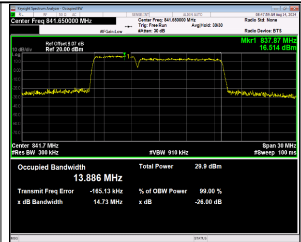
5-5-5MHz-10MHz-16QAM-16QAM-20528-20600-25RB# 0-50RB#0-PASS
