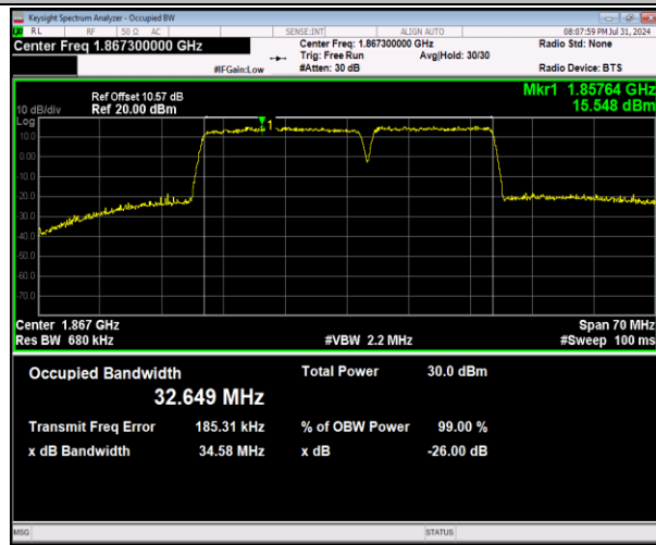
2-2-20MHz-15MHz-64QAM-64QAM-18700-18871-100RB#0-75RB#0-PASS
