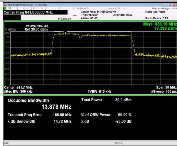
5-5-5MHz-10MHz-64QAM-64QAM-20528-20600-25RB#0- 50RB#0-PASS
