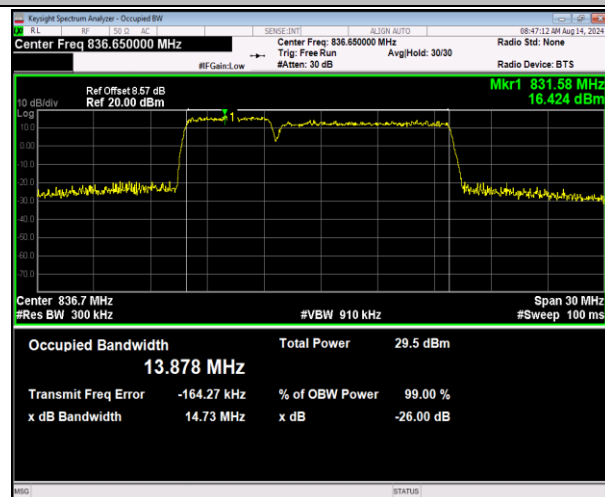
5-5-5MHz-10MHz-16QAM-16QAM-20478-20550-25RB#0- 50RB#0-PASS
