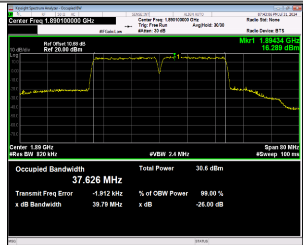
2-2-20MHz-20MHz-64QAM-64QAM-18902-19100-100RB#0-100RB#0-PASS
