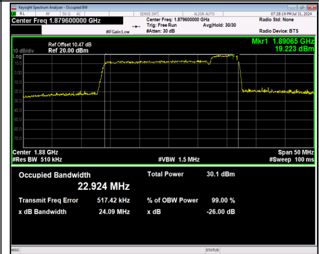
2-2-20MHz-5MHz-64QAM-64QAM-18875-18992-100RB #0-25RB#0-PASS
