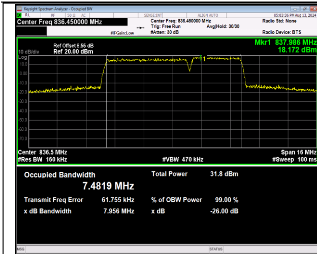
5-5-5MHz-3MHz-QPSK-QPSK-20510-20549-25RB#0-15 RB#0-PASS
