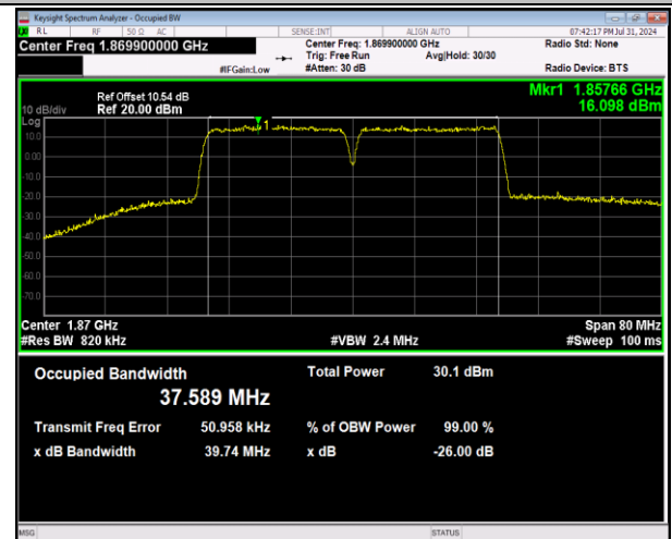
2-2-20MHz-20MHz-64QAM-64QAM-18700-18898-100RB#0-100RB#0-PASS
