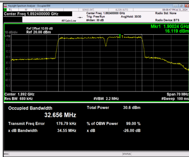
2-2-20MHz-15MHz-64QAM-64QAM-18951-19122-100RB#0-75RB#0-PASS
