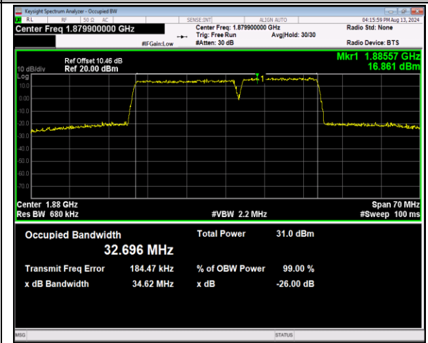
2-2-20MHz-15MHz-QPSK-QPSK-18826-18997-100RB#0-75RB#0-PASS
