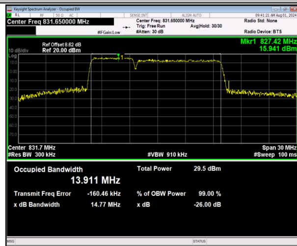
5-5-5MHz-10MHz-64QAM-64QAM-20428-20500-25RB#0- 50RB#0-PASS
