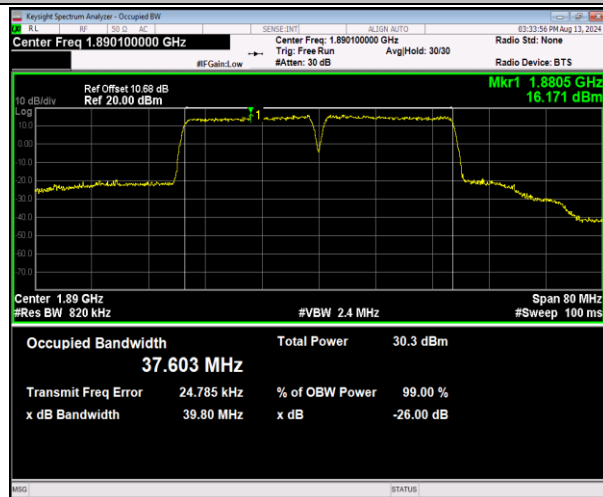
2-2-20MHz-20MHz-16QAM-16QAM-18902-19100-100RB#0-100RB#0-PASS
