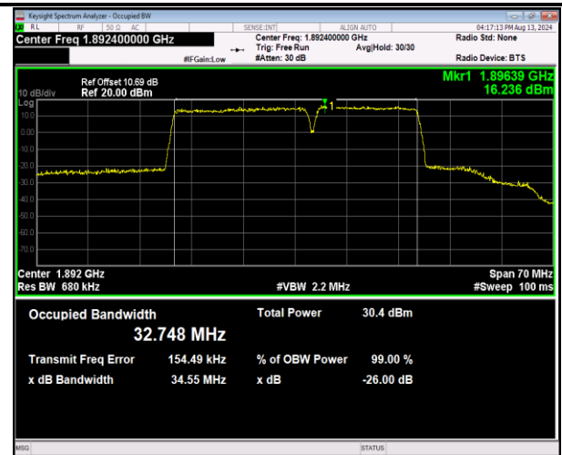
2-2-20MHz-15MHz-16QAM-16QAM-18951-19122-100RB#0-75RB#0-PASS
