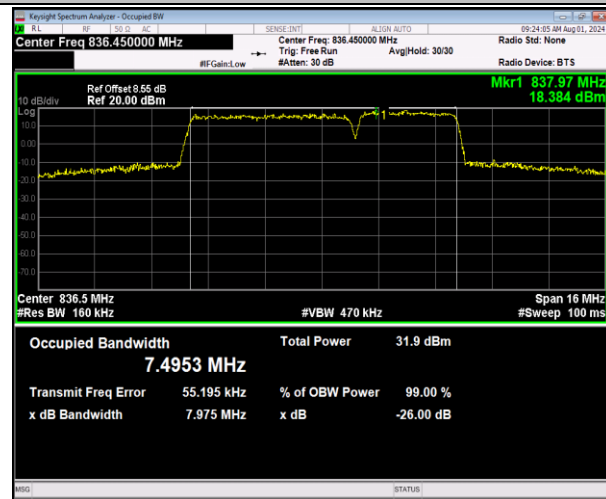
5-5-5MHz-3MHz-64QAM-64QAM-20510-20549-25RB#0-15RB#0-PASS
