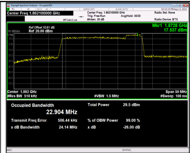
2-2-20MHz-5MHz-16QAM-16QAM-18700-18817-100RB #0-25RB#0-PASS
