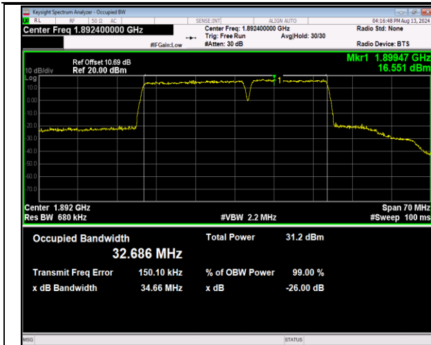
2-2-20MHz-15MHz-QPSK-QPSK-18951-19122-100RB#0-75RB#0-PASS
