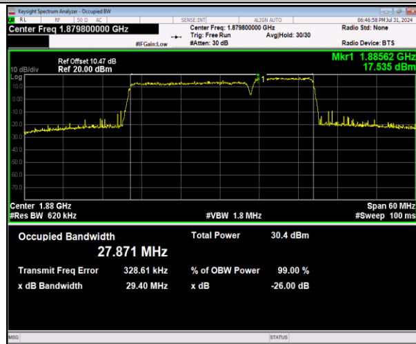
2-2-20MHz-10MHz-64QAM-64QAM-18851-18995-100RB#0-50RB#0-PASS
