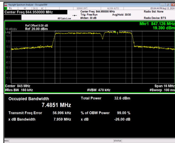
5-5-5MHz-3MHz-16QAM-16QAM-20595-20634-25RB#0-15RB#0-PASS
