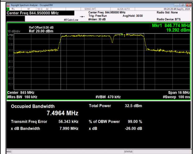
5-5-5MHz-3MHz-64QAM-64QAM-20595-20634-25RB#0-15RB#0-PASS
