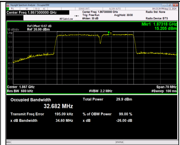
2-2-20MHz-15MHz-16QAM-16QAM-18700-18871-100RB#0-75RB#0-PASS
