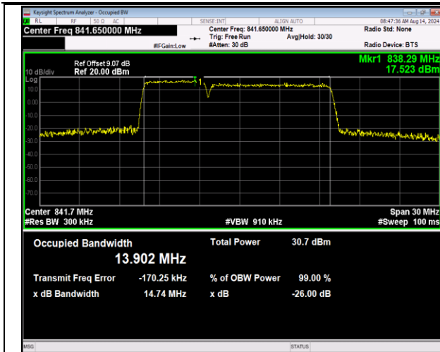
5-5-5MHz-10MHz-QPSK-QPSK-20528-20600-25RB#0-50 RB#0-PASS
