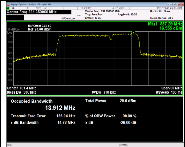
5-5-10MHz-5MHz-64QAM-64QAM-20450-20522-50RB# 0-25RB#0-PASS
