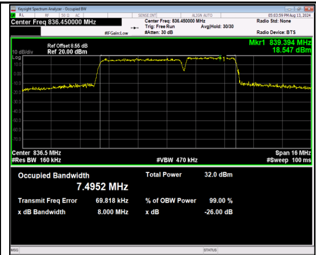
5-5-5MHz-3MHz-16QAM-16QAM-20510-20549-25RB#0-15RB#0-PASS
