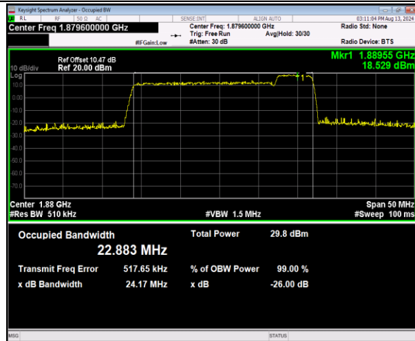
2-2-20MHz-5MHz-16QAM-16QAM-18875-18992-100RB# 0-25RB#0-PASS
