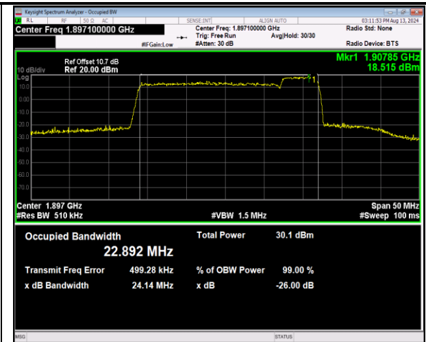
2-2-20MHz-5MHz-16QAM-16QAM-19050-19167-100RB #0-25RB#0-PASS
