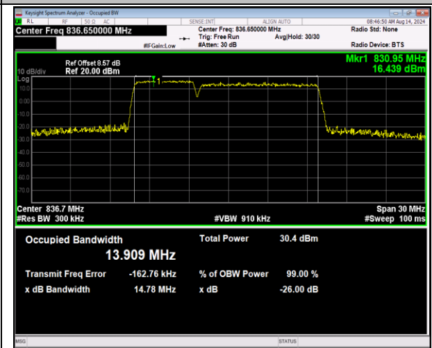
5-5-5MHz-10MHz-QPSK-QPSK-20478-20550-25RB#0-5 0RB#0-PASS
