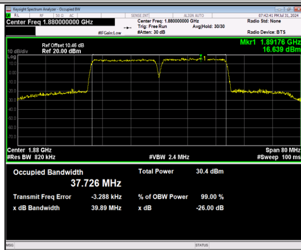
2-2-20MHz-20MHz-64QAM-64QAM-18801-18999-100RB#0-100RB#0-PASS
