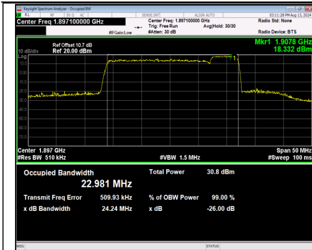
2-2-20MHz-5MHz-QPSK-QPSK-19050-19167-100RB#0-2 5RB#0-PASS
