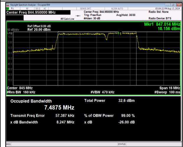
5-5-5MHz-3MHz-QPSK-QPSK-20595-20634-25RB#0-15RB#0-PASS
