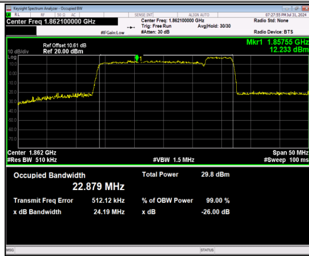
2-2-20MHz-5MHz-64QAM-64QAM-18700-18817-100RB# 0-25RB#0-PASS
