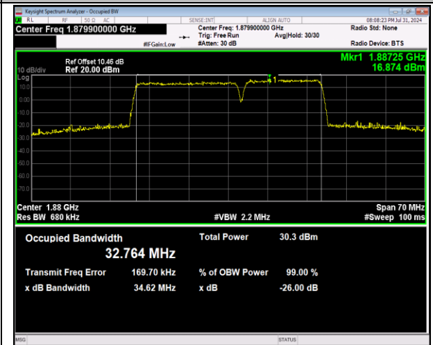
2-2-20MHz-15MHz-64QAM-64QAM-18826-18997-100RB#0-75RB#0-PASS
