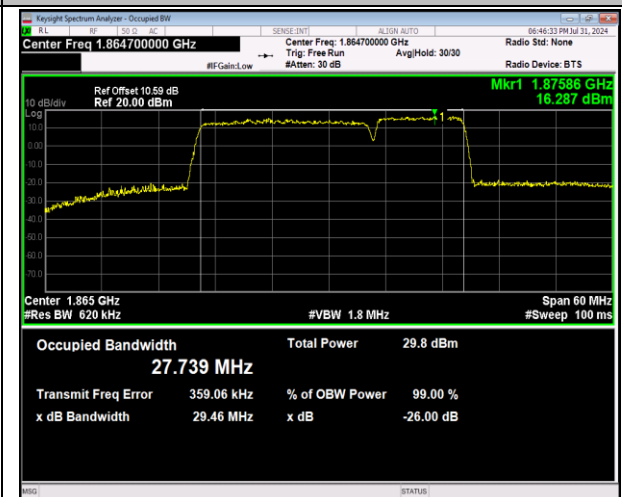
2-2-20MHz-10MHz-64QAM-64QAM-18700-18844-100R B#0-50RB#0-PASS
