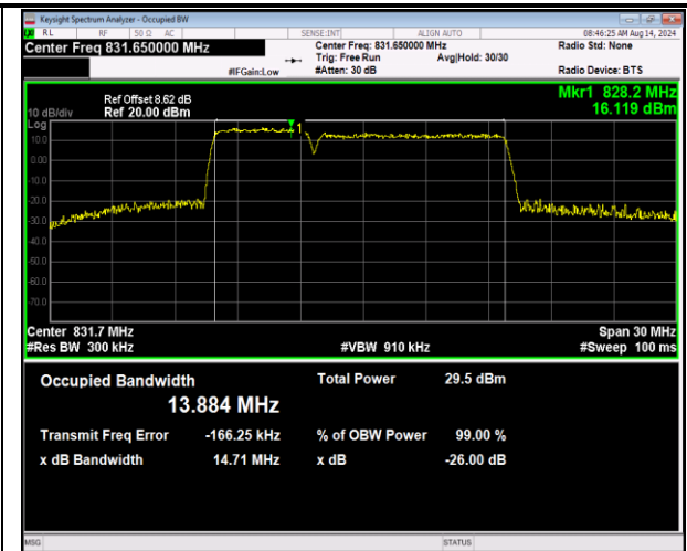
5-5-5MHz-10MHz-16QAM-16QAM-20428-20500-25RB# 0-50RB#0-PASS
