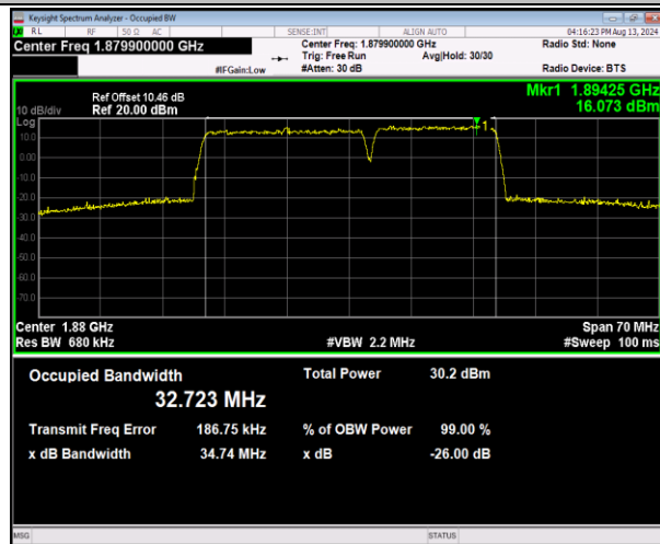
2-2-20MHz-15MHz-16QAM-16QAM-18826-18997-100RB#0-75RB#0-PASS
