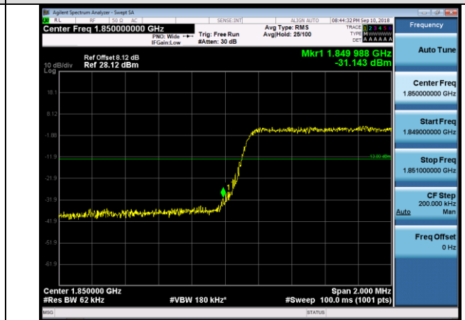
LCH_16QAM_15RB#0
