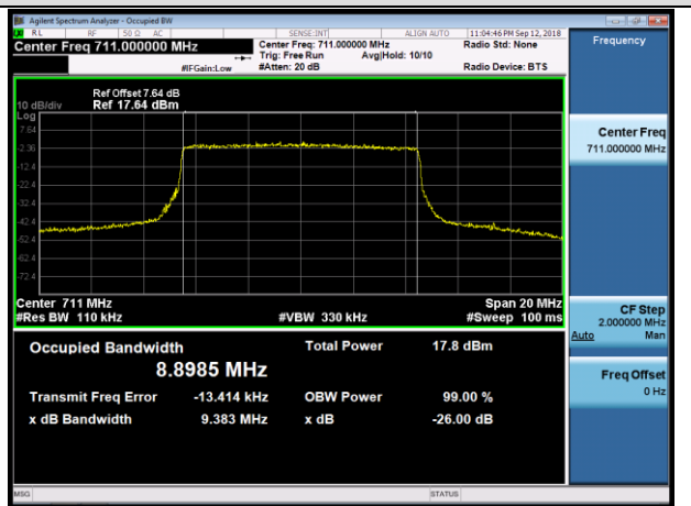
HCH_16QAM_50RB#0
