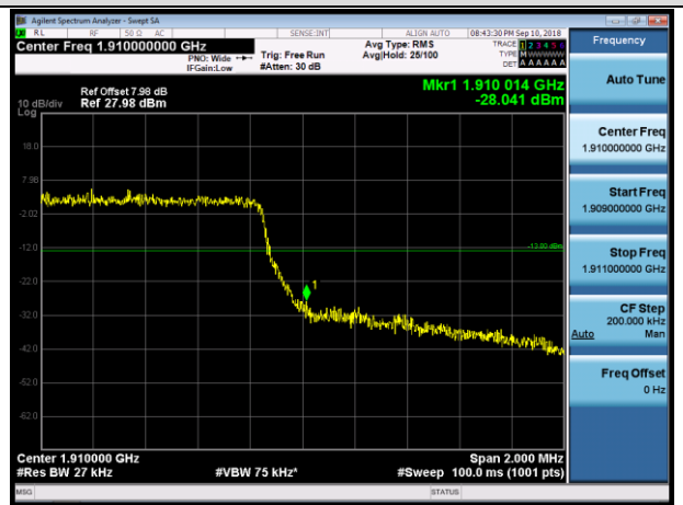
HCH_16QAM_6RB#0
