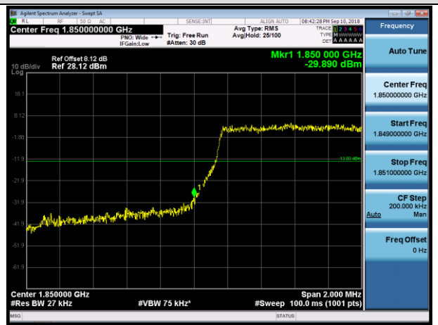
LCH_16QAM_6RB#0
