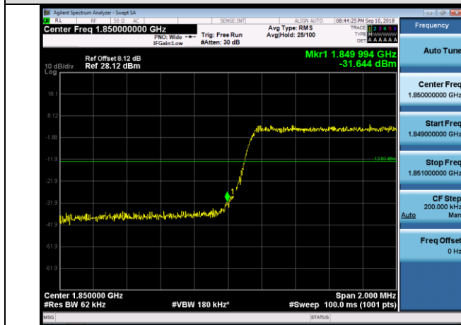
LCH_QPSK_15RB#0
