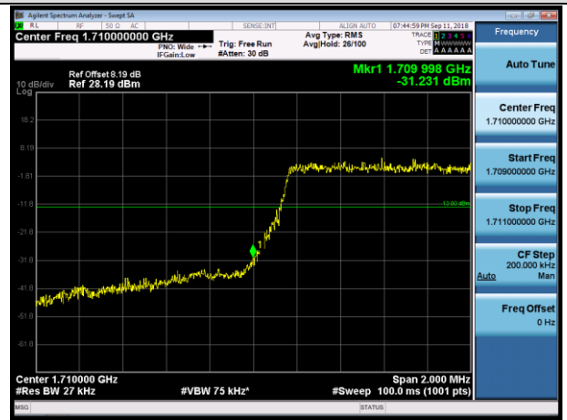
LCH_16QAM_6RB#0
