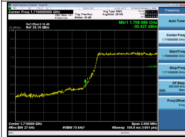
LCH_QPSK_6RB#0
