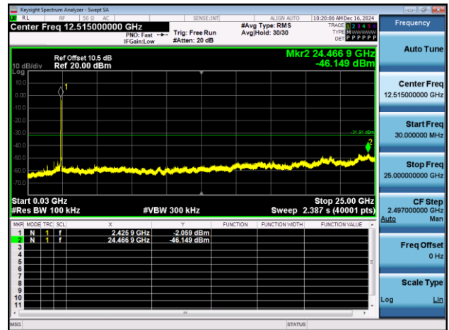
11AX40SISO-Ant1-2437-30~25000-PASS
