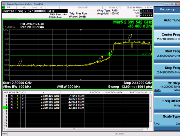
11AX20SISO-Ant1-2412-PASS
