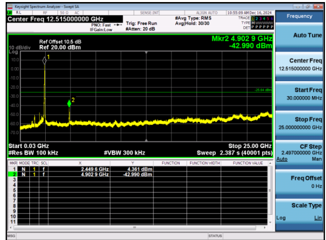
11AX40SISO-Ant1-2452-30~25000-PASS
