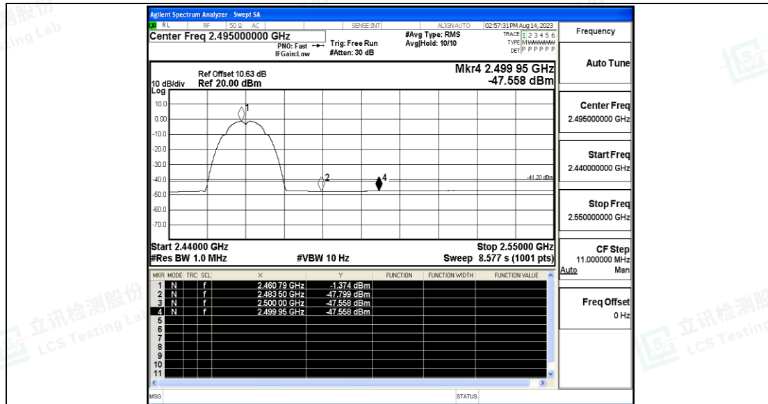
11B_Ant1_High_2462_Peak
