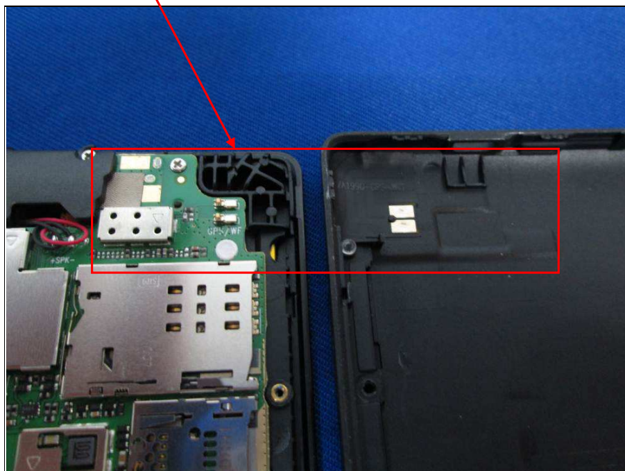
BT/WLAN Diversity Antenna
