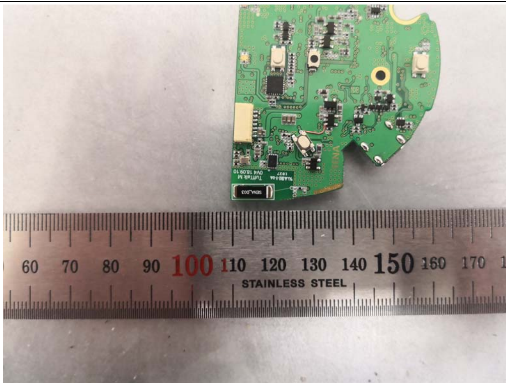
Zigbee Antenna
