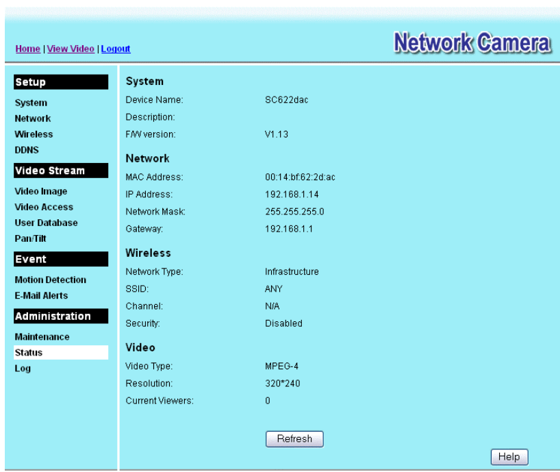
Figure 39: Status Screen
