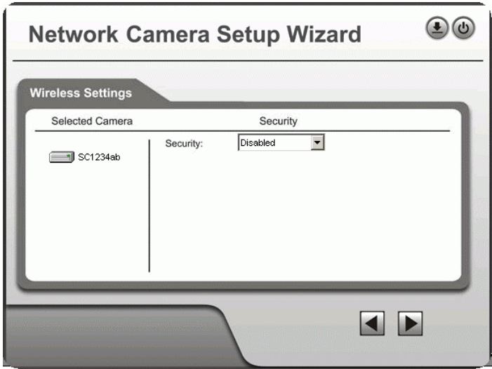
Figure 8: Security Screen
