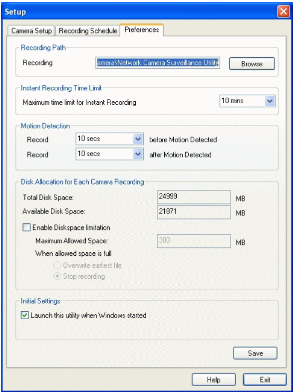
Figure 47: Preferences Screen
