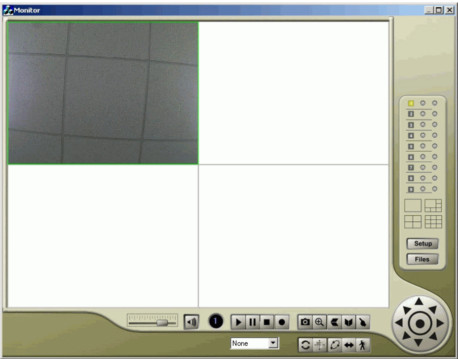
Figure 43: Main Screen
