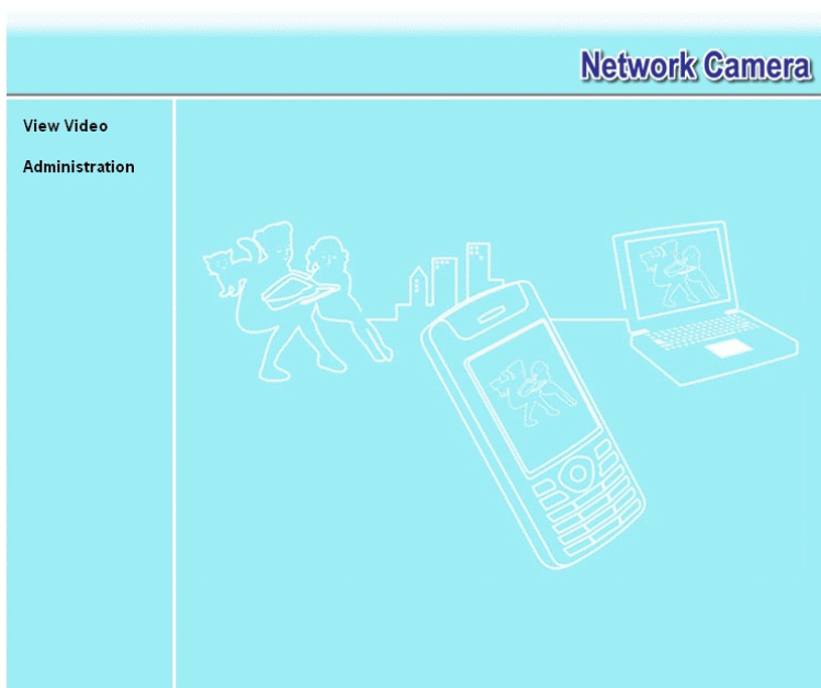
Figure 14: Home Screen
