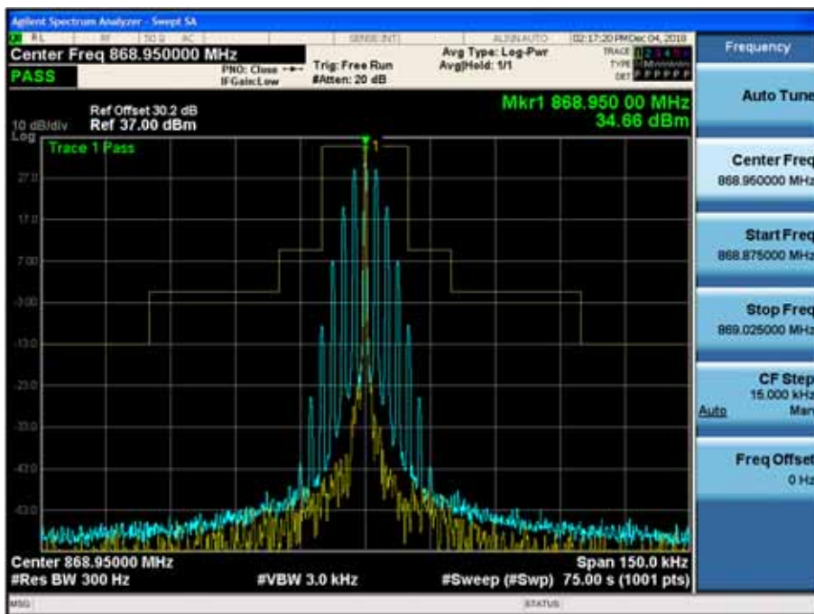
(14K0F3E _ 868.95 MHz)_High
