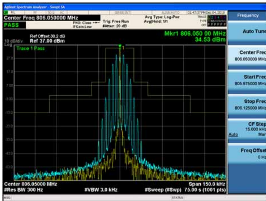
(16K0F3E _ 806.05 MHz)_High
