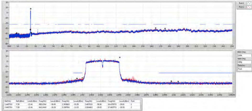
VHT40-BF_Nss1,(MCS0)_2TX 2422MHz
