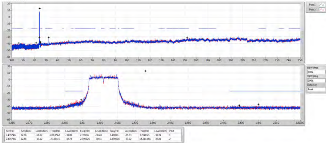
802.11g-BF_Nss1,(6Mbps)_2TX 2412MHz
