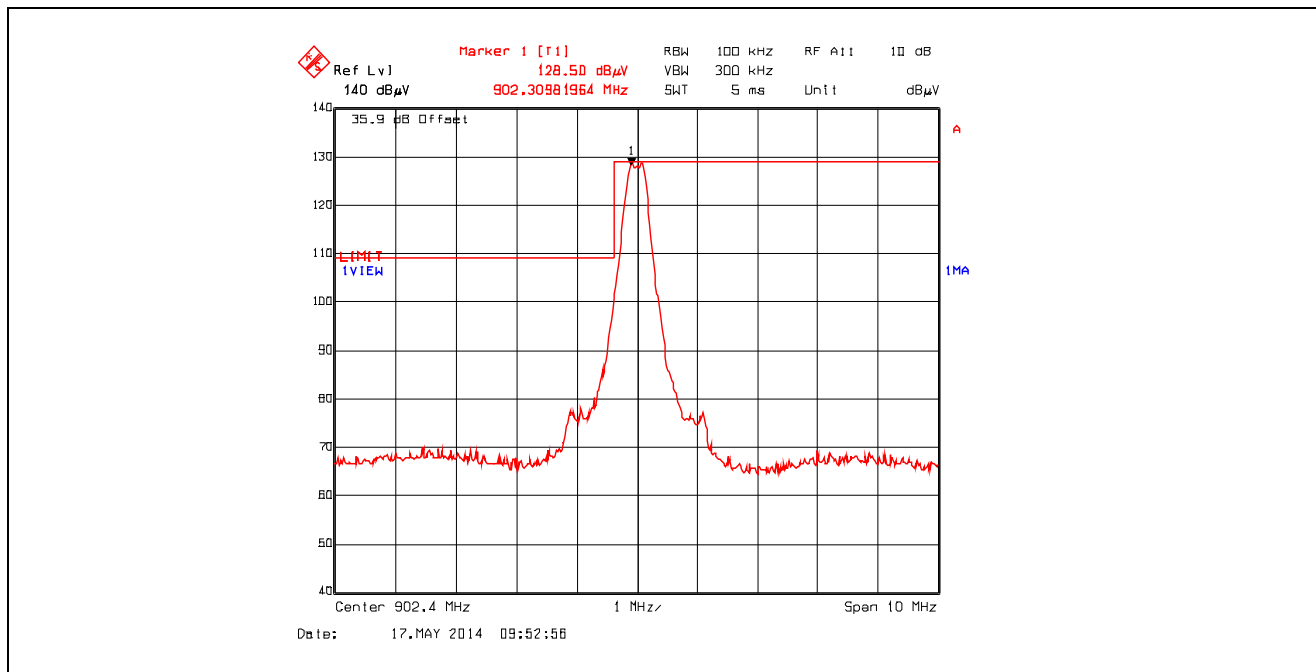
Plot 5.6.4.1.2.1. Band-Edge RF Radiated Emissions at 3 m, Horizontal Polarization Single Frequency Mode, Low End of Frequency Band, Power Setting 45, Data Rate at 345600 kbps
