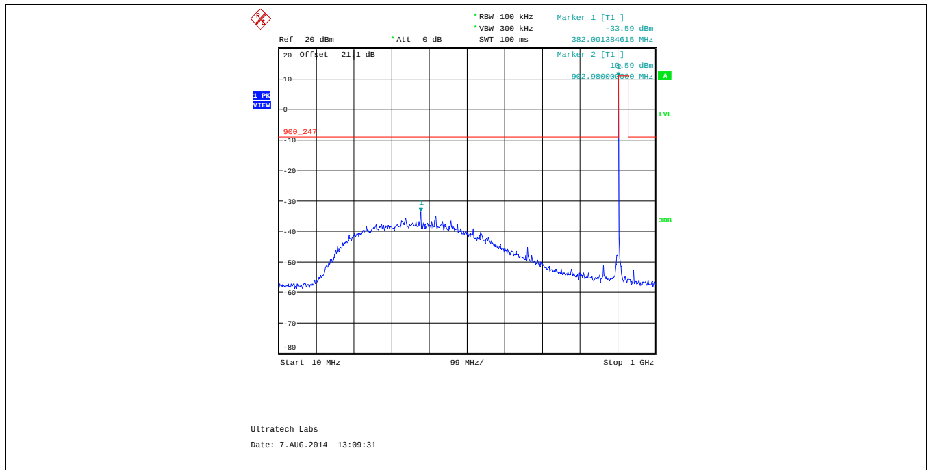
Plot 5.5.4.2.19. Conducted Spurious Emissions Low Power, 902.4 MHz, Data Rate at 24686 kbps, 10 MHz – 1 GHz
