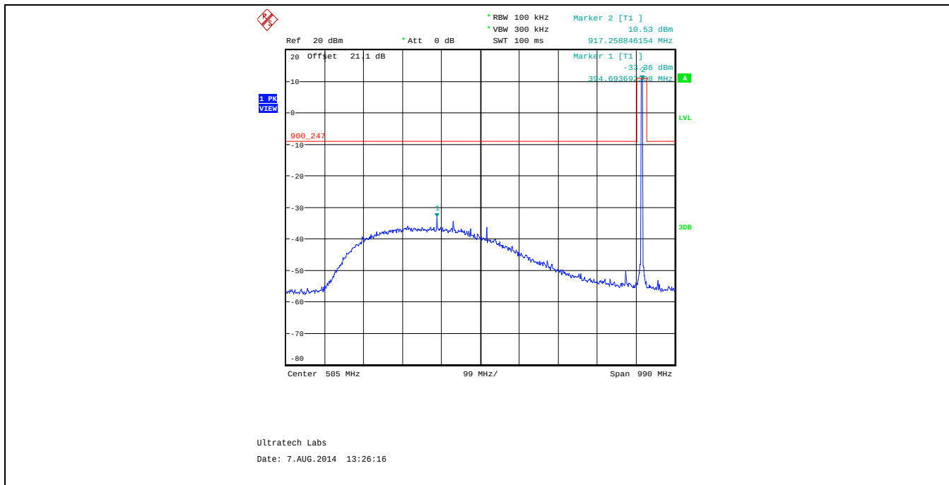
Plot 5.5.4.2.27. Conducted Spurious Emissions Low Power, 915.0 MHz, Data Rate at 230400 kbps, 10 MHz – 1 GHz
