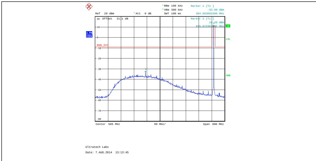
Plot 5.5.4.2.21. Conducted Spurious Emissions Low Power, 915.0 MHz, Data Rate at 24686 kbps, 10 MHz – 1 GHz
