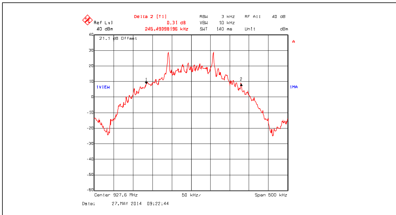
Plot 5.3.4.18. 20 dB Bandwidth, 927.6 MHz, 400 kHz Channel Spacing, Data Rate at 276480 kbps
