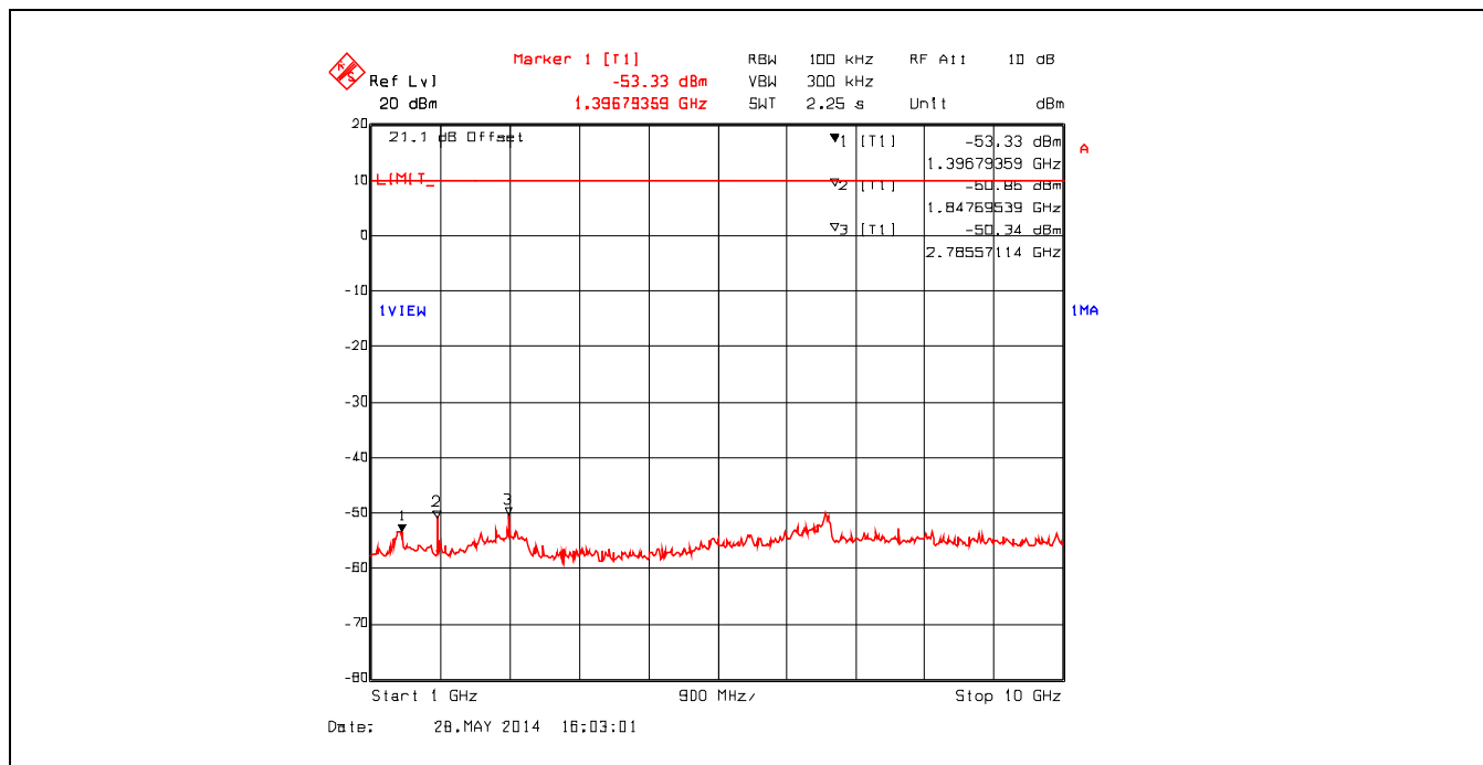
Plot 5.5.4.2.12. Conducted Spurious Emissions High Power, 927.6 MHz, Data Rate at 230400 kbps, 1 GHz – 10 GHz
