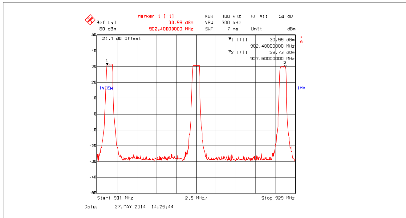
Plot 5.3.4.29. Number of Hopping Frequencies, 50 kHz Channel Spacing, Data Rate at 19200 kbps 50 Hopping Channels from 901 – 929 MHz
