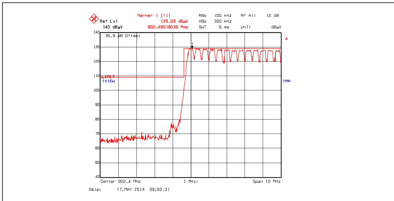
Plot 5.6.4.1.2.2. Band-Edge RF Radiated Emissions at 3 m, Horizontal Polarization Pseudorandom Channel Hopping Mode, Low End of Frequency Band, Power Setting 45, Data Rate at 345600 kbps
