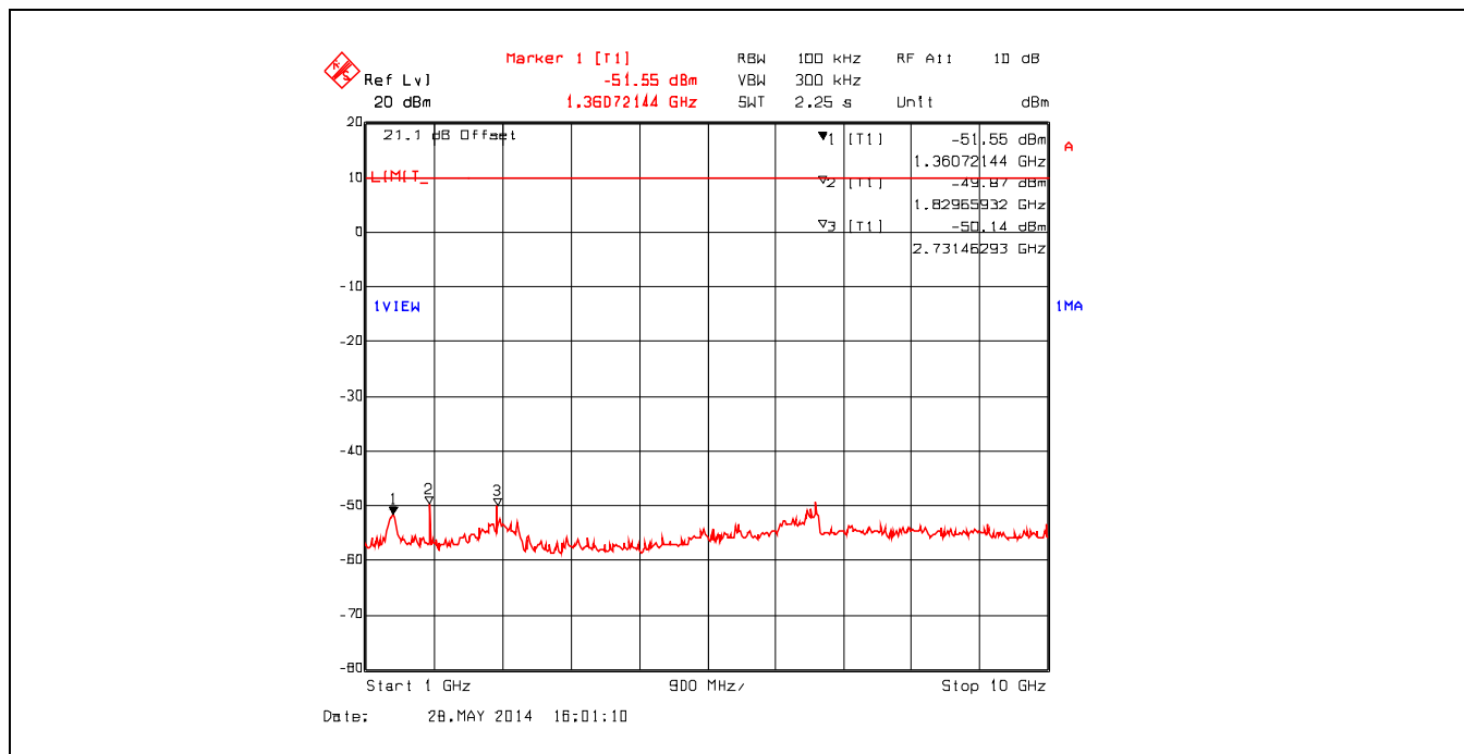
Plot 5.5.4.2.10. Conducted Spurious Emissions High Power, 915.0 MHz, Data Rate at 230400 kbps, 1 GHz – 10 GHz
