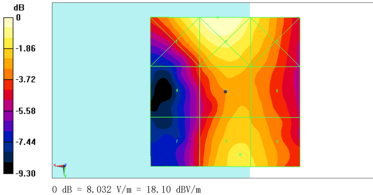
Fig B.3 HAC RF E-Field LTE Band41 QPSK CH40620
