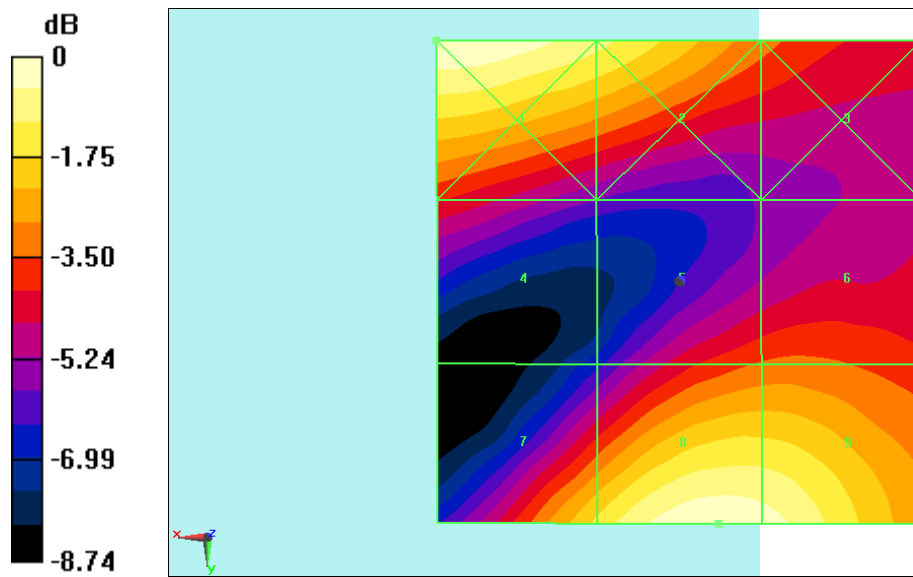
Fig B.2 HAC RF E-Field GSM 1900 Middle
