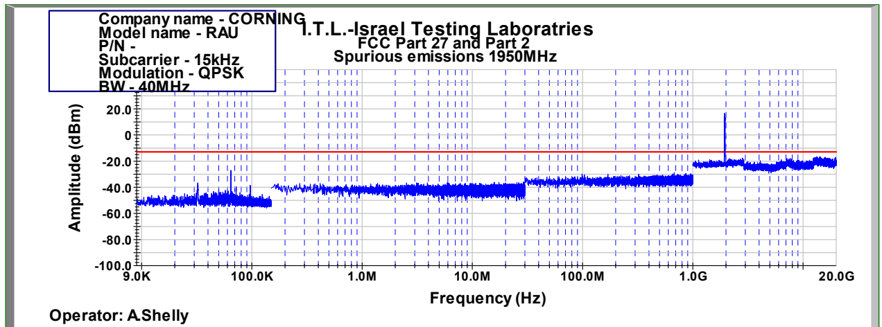
Figure 1041: Spurious Emissions at Antenna Terminal QPSK 40MHz B.W.; 1950.0MHz, 15kHz
