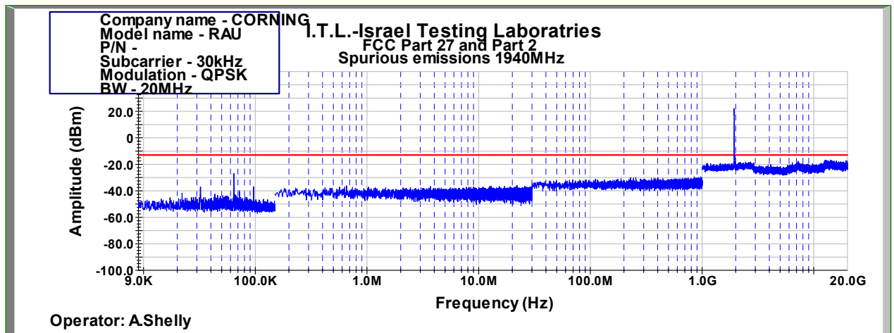
Figure 1026: Spurious Emissions at Antenna Terminal QPSK 20MHz B.W.; 1940.0MHz, 30kHz
