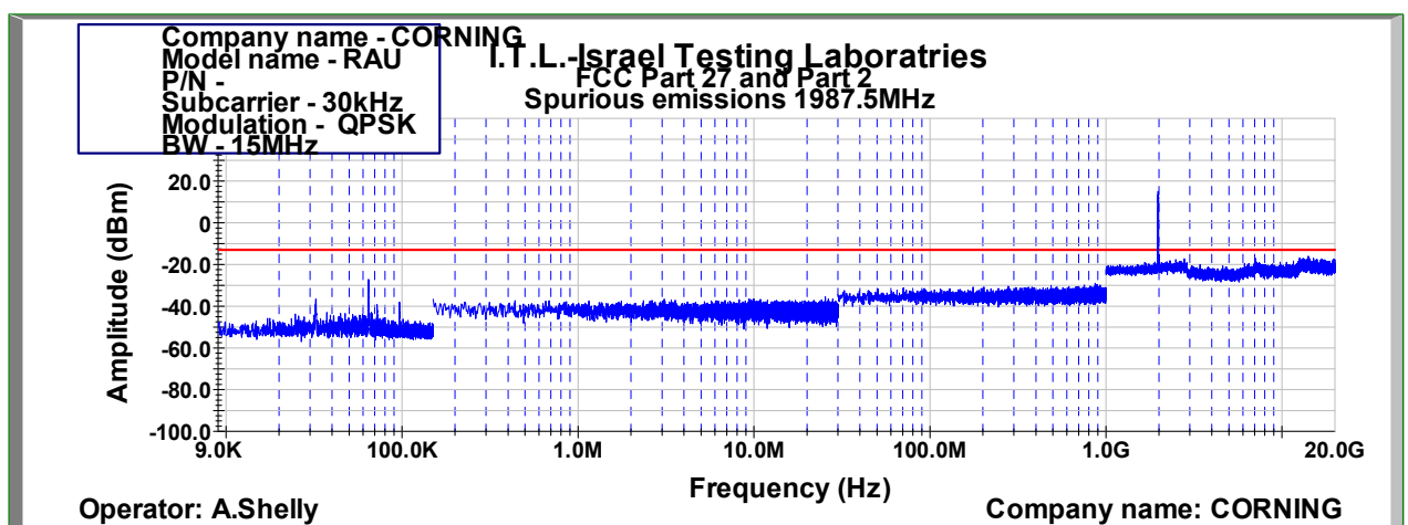
Figure 1019: Spurious Emissions at Antenna Terminal QPSK 15MHz B.W.; 1987.5MHz, 30kHz
