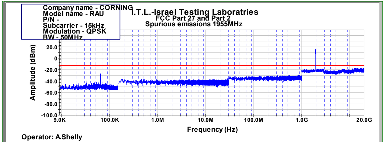
Figure 1050: Spurious Emissions at Antenna Terminal QPSK 50MHz B.W.; 1955.0MHz, 15kHz
