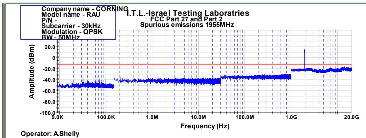
Figure 1053: Spurious Emissions at Antenna Terminal QPSK 50MHz B.W.; 1955.0MHz, 30kHz
