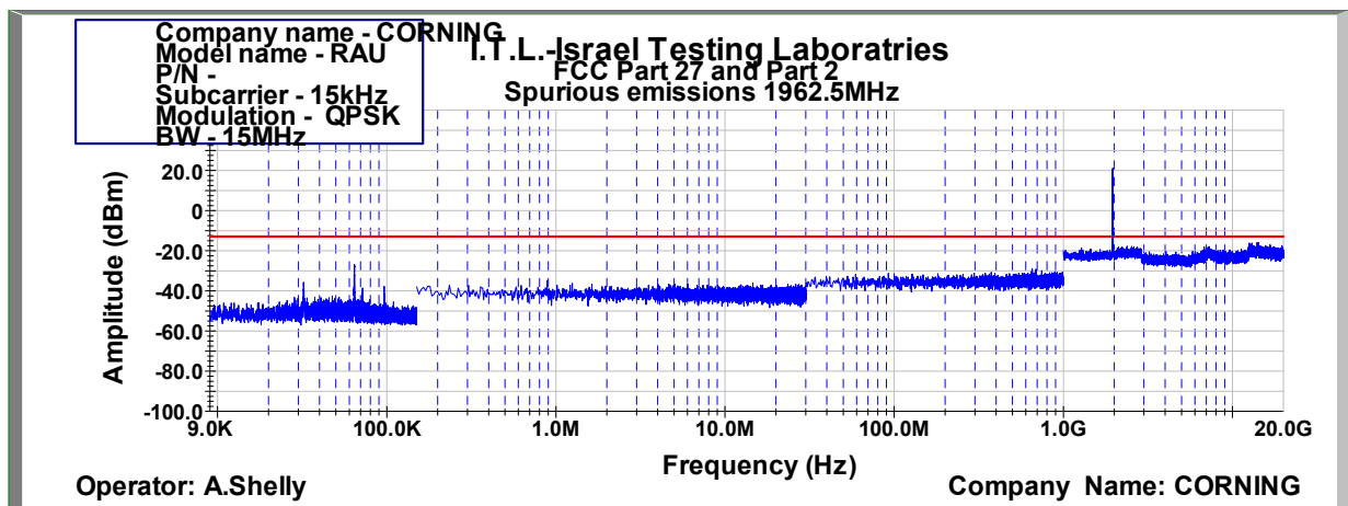
Figure 1015: Spurious Emissions at Antenna Terminal QPSK 15MHz B.W.; 1962.5MHz, 15kHz
