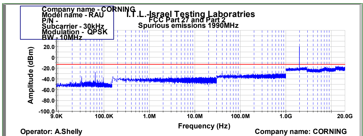
Figure 1010: Spurious Emissions at Antenna Terminal QPSK 10MHz B.W.; 1990.0MHz, 30kHz
