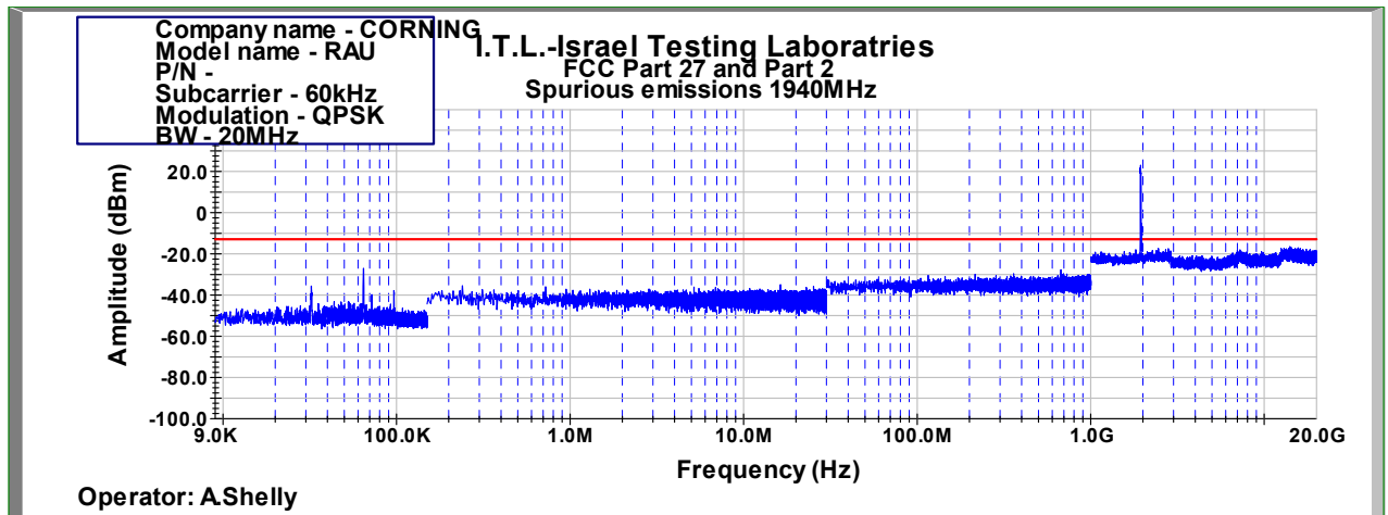
Figure 1029: Spurious Emissions at Antenna Terminal QPSK 20MHz B.W.; 1940.0MHz, 60kHz
