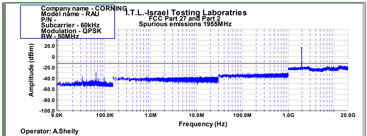
Figure 1056: Spurious Emissions at Antenna Terminal QPSK 50MHz B.W.; 1955.0MHz, 60kHz
