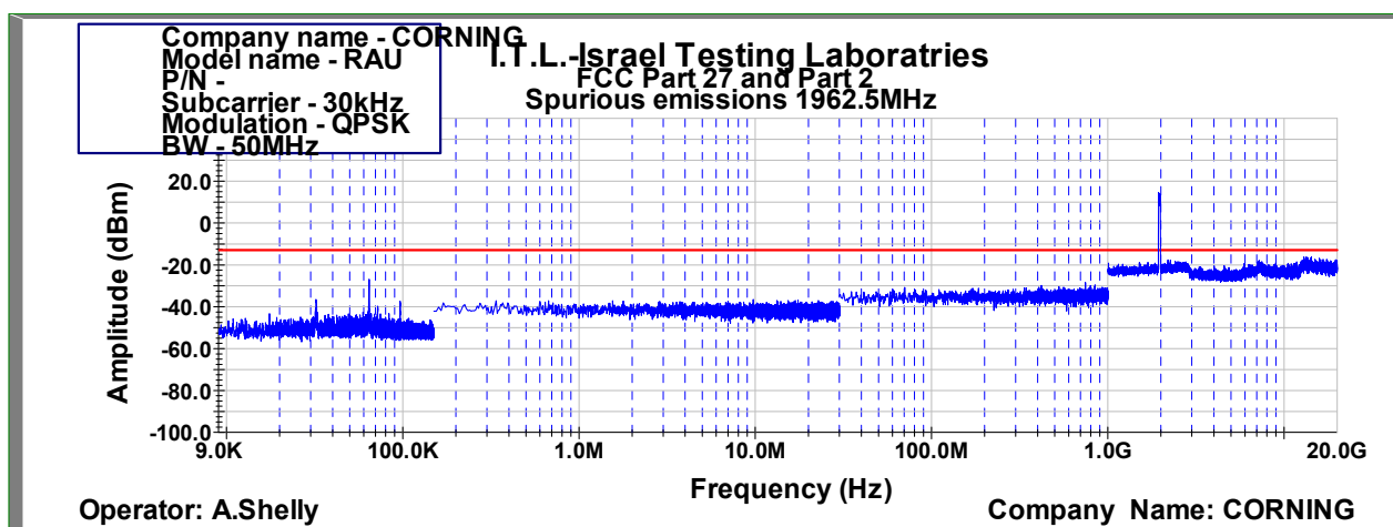
Figure 1054: Spurious Emissions at Antenna Terminal QPSK 50MHz B.W.; 1962.5MHz, 30kHz
