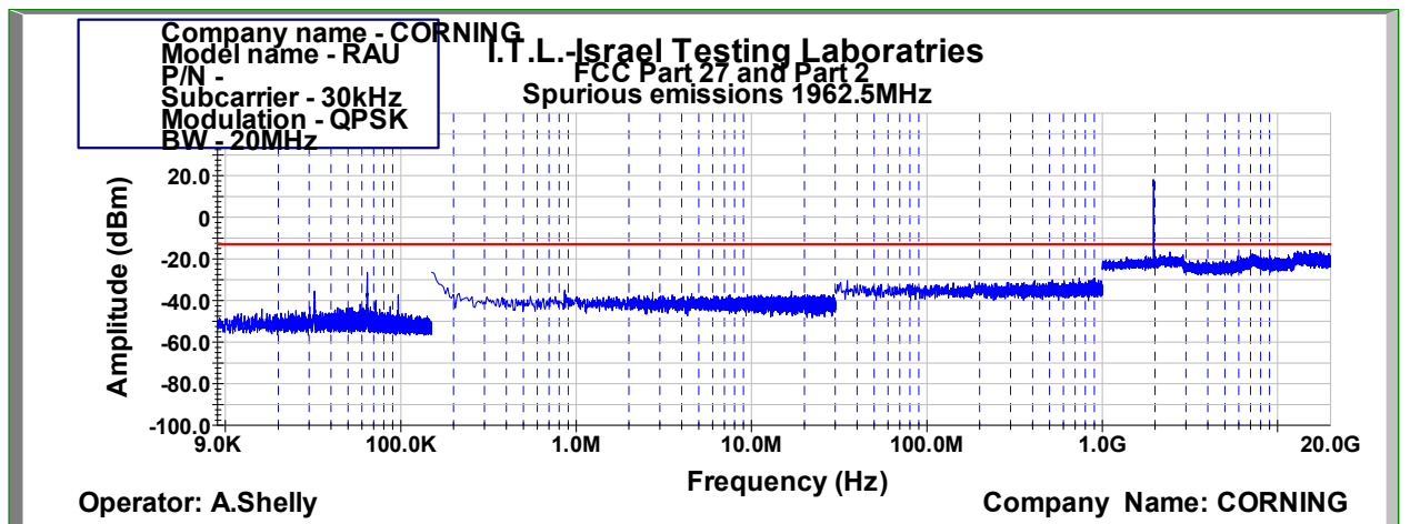
Figure 1027: Spurious Emissions at Antenna Terminal QPSK 20MHz B.W.; 1962.5MHz, 30kHz
