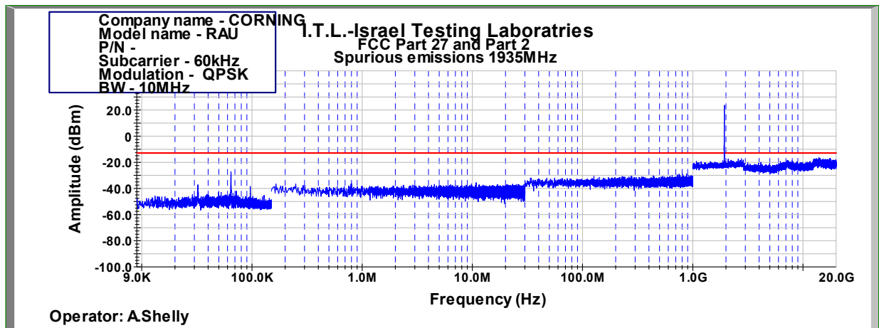
Figure 1011: Spurious Emissions at Antenna Terminal QPSK 10MHz B.W.; 1935.0MHz, 60kHz
