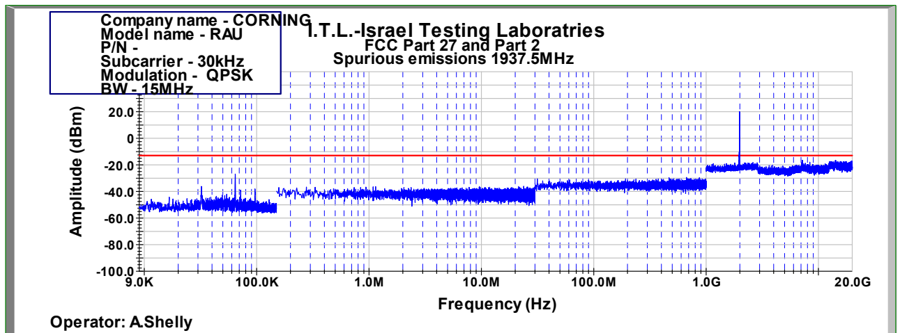
Figure 1017: Spurious Emissions at Antenna Terminal QPSK 15MHz B.W.; 1937.5MHz, 30kHz
