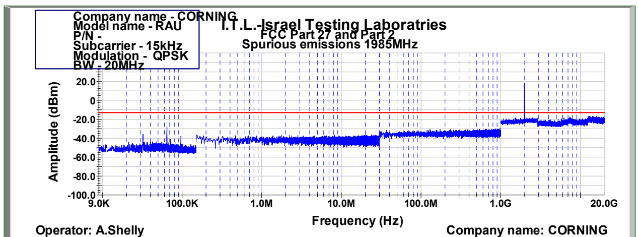
Figure 1025: Spurious Emissions at Antenna Terminal QPSK 20MHz B.W.; 1985.0MHz, 15kHz
