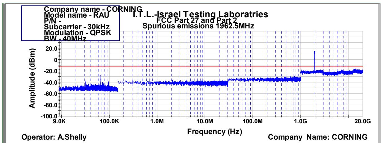
Figure 1045: Spurious Emissions at Antenna Terminal QPSK 40MHz B.W.; 1962.5MHz, 30kHz
