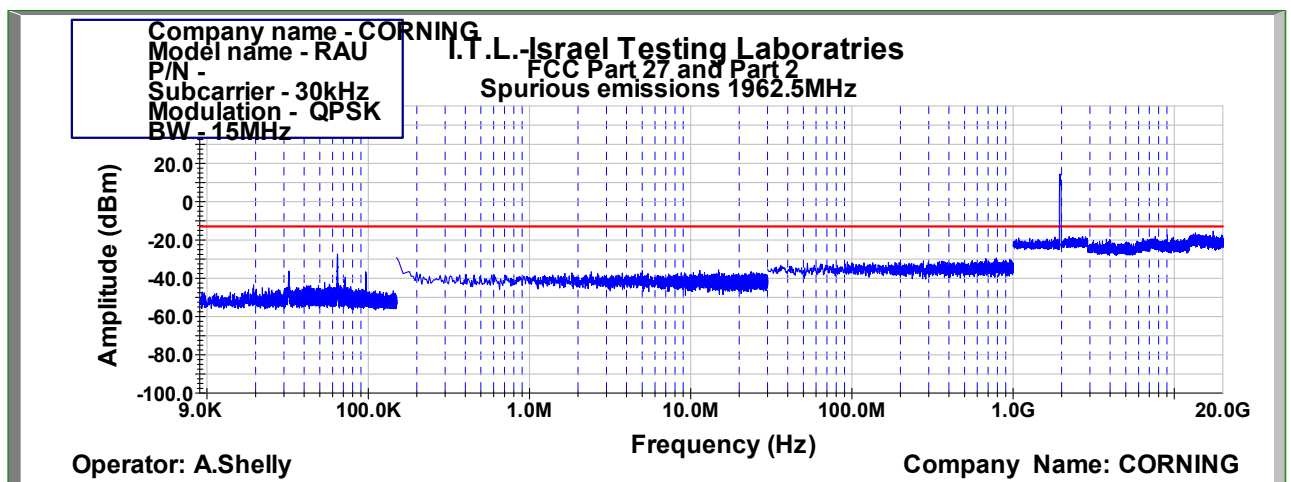
Figure 1018: Spurious Emissions at Antenna Terminal QPSK 15MHz B.W.; 1962.5MHz, 30kHz
