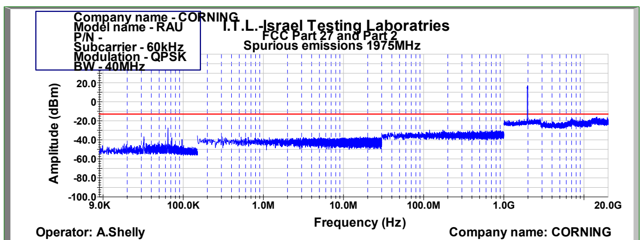
Figure 1049: Spurious Emissions at Antenna Terminal QPSK 40MHz B.W.; 1975.0MHz, 60kHz
