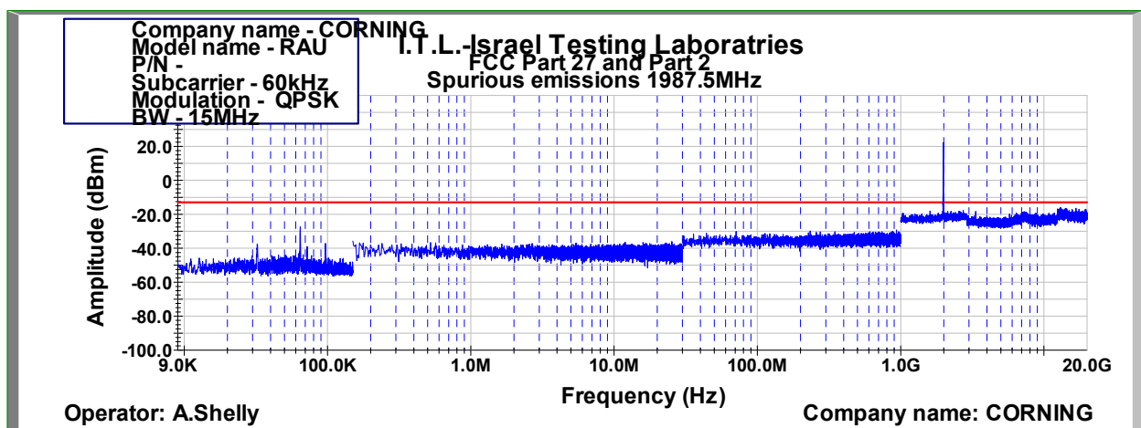
Figure 1022: Spurious Emissions at Antenna Terminal QPSK 15MHz B.W.; 1987.5MHz, 60kHz
