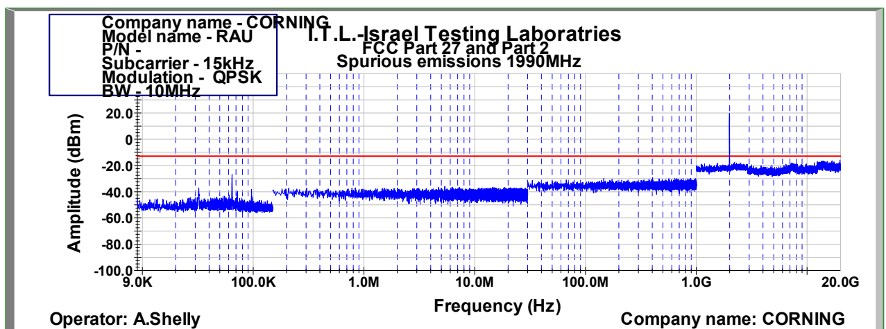
Figure 1007: Spurious Emissions at Antenna Terminal QPSK 10MHz B.W.; 1990.0MHz, 15kHz
