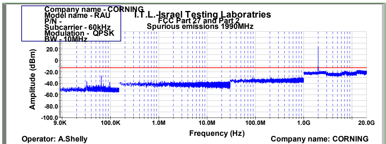
Figure 1013: Spurious Emissions at Antenna Terminal QPSK 10MHz B.W.; 1990.0MHz, 60kHz
