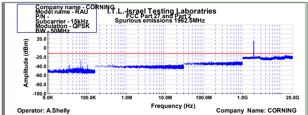
Figure 1051: Spurious Emissions at Antenna Terminal QPSK 50MHz B.W.; 1962.5MHz, 15kHz
