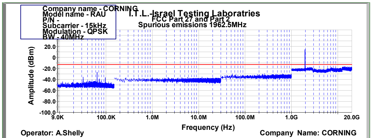
Figure 1042: Spurious Emissions at Antenna Terminal QPSK 40MHz B.W.; 1962.5MHz, 15kHz
