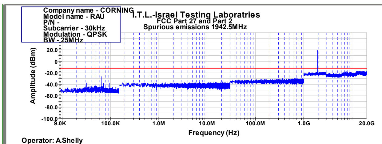
Figure 1035: Spurious Emissions at Antenna Terminal QPSK 25MHz B.W.; 1942.5MHz, 30kHz
