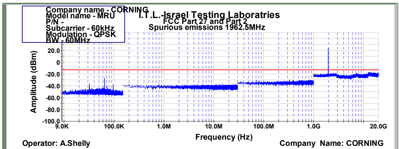
Figure 1063: Spurious Emissions at Antenna Terminal QPSK 60MHz B.W.; 1962.5MHz, 60kHz
