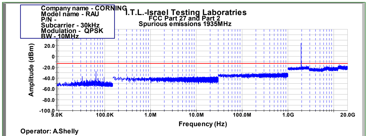
Figure 1008: Spurious Emissions at Antenna Terminal QPSK 10MHz B.W.; 1935.0MHz, 30kHz
