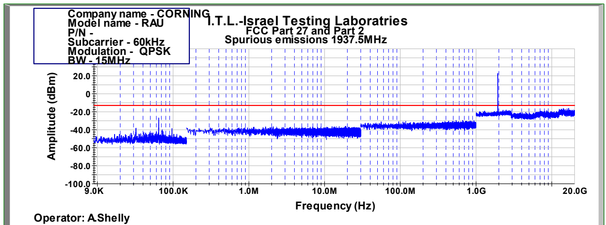
Figure 1020: Spurious Emissions at Antenna Terminal QPSK 15MHz B.W.; 1937.5MHz, 60kHz
