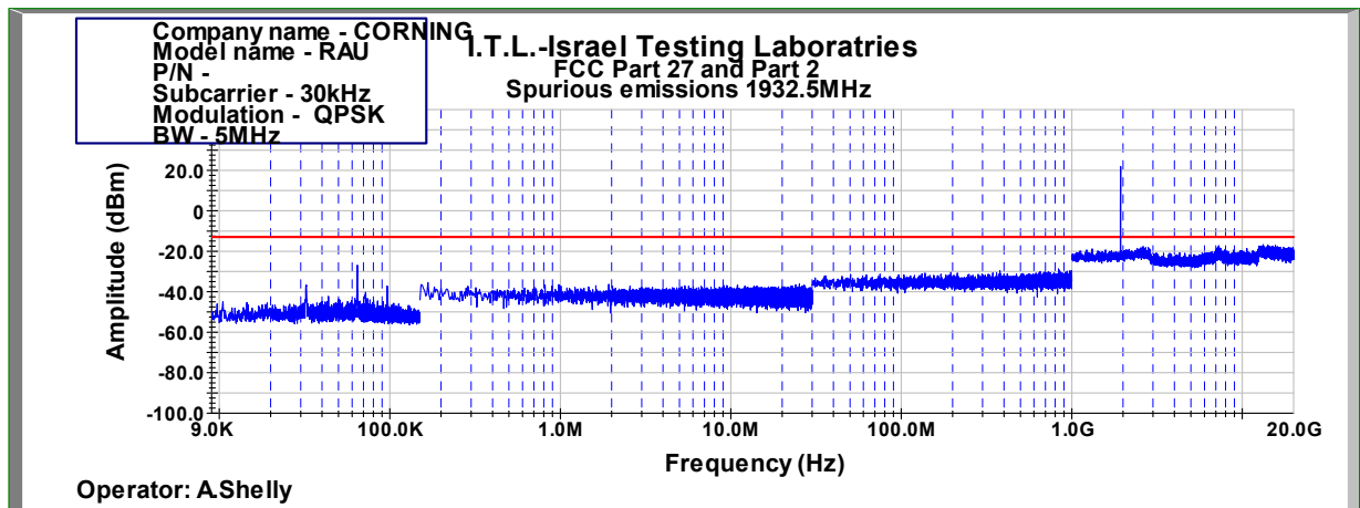
Figure 1002: Spurious Emissions at Antenna Terminal QPSK 5MHz B.W.; 1932.5MHz, 30kHz
