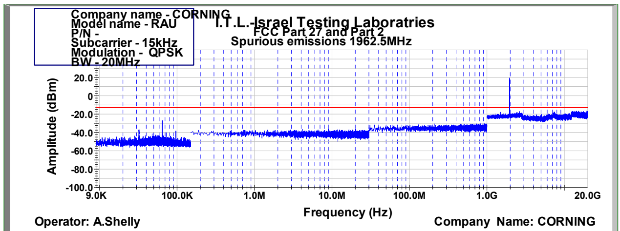
Figure 1024: Spurious Emissions at Antenna Terminal QPSK 20MHz B.W.; 1962.5MHz, 15kHz
