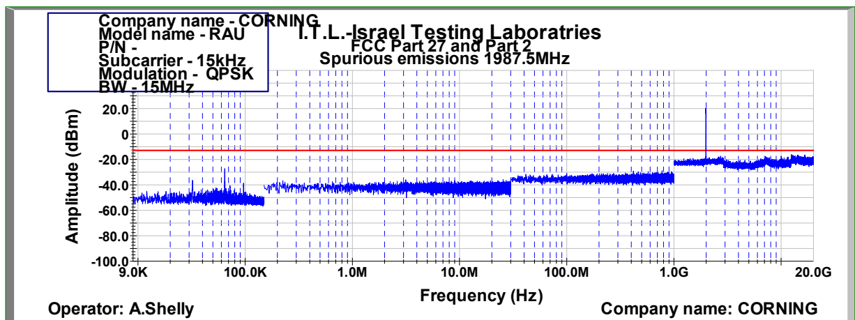
Figure 1016: Spurious Emissions at Antenna Terminal QPSK 15MHz B.W.; 1987.5MHz, 15kHz
