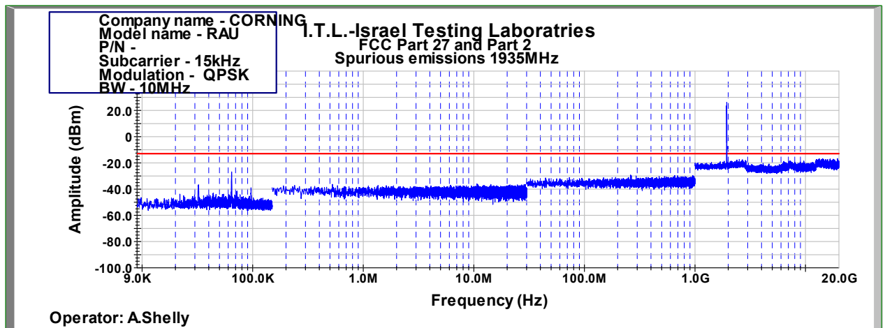
Figure 1005: Spurious Emissions at Antenna Terminal QPSK 10MHz B.W.; 1935.00MHz, 15kHz
