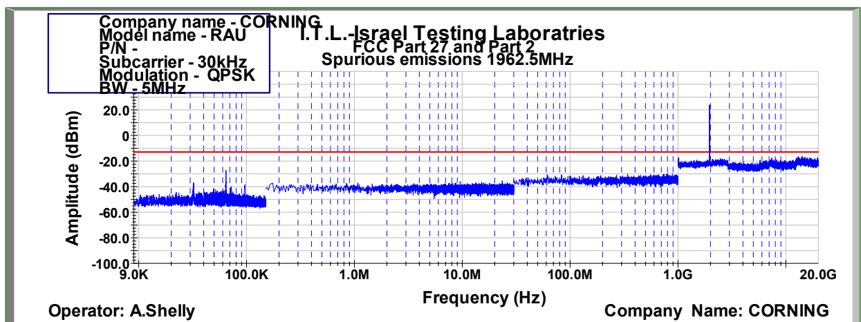
Figure 1003: Spurious Emissions at Antenna Terminal QPSK 5MHz B.W.; 1962.5MHz, 30kHz
