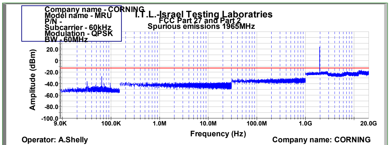
Figure 1064: Spurious Emissions at Antenna Terminal QPSK 60MHz B.W.; 1965.0MHz, 60kHz
