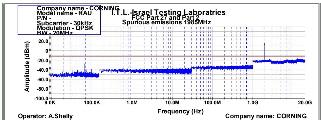
Figure 1028: Spurious Emissions at Antenna Terminal QPSK 20MHz B.W.; 1985.0MHz, 30kHz
