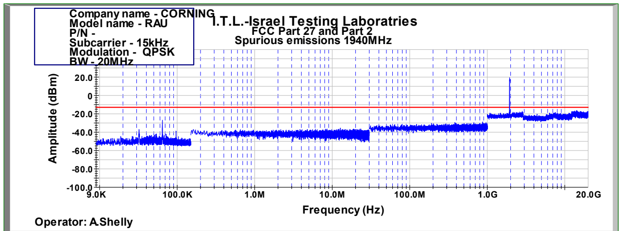
Figure 1023: Spurious Emissions at Antenna Terminal QPSK 20MHz B.W.; 1940.0MHz, 15kHz
