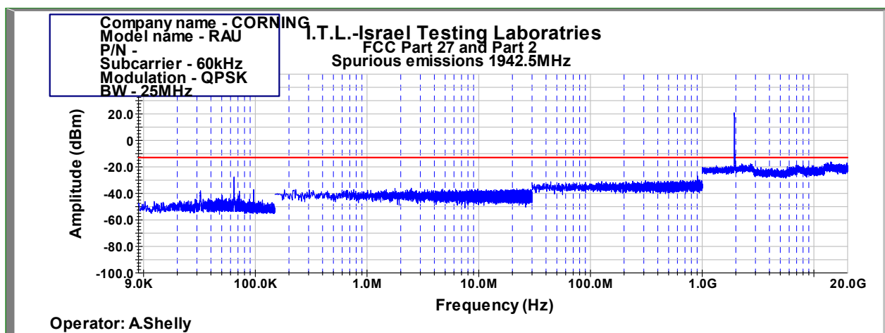
Figure 1038: Spurious Emissions at Antenna Terminal QPSK 25MHz B.W.; 1942.5MHz, 60kHz
