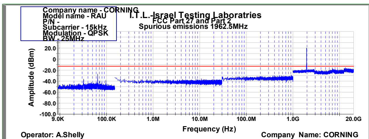
Figure 1033: Spurious Emissions at Antenna Terminal QPSK 25MHz B.W.; 1962.5MHz, 15kHz
