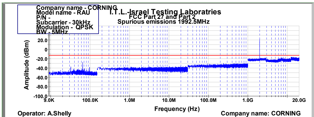
Figure 1004: Spurious Emissions at Antenna Terminal QPSK 5MHz B.W.; 1992.5MHz, 30kHz
