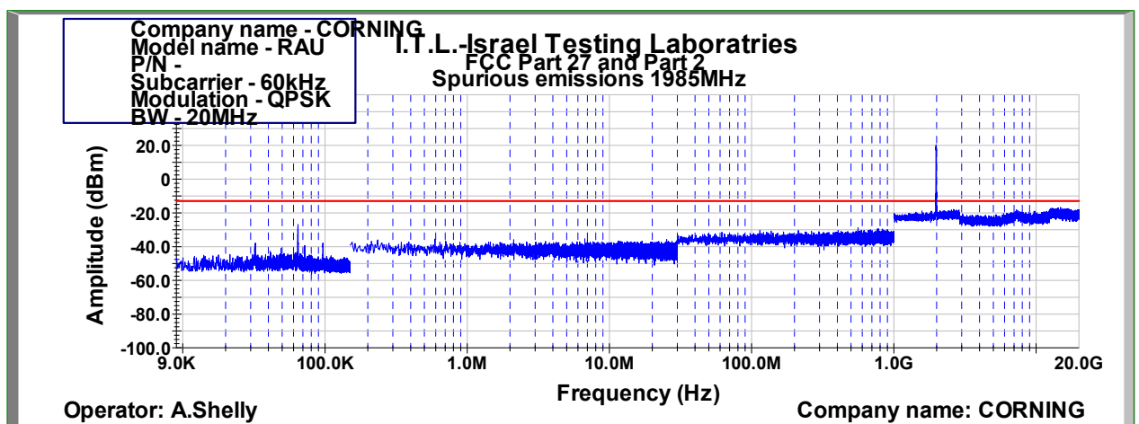
Figure 1031: Spurious Emissions at Antenna Terminal QPSK 20MHz B.W.; 1985.0MHz, 60kHz
