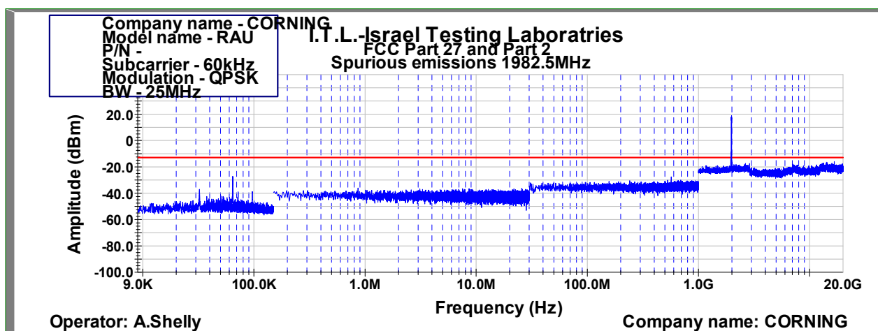
Figure 1040: Spurious Emissions at Antenna Terminal QPSK 25MHz B.W.; 1982.5MHz, 60kHz
