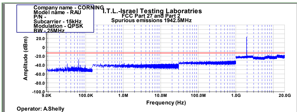
Figure 1032: Spurious Emissions at Antenna Terminal QPSK 25MHz B.W.; 1942.5MHz, 15kHz
