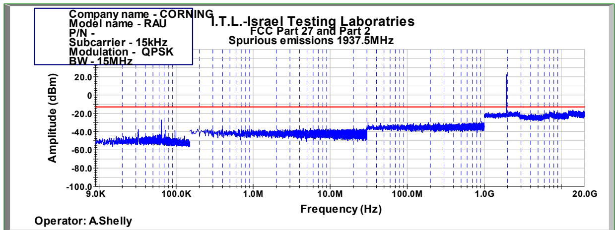
Figure 1014: Spurious Emissions at Antenna Terminal QPSK 15MHz B.W.; 1937.5MHz, 15kHz
