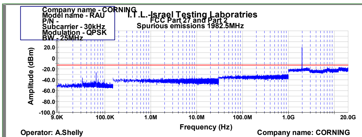
Figure 1037: Spurious Emissions at Antenna Terminal QPSK 25MHz B.W.; 1982.5MHz, 30kHz
