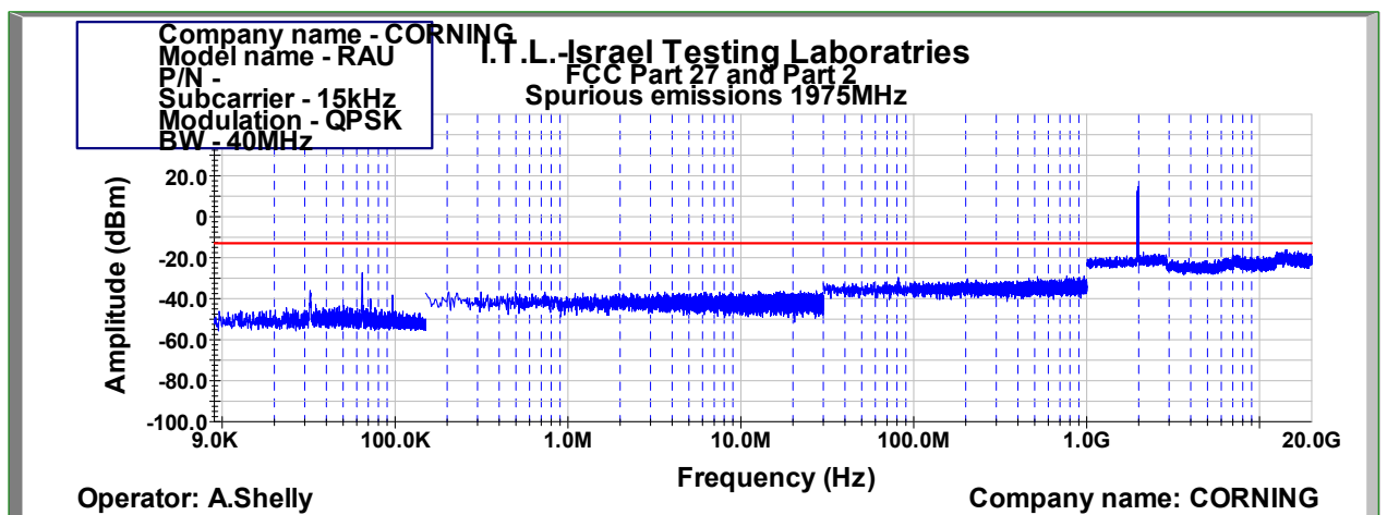
Figure 1043: Spurious Emissions at Antenna Terminal QPSK 40MHz B.W.; 1975.0MHz, 15kHz
