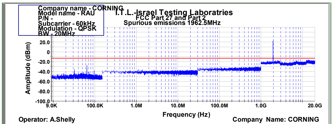
Figure 1030: Spurious Emissions at Antenna Terminal QPSK 20MHz B.W.; 1962.5MHz, 60kHz
