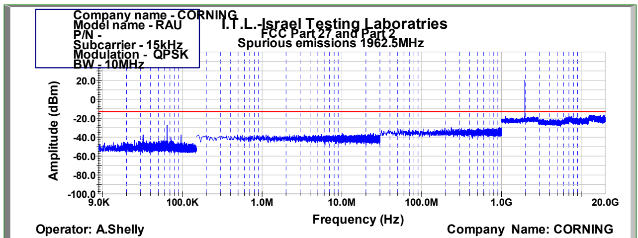
Figure 1006: Spurious Emissions at Antenna Terminal QPSK 10MHz B.W.; 1962.5MHz, 15kHz
