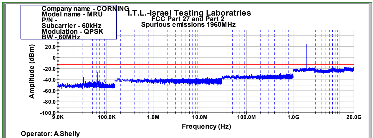
Figure 1062: Spurious Emissions at Antenna Terminal QPSK 60MHz B.W.; 1960.0MHz, 60kHz
