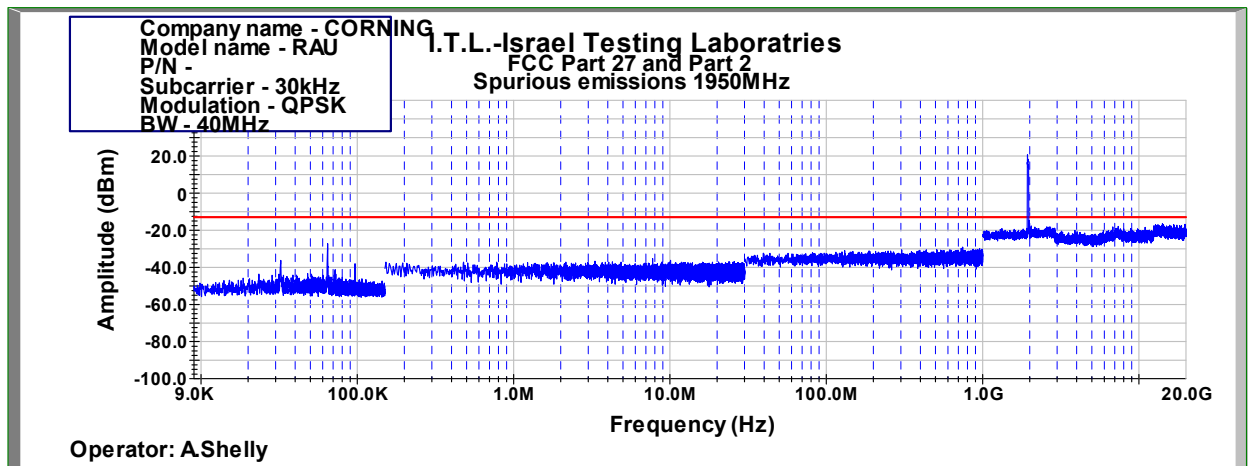
Figure 1044: Spurious Emissions at Antenna Terminal QPSK 40MHz B.W.; 1950.0MHz, 30kHz
