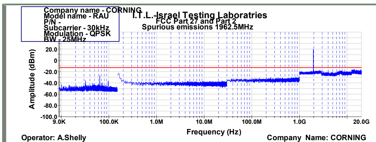
Figure 1036: Spurious Emissions at Antenna Terminal QPSK 25MHz B.W.; 1962.5MHz, 30kHz
