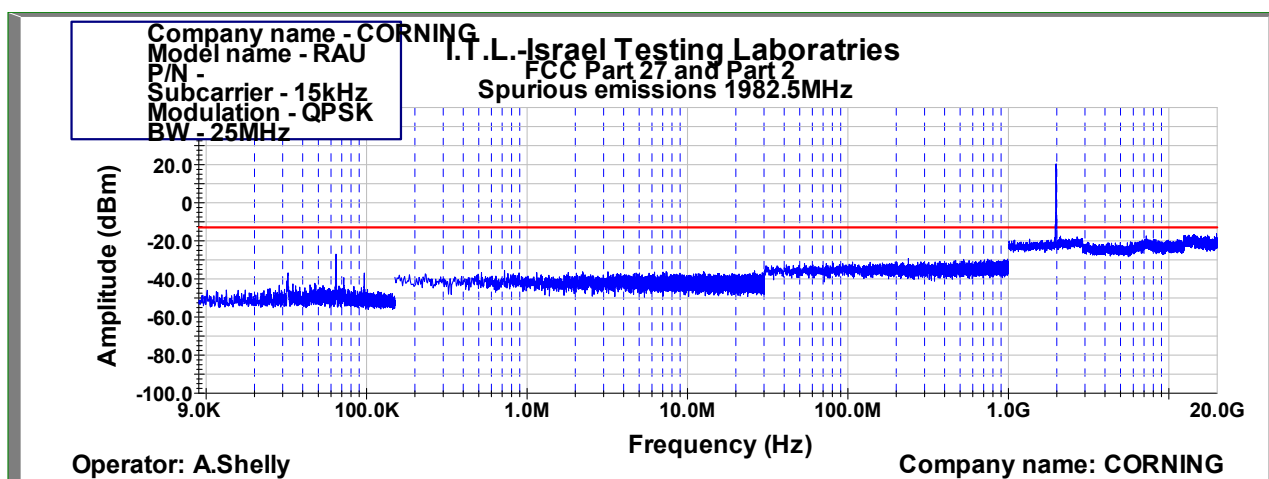
Figure 1034: Spurious Emissions at Antenna Terminal QPSK 25MHz B.W.; 1982.5MHz, 15kHz
