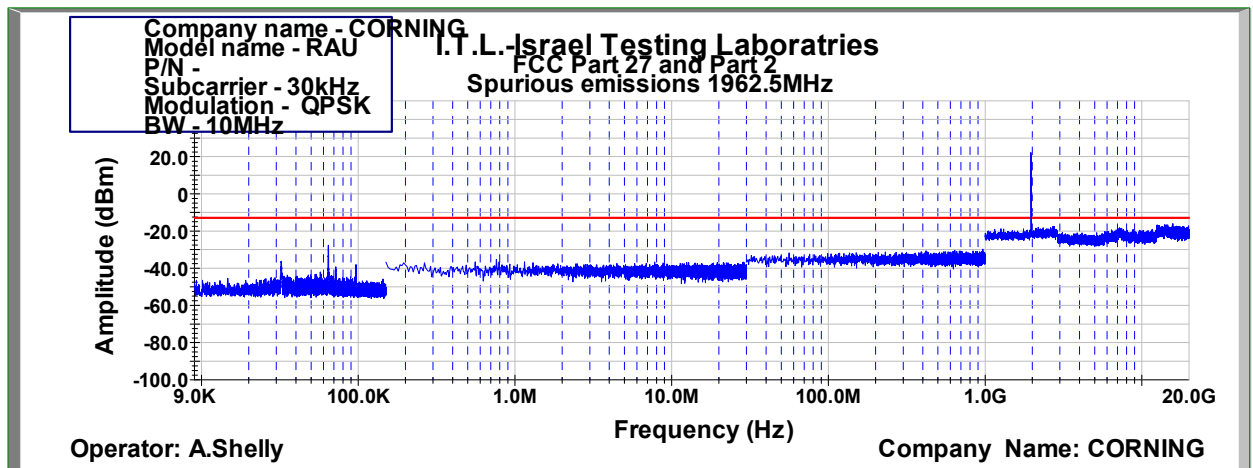
Figure 1009: Spurious Emissions at Antenna Terminal QPSK 10MHz B.W.; 1962.5MHz, 30kHz
