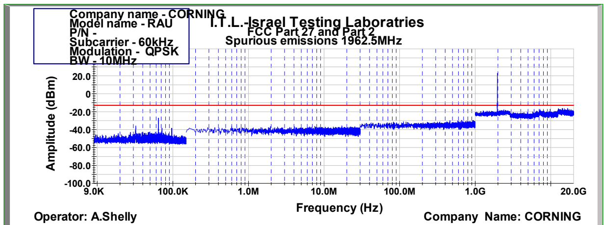
Figure 1012: Spurious Emissions at Antenna Terminal QPSK 10MHz B.W.; 1962.5MHz, 60kHz
