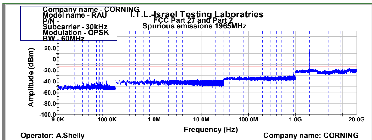
Figure 1061: Spurious Emissions at Antenna Terminal QPSK 60MHz B.W.; 1965.0MHz, 30kHz
