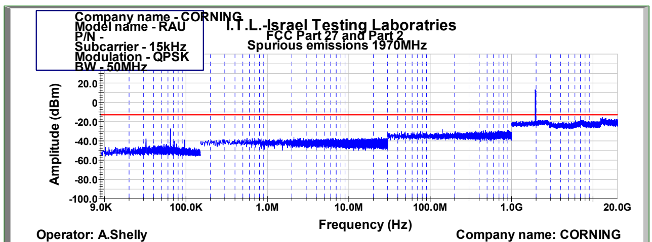
Figure 1052: Spurious Emissions at Antenna Terminal QPSK 50MHz B.W.; 1970.0MHz, 15kHz
