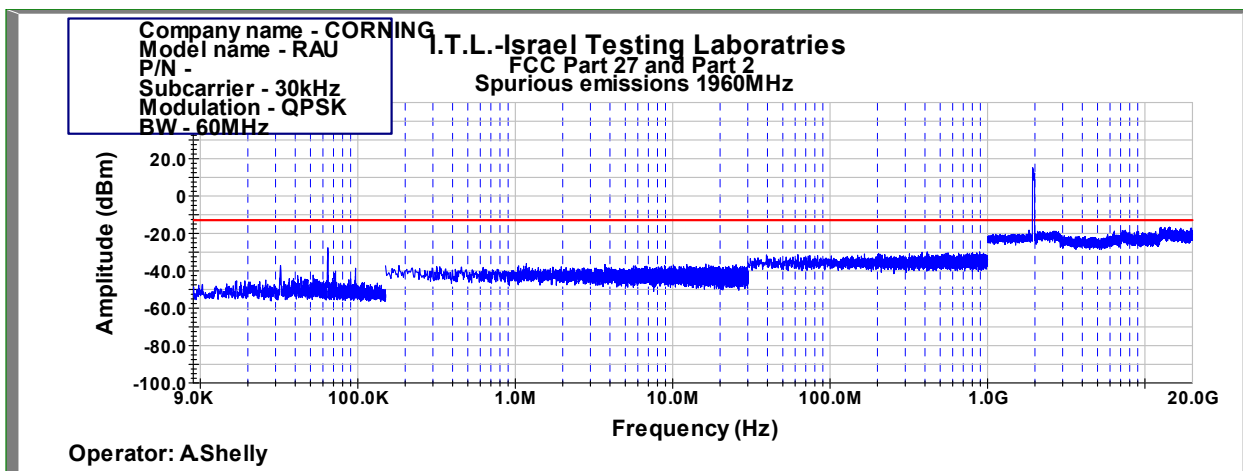
Figure 1059: Spurious Emissions at Antenna Terminal QPSK 60MHz B.W.; 1960.0MHz, 30kHz
