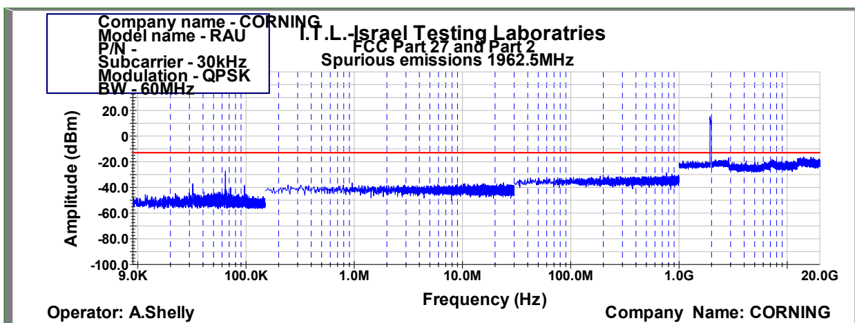
Figure 1060: Spurious Emissions at Antenna Terminal QPSK 60MHz B.W.; 1962.5MHz, 30kHz
