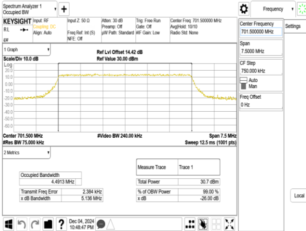
Band12_5MHz_64QAM_RB25_0_CH23035
