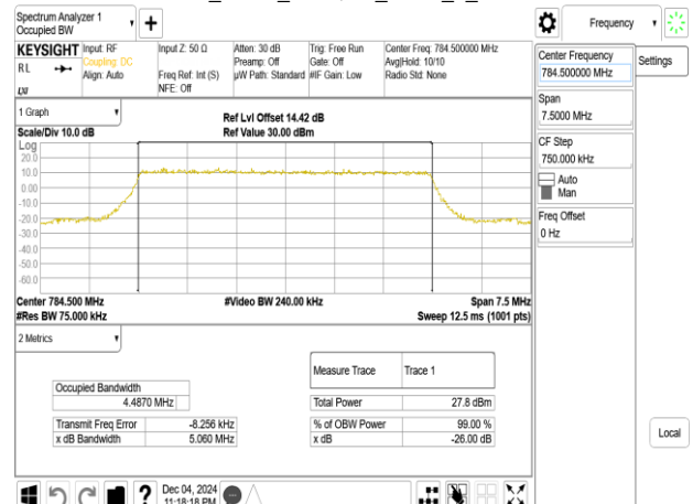
Band13_5MHz_256QAM_RB25_0_CH23255
