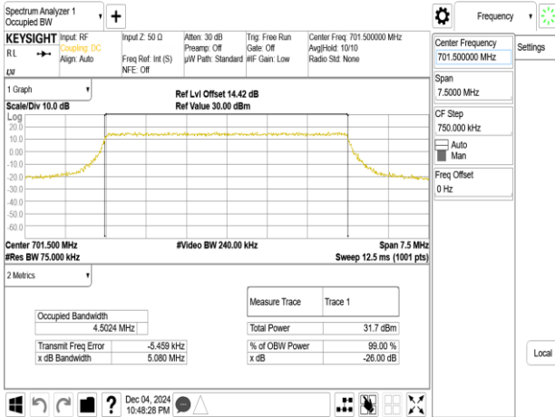
Band12_5MHz_16QAM_RB25_0_CH23035
