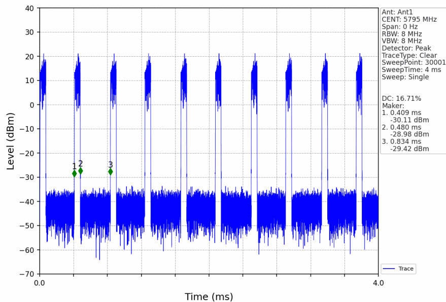
802.11ac(VHT40)_HCH_5795MHz_Ant1_NTNV
