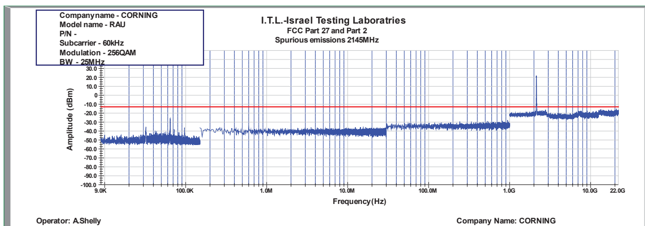
Figure 973: Spurious Emissions at Antenna Terminal 256QAM 25MHz B.W.; 2145.0MHz, 60kHz
