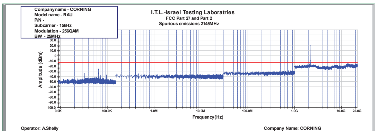
Figure 967: Spurious Emissions at Antenna Terminal 256QAM 25MHz B.W.; 2145.0MHz, 15kHz
