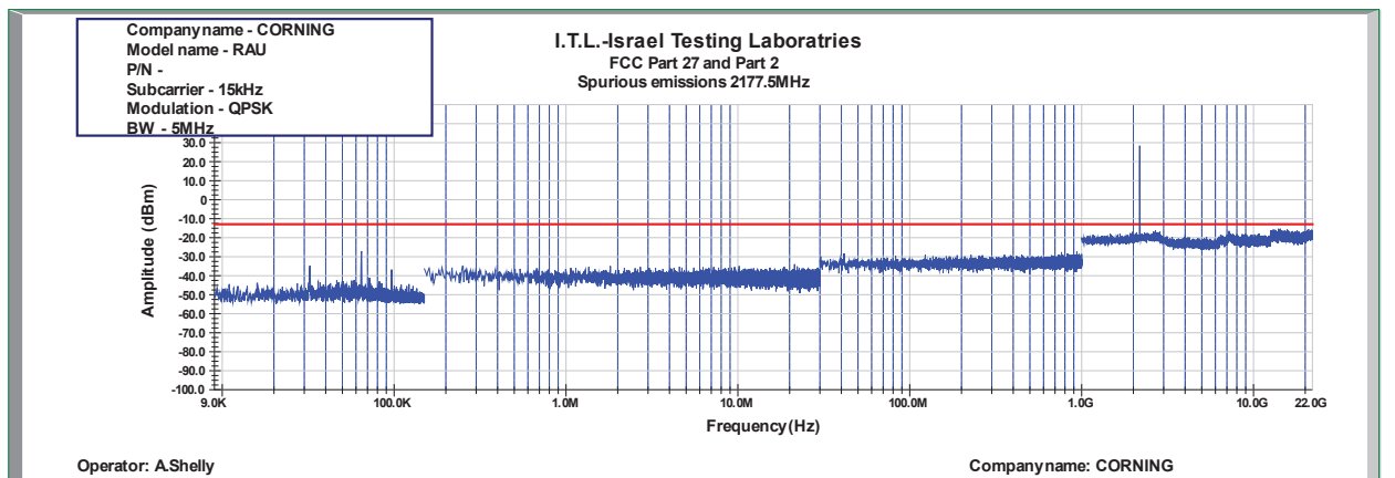
Figure 1001: Spurious Emissions at Antenna Terminal QPSK 5MHz B.W.; 2177.5MHz, 15kHz
