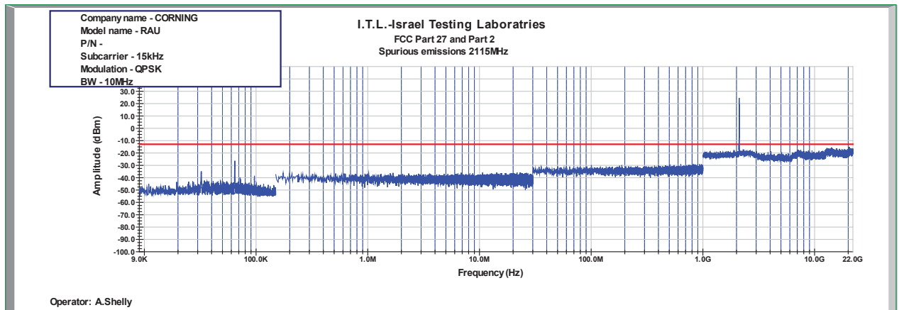
Figure 1005: Spurious Emissions at Antenna Terminal QPSK 10MHz B.W.; 2115.0MHz, 15kHz
