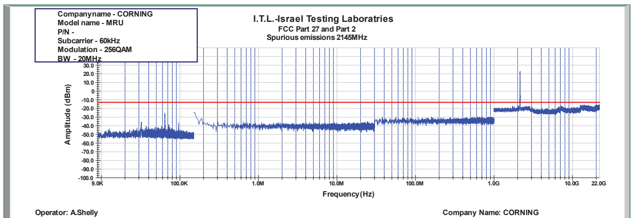
Figure 964: Spurious Emissions at Antenna Terminal 256QAM 20MHz B.W.; 2145.0MHz, 60kHz
