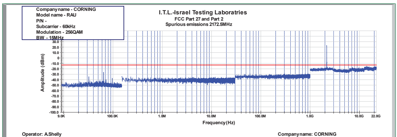
Figure 956: Spurious Emissions at Antenna Terminal 256QAM 15MHz B.W.; 2172.5MHz, 60kHz
