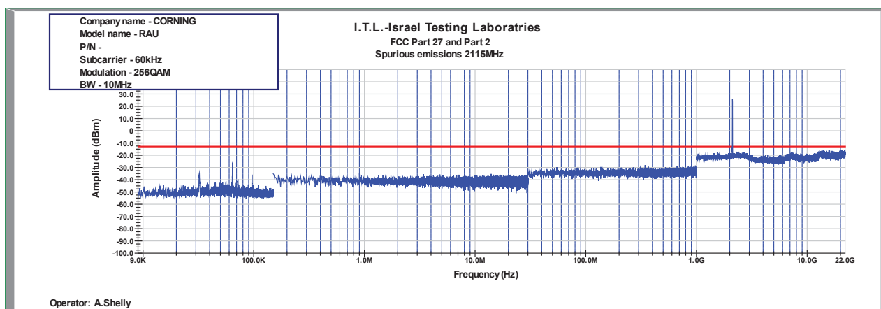
Figure 945: Spurious Emissions at Antenna Terminal 256QAM 10MHz B.W.; 2115.0MHz, 60kHz
