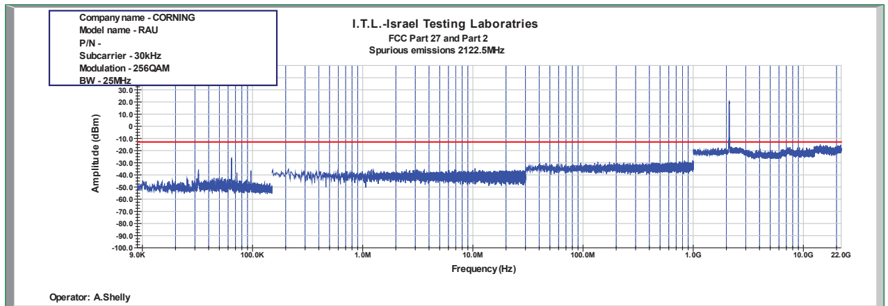
Figure 969: Spurious Emissions at Antenna Terminal 256QAM 25MHz B.W.; 2122.5MHz, 30kHz
