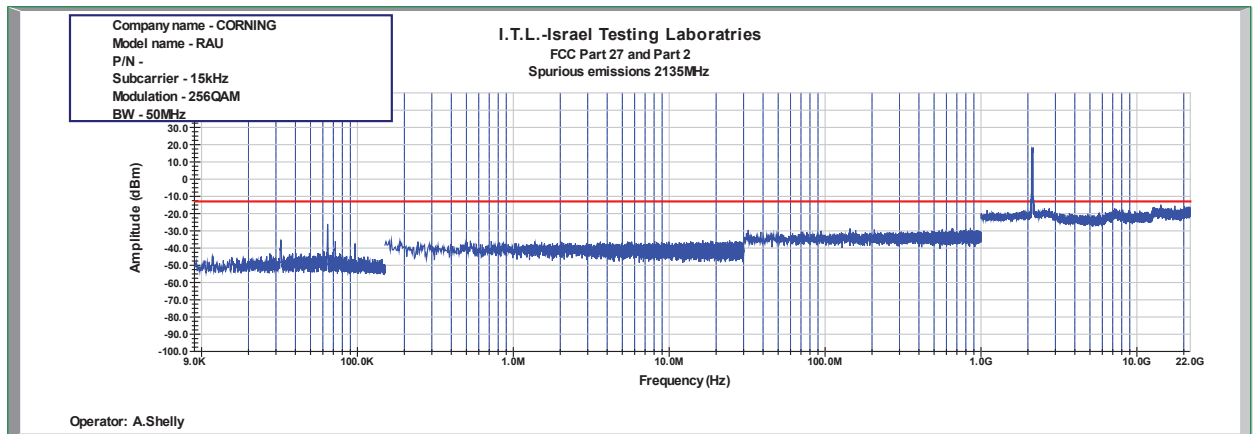
Figure 984: Spurious Emissions at Antenna Terminal 256QAM 50MHz B.W.; 2135.0MHz, 15kHz
