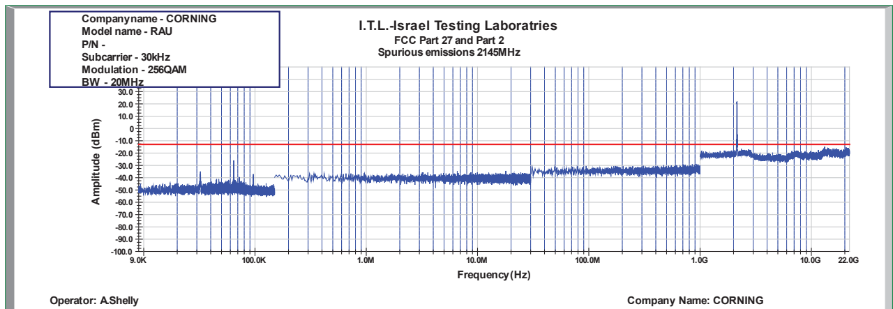
Figure 961: Spurious Emissions at Antenna Terminal 256QAM 20MHz B.W.; 2145.0MHz, 30kHz
