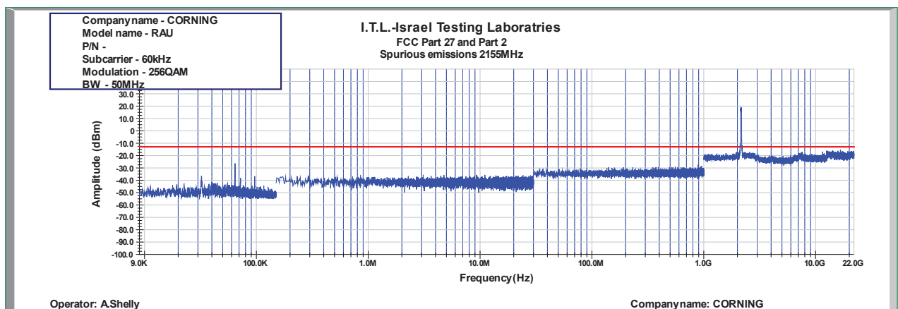
Figure 992: Spurious Emissions at Antenna Terminal 256QAM 50MHz B.W.; 2155.0MHz, 60kHz
