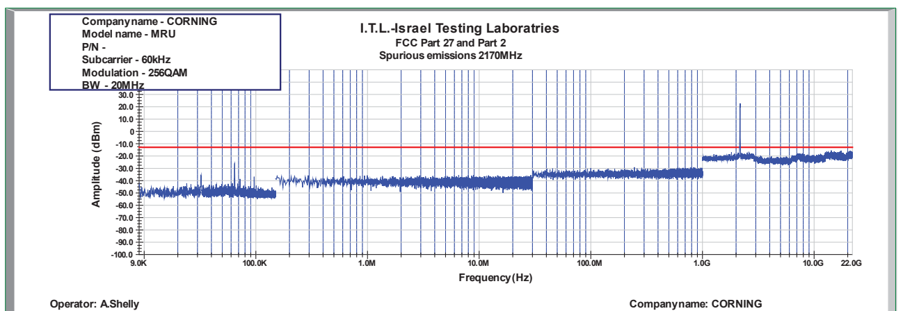
Figure 965: Spurious Emissions at Antenna Terminal 256QAM 20MHz B.W.; 2170.0MHz, 60kHz
