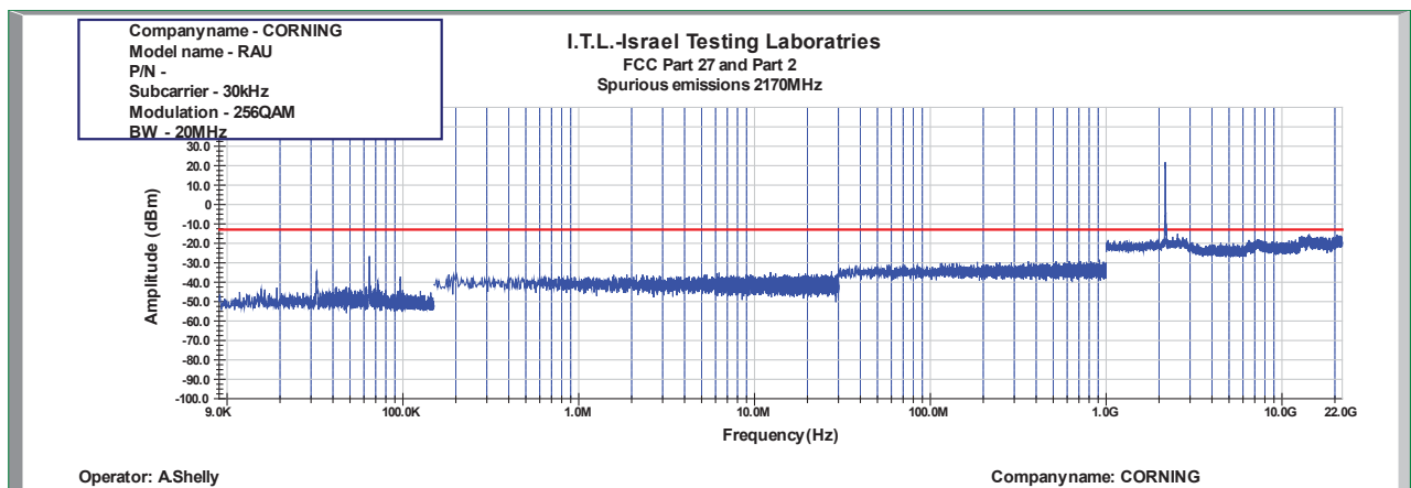
Figure 962: Spurious Emissions at Antenna Terminal 256QAM 20MHz B.W.; 2170.0MHz, 30kHz
