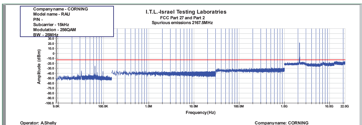
Figure 968: Spurious Emissions at Antenna Terminal 256QAM 25MHz B.W.; 2167.5MHz, 15kHz
