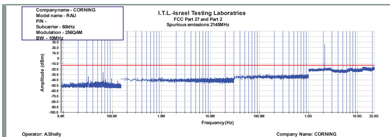
Figure 946: Spurious Emissions at Antenna Terminal 256QAM 10MHz B.W.; 2145.0MHz, 60kHz
