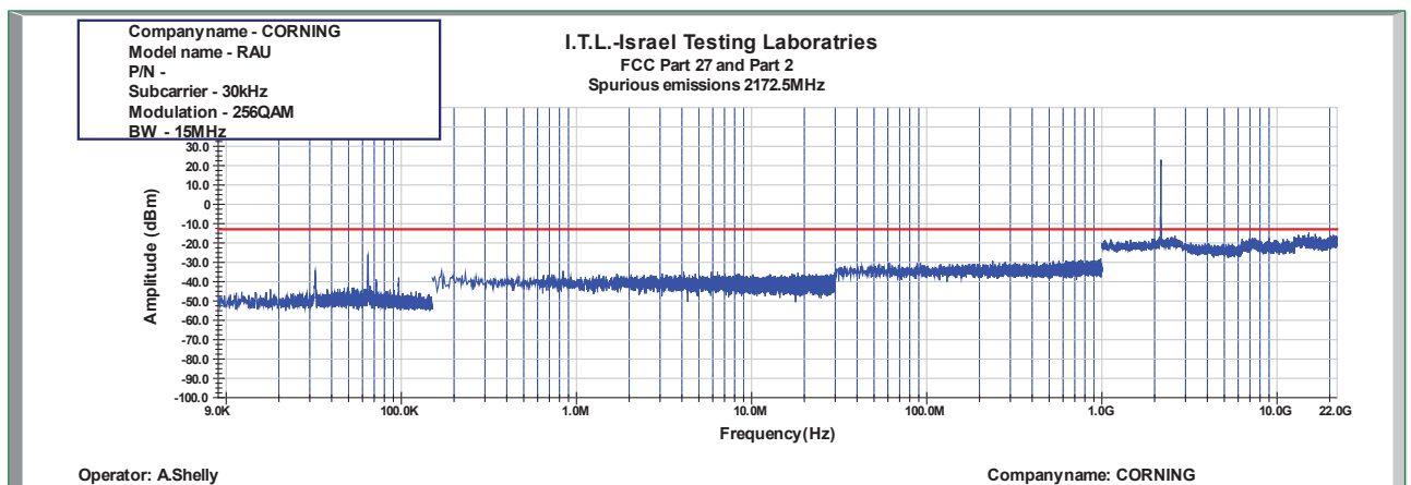
Figure 953: Spurious Emissions at Antenna Terminal 256QAM 15MHz B.W.; 2172.5MHz, 30kHz
