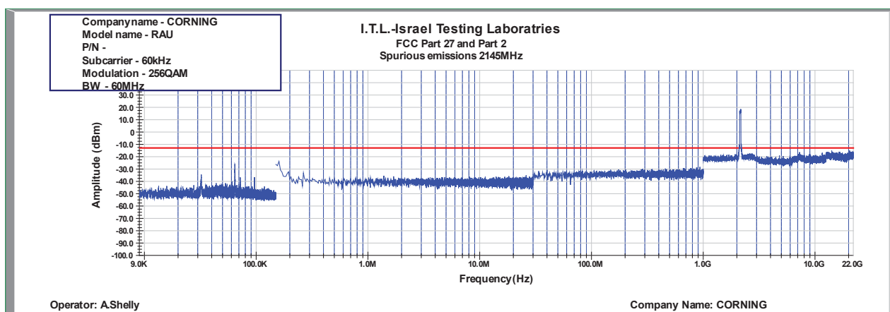
Figure 997: Spurious Emissions at Antenna Terminal 256QAM 60MHz B.W.; 2145.0MHz, 60kHz
