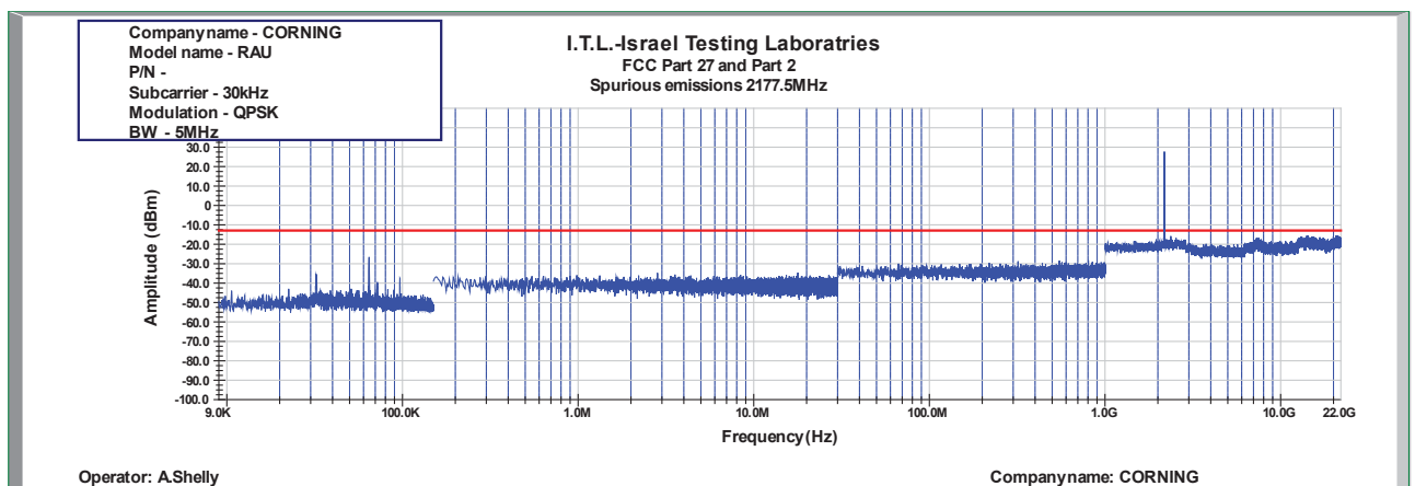
Figure 1004: Spurious Emissions at Antenna Terminal QPSK 5MHz B.W.; 2177.5MHz, 30kHz
