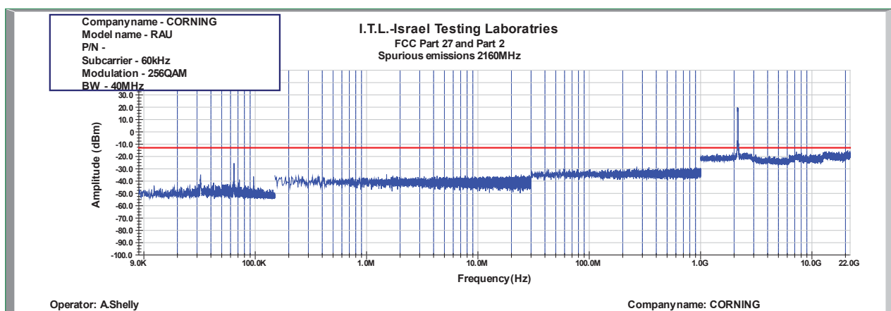
Figure 983: Spurious Emissions at Antenna Terminal 256QAM 40MHz B.W.; 2160.0MHz, 60kHz
