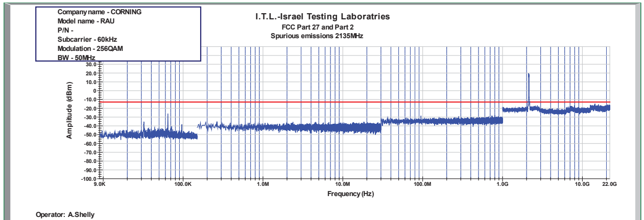
Figure 990: Spurious Emissions at Antenna Terminal 256QAM 50MHz B.W.; 2135.0MHz, 60kHz
