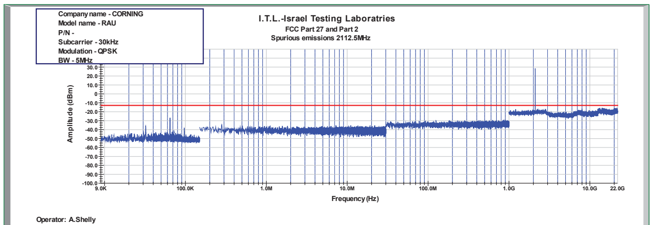
Figure 1002: Spurious Emissions at Antenna Terminal QPSK 5MHz B.W.; 2112.5MHz, 30kHz
