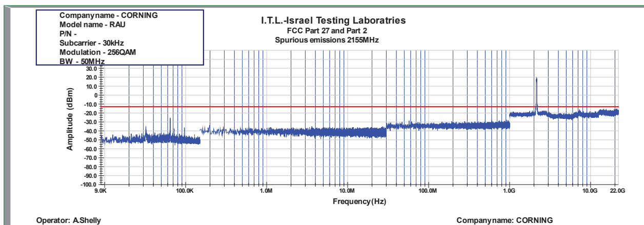
Figure 989: Spurious Emissions at Antenna Terminal 256QAM 50MHz B.W.; 2155.0MHz, 30kHz
