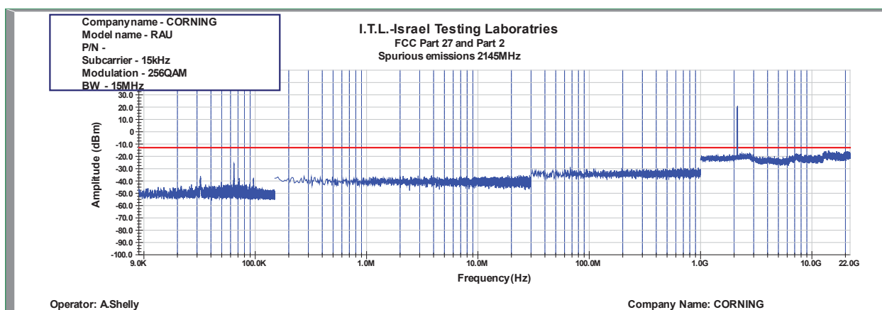
Figure 949: Spurious Emissions at Antenna Terminal 256QAM 15MHz B.W.; 2145.0MHz, 15kHz
