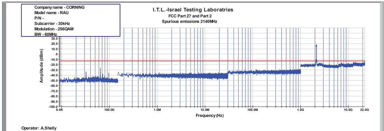
Figure 993: Spurious Emissions at Antenna Terminal 256QAM 60MHz B.W.; 2140.0MHz, 30kHz
