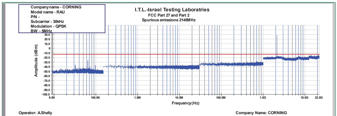
Figure 1003: Spurious Emissions at Antenna Terminal QPSK 5MHz B.W.; 2145.0MHz, 30kHz
