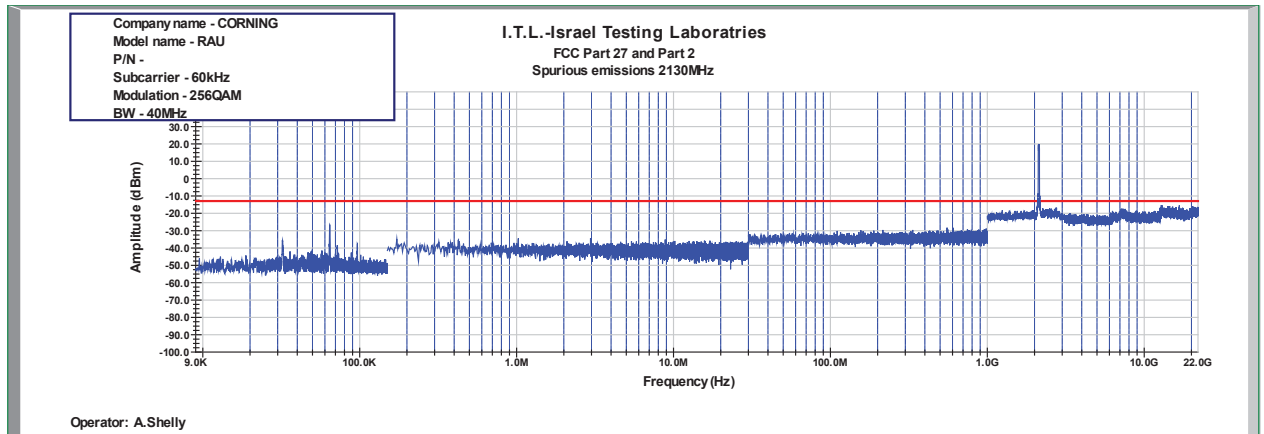
Figure 981: Spurious Emissions at Antenna Terminal 256QAM 40MHz B.W.; 2130.0MHz, 60kHz
