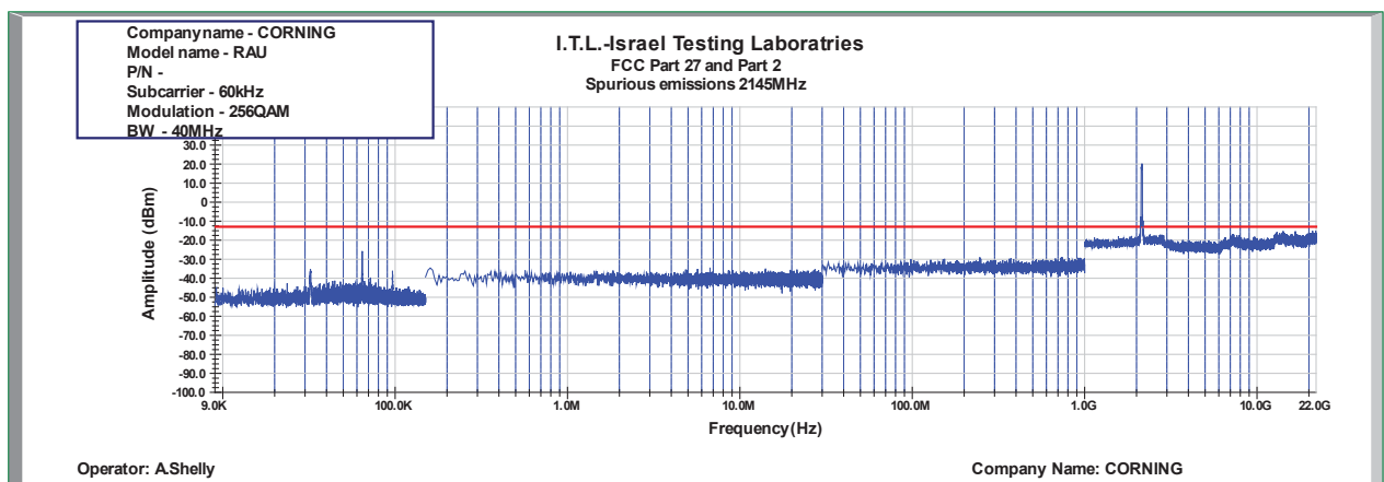
Figure 982: Spurious Emissions at Antenna Terminal 256QAM 40MHz B.W.; 2145.0MHz, 60kHz
