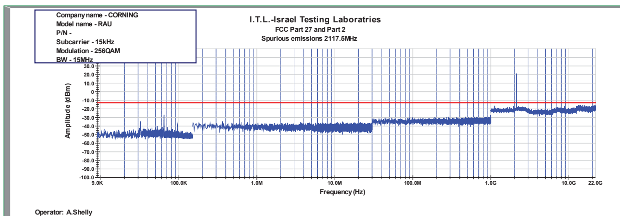
Figure 948: Spurious Emissions at Antenna Terminal 256QAM 15MHz B.W.; 2117.5MHz, 15kHz
