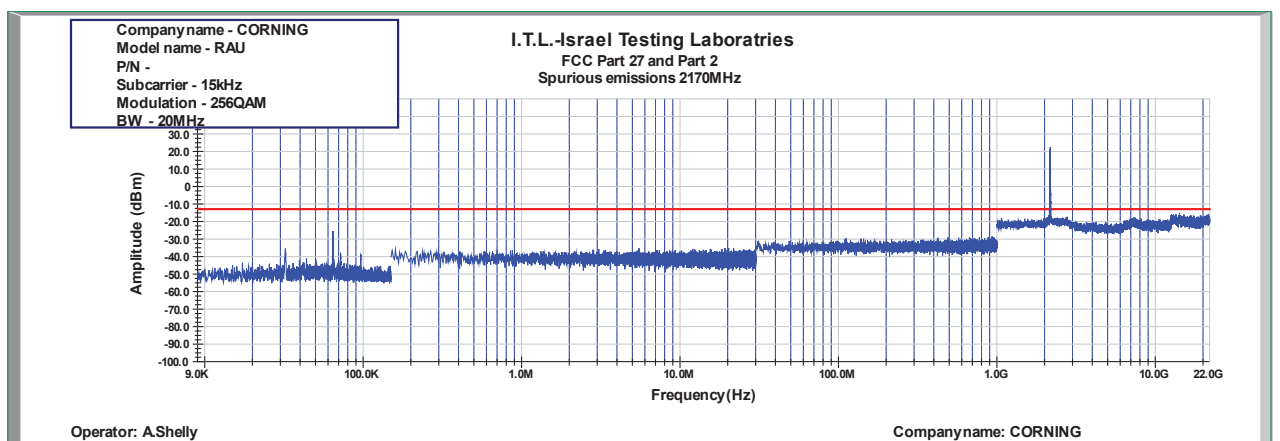
Figure 959: Spurious Emissions at Antenna Terminal 256QAM 20MHz B.W.; 2170.0MHz, 15kHz
