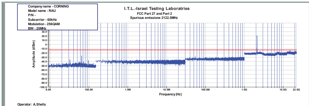
Figure 972: Spurious Emissions at Antenna Terminal 256QAM 25MHz B.W.; 2122.5MHz, 60kHz
