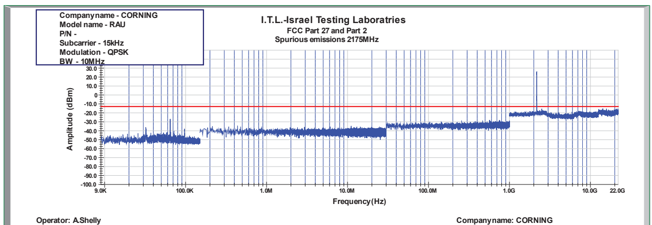
Figure 1007: Spurious Emissions at Antenna Terminal QPSK 10MHz B.W.; 2175.0MHz, 15kHz
