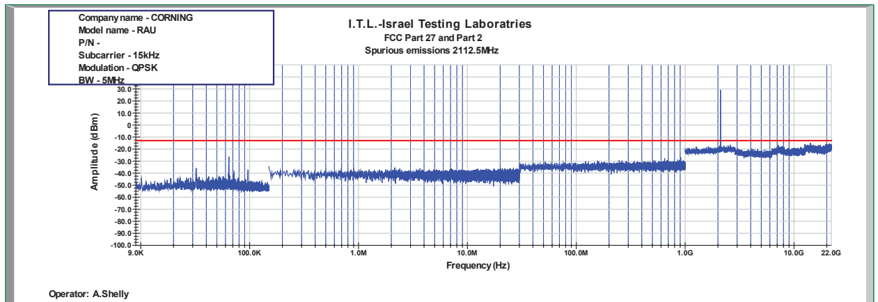
Figure 999: Spurious Emissions at Antenna Terminal QPSK 5MHz B.W.; 2112.5MHz, 15kHz
