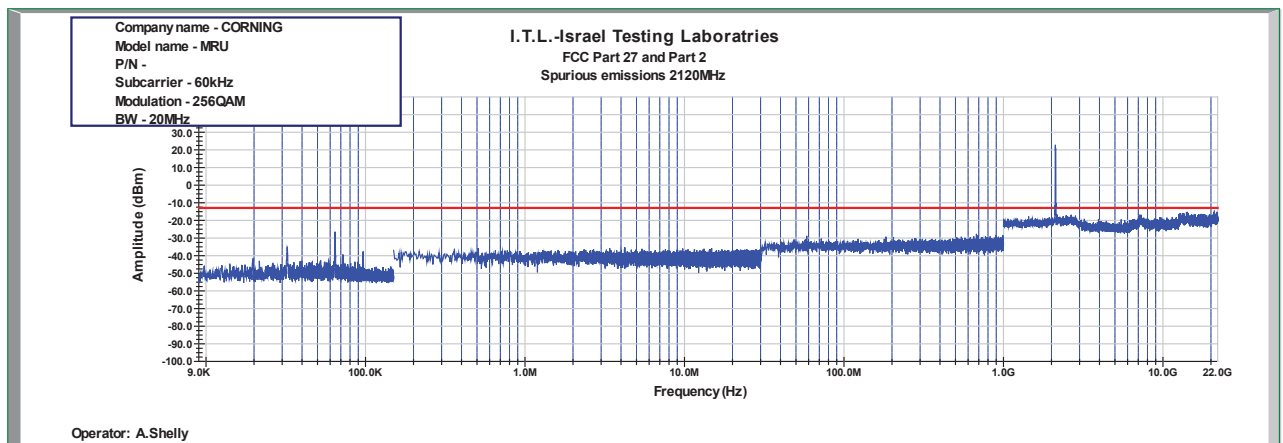
Figure 963: Spurious Emissions at Antenna Terminal 256QAM 20MHz B.W.; 2120.0MHz, 60kHz
