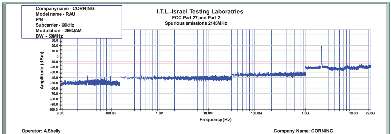
Figure 991: Spurious Emissions at Antenna Terminal 256QAM 50MHz B.W.; 2145.0MHz, 60kHz
