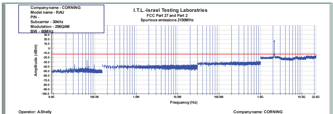
Figure 995: Spurious Emissions at Antenna Terminal 256QAM 60MHz B.W.; 2150.0MHz, 30kHz
