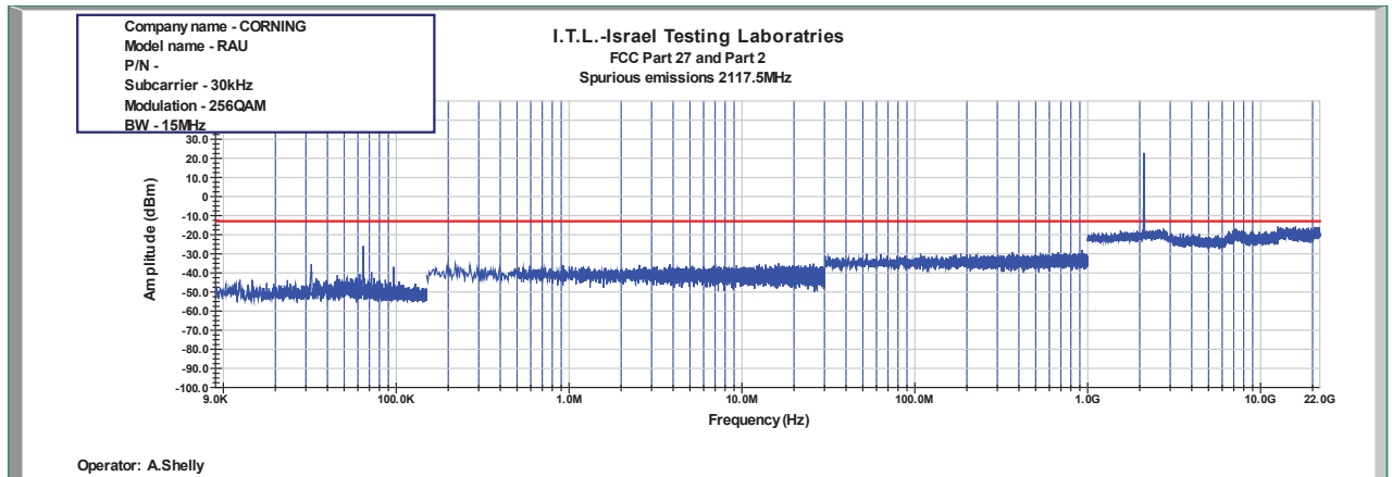
Figure 951: Spurious Emissions at Antenna Terminal 256QAM 15MHz B.W.; 2117.5MHz, 30kHz
