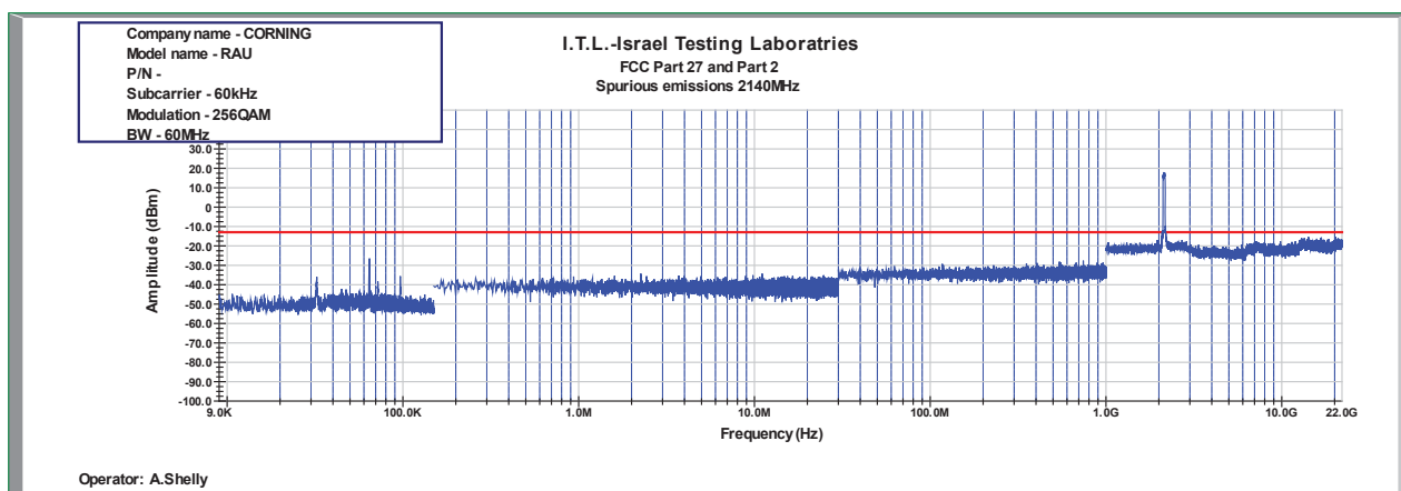
Figure 996: Spurious Emissions at Antenna Terminal 256QAM 60MHz B.W.; 2140.0MHz, 60kHz
