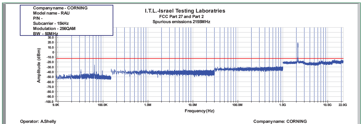
Figure 986: Spurious Emissions at Antenna Terminal 256QAM 50MHz B.W.; 2155.0MHz, 15kHz
