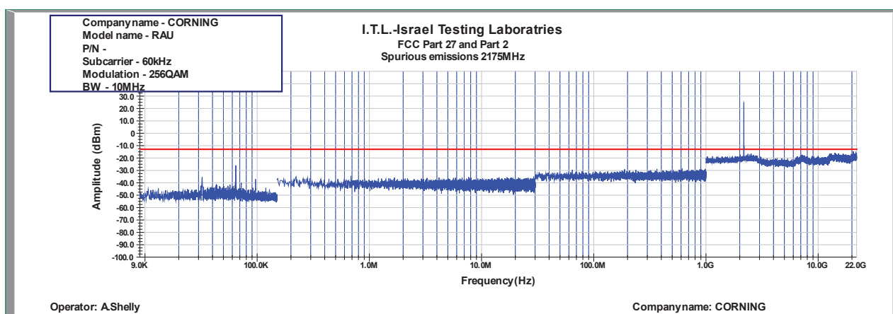
Figure 947: Spurious Emissions at Antenna Terminal 256QAM 10MHz B.W.; 2175.0MHz, 60kHz
