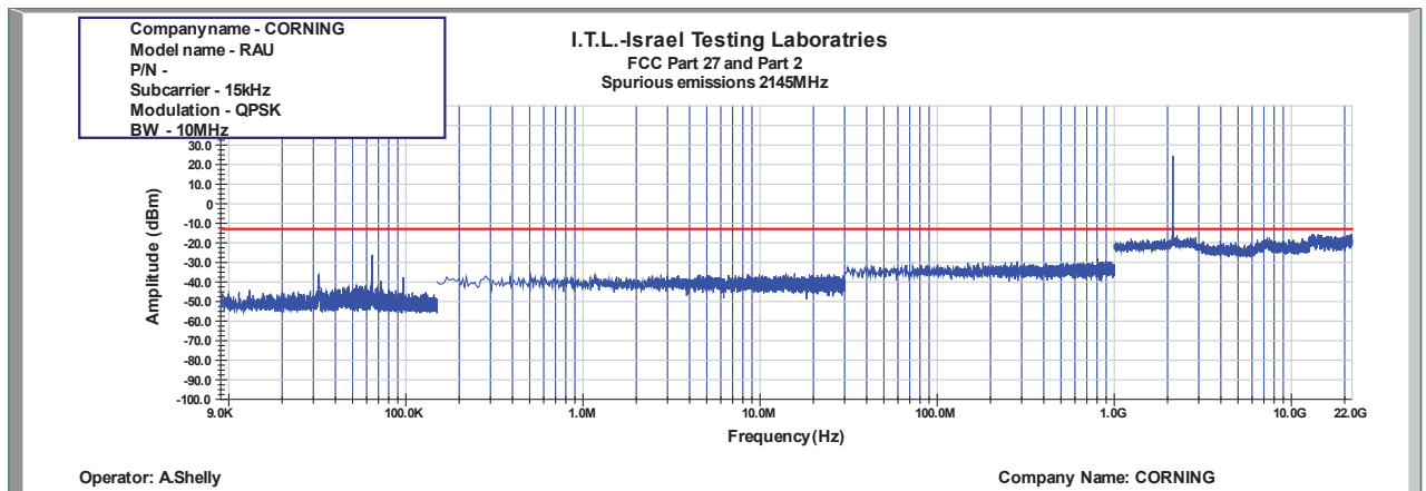
Figure 1006: Spurious Emissions at Antenna Terminal QPSK 10MHz B.W.; 2145.0MHz, 15kHz
