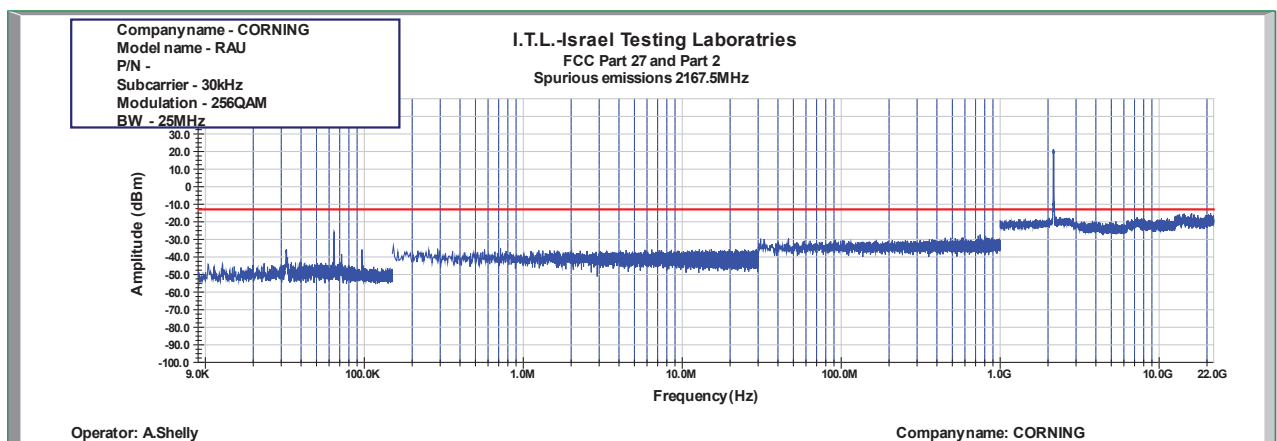
Figure 971: Spurious Emissions at Antenna Terminal 256QAM 25MHz B.W.; 2167.5MHz, 30kHz
