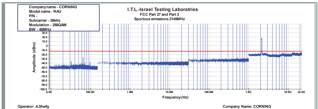
Figure 994: Spurious Emissions at Antenna Terminal 256QAM 60MHz B.W.; 2145.0MHz, 30kHz
