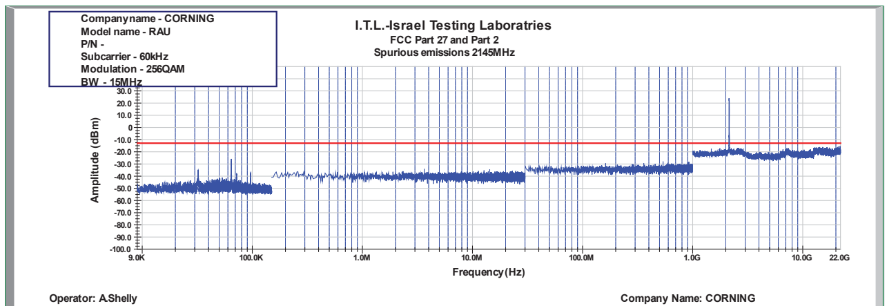
Figure 955: Spurious Emissions at Antenna Terminal 256QAM 15MHz B.W.; 2145.0MHz, 60kHz
