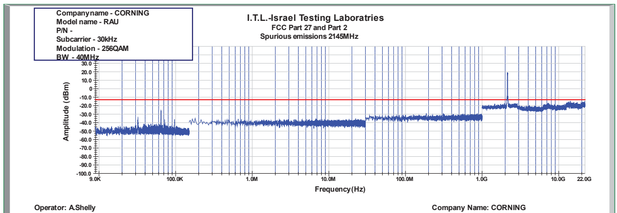
Figure 979: Spurious Emissions at Antenna Terminal 256QAM 40MHz B.W.; 2145.0MHz, 30kHz
