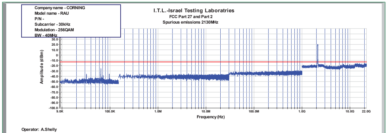
Figure 978: Spurious Emissions at Antenna Terminal 256QAM 40MHz B.W.; 2130.0MHz, 30kHz
