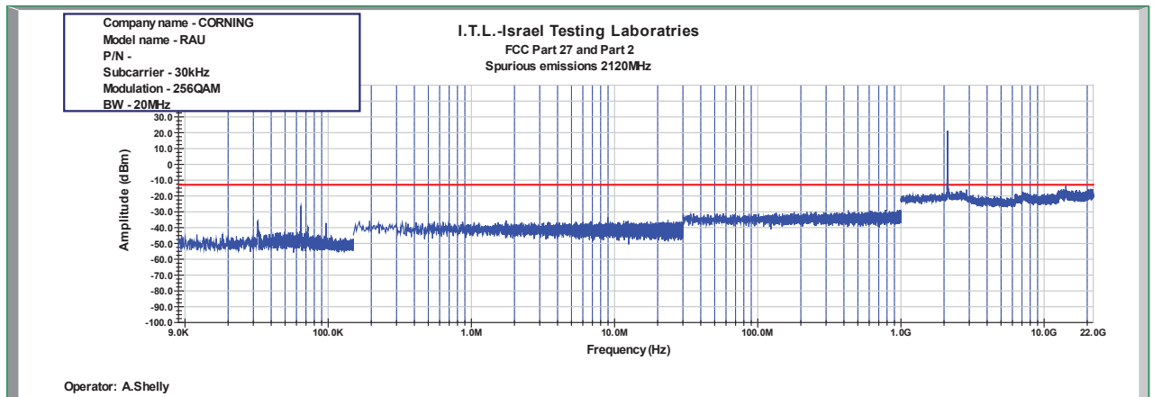
Figure 960: Spurious Emissions at Antenna Terminal 256QAM 20MHz B.W.; 2120.0MHz, 30kHz
