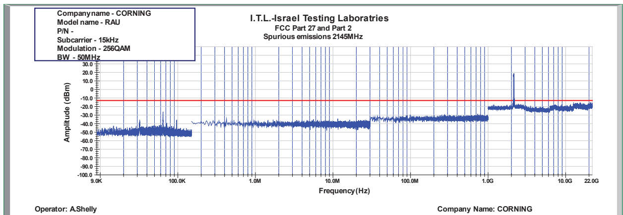
Figure 985: Spurious Emissions at Antenna Terminal 256QAM 50MHz B.W.; 2145.0MHz, 15kHz
