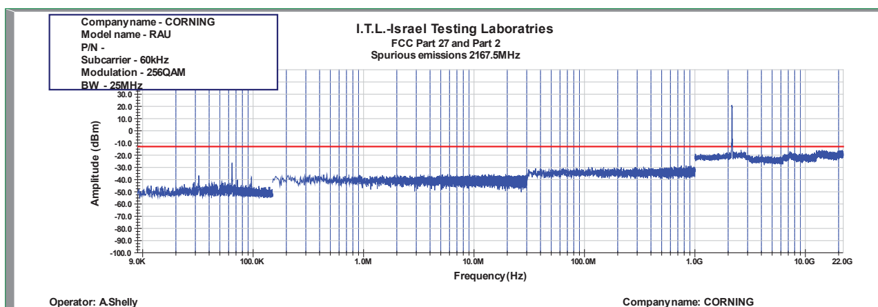
Figure 974: Spurious Emissions at Antenna Terminal 256QAM 25MHz B.W.; 2167.5MHz, 60kHz
