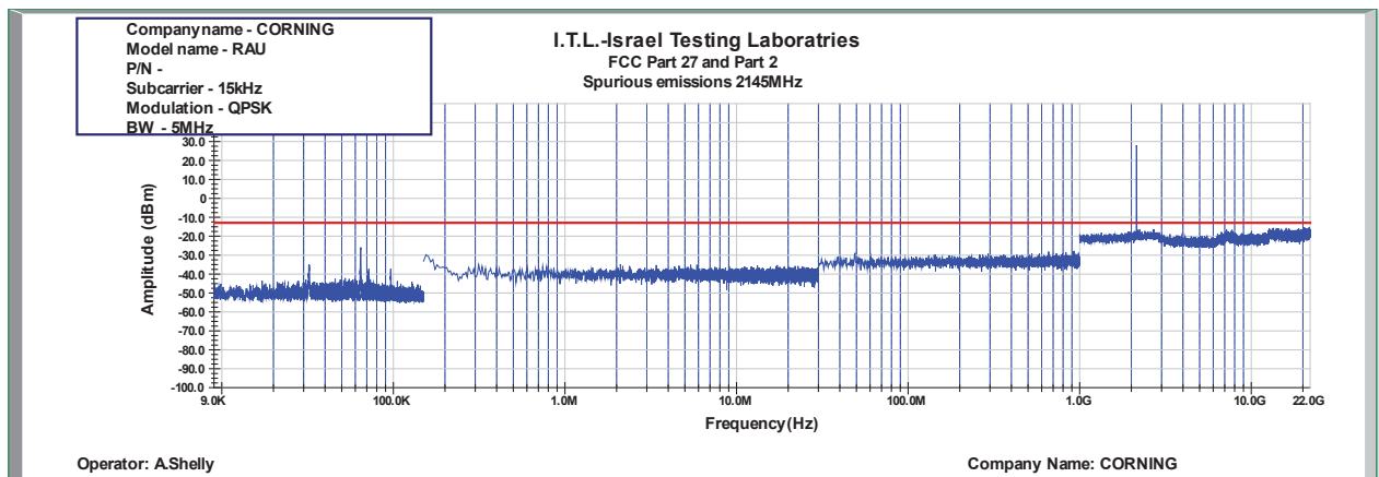
Figure 1000: Spurious Emissions at Antenna Terminal QPSK 5MHz B.W.; 2145.0MHz, 15kHz
