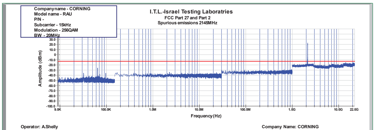
Figure 958: Spurious Emissions at Antenna Terminal 256QAM 20MHz B.W.; 2145.0MHz, 15kHz
