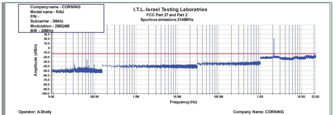
Figure 970: Spurious Emissions at Antenna Terminal 256QAM 25MHz B.W.; 2145.0MHz, 30kHz
