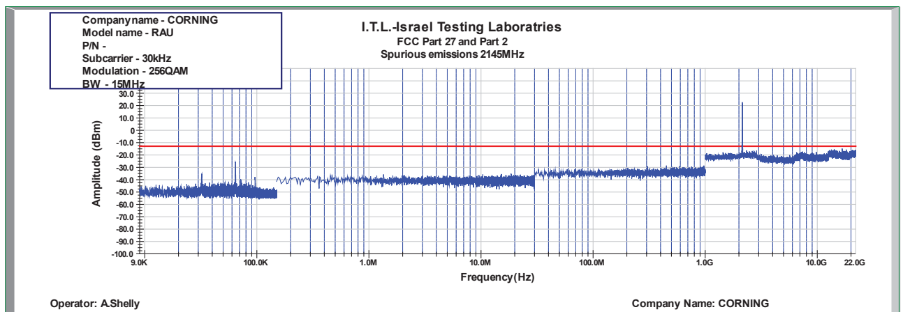
Figure 952: Spurious Emissions at Antenna Terminal 256QAM 15MHz B.W.; 2145.0MHz, 30kHz
