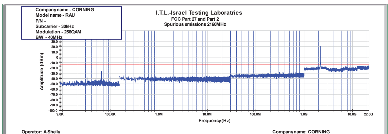
Figure 980: Spurious Emissions at Antenna Terminal 256QAM 40MHz B.W.; 2160.0MHz, 30kHz
