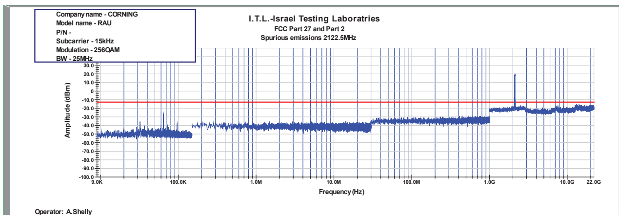
Figure 966: Spurious Emissions at Antenna Terminal 256QAM 25MHz B.W.; 2122.5MHz, 15kHz
