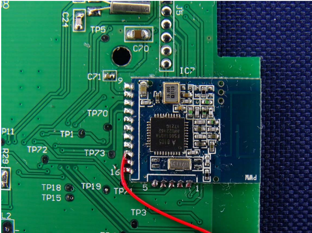
(21) EUT Photo (Module & Antenna)
