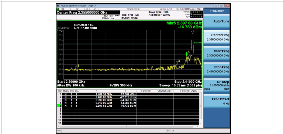
2.4G-Ant2-2402.4-PASS
