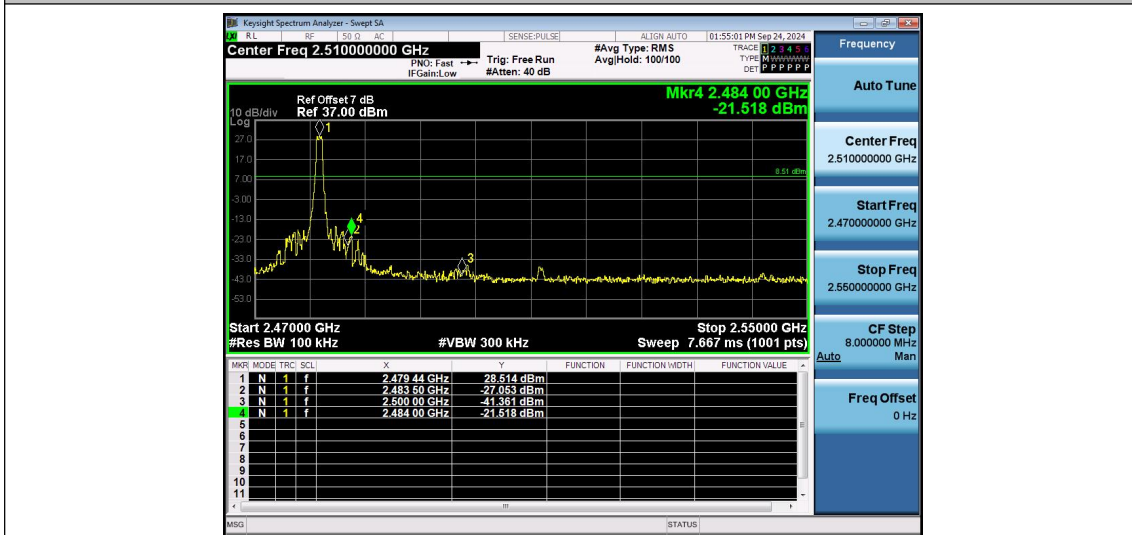
2.4G-Ant2-2479.4-PASS
