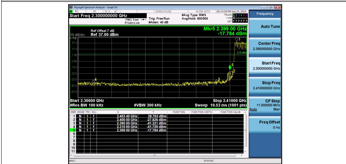
2.4G-Ant2-Hop-PASS
