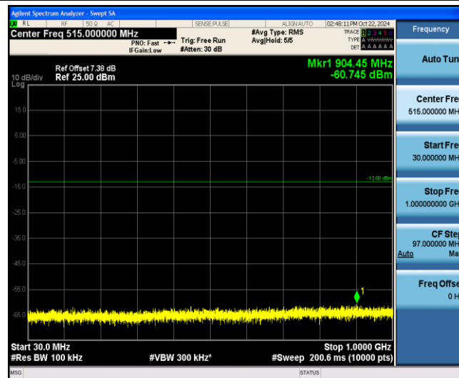
Band4-15MHz-16QAM-20325-1-0-Low-30-1000--60.75-PASS
