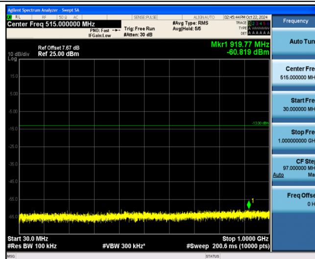
Band4-15MHz-16QAM-20025-1-0-Low-30-1000--60.82-PASS
