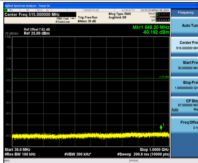
Band25-3MHz-16QAM-26055-1-0-Low-30-1000--60.19-PASS
