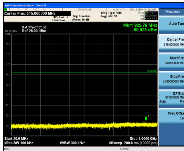
Band4-20MHz-16QAM-20050-1-0-Low-30-1000--60.52-PASS
