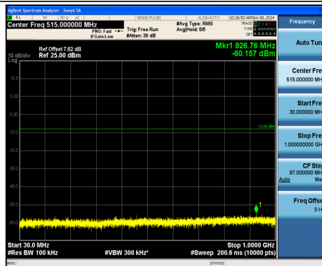
Band25-1.4MHz-16QAM-26365-1-0-Low-30-1000--60.16-PASS
