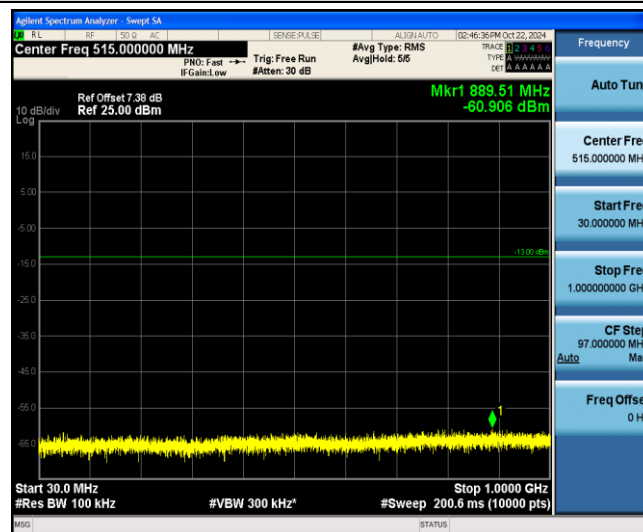
Band4-15MHz-QPSK-20175-1-0-Low-30-1000--60.91-PASS
