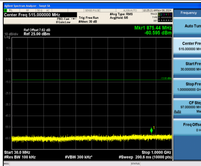
Band25-1.4MHz-QPSK-26047-1-0-Low-30-1000--60.6-PASS
