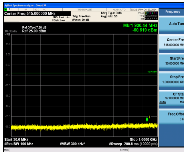
Band4-10MHz-16QAM-20350-1-0-Low-30-1000--60.62-PASS
