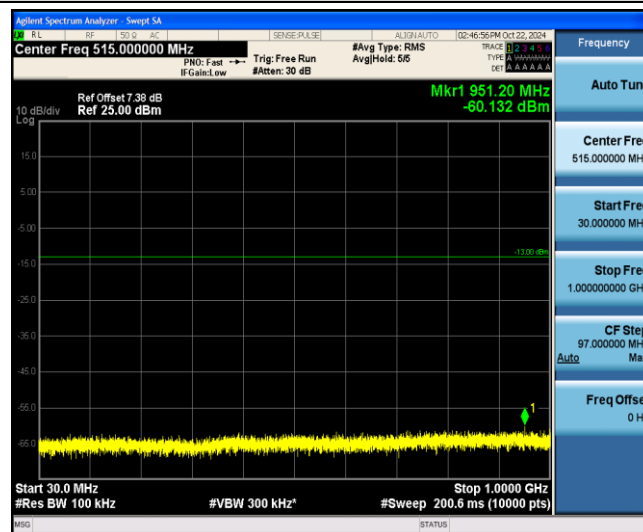
Band4-15MHz-16QAM-20175-1-0-Low-30-1000--60.13-PASS
