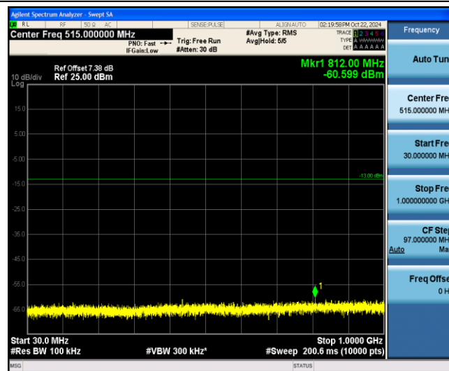
Band4-10MHz-16QAM-20175-1-0-Low-30-1000--60.6-PASS
