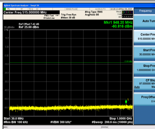
Band25-1.4MHz-16QAM-26683-1-0-High-30-1000--60.82-PASS
