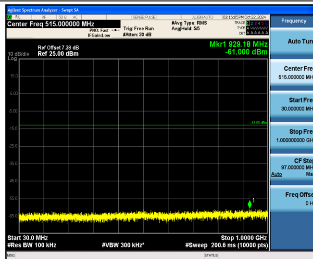
Band4-20MHz-QPSK-20175-1-0-Low-30-1000--61-PASS
