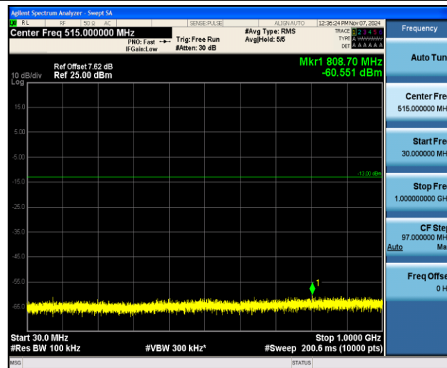
Band25-5MHz-QPSK-26065-1-0-Low-30-1000--60.55-PASS
