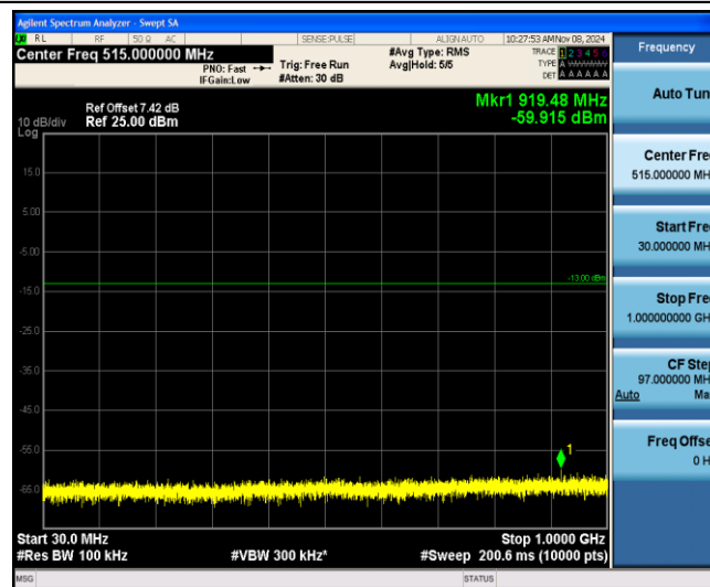
Band25-1.4MHz-QPSK-26683-1-0-High-30-1000--59.92-PASS
