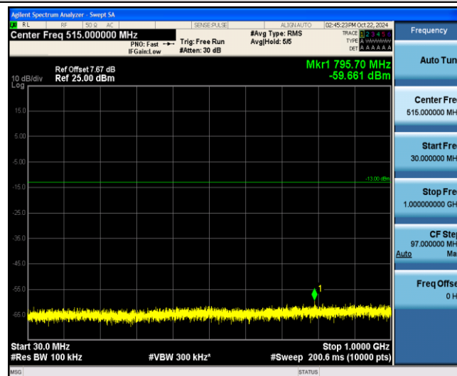
Band4-15MHz-QPSK-20025-1-0-Low-30-1000--59.66-PASS
