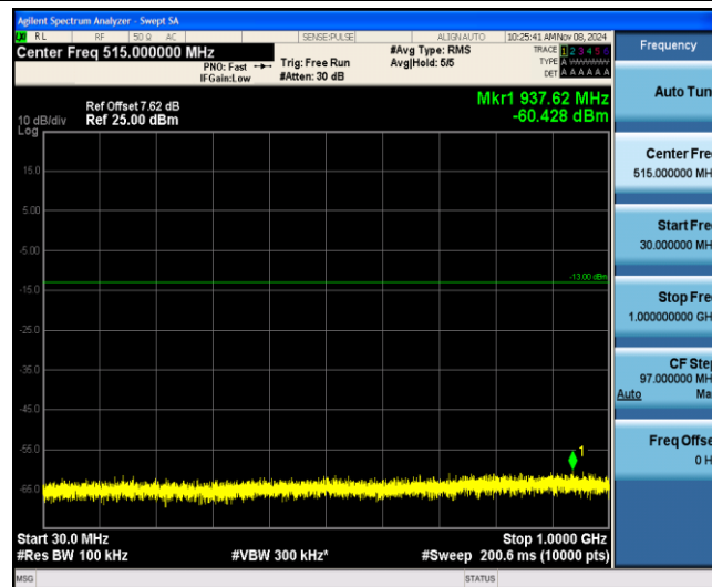
Band25-1.4MHz-16QAM-26047-1-0-Low-30-1000--60.43-PASS
