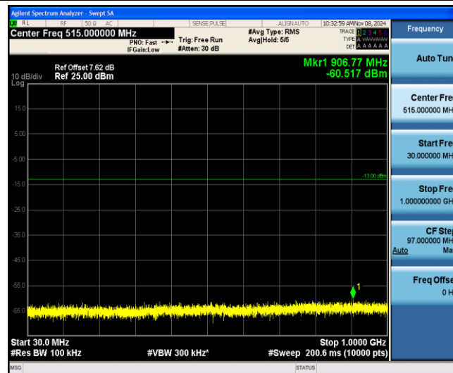
Band25-3MHz-QPSK-26055-1-0-Low-30-1000--60.52-PASS
