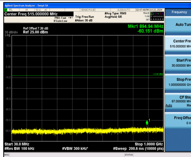
Band4-15MHz-QPSK-20325-1-0-Low-30-1000--60.15-PASS
