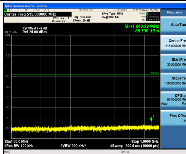
Band25-3MHz-16QAM-26675-1-0-Low-30-1000--58.7-PASS
