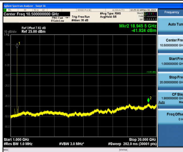
Band25-1.4MHz-QPSK-26047-1-0-Low-1000-20000--41.92-PASS
