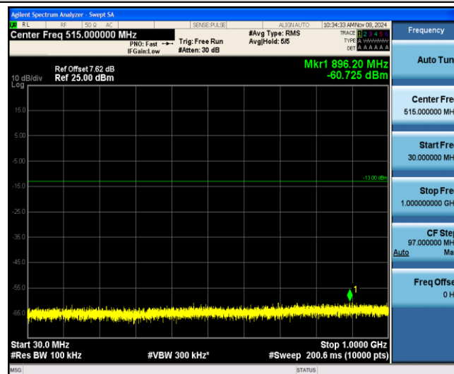
Band25-3MHz-16QAM-26365-1-0-Low-30-1000--60.73-PASS
