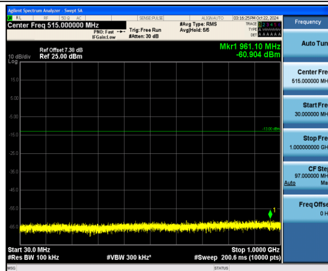
Band4-20MHz-16QAM-20175-1-0-Low-30-1000--60.9-PASS
